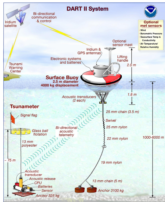
Figure 11. Schematic of the DART™ system.
