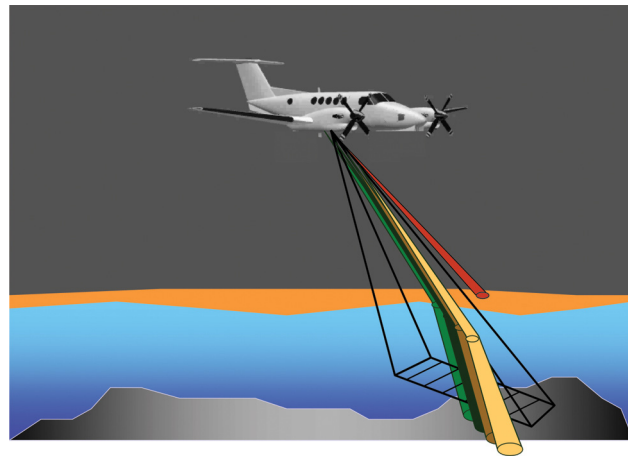
Figure 25. Airborne LiDAR data collection.
