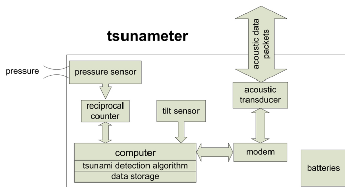
Figure 14. Block diagram of DART™ Bottom Pressure Recorder adapted from Meinig et al., 2005a.
