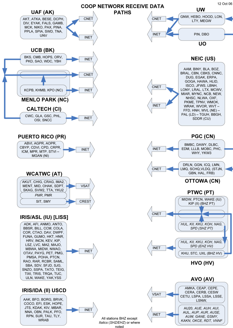
Figure 35. TWC cooperative seismic data transmission paths.
