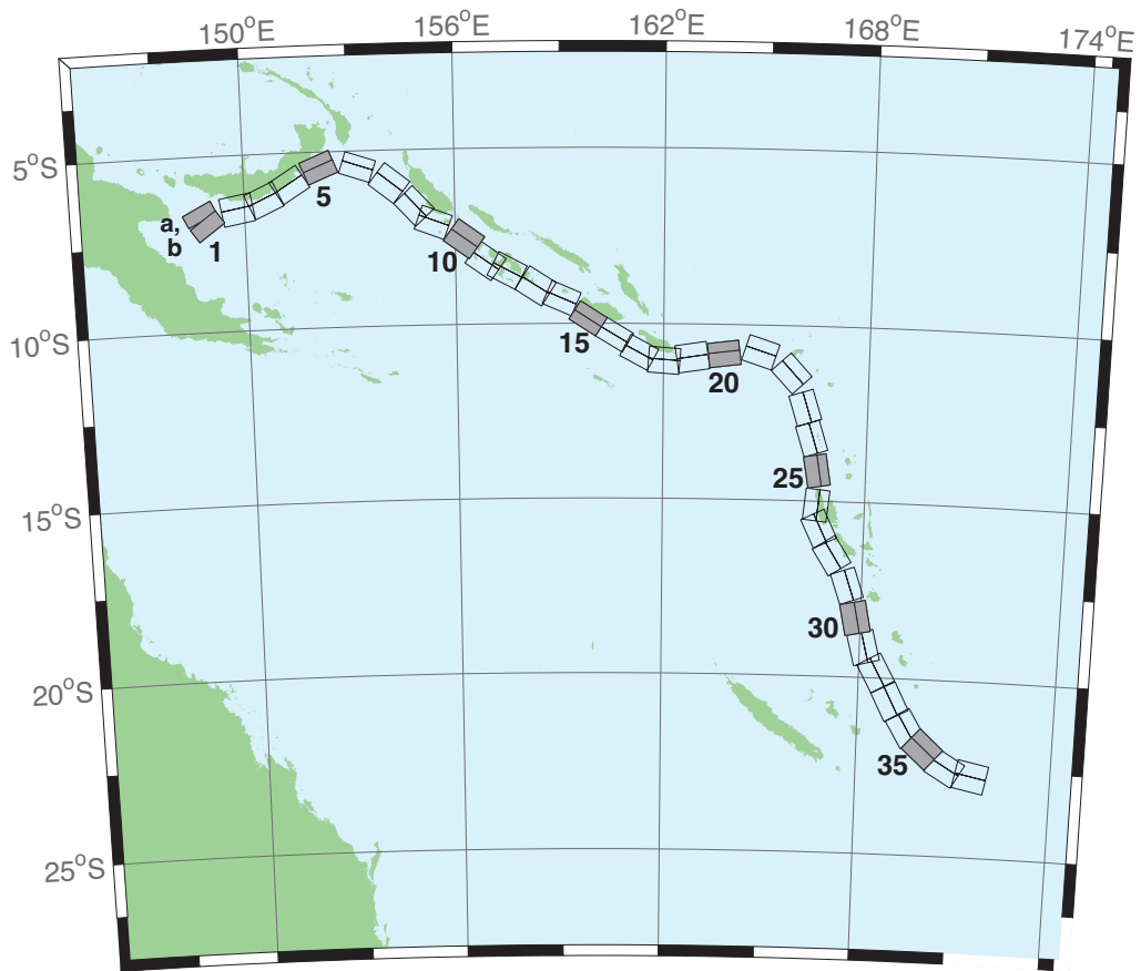
Figure 42: New Britain–Solomons–Vanuatu Zone unit sources.
