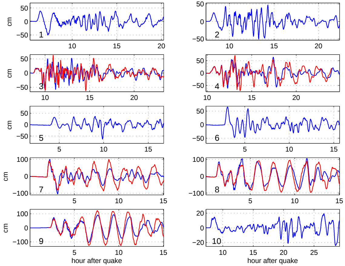
Figure 25: Time histories at the virtual gage on Japonski island, according to Forecast Model (blue) and Reference Model (red), in Mega events 1-10 (as numbered in the plots).
