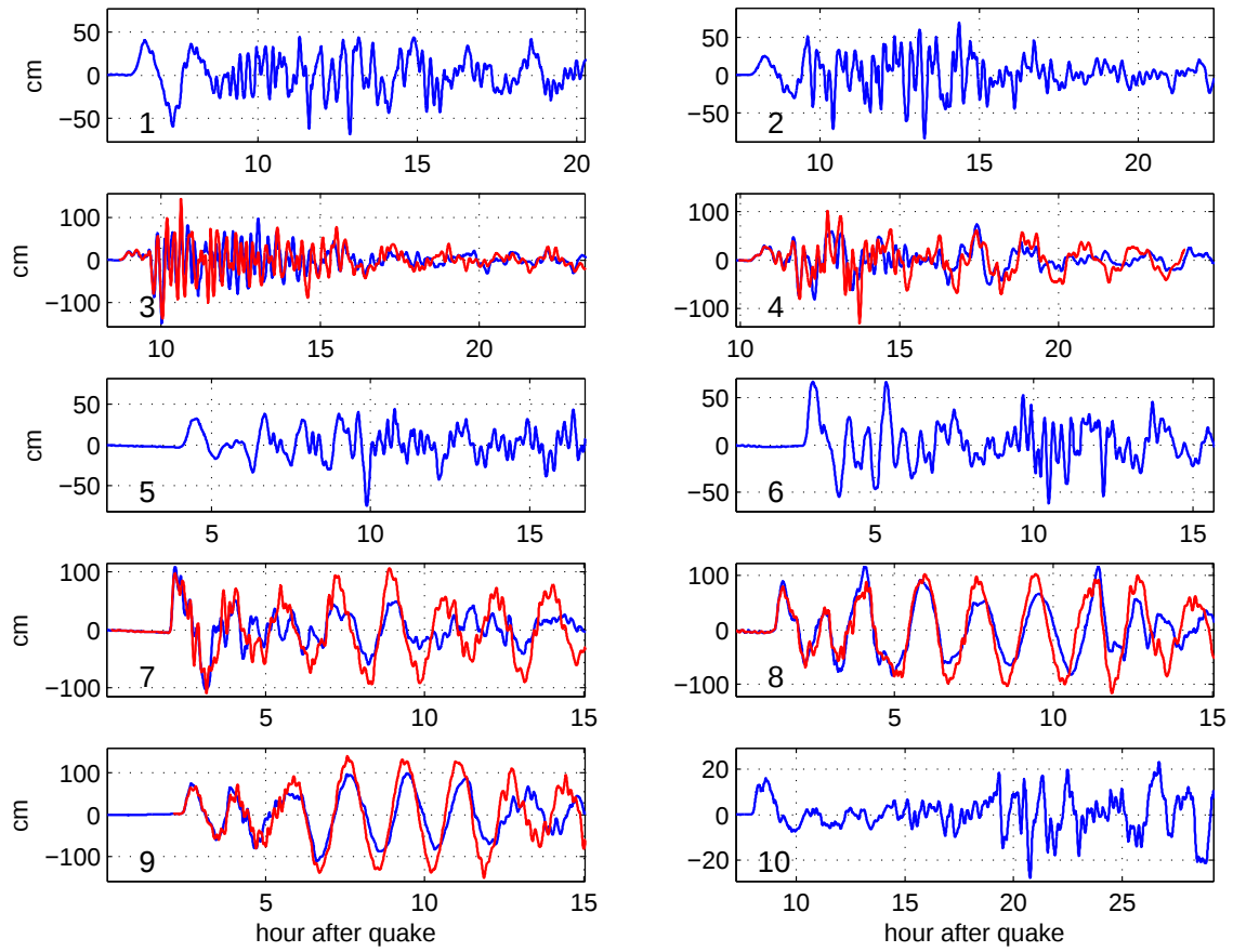
Figure 23: Time histories at the gage location, according to Forecast Model (blue) and Reference Model (red), in Mega events 1-10 (as numbered in the plots).
