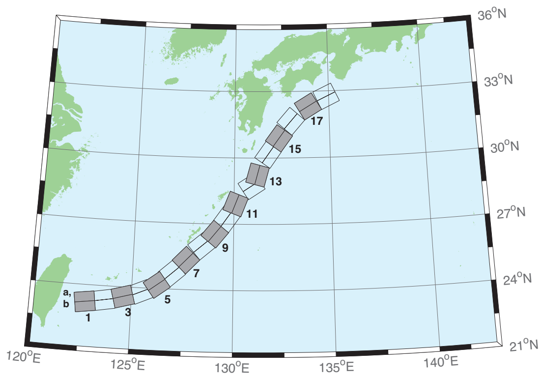
Figure 43: Ryukyu-Kyushu-Nankai Zone unit sources.
