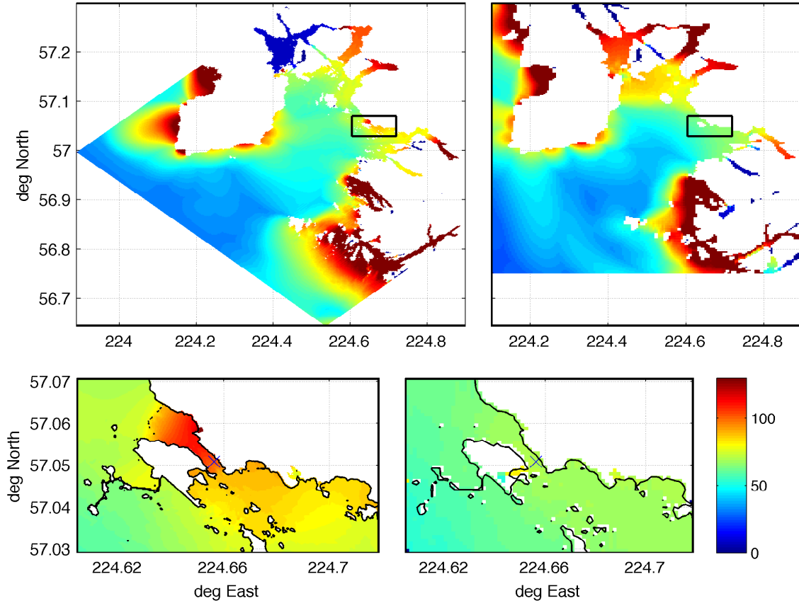
Figure 28: Maximum water elevation with respect to still sea level in Mega 4 event: top left - B grid, reference model, with contour of C-grid shown in black; top right - B grid, forecast model, with C-grid contour shown in black; bottom panes: left - C grid, reference model; right - C grid, forecast model. Cross - gage location. Shown contour of the original shoreline position. Colorscale: cm.
