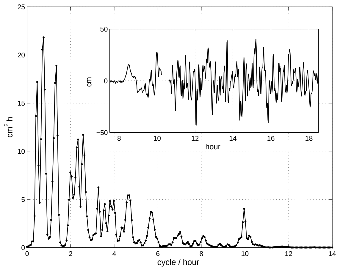
Figure 10: Power spectrum of the signal of the Mar. 11, 2011 tsunami at Sitka. Inner plot: first 11 h (or as much as available) of the tsunami signal at the gage, time after the quake.
