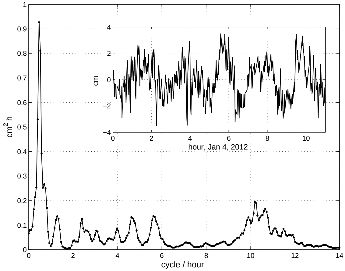
Figure 4: Power spectrum of the gage background signal computed for a twelve day record in January 2-13, 2012. Inner plot: sample background signal (residual of tidal removal) at the gage.
