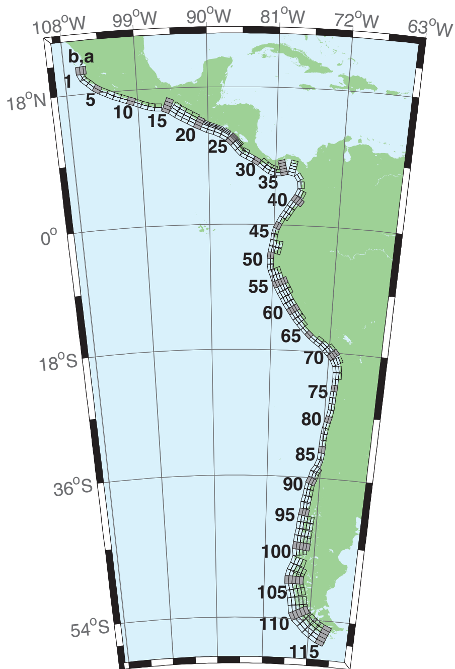
Figure 36: Central and South America Subduction Zone unit sources.
