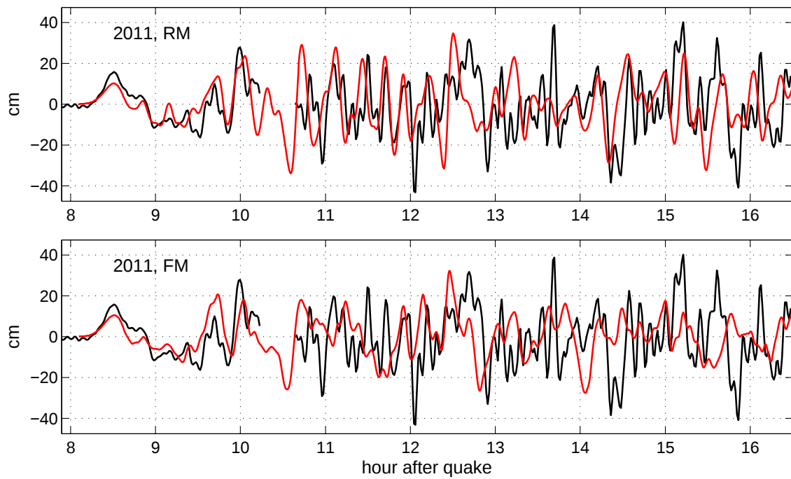
Figure 21: Simulated time history (red) of the March 11, 2011 tsunami at Sitka tide gage vs. de-tided gage record (black); top pane - simulation with the Reference Model, bottom pane - with the Forecast Model. Model is delayed 7 min.
