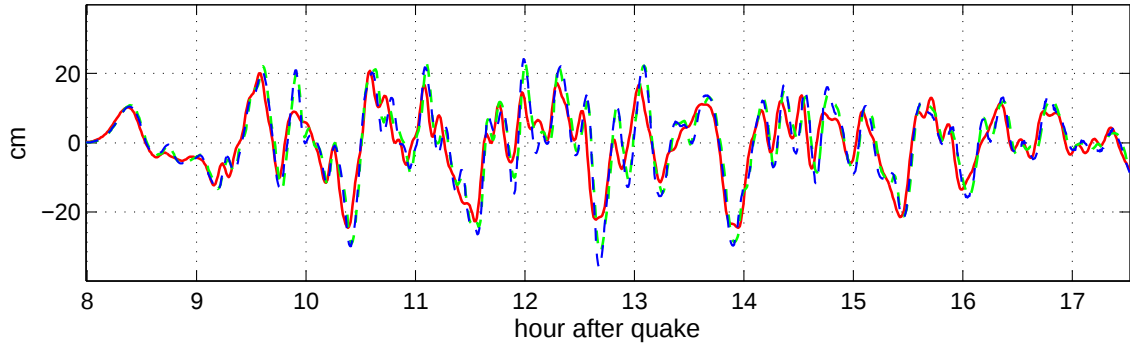
Figure 16: Time histories at the gage computed directly with the optimized B grid (red), and further refined with the use of either optimized C grid at 3 arc-sec resolution (green dashed) or reference C grid with 2/3 arc-sec resolution (blue dashed). Simulation of the 2011 East Japan tsunami.
