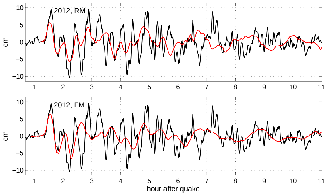
Figure 22: Simulated time history (red) of the October 28, 2012 tsunami at Sitka tide gage vs. de-tided gage record (black); top pane - simulation with the Reference Model, bottom pane - with the Forecast Model. Model is advanced 6 min.
