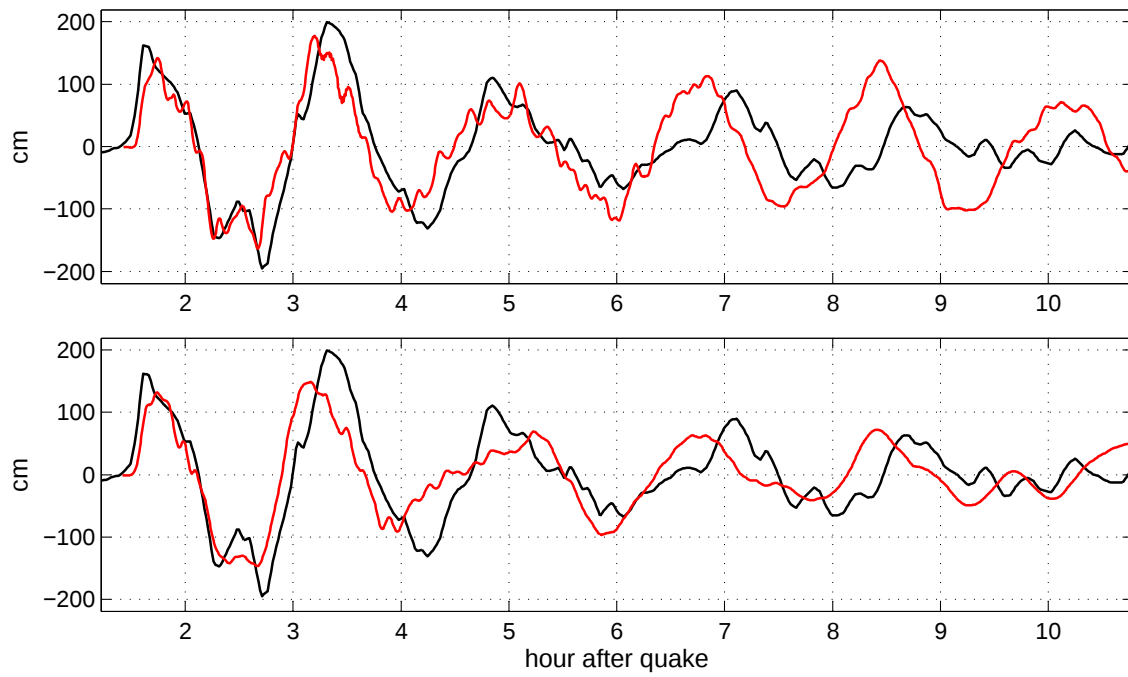
Figure 19: Simulated time history (red) of the March 28, 1964 tsunami at Sitka tide gage vs. detided gage record (black); top pane - simulation with the Reference Model, bottom pane - with the Forecast Model.
