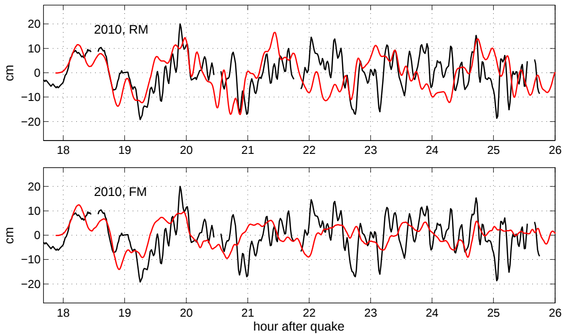
Figure 20: Simulated time history (red) of the February 27, 2010 tsunami at Sitka tide gage vs. de-tided gage record (black); top pane - simulation with the Reference Model, bottom pane - with the Forecast Model. Model is delayed 12 min.
