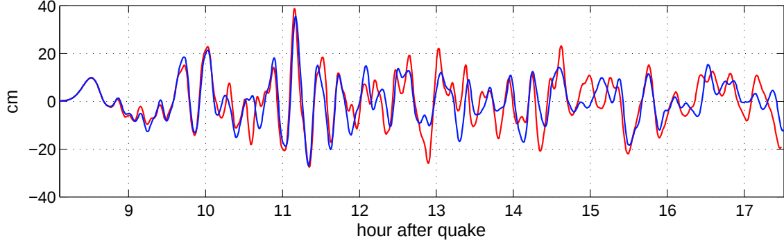
Figure 15: Simulated time history of the March 11, 2011 tsunami at Sitka tide gage. Simulation was performed with the same (reference) set of B and C grids enclosed in either reference (red) or optimized (blue) A grid.
