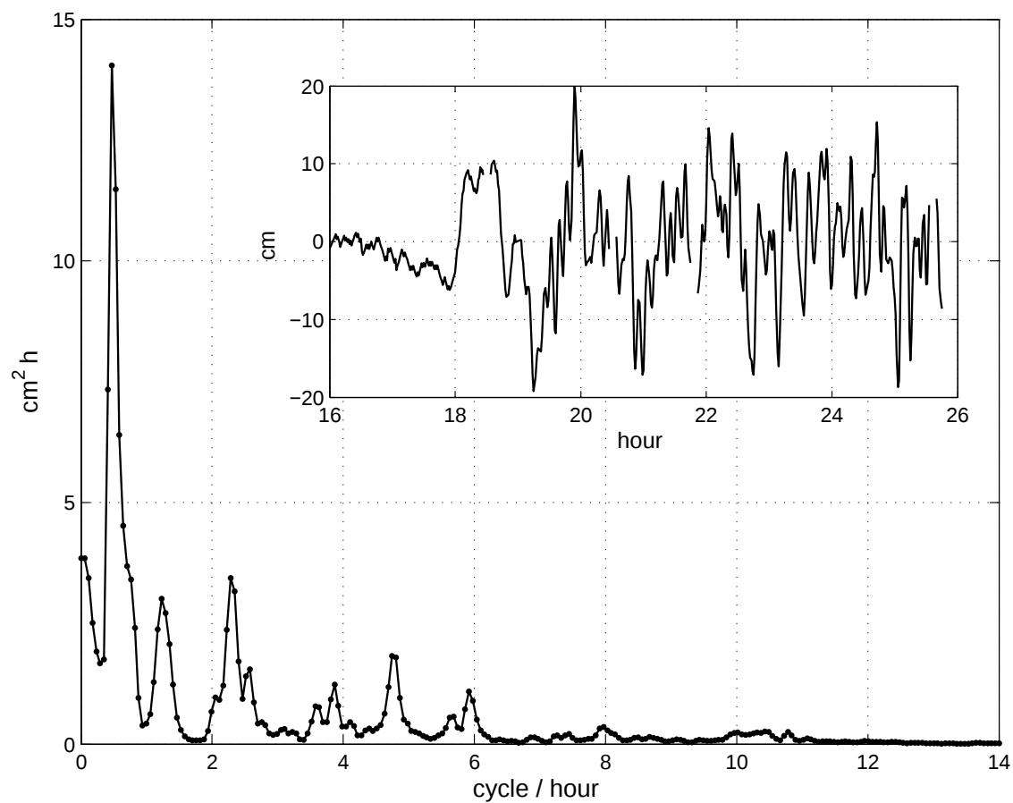
Figure 9: Power spectrum of the signal of the Feb. 27, 2010 tsunami at Sitka. Inner plot: first 11 h (or as much as available) of the tsunami signal at the gage, time after the quake.
