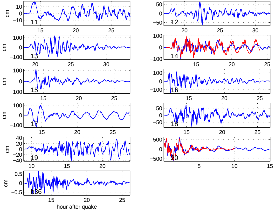
Figure 24: Time histories at the gage location, according to Forecast Model (blue) and Reference Model (red), in Mega events 11-20 (as numbered in the plots) and in Mw 7.5 event.
