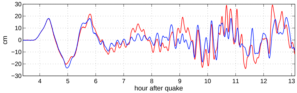
Figure 14: Simulated time history of the March 9, 1957 tsunami at Sitka tide gage. Simulation was performed with the same (reference) set of B and C grids enclosed in either reference (red) or optimized (blue) A grid.
