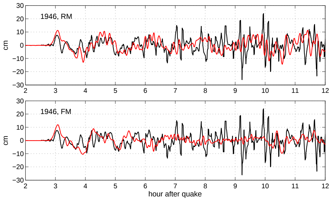
Figure 18: Simulated time history (red) of the April 1, 1946 tsunami at Sitka tide gage vs. de-tided gage record (black); top pane - simulation with the Reference Model, bottom pane - with the Forecast Model.
