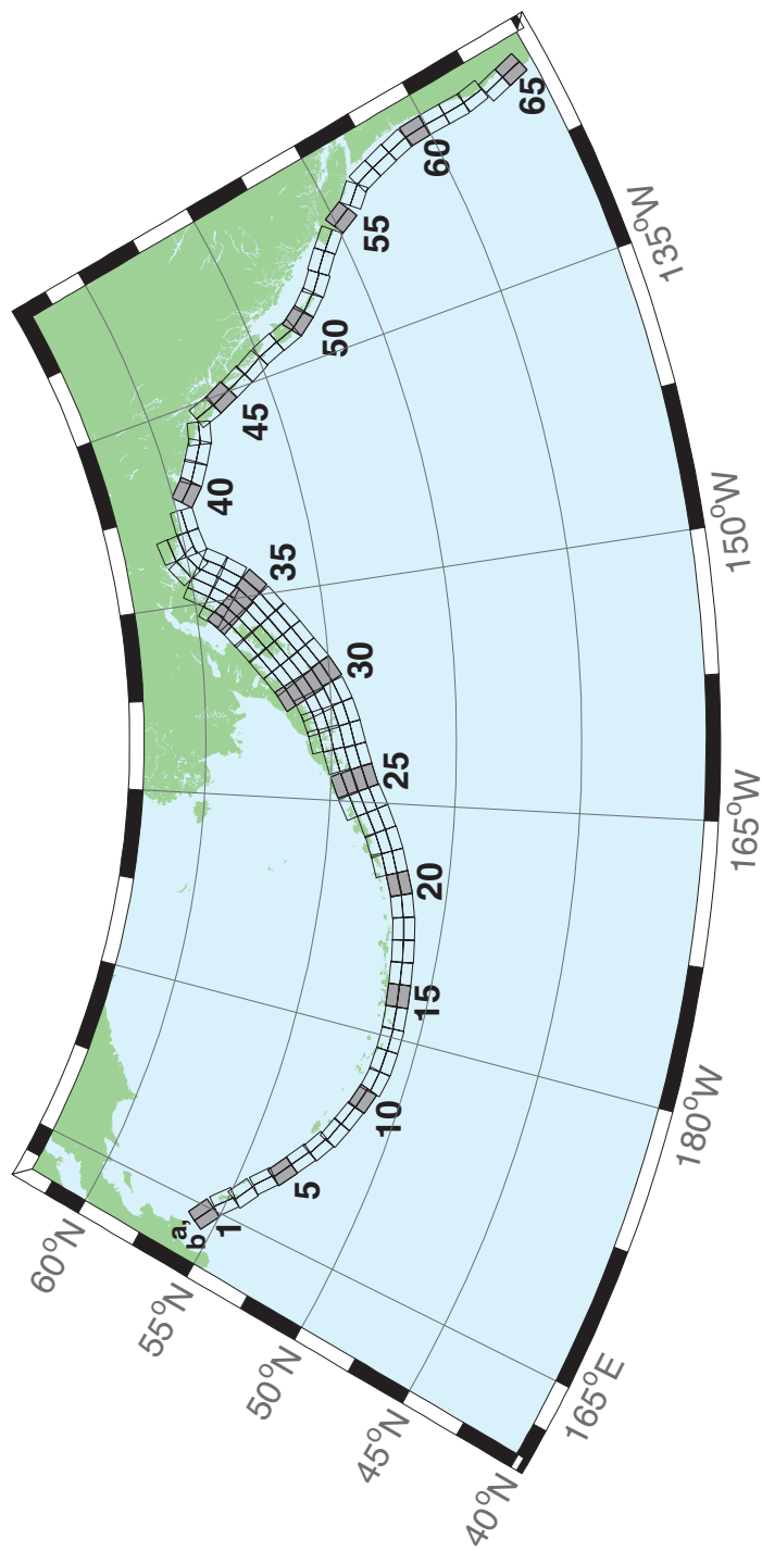
Figure 35: Aleutian–Alaska–Cascadia Subduction Zone unit sources.
