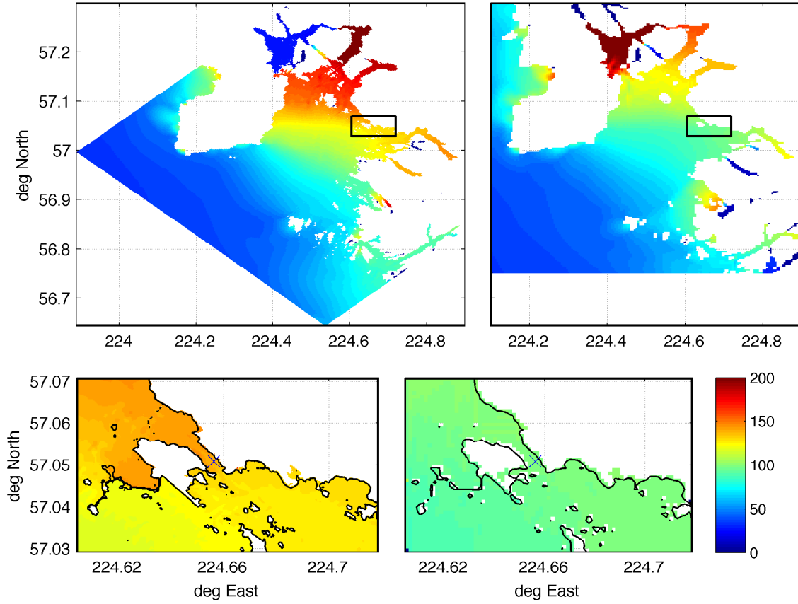
Figure 31: Maximum water elevation with respect to still sea level in Mega 9 event: top left - B grid, reference model, with contour of C-grid shown in black; top right - B grid, forecast model, with C-grid contour shown in black; bottom panes: left - C grid, reference model; right - C grid, forecast model. Cross - gage location. Shown contour of the original shoreline position. Colorscale: cm.
