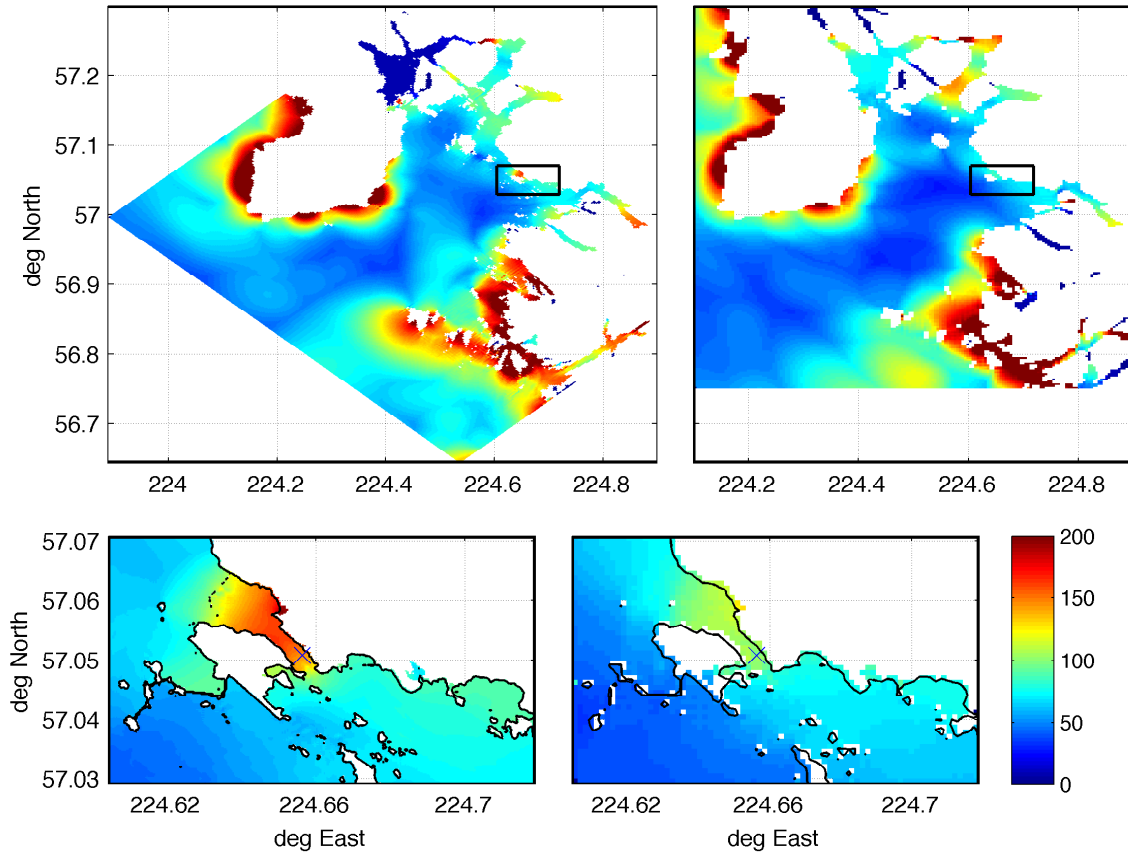
Figure 27: Maximum water elevation with respect to still sea level in Mega 3 event: top left - B grid, reference model, with contour of C-grid shown in black; top right - B grid, forecast model, with C-grid contour shown in black; bottom panes: left - C grid, reference model; right - C grid, forecast model. Cross - gage location. Shown contour of the original shoreline position. Colorscale: cm.
