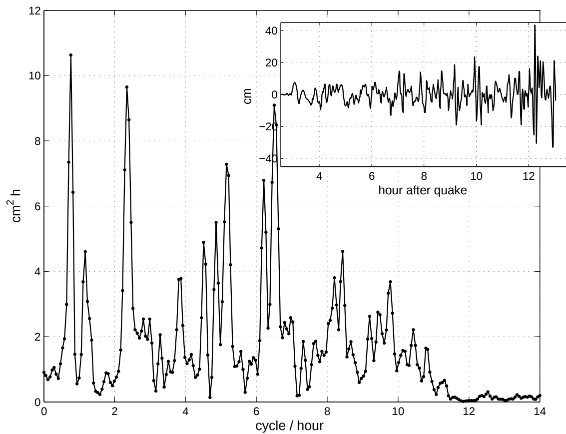
Figure 5: Power spectrum of the signal of the Apr. 1, 1946 tsunami at Sitka. Inner plot: first 11 h (or as much as available) of the tsunami signal at the gage, time after the quake.
