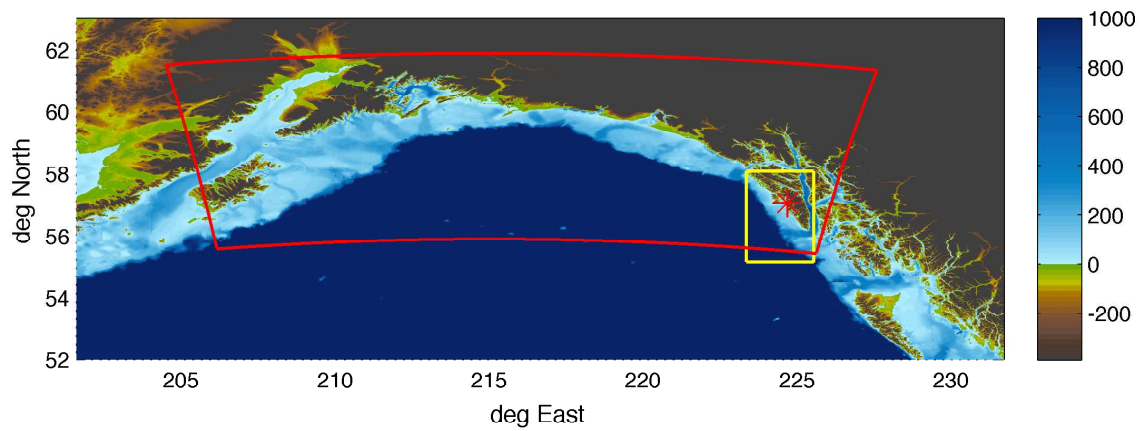
Figure 11: Coverage of the reference 20-s A grid (red contour), and 30-s optimized A grid (yellow contour). Red star marks the forecast area (Sitka sound).
