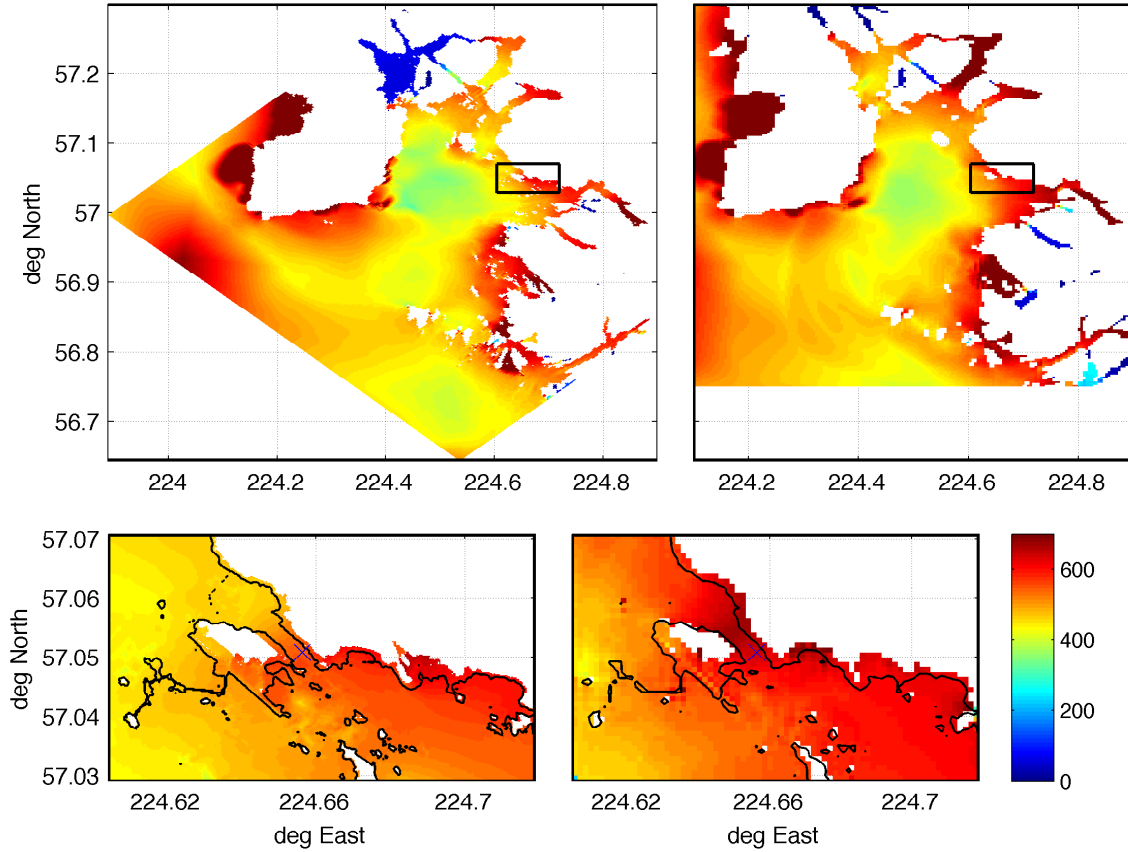
Figure 33: Maximum water elevation with respect to still sea level in Mega 20 (local) event: top left - B grid, reference model, with contour of C-grid shown in black; top right - B grid, forecast model, with C-grid contour shown in black; bottom panes: left - C grid, reference model; right - C grid, forecast model. Cross - gage location. Shown contour of the original shoreline position. Colorscale: cm.
