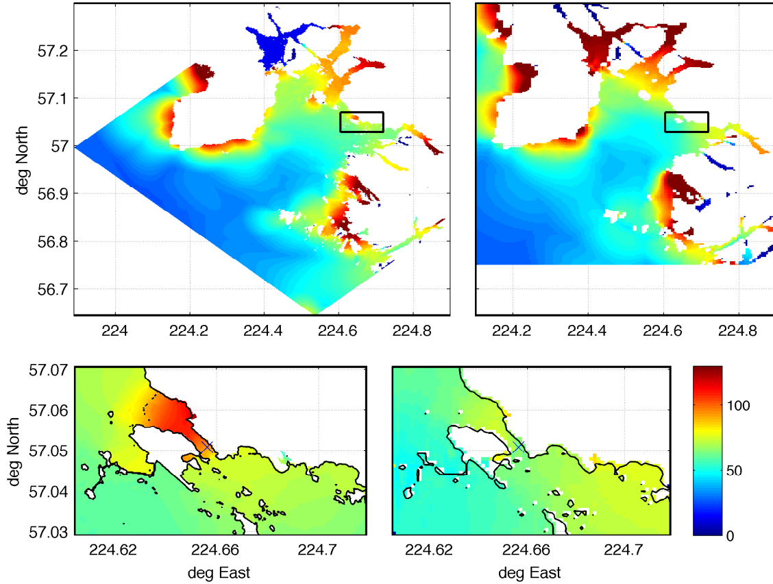
Figure 32: Maximum water elevation with respect to still sea level in Mega 14 event: top left - B grid, reference model, with contour of C-grid shown in black; top right - B grid, forecast model, with C-grid contour shown in black; bottom panes: left - C grid, reference model; right - C grid, forecast model. Cross - gage location. Shown contour of the original shoreline position. Colorscale: cm.
