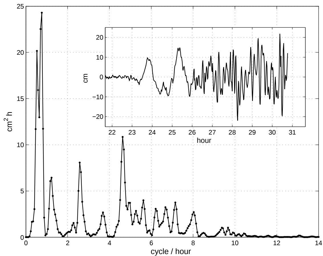
Figure 6: Power spectrum of the signal of the Nov. 4, 1952 tsunami at Sitka. Inner plot: first 11 h (or as much as available) of the tsunami signal at the gage, time from 00:00 on Nov. 4, 1952.
