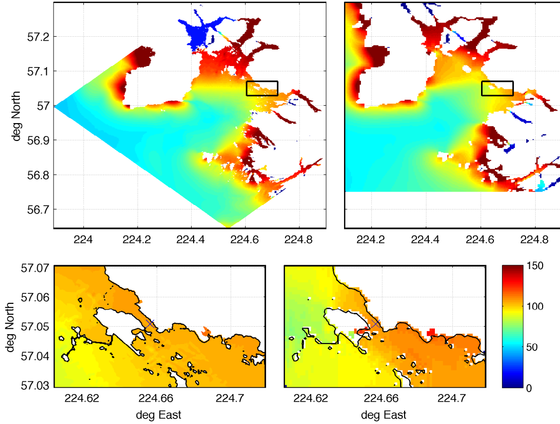
Figure 29: Maximum water elevation with respect to still sea level in Mega 7 event: top left - B grid, reference model, with contour of C-grid shown in black; top right - B grid, forecast model, with C-grid contour shown in black; bottom panes: left - C grid, reference model; right - C grid, forecast model. Cross - gage location. Shown contour of the original shoreline position. Colorscale: cm.
