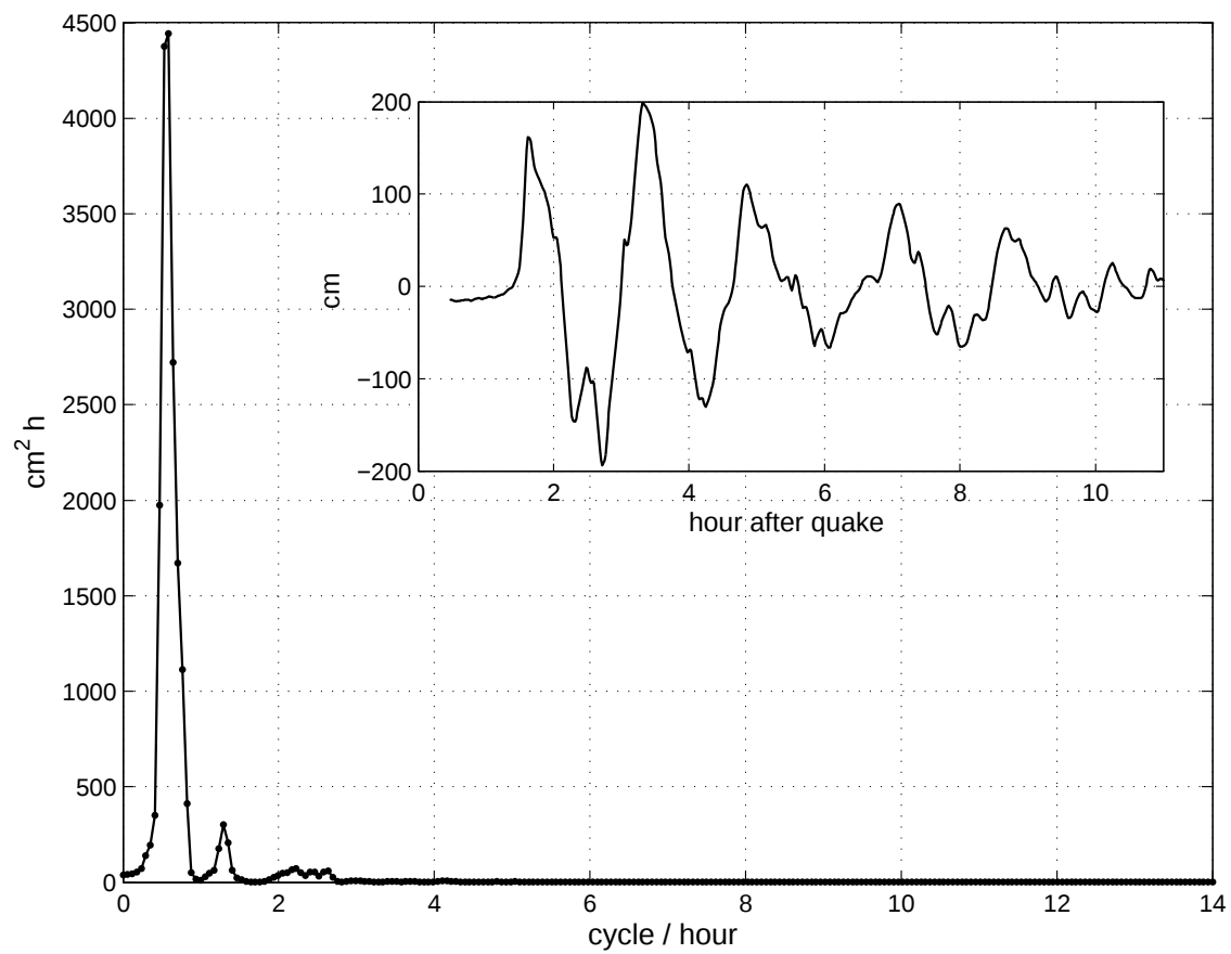
Figure 8: Power spectrum of the signal of the Mar. 28, 1964 tsunami at Sitka. Inner plot: first 11 h (or as much as available) of the tsunami signal at the gage, time after the quake.
