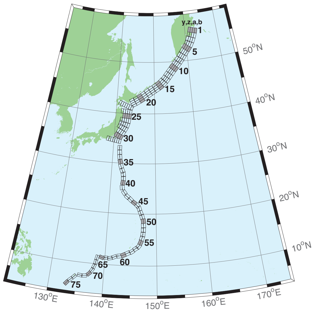
Figure 38: Kamchatka-Kuril-Japan-Izu-Mariana-Yap Subduction Zone unit sources.
