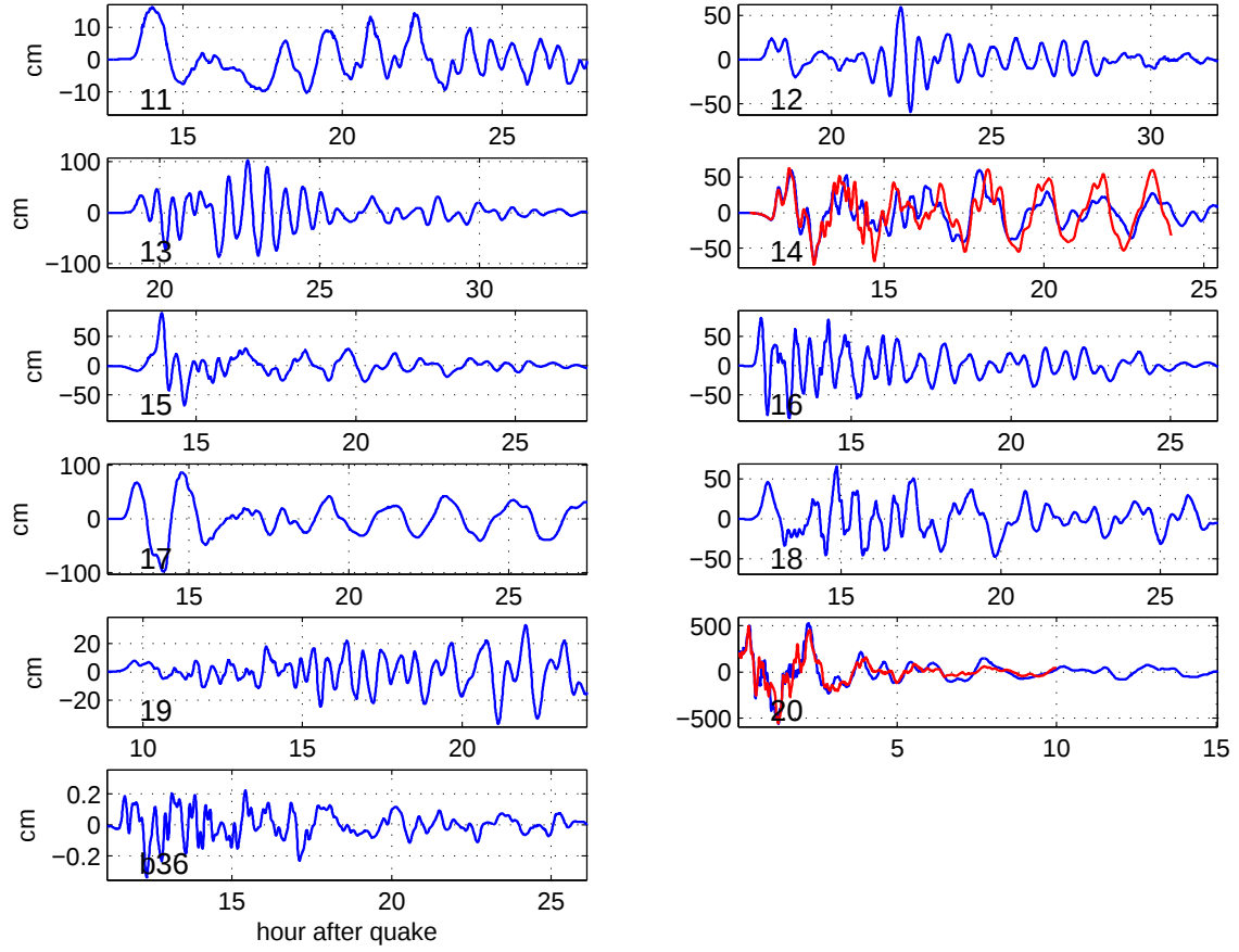
Figure 26: Time histories at the virtual gage on Japonski island, according to Forecast Model (blue) and Reference Model (red), in Mega events 11-20 (as numbered in the plots) and in Mw 7.5 event.
