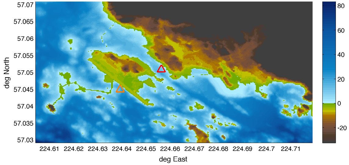
Figure 13: Reference C grid. Red triangle points tide gauge location, orange triangle - virtual gauge. Colorscale - meters.
