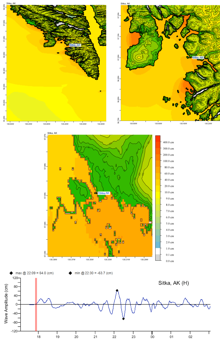
Figure 46: Response of the Sitka forecast model to synthetic scenario CSSZ 89-98 (alpha=25). Maximum sea surface elevation for A-grid (top left), B-grid (top right), C-grid (center). Sea surface elevation time series at the C-grid warning point (bottom), to be compared with timeseries 12 in Figure 24.
