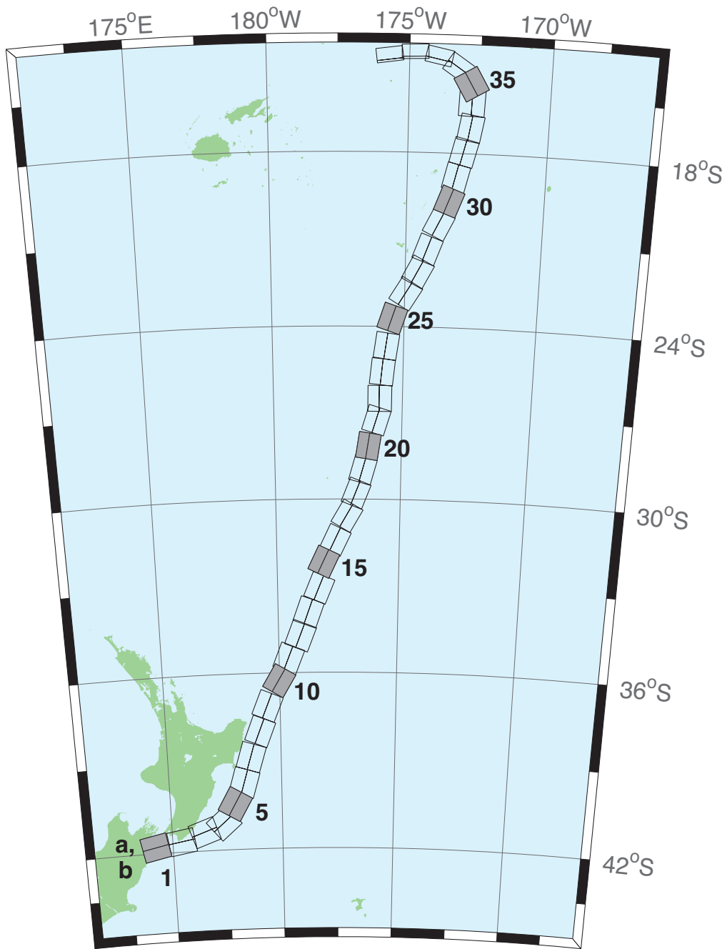
Figure 41: New Zealand–Keradec–Tonga Subduction Zone unit sources.
