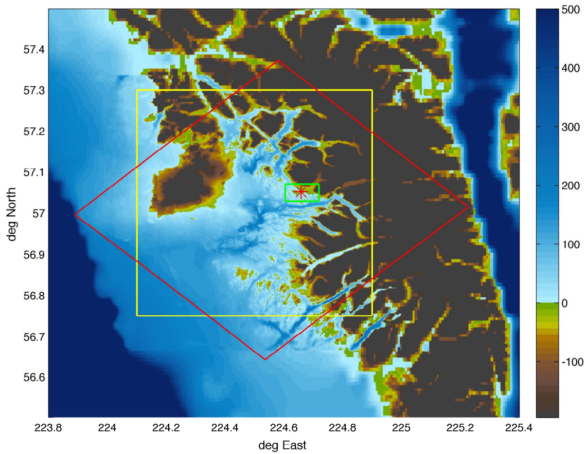
Figure 12: Contours of reference B grid (red), optimized B grid (yellow) and C grid (green). Red star points tide gauge location. Colorscale - meters.
