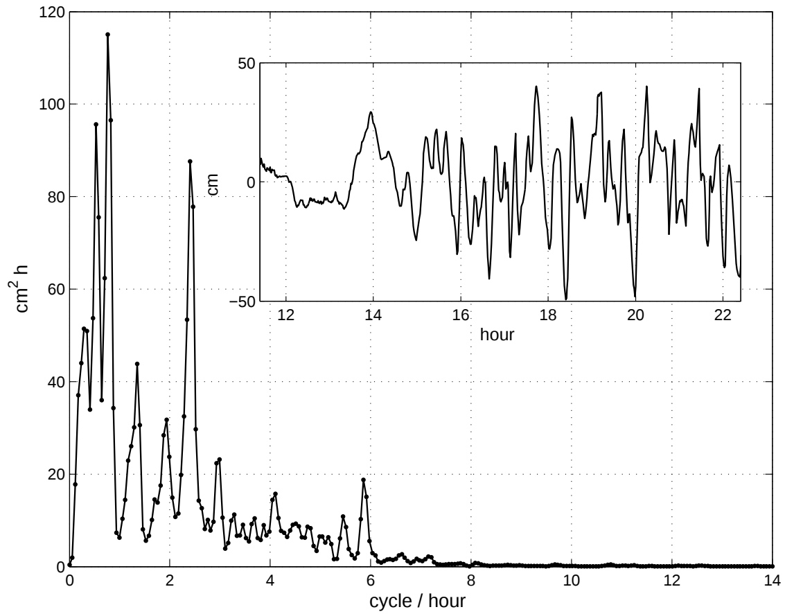
Figure 7: Power spectrum of the signal of the Mar. 22, 1960 tsunami at Sitka. Inner plot: first 11 h (or as much as available) of the tsunami signal at the gage, time from 00:00 on Mar. 23, 1960.
