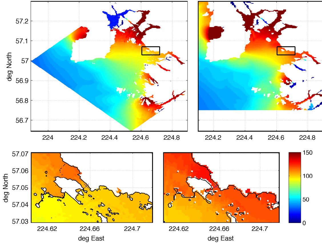
Figure 30: Maximum water elevation with respect to still sea level in Mega 8 event: top left - B grid, reference model, with contour of C-grid shown in black; top right - B grid, forecast model, with C-grid contour shown in black; bottom panes: left - C grid, reference model; right - C grid, forecast model. Cross - gage location. Shown contour of the original shoreline position. Colorscale: cm.
