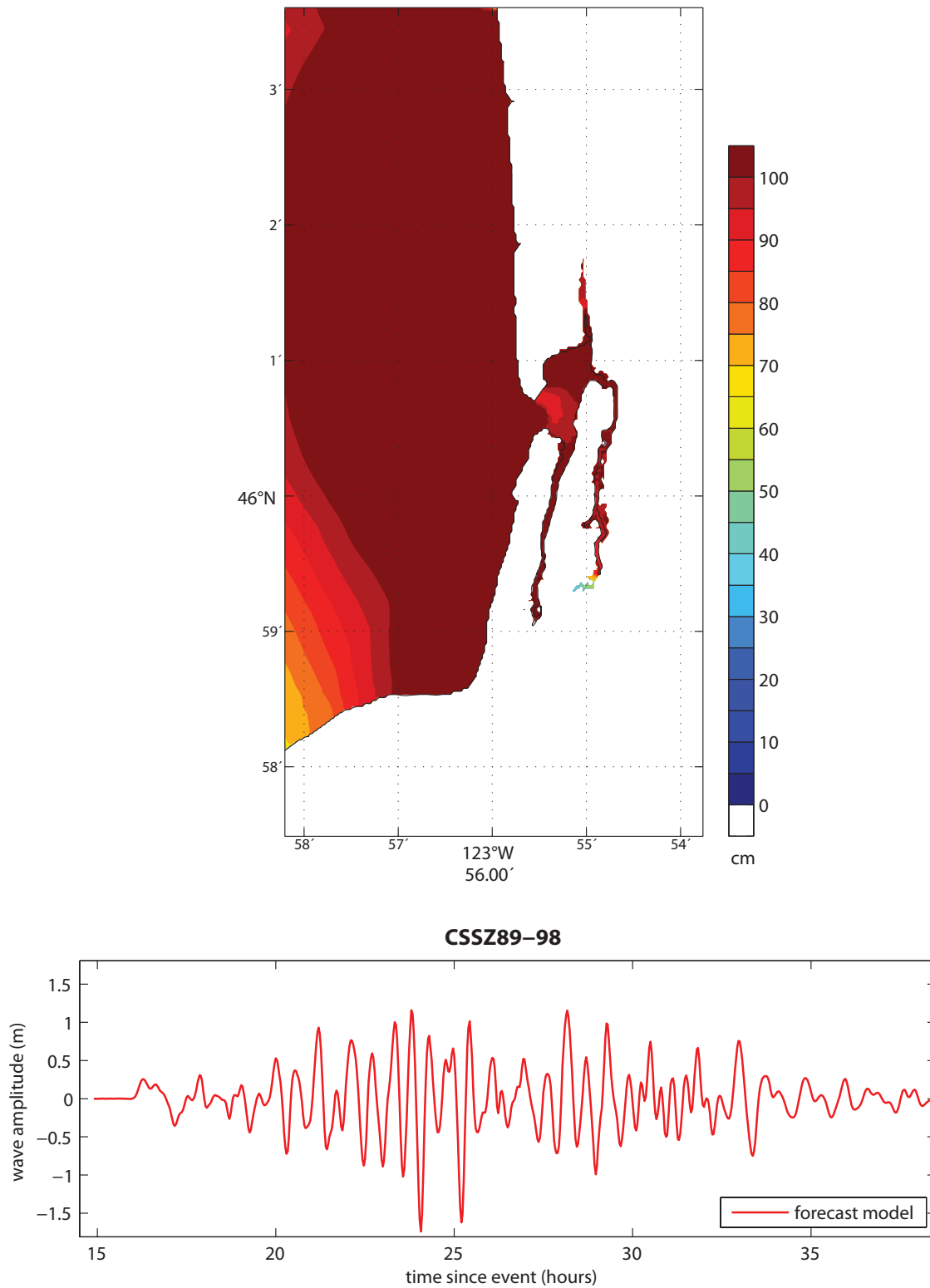
Figure 31: Results from the forecast model for the CSSZ 89–98 Mw 9.3 synthetic event. The upper panel shows the map of predicted maximum wave heights in the Seaside C-grid, and the lower panel shows the time series of wave amplitude at the warning point location.
