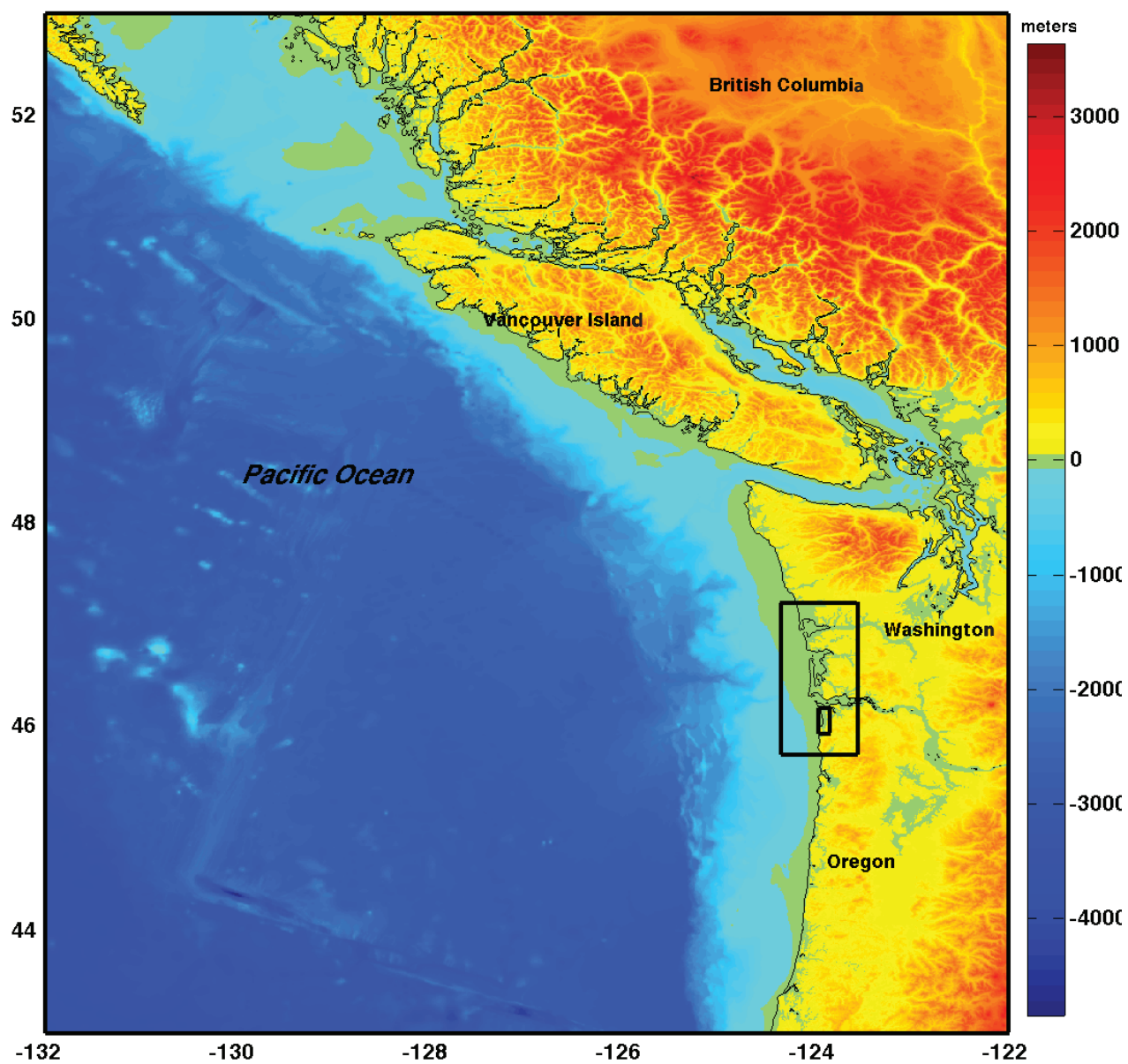
Figure 3: Merged digital elevation model based on best available bathymetric and topographic data used to develop both the Seaside high-resolution reference and the optimized tsunami forecast models (Venturato, 2005). The figure shows the set of three nested grids, the smallest and highest-resolution grid being the C-grid.
