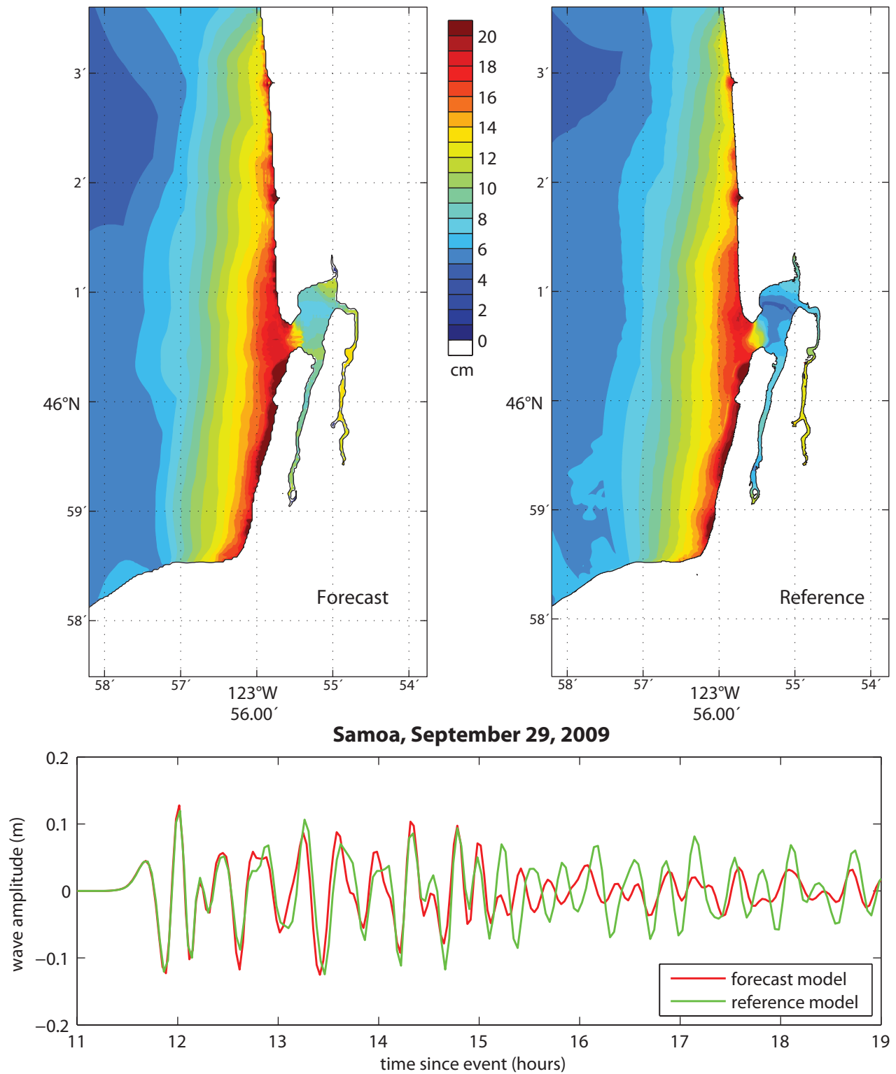
Figure 17: Model results for the 2009 Samoa tsunami. Uppermost panels show, respectively, the tsunami forecast model and the high-resolution reference model maximum wave height results. The lower panel shows a comparison between the model-computed time series and observed wave heights at the Seaside warning point.
