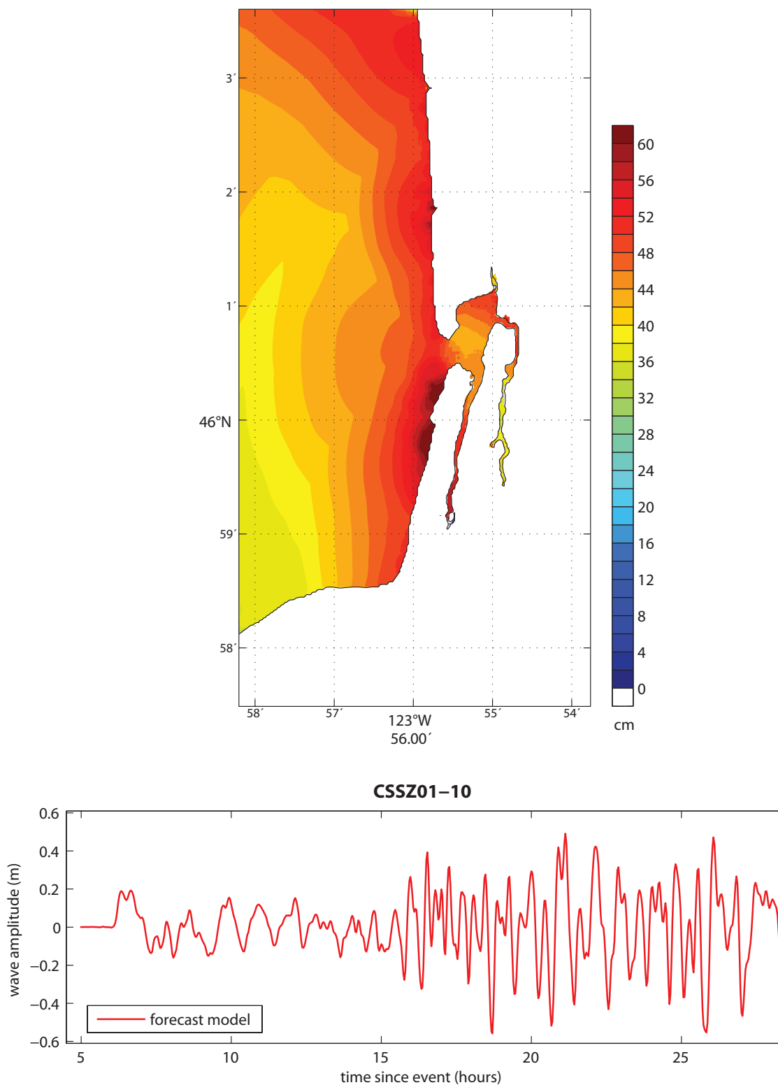
Figure 29: Results from the forecast model for the CSSZ 1–10 Mw 9.3 synthetic event. The upper panel shows the map of predicted maximum wave heights in the Seaside C-grid, and the lower panel shows the time series of wave amplitude at the warning point location.
