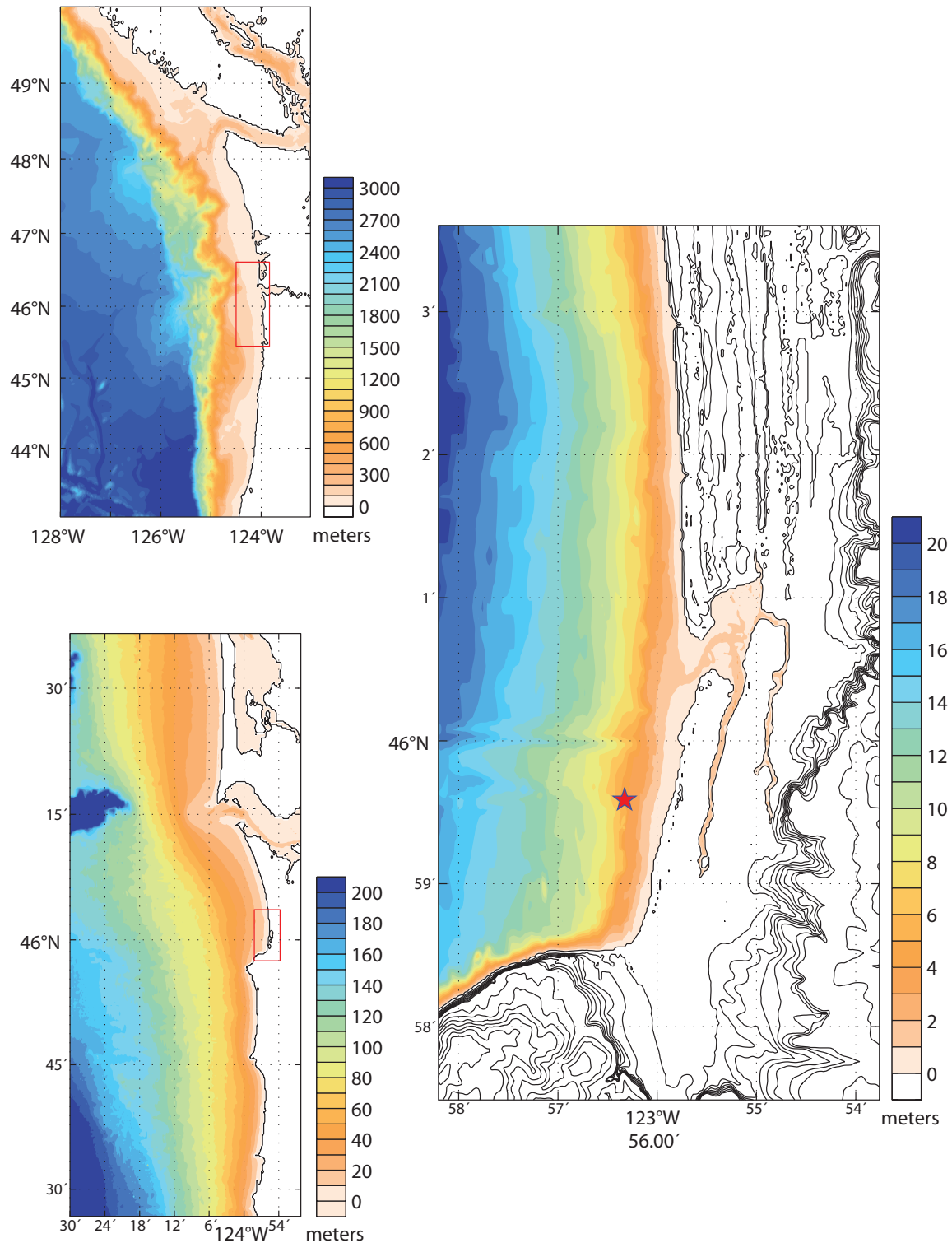
Figure 6: Bathymetry in meters used for the tsunami forecast model grids for Seaside, Oregon. The A-grid is shown in the top left panel, the B-grid in the lower left panel, and the C-grid is shown in the right panel. Topography of the C-grid is contoured with 40-m intervals. The red boxes in the A and B plots mark the extents of the B- and C-grids, respectively.
