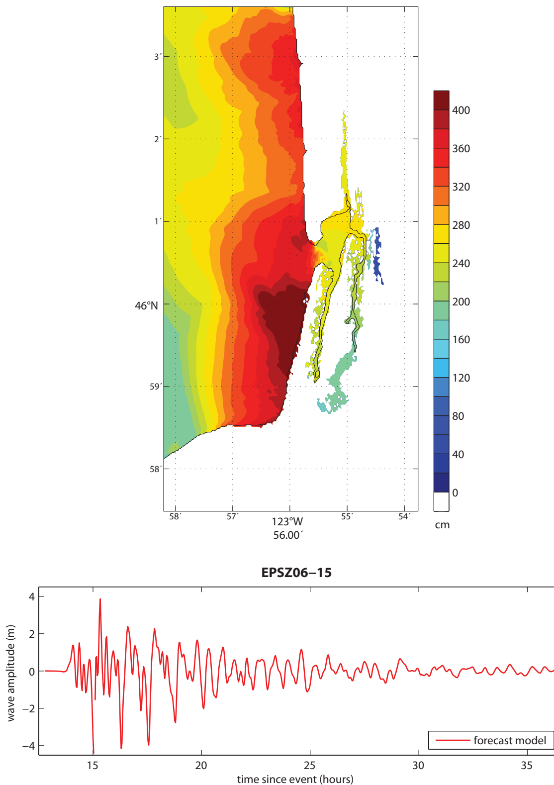
Figure 37: Results from the forecast model for the EPSZ 6–15 Mw 9.3 synthetic event. The upper panel shows the map of predicted maximum wave heights in the Seaside C-grid, and the lower panel shows the time series of wave amplitude at the warning point location.
