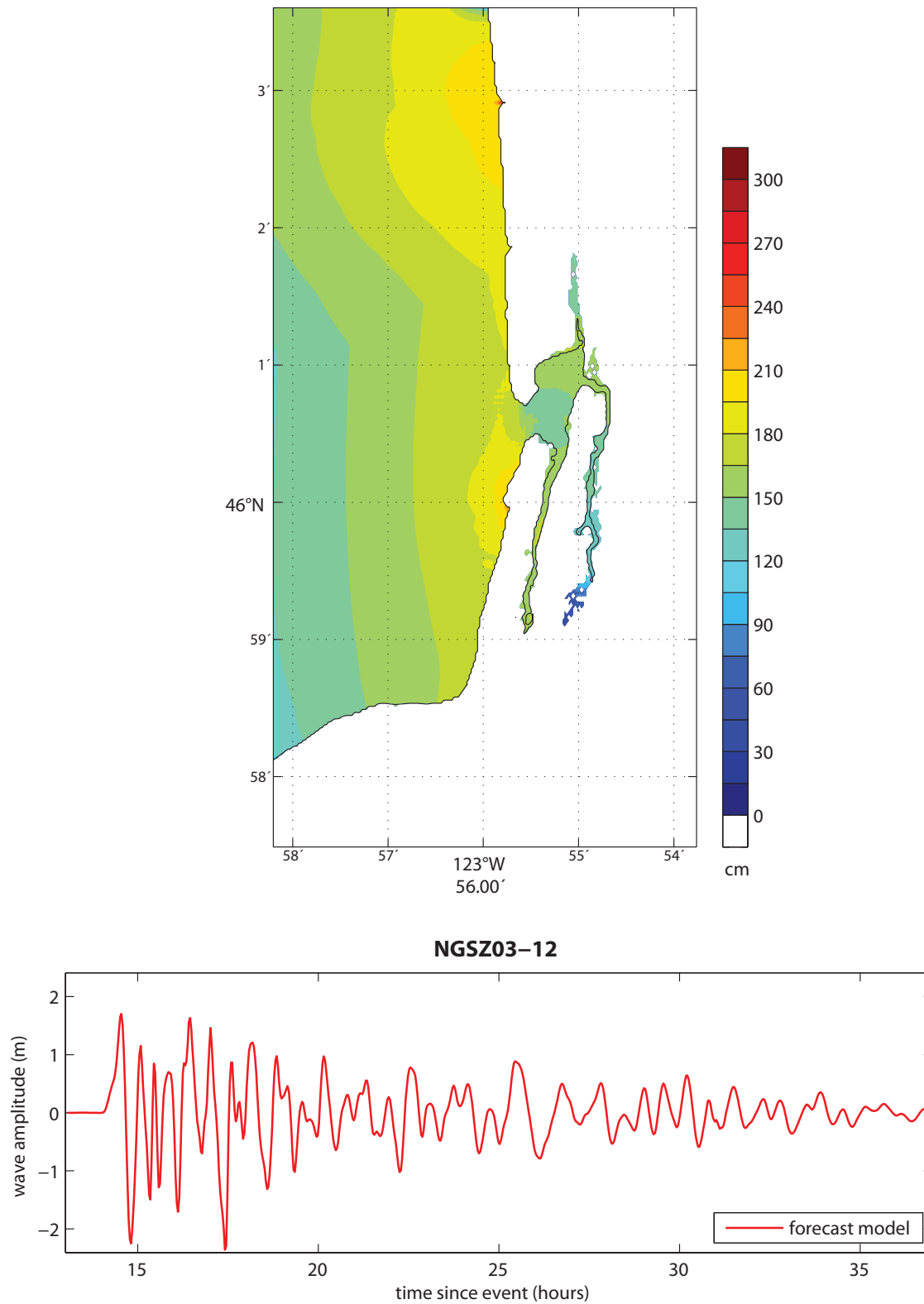
Figure 36: Results from the forecast model for the NGSZ 3–12 Mw 9.3 synthetic event. The upper panel shows the map of predicted maximum wave heights in the Seaside C-grid, and the lower panel shows the time series of wave amplitude at the warning point location.
