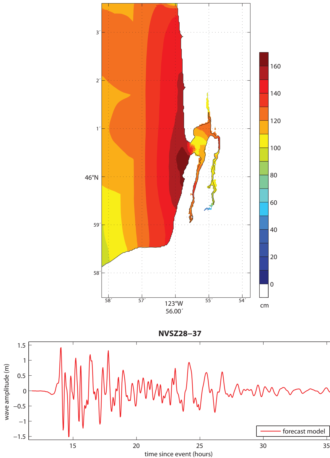
Figure 34: Results from the forecast model for the NVSZ 28–37 Mw 9.3 synthetic event. The upper panel shows the map of predicted maximum wave heights in the Seaside C-grid, and the lower panel shows the time series of wave amplitude at the warning point location.
