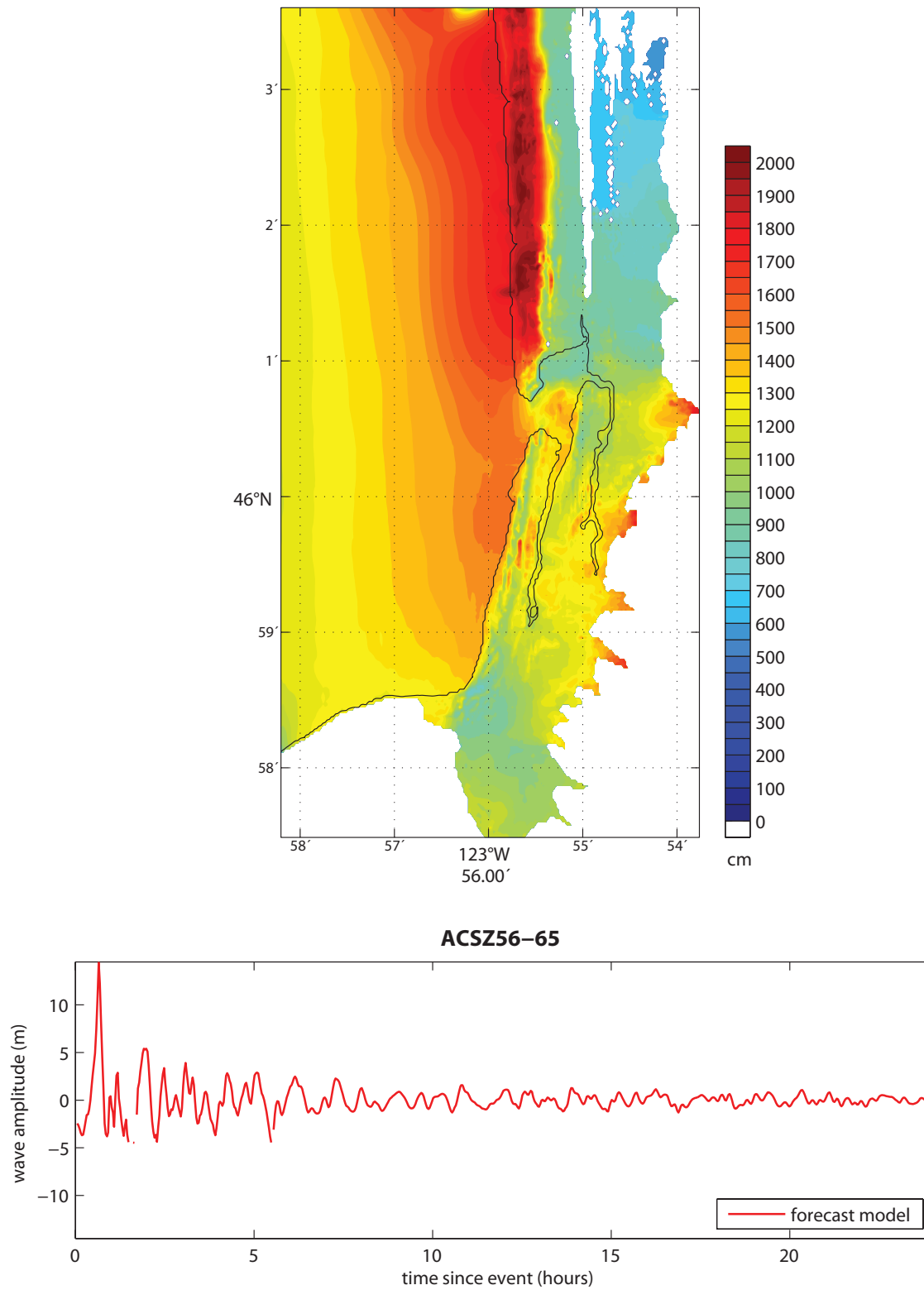
Figure 28: Results from the forecast model for the ACSZ 56–65 Mw 9.3 synthetic event. The upper panel shows the map of predicted maximum wave heights in the Seaside C-grid, and the lower panel shows the time series of wave amplitude at the warning point location.
