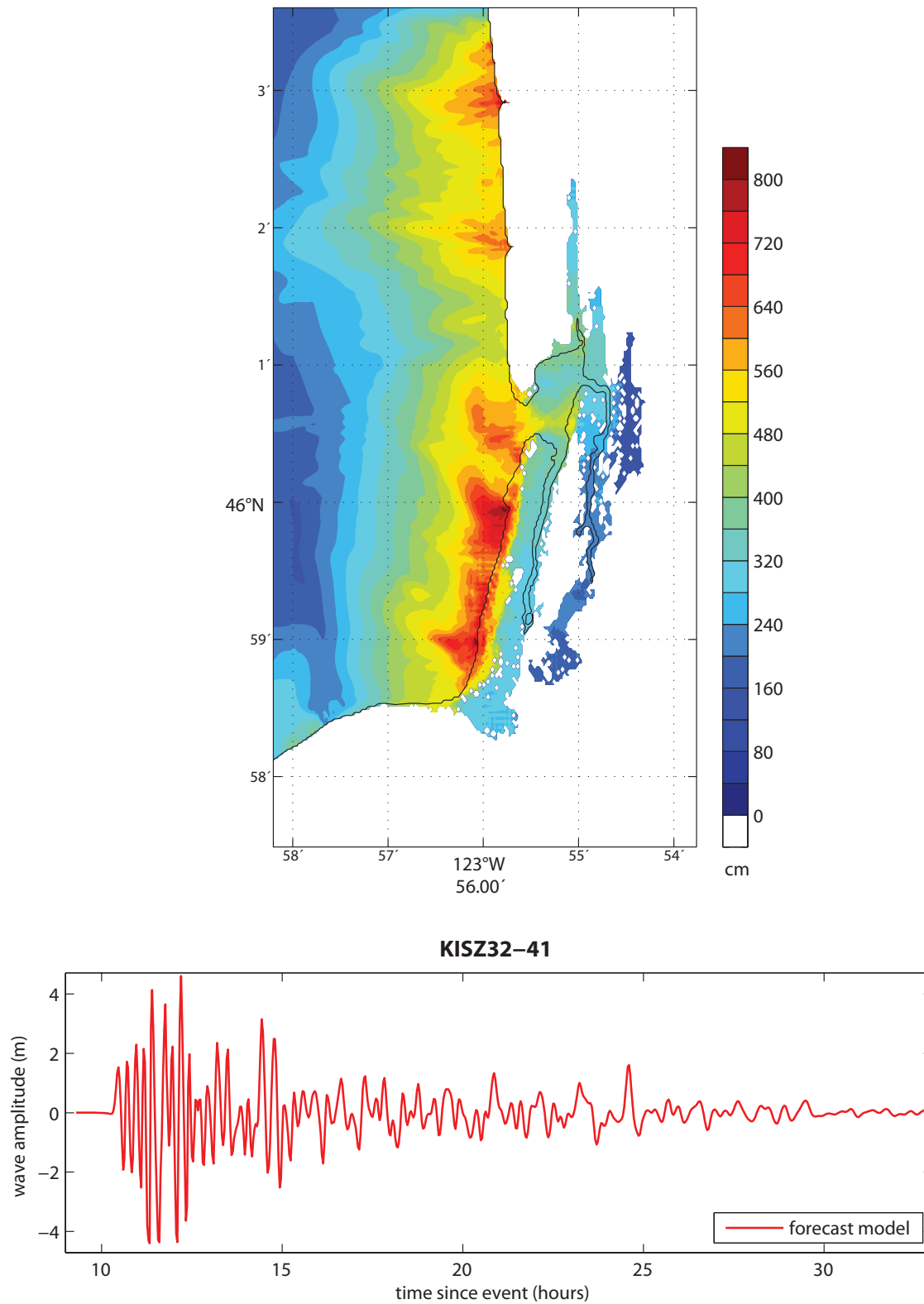
Figure 22: Results from the forecast model for the KISZ 32–41 Mw 9.3 synthetic event. The upper panel shows the map of predicted maximum wave heights in the Seaside C-grid, and the lower panel shows the time series of wave amplitude at the warning point location.
