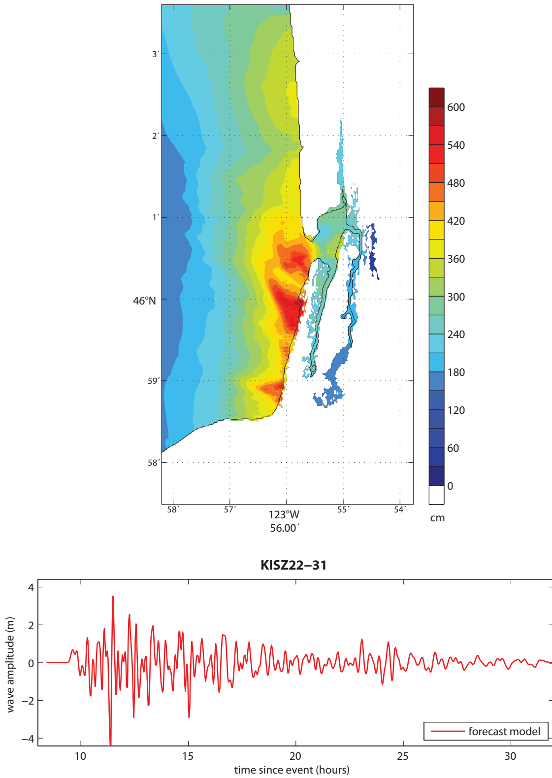
Figure 21: Results from the forecast model for the KISZ 22–31 Mw 9.3 synthetic event. The upper panel shows the map of predicted maximum wave heights in the Seaside C-grid, and the lower panel shows the time series of wave amplitude at the warning point location.
