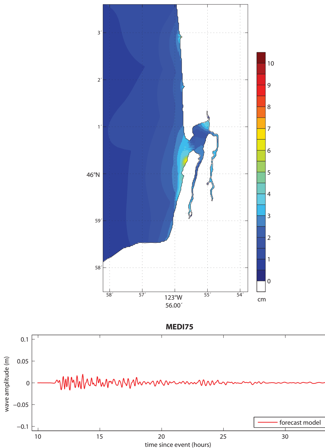
Figure 39: Results from the forecast model for the medium NTSZ B36 Mw 7.5 synthetic event. The upper panel shows the map of predicted maximum wave heights in the Seaside C-grid, and the lower panel shows the time series of wave amplitude at the warning point location.
