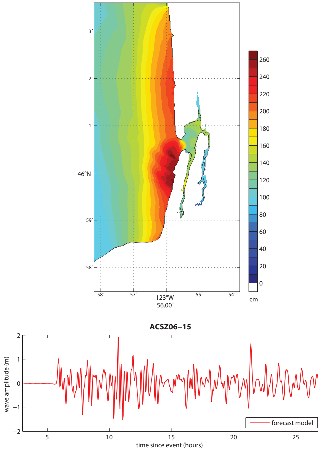
Figure 24: Results from the forecast model for the ACSZ 6–15 Mw 9.3 synthetic event. The upper panel shows the map of predicted maximum wave heights in the Seaside C-grid, and the lower panel shows the time series of wave amplitude at the warning point location.
