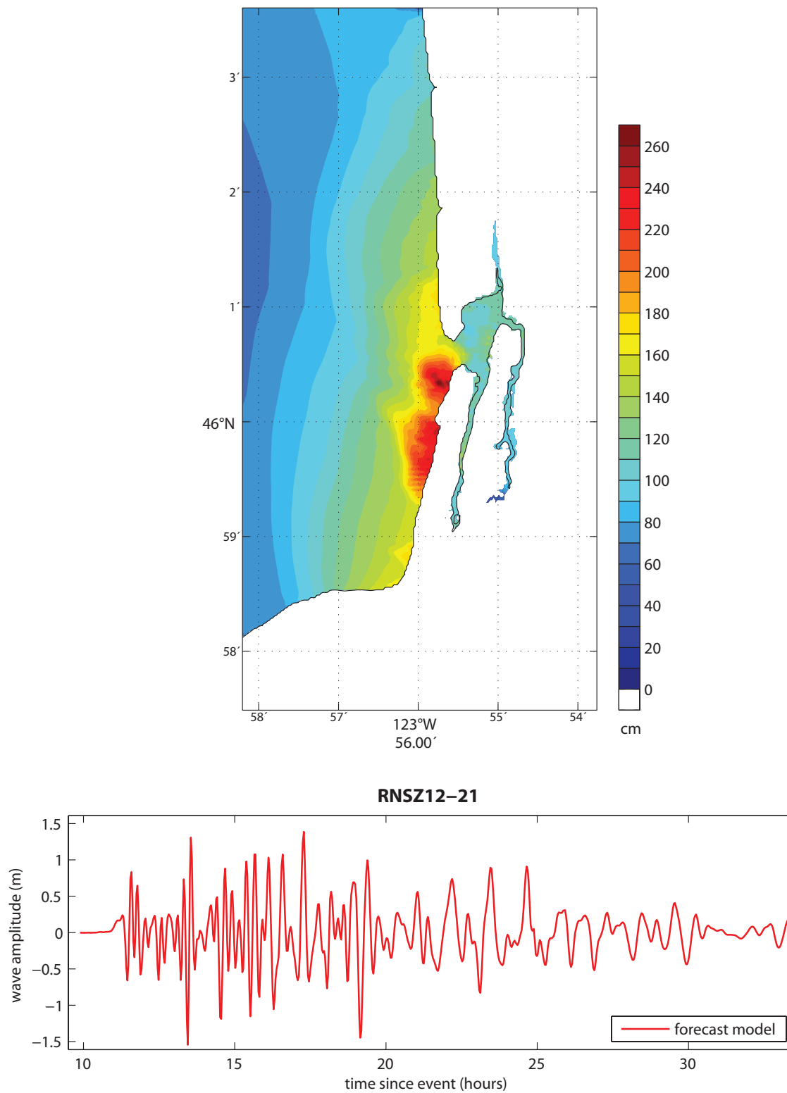
Figure 38: Results from the forecast model for the RNSZ 12–21 Mw 9.3 synthetic event. The upper panel shows the map of predicted maximum wave heights in the Seaside C-grid, and the lower panel shows the time series of wave amplitude at the warning point location.
