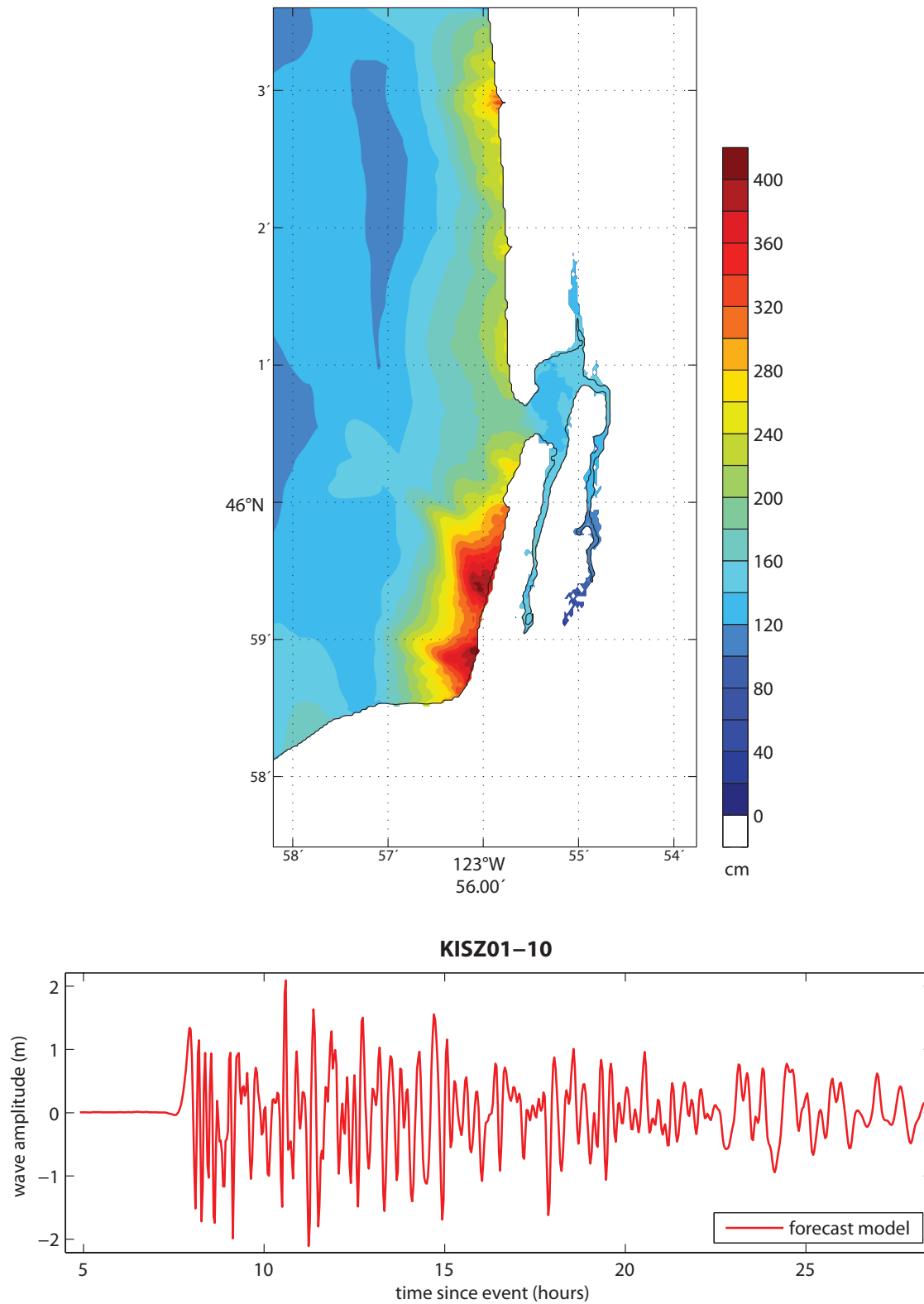
Figure 20: Results from the forecast model for the KISZ 01–10 Mw 9.3 synthetic event. The upper panel shows the map of predicted maximum wave heights in the Seaside C-grid, and the lower panel shows the time series of wave amplitude at the warning point location.
