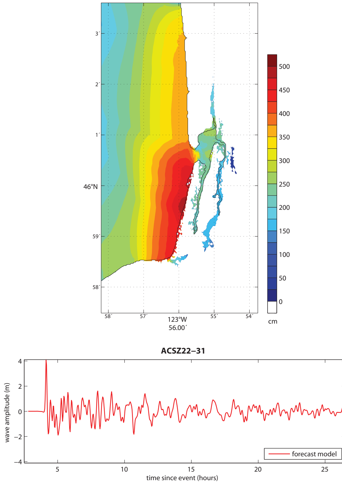
Figure 26: Results from the forecast model for the ACSZ 22–31 Mw 9.3 synthetic event. The upper panel shows the map of predicted maximum wave heights in the Seaside C-grid, and the lower panel shows the time series of wave amplitude at the warning point location.
