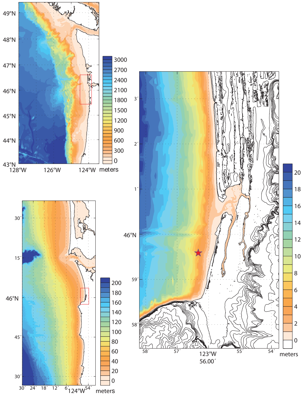
Figure 5: Bathymetry in meters for the high-resolution reference model grids for Seaside, Oregon. The A-grid is shown in the top left panel, the B-grid in the lower left panel, and the C-grid is shown in the right panel. Topography of the C-grid is contoured with 40-m intervals. The red boxes in the A and B plots mark the extents of the B- and C-grids, respectively.
