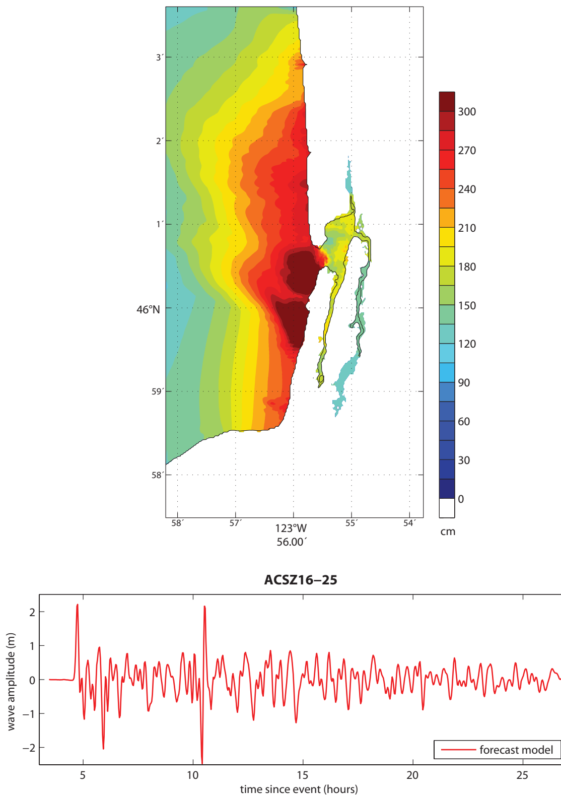
Figure 25: Results from the forecast model for the ACSZ 16–25 Mw 9.3 synthetic event. The upper panel shows the map of predicted maximum wave heights in the Seaside C-grid, and the lower panel shows the time series of wave amplitude at the warning point location.
