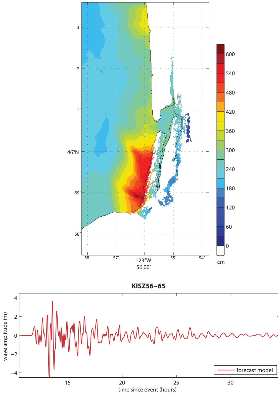
Figure 23: Results from the forecast model for the KISZ 56–65 Mw 9.3 synthetic event. The upper panel shows the map of predicted maximum wave heights in the Seaside C-grid, and the lower panel shows the time series of wave amplitude at the warning point location.
