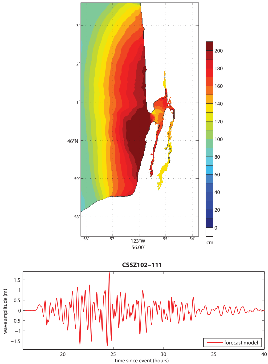
Figure 32: Results from the forecast model for the CSSZ 102–111 Mw 9.3 synthetic event. The upper panel shows the map of predicted maximum wave heights in the Seaside C-grid, and the lower panel shows the time series of wave amplitude at the warning point location.
