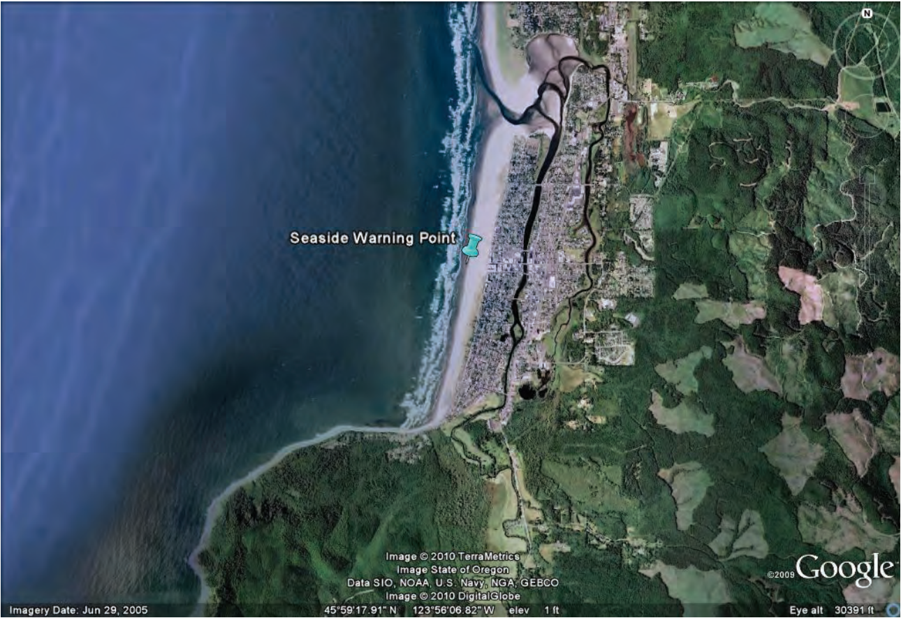
Figure 4: Map showing location of Seaside warning point (courtesy of Google).
