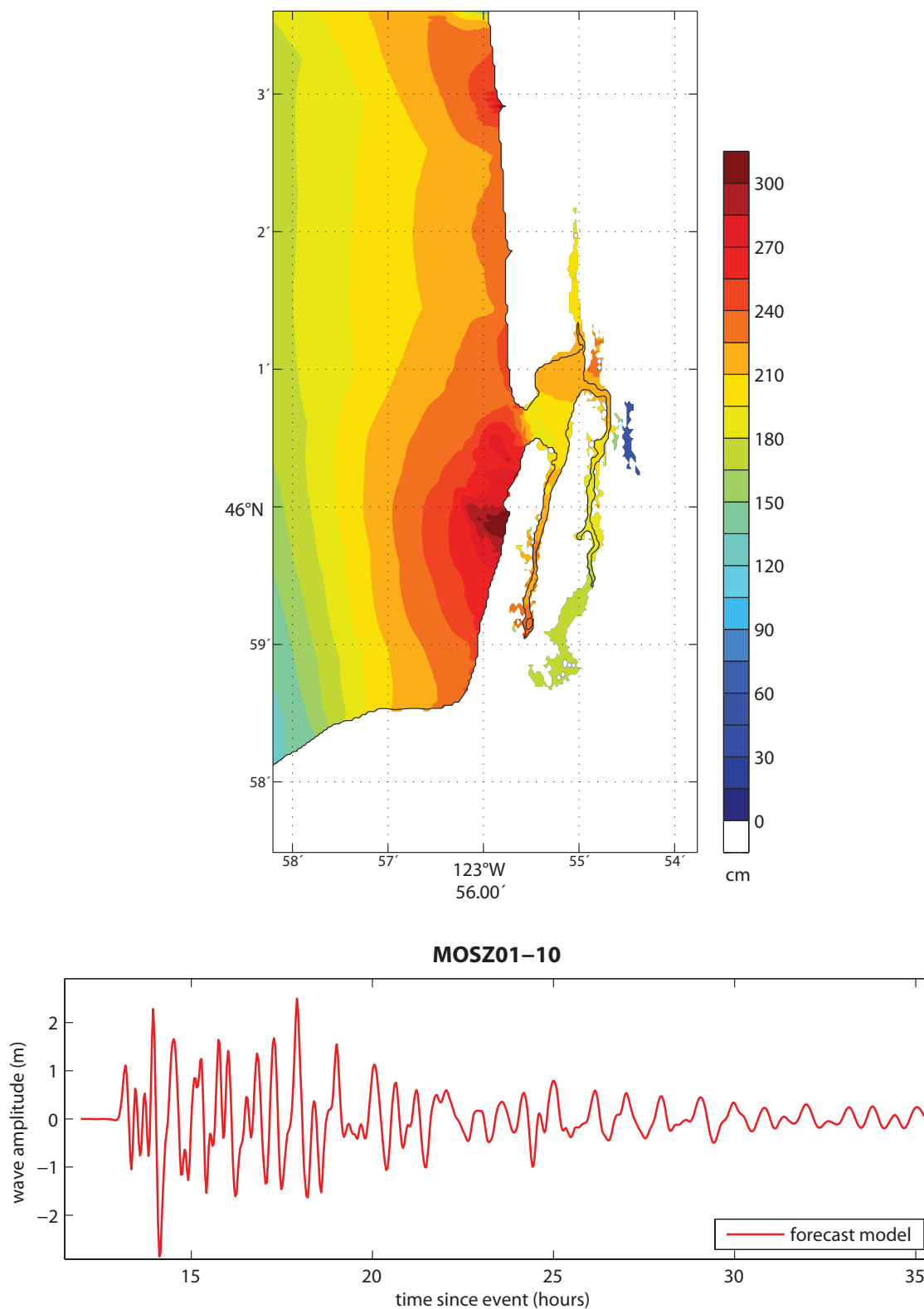
Figure 35: Results from the forecast model for the MOSZ 1–10 Mw 9.3 synthetic event. The upper panel shows the map of predicted maximum wave heights in the Seaside C-grid, and the lower panel shows the time series of wave amplitude at the warning point location.
