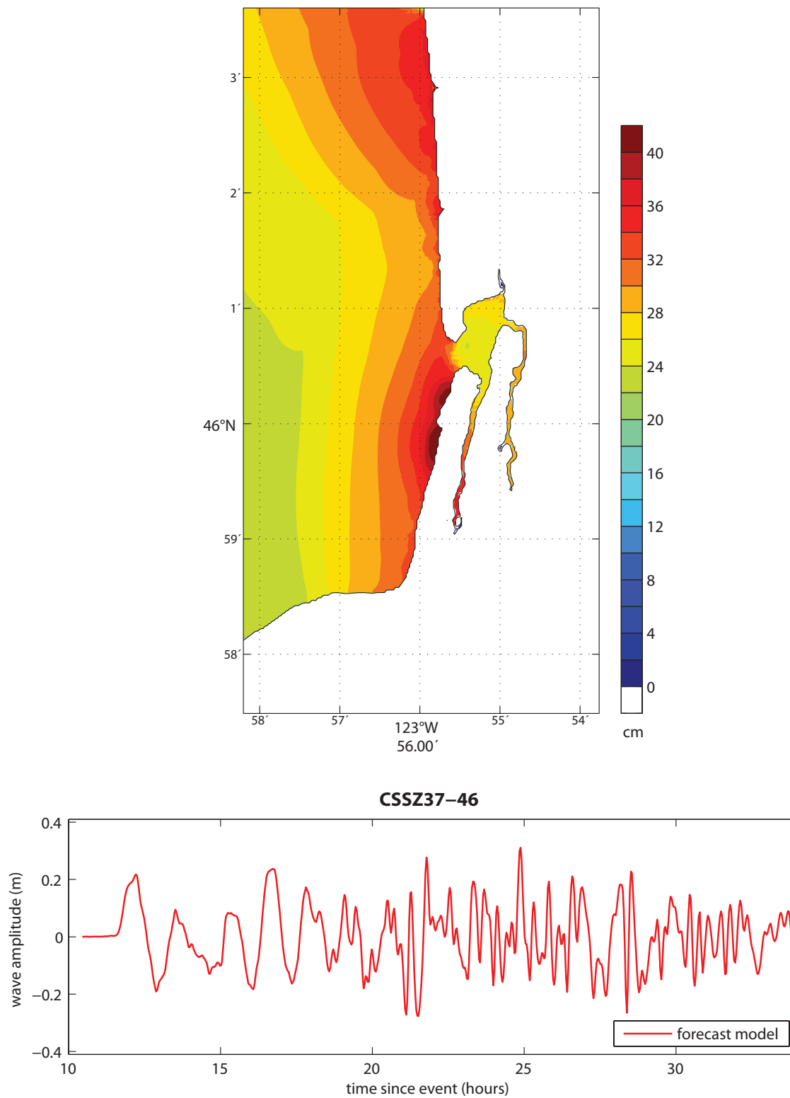
Figure 30: Results from the forecast model for the CSSZ 37–46 Mw 9.3 synthetic event. The upper panel shows the map of predicted maximum wave heights in the Seaside C-grid, and the lower panel shows the time series of wave amplitude at the warning point location.
