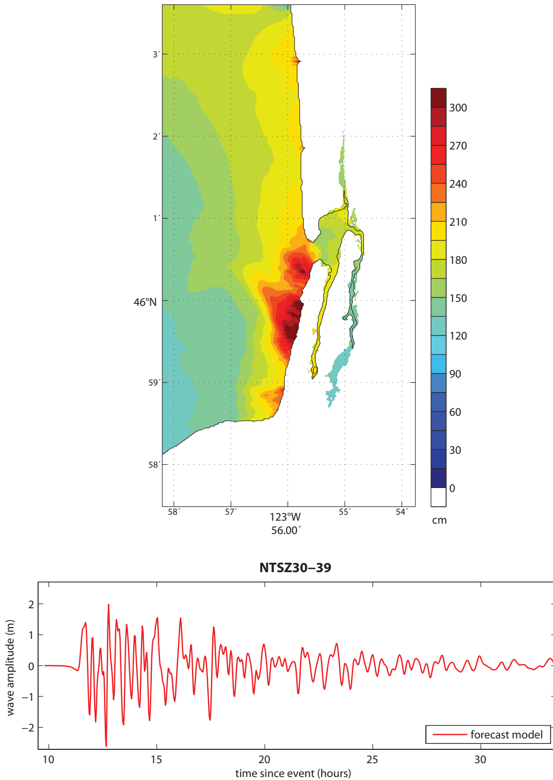
Figure 33: Results from the forecast model for the NTSZ 30–39 Mw 9.3 synthetic event. The upper panel shows the map of predicted maximum wave heights in the Seaside C-grid, and the lower panel shows the time series of wave amplitude at the warning point location.
