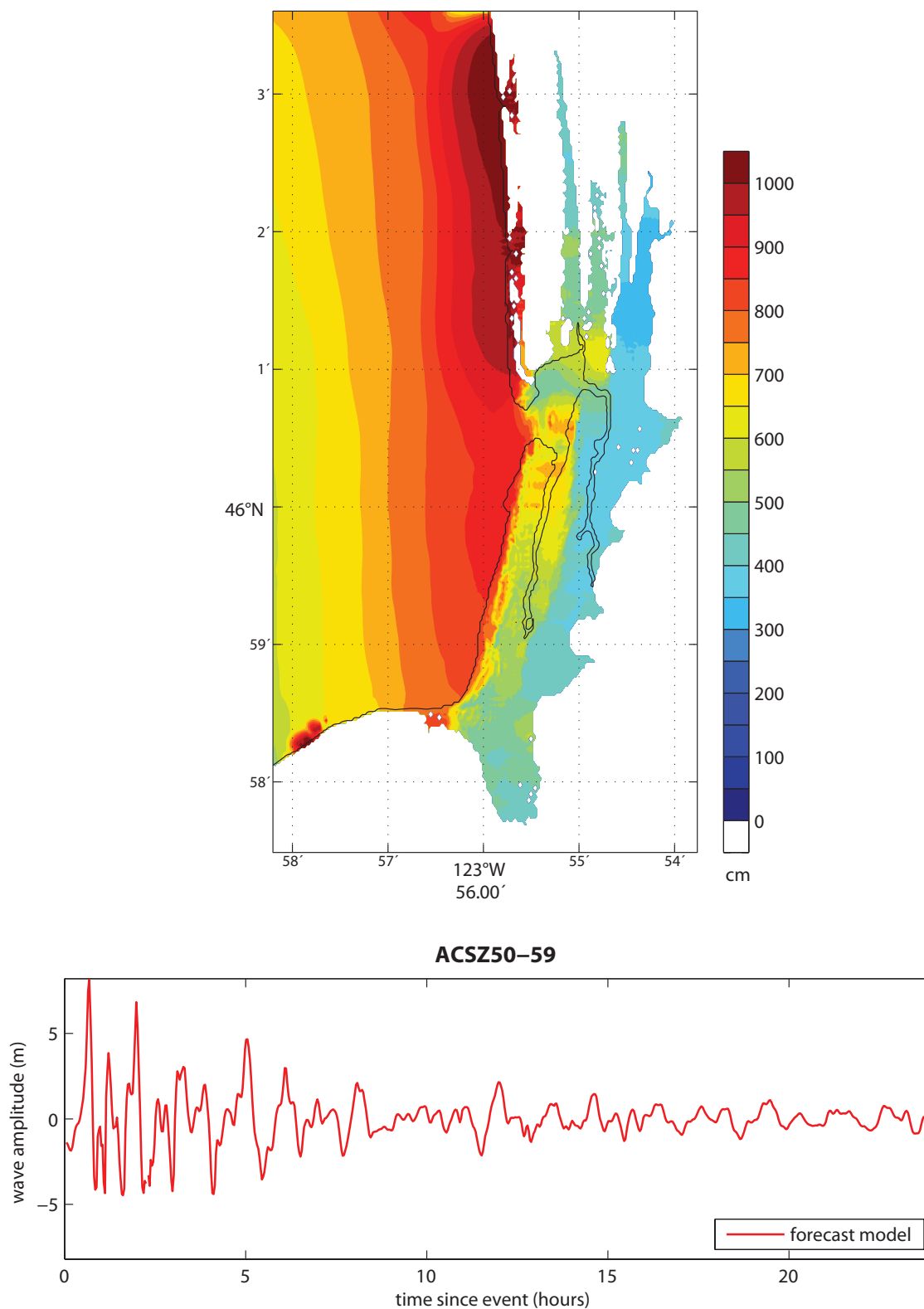
Figure 27: Results from the forecast model for the ACSZ 50–59 Mw 9.3 synthetic event. The upper panel shows the map of predicted maximum wave heights in the Seaside C-grid, and the lower panel shows the time series of wave amplitude at the warning point location.
