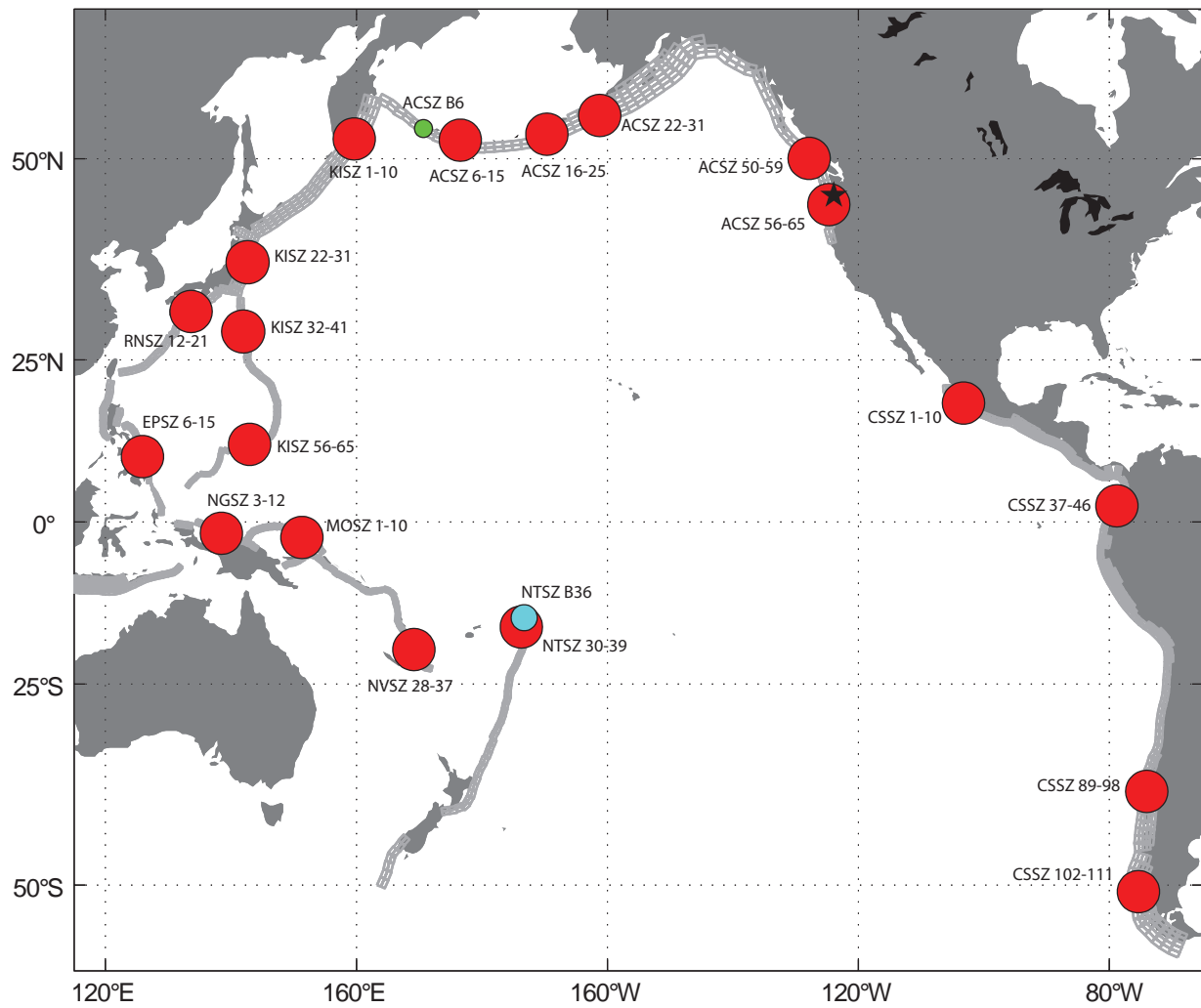
Figure 19: Map of the Pacific Ocean Basin showing location of 19 simulated Mw 9.3 events, the Mw 7.5 medium event, and the micro event used to test and validate the Seaside forecast model. The solid star denotes the location of Seaside.
