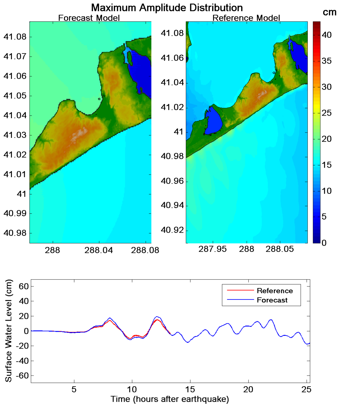
Figure 16. Maximum tsunami wave amplitude distribution of C-grid for synthetic scenario AT68-77ab with M_w=9.3 . Bottom figure is the simulated tsunami time series at the selected warning point (circle on the east side of the bay (north of Montauk)).
