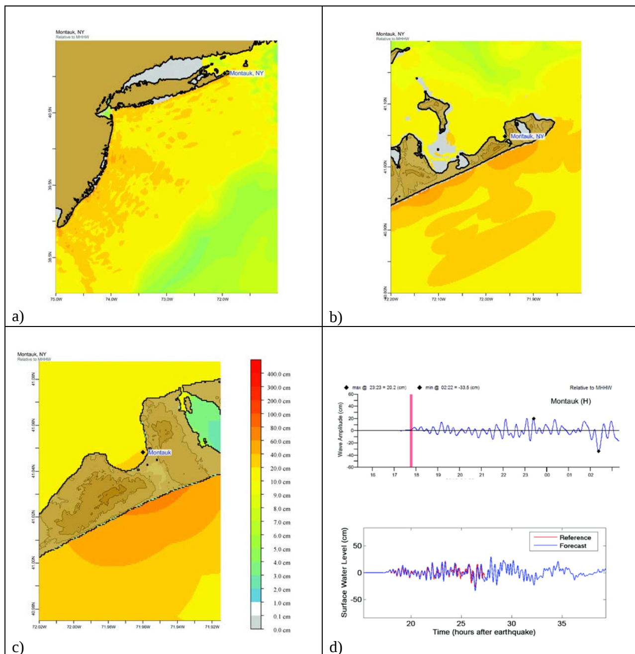
Figure 25. Response of the Montauk forecast model to synthetic scenario SSSZ 1-10 (alpha=25). Maximum sea surface elevation for (a) A-grid, b) B-grid, c) C-grid. Sea surface elevation time series at the C-grid warning point (d)
