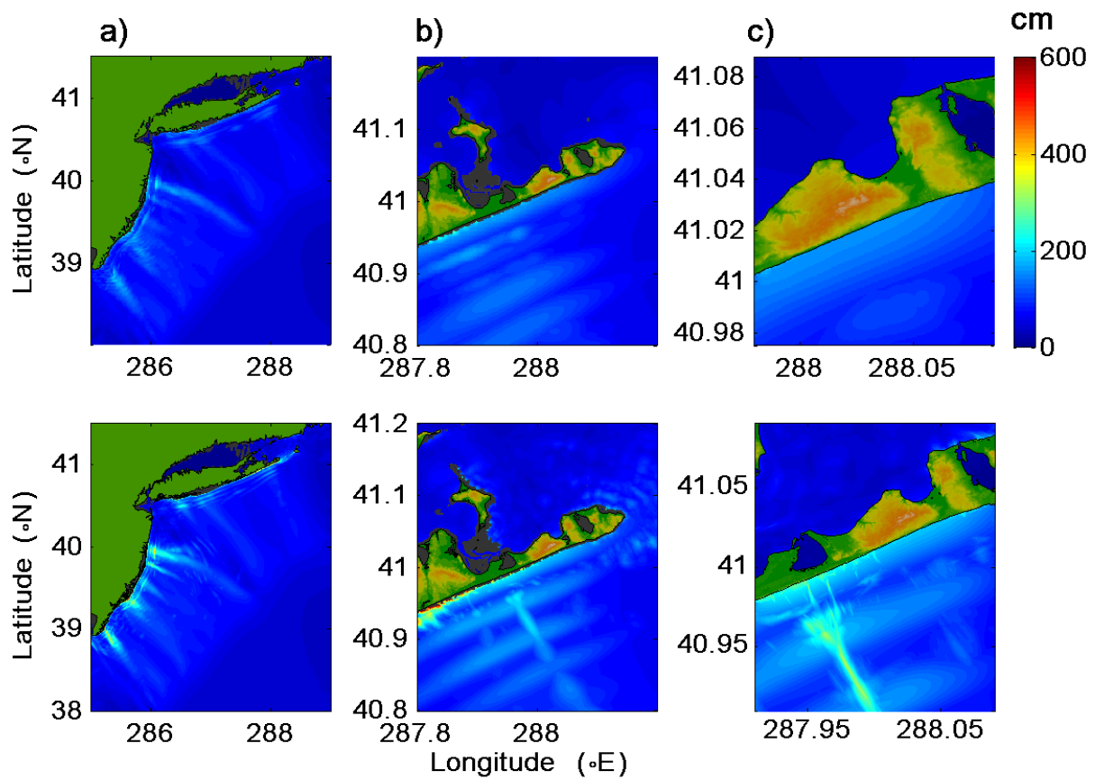
Figure 9. Maximum tsunami wave amplitude distribution for Grids A, B and C using synthetic scenario AT38-47ab with M_w=9.3 . Forecast model (upper) and reference model (lower).
