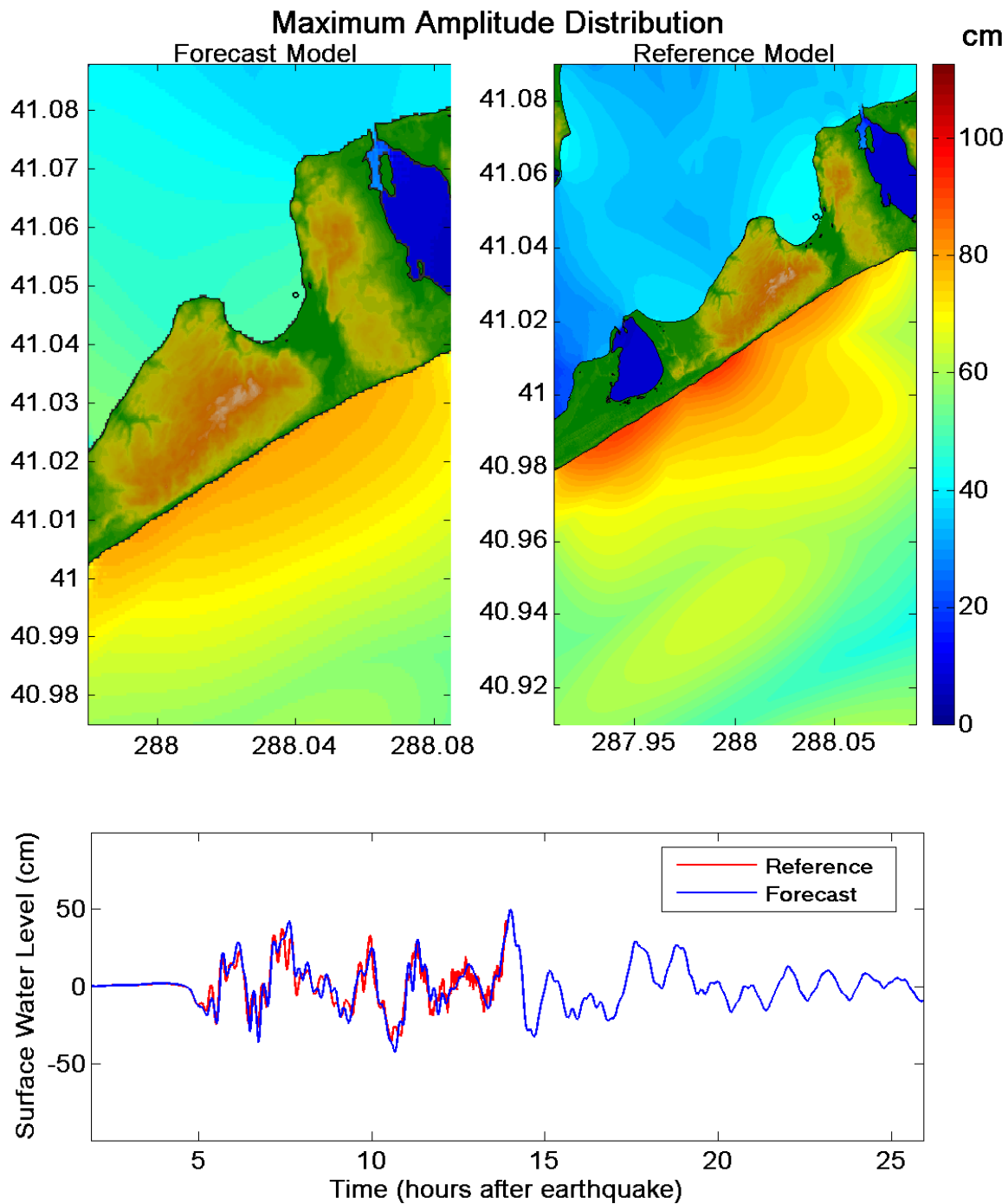
Figure 18. Maximum tsunami wave amplitude distribution of C-grid for synthetic scenario AT82-91ab with M_w=9.3 . Bottom figure is the simulated tsunami time series at the selected warning point (circle on the east side of the bay (north of Montauk)).
