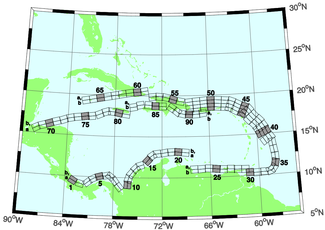
Figure 21. Atlantic Source Zone unit sources.
