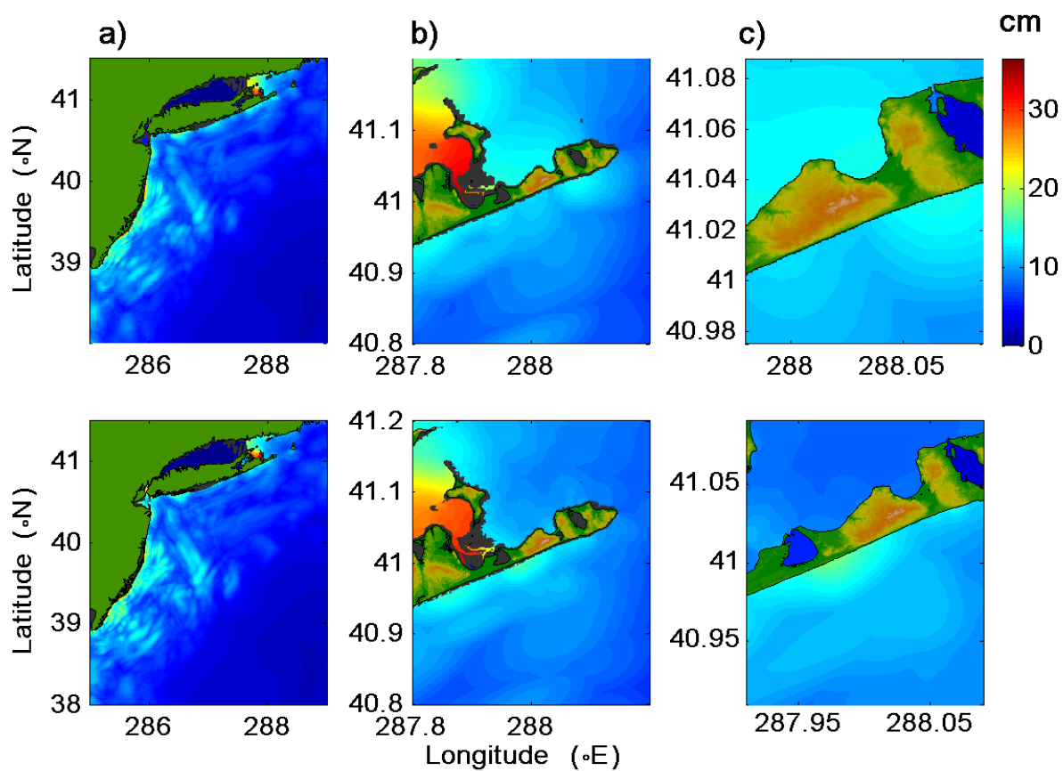
Figure 7. Maximum tsunami wave amplitude distribution for Grids A, B and C using 1755 Lisbon scenario. Forecast model (upper) and reference model (lower).
