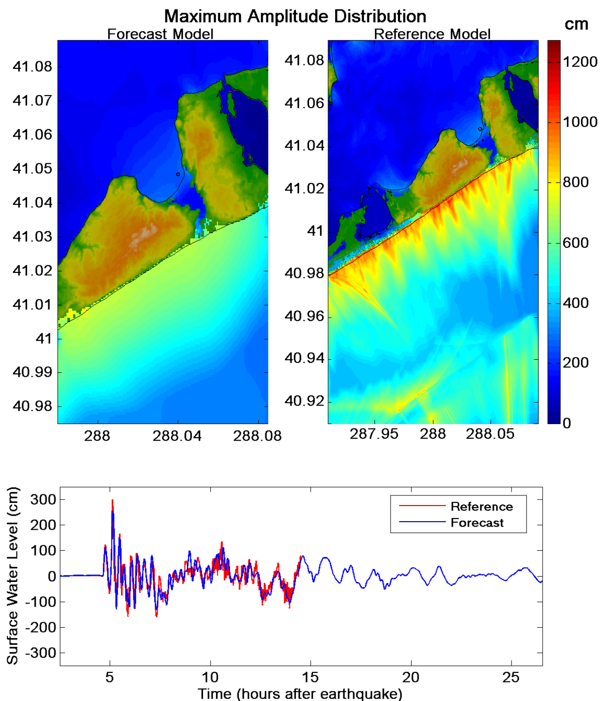
Figure 12. Maximum tsunami wave amplitude distribution of C-grid for synthetic scenario AT48-57ab with M_w=9.3 . Bottom figure is the simulated tsunami time series at the selected warning point (circle on the east side of the bay (north of Montauk)).
