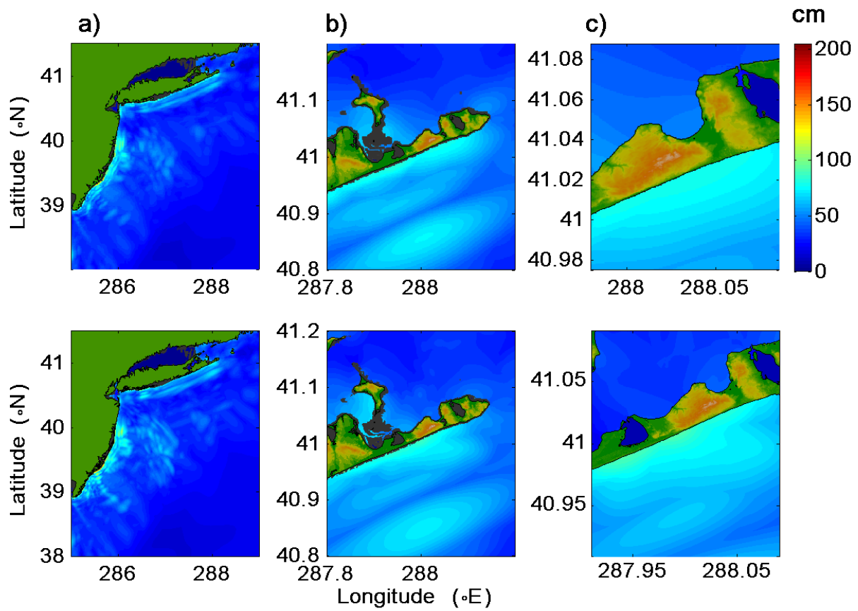
Figure 17. Maximum tsunami wave amplitude distribution for Grids A, B and C using synthetic scenario AT82-91ab with M_w=9.3 . Forecast model (upper) and reference model (lower).
