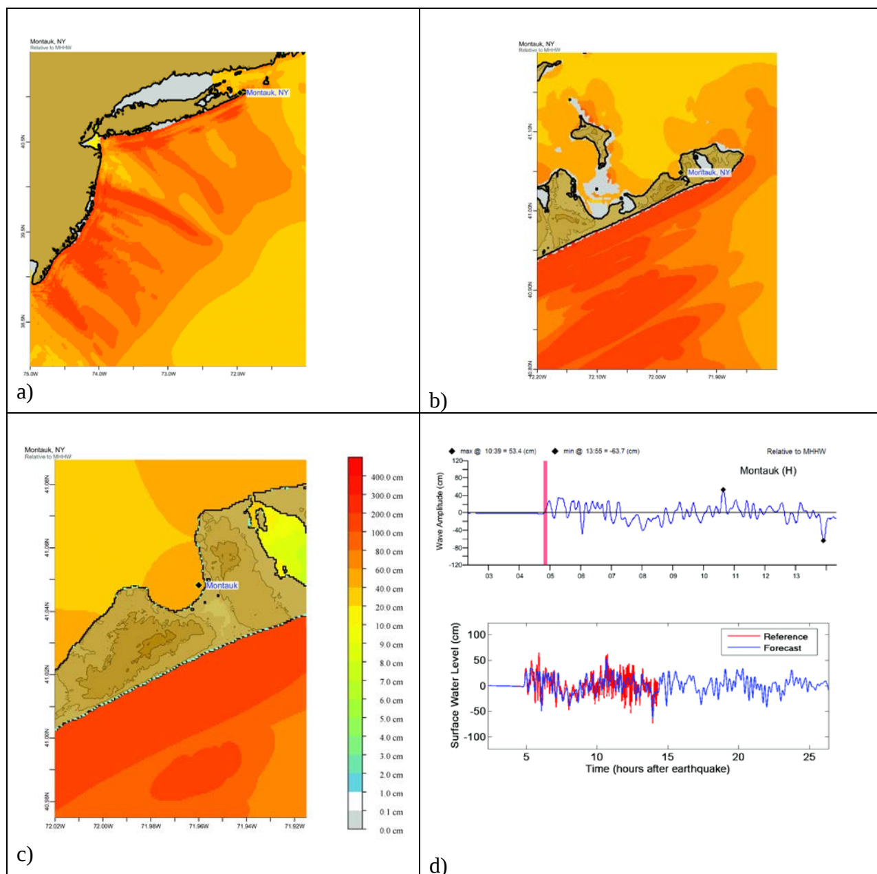
Figure 23. Response of the Montauk forecast model to synthetic scenario ATSZ 38-47 (alpha=25). Maximum sea surface elevation for (a) A-grid, b) B-grid, c) C-grid. Sea surface elevation time series at the C-grid warning point (d). The lower time series plot is the result obtained during model development and is shown for comparison with test results.
