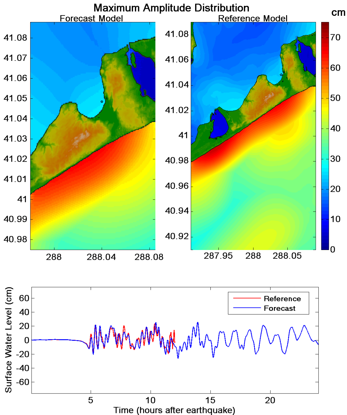
Figure 14. Maximum tsunami wave amplitude distribution of C-grid for synthetic scenario AT58-67ab with M_w=9.3 . Bottom figure is the simulated tsunami time series at the selected warning point (circle on the east side of the bay (north of Montauk)).
