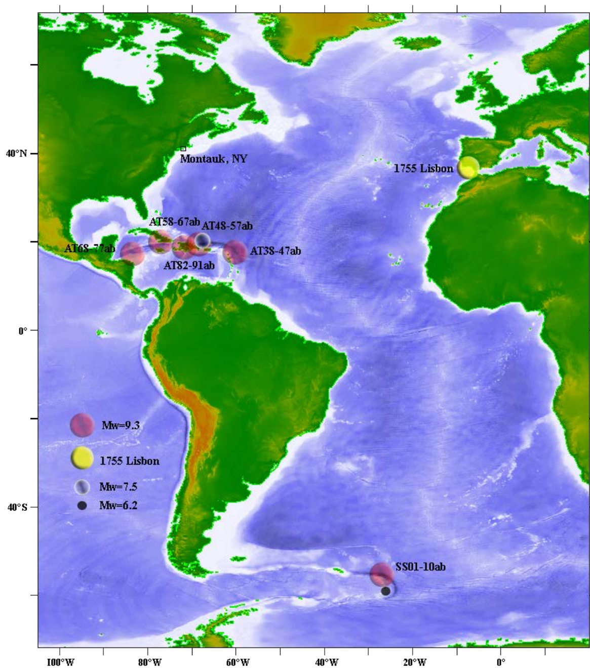
Figure 6. Location of synthetic scenarios simulated relative to Montauk, NY.
