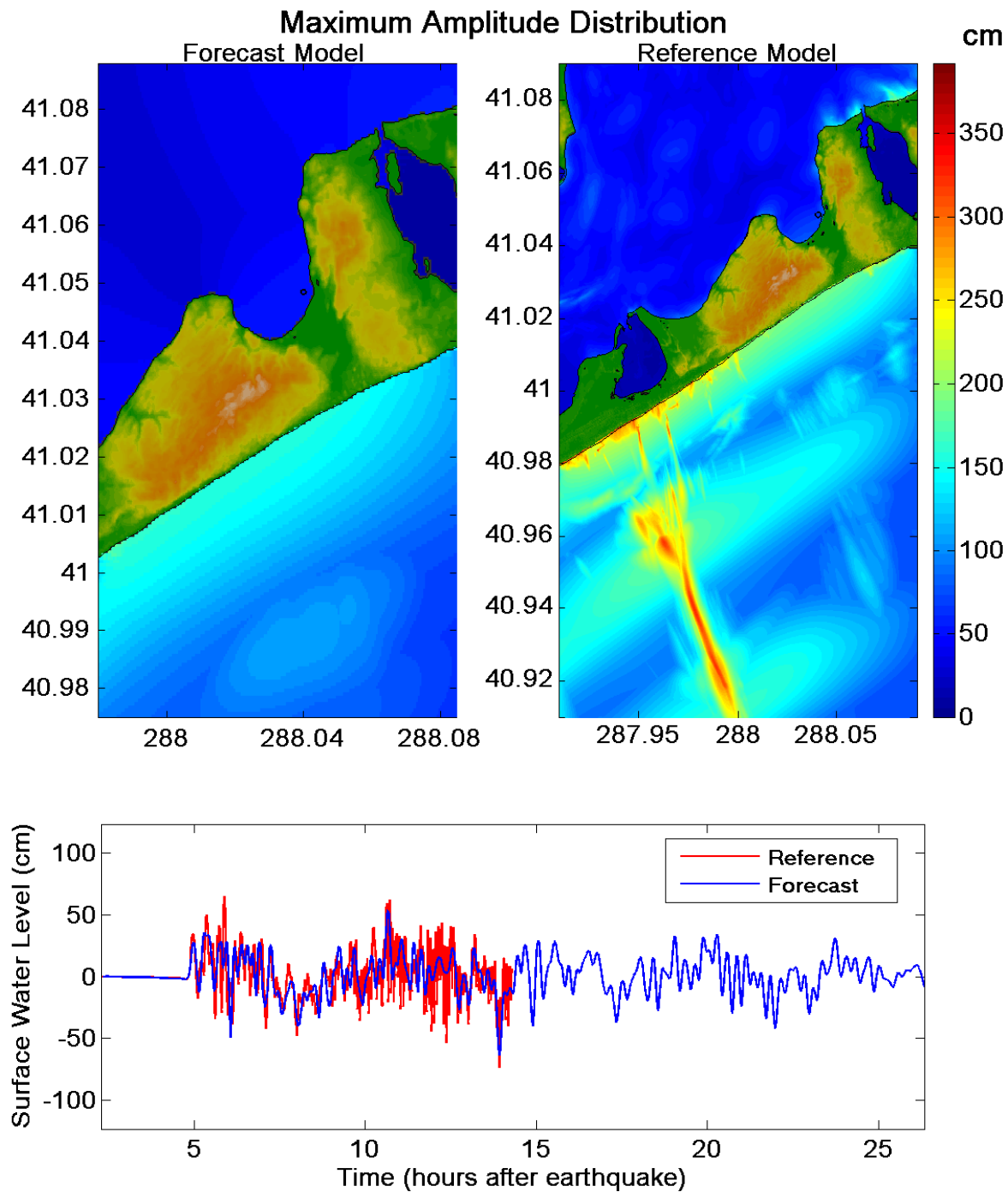
Figure 10. Maximum tsunami wave amplitude distribution of C-grid for synthetic scenario AT38-47ab with M_w=9.3 . Bottom figure is the simulated tsunami time series at the selected warning point (circle on the east side of the bay (north of Montauk)).
