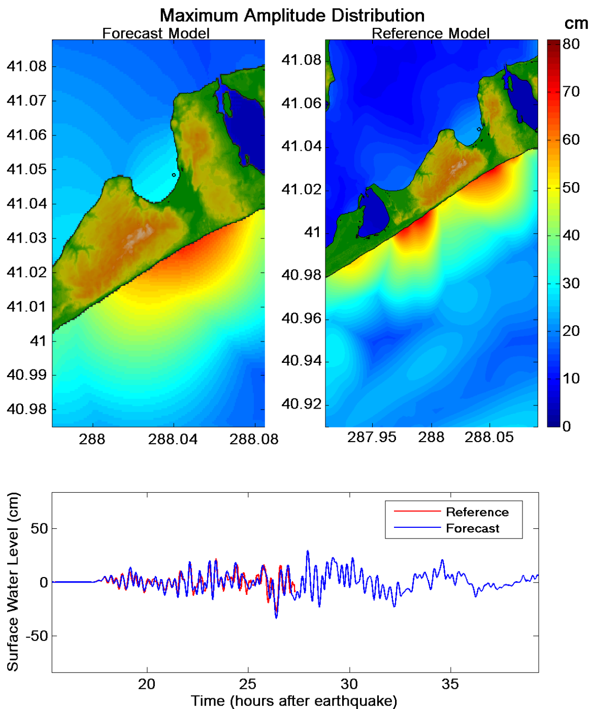
Figure 20. Maximum tsunami wave amplitude distribution of C-grid for synthetic scenario SS01-10ab with M_w=9.3 . Bottom figure is the simulated tsunami time series at the selected warning point (circle on the east side of the bay (north of Montauk)).
