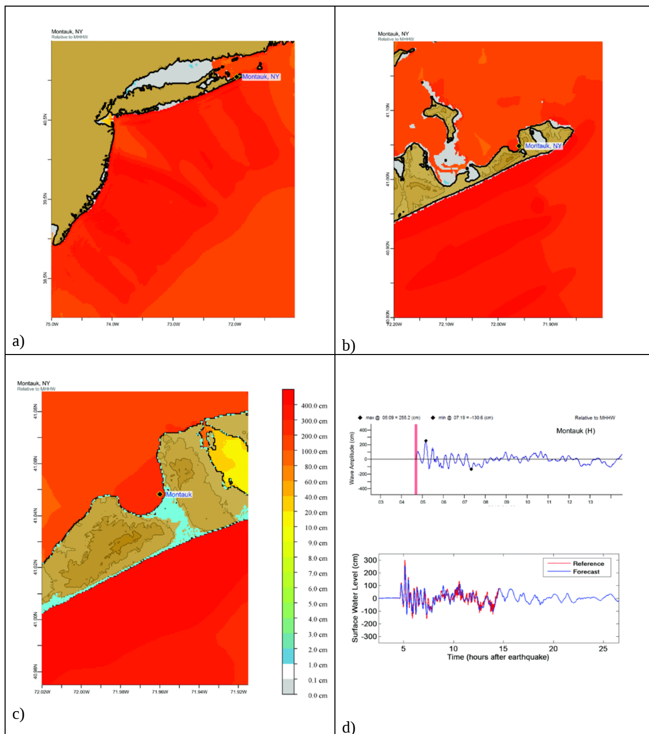
Figure 24. Response of the Montauk forecast model to synthetic scenario ATSZ 48-57 (alpha=25). Maximum sea surface elevation for (a) A-grid, b) B-grid, c) C-grid. Sea surface elevation time series at the C-grid warning point (d). The lower time series plot is the result obtained during model development and is shown for comparison with test results.
