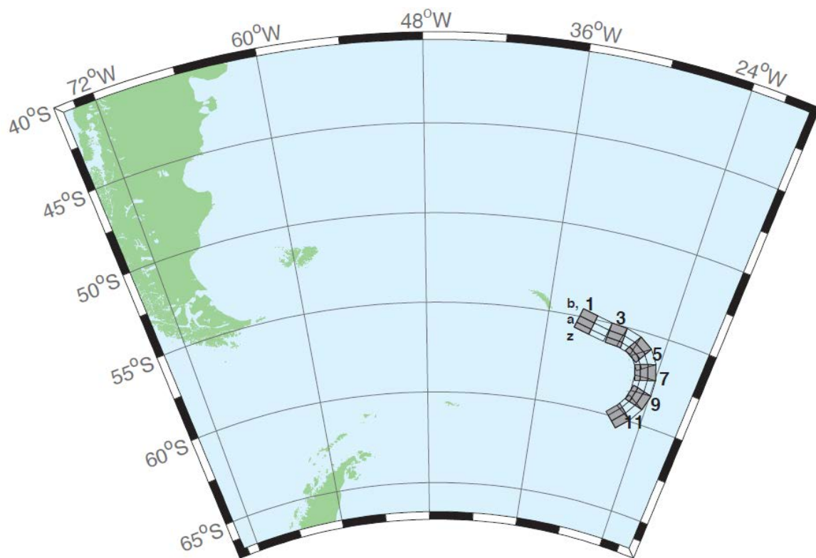
Figure 22. South Sandwich source zone unit sources.
