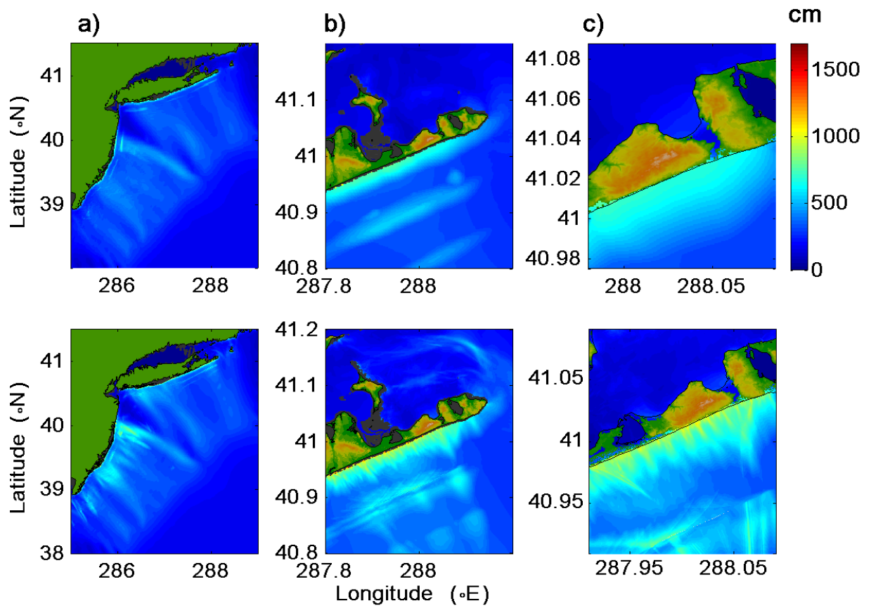
Figure 11. Maximum tsunami wave amplitude distribution for Grids A, B and C using synthetic scenario AT48-57ab with M_w=9.3 . Forecast model (upper) and reference model (lower).
