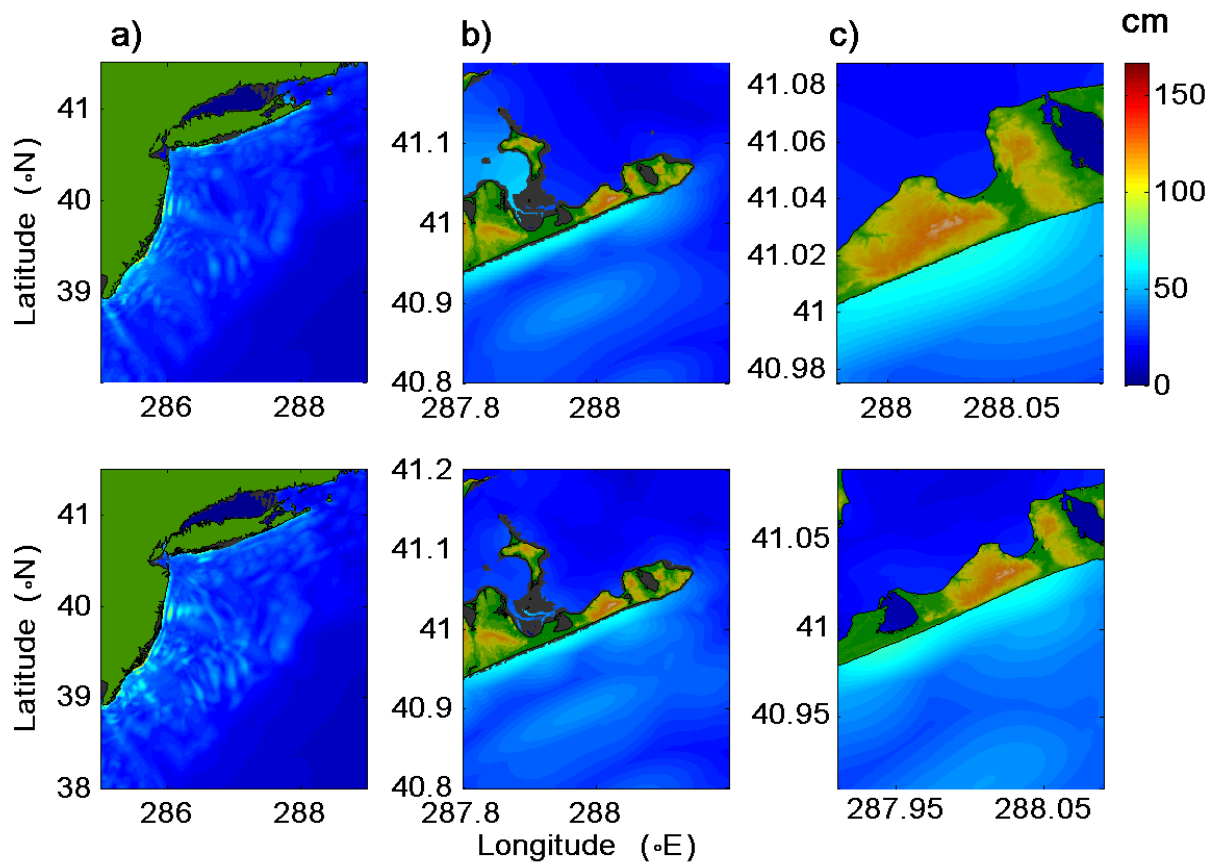
Figure 13. Maximum tsunami wave amplitude distribution for Grids A, B and C using synthetic scenario AT58-67ab with M_w=9.3 . Forecast model (upper) and reference model (lower).
