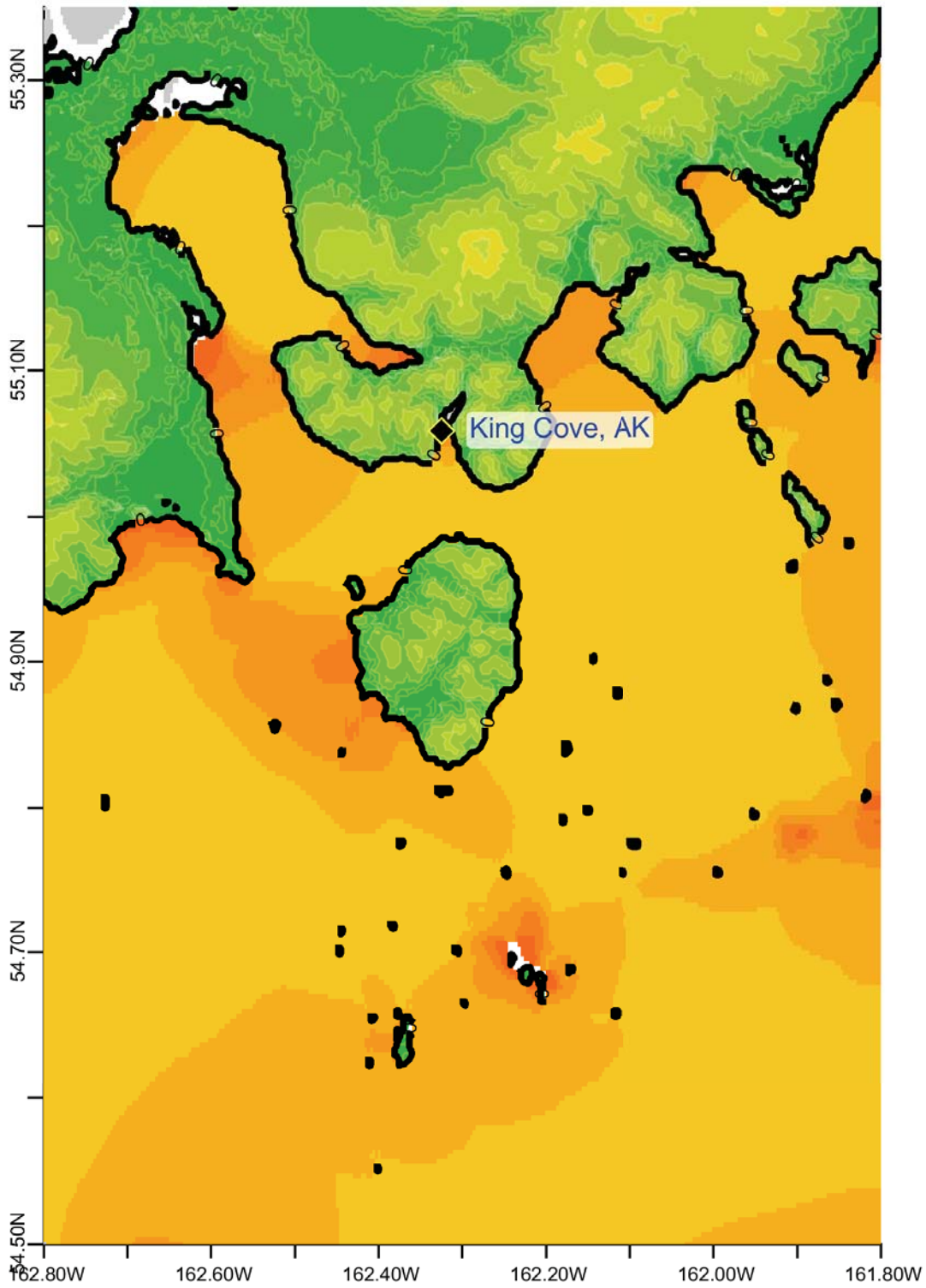
Figure 10. Max computed wave amplitude of B grid, King Cove, Alaska, for synthetic event CSSZ 89-98.
