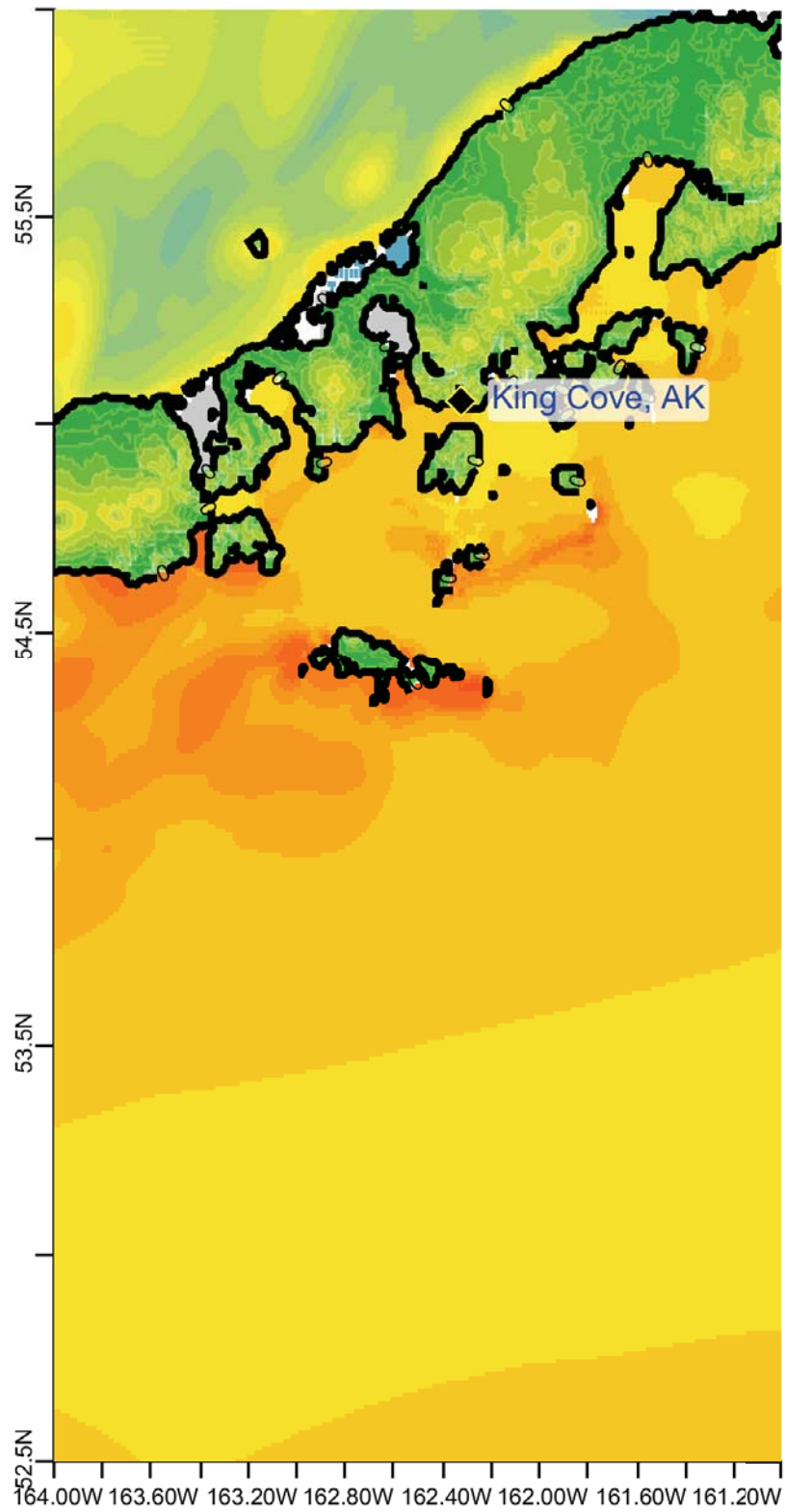
Figure 9. Max computed wave amplitude of A grid, King Cove, Alaska, for synthetic event CSSZ 89-98.
