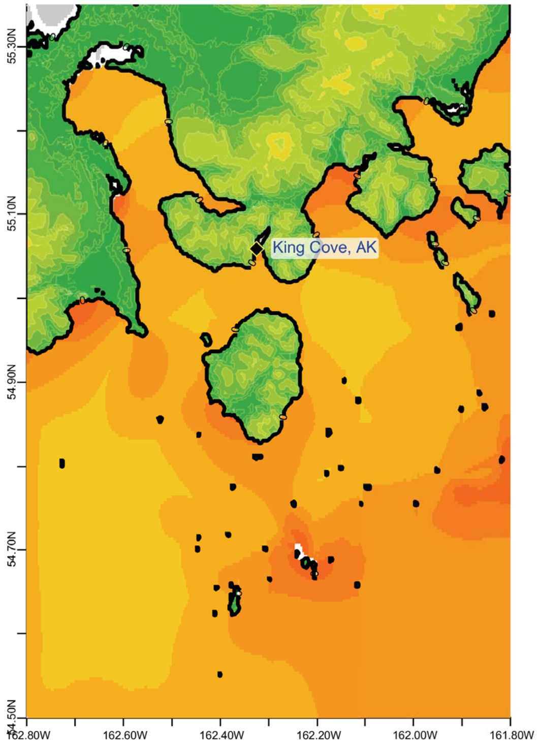
Figure 14. Max computed wave amplitude of B grid, King Cove, Alaska, for synthetic event NTSZ 30-39.
