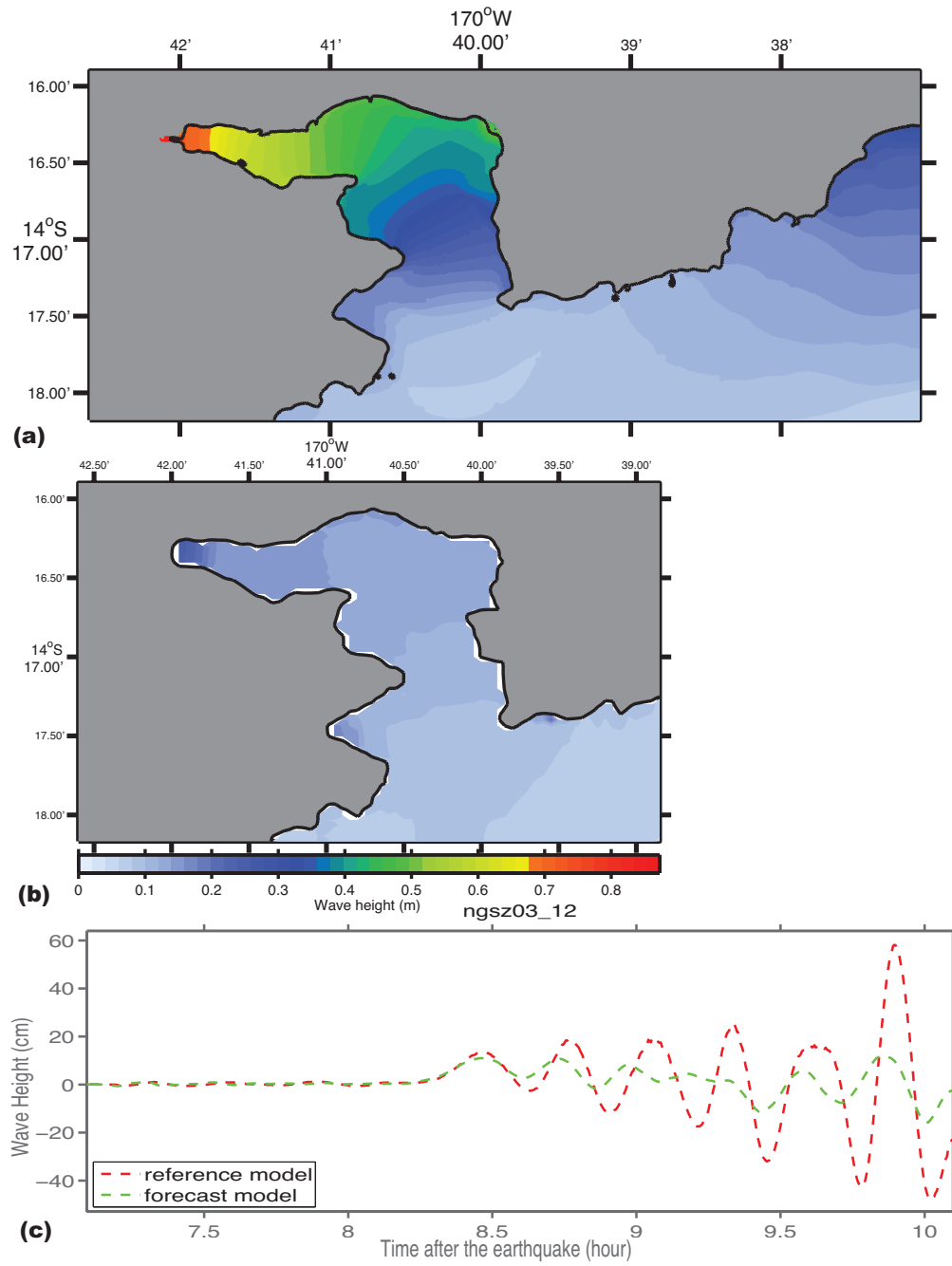
Figure 32: Magnitude 9.4 NGSZ source segment 3-12 synthetic scenario model results. (a) Maximum computed wave heights computed with reference model grids. (b) Maximum computed wave heights computed with forecast model grids. (c) Comparison of time series computed with reference model and forecast model grids at the Pago Pago tide gauge.
