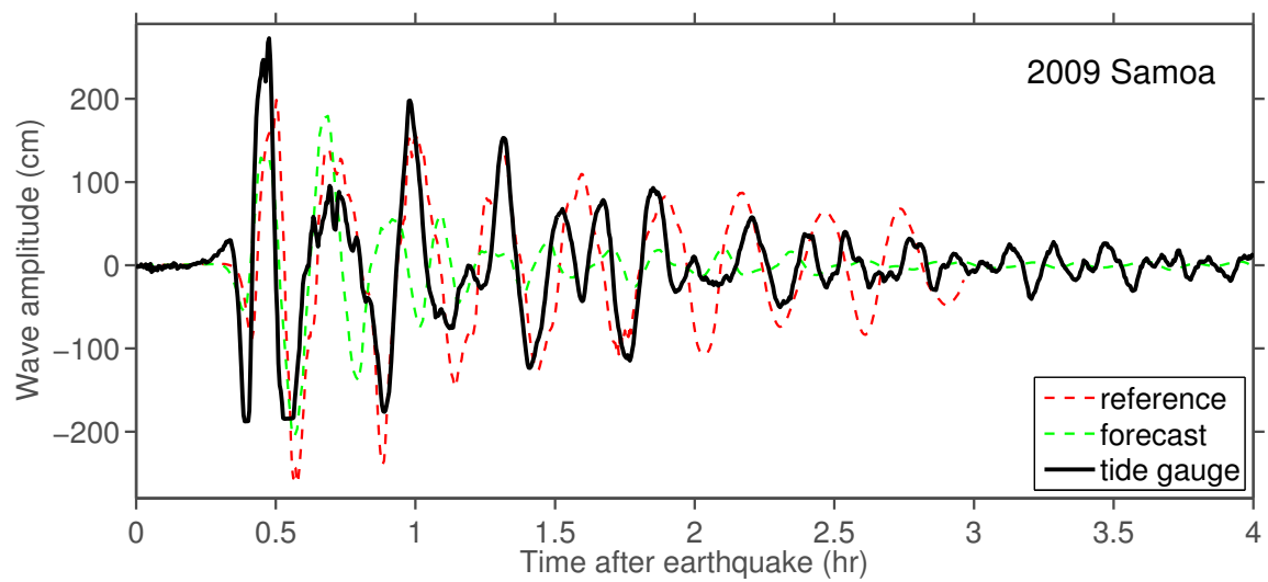
Figure 13: Pago Pago harbor tide gauge observations during the 2009 Samoa tsunami compared to reference and forecast model predictions.
