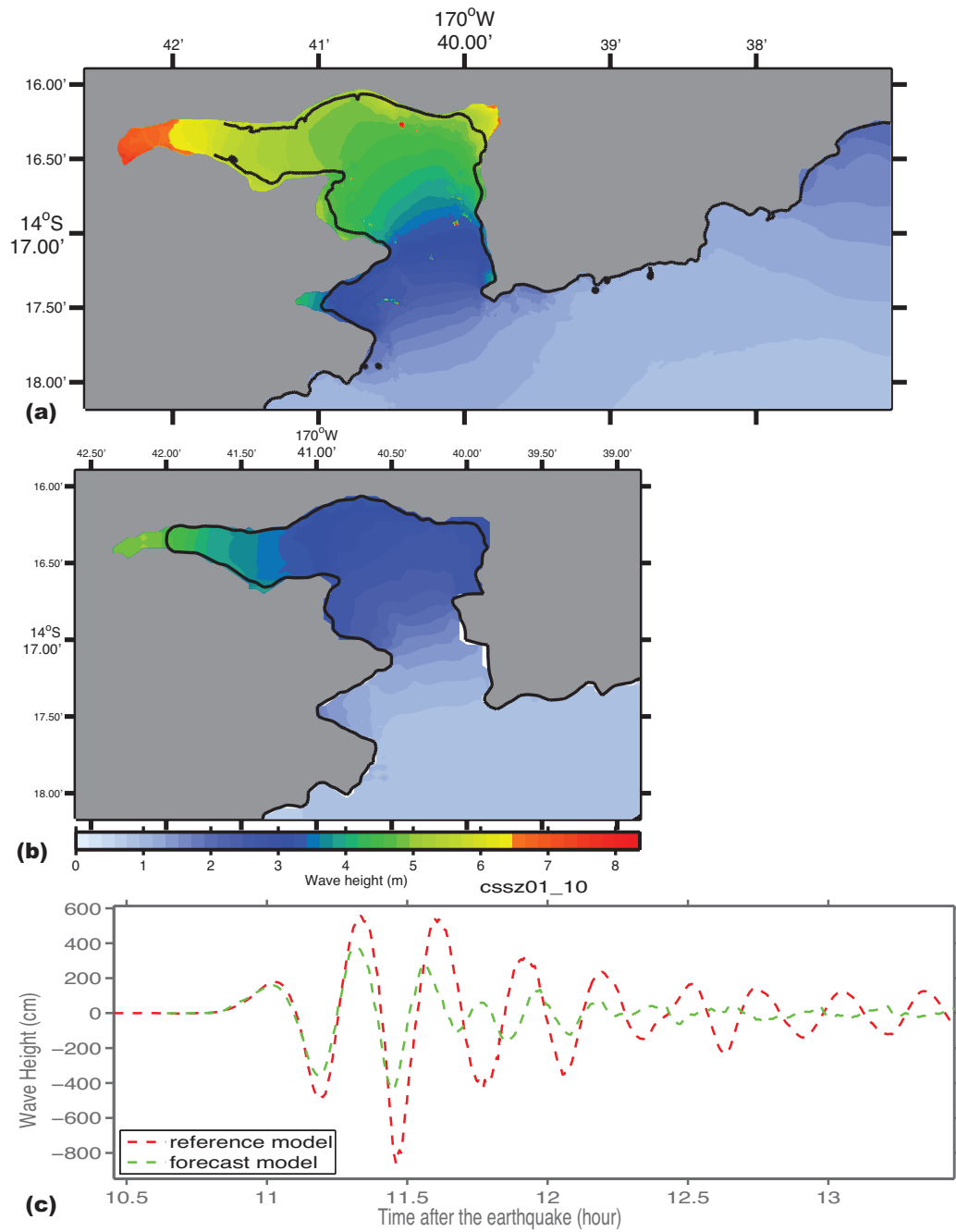
Figure 22: Magnitude 9.4 CSSZ source segment 1-10 synthetic scenario model results. (a) Maximum computed wave heights computed with reference model grids. (b) Maximum computed wave heights computed with forecast model grids. (c) Comparison of time series computed with reference model and forecast model grids at the Pago Pago tide gauge.
