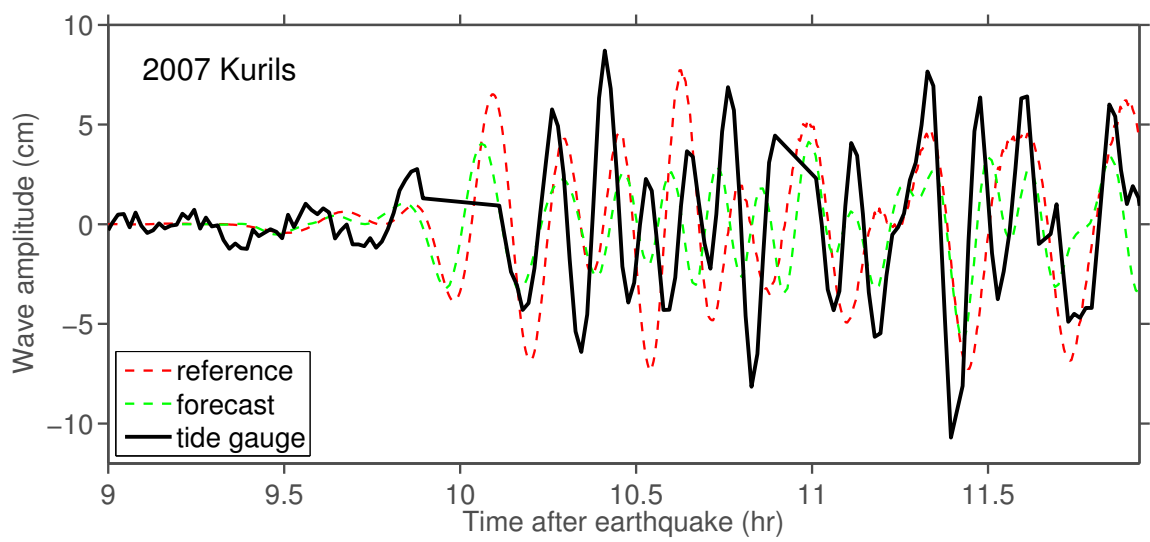
Figure 11: Pago Pago harbor tide gauge observations during the 2007 Kuril Islands tsunami compared to reference and forecast model predictions.
