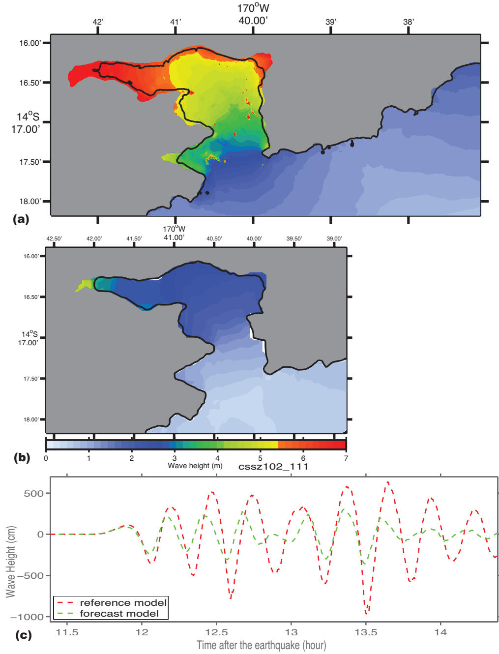
Figure 25: Magnitude 9.4 CSSZ source segment 102-111 synthetic scenario model results. (a) Maximum computed wave heights computed with reference model grids. (b) Maximum computed wave heights computed with forecast model grids. (c) Comparison of time series computed with reference model and forecast model grids at the Pago Pago tide gauge.
