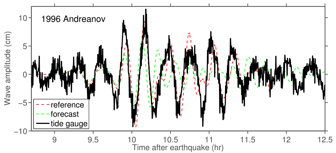
Figure 9: Pago Pago harbor tide gauge observations during the 1996 Andreanov tsunami compared to reference and forecast model predictions.
