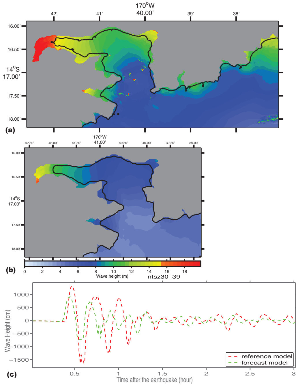
Figure 33: Magnitude 9.4 NTSZ source segment 30-39 synthetic scenario model results. (a) Maximum computed wave heights computed with reference model grids. (b) Maximum computed wave heights computed with forecast model grids. (c) Comparison of time series computed with reference model and forecast model grids at the Pago Pago tide gauge.
