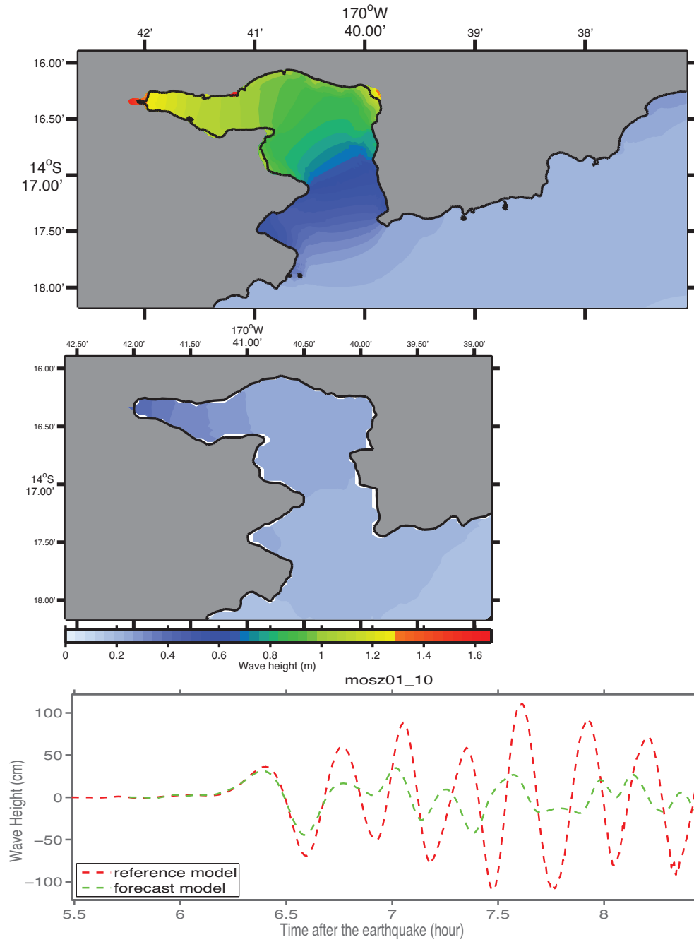
Figure 31: Magnitude 9.4 MOSZ source segment 1-10 synthetic scenario model results. (a) Maximum computed wave heights computed with reference model grids. (b) Maximum computed wave heights computed with forecast model grids. (c) Comparison of time series computed with reference model and forecast model grids at the Pago Pago tide gauge.
