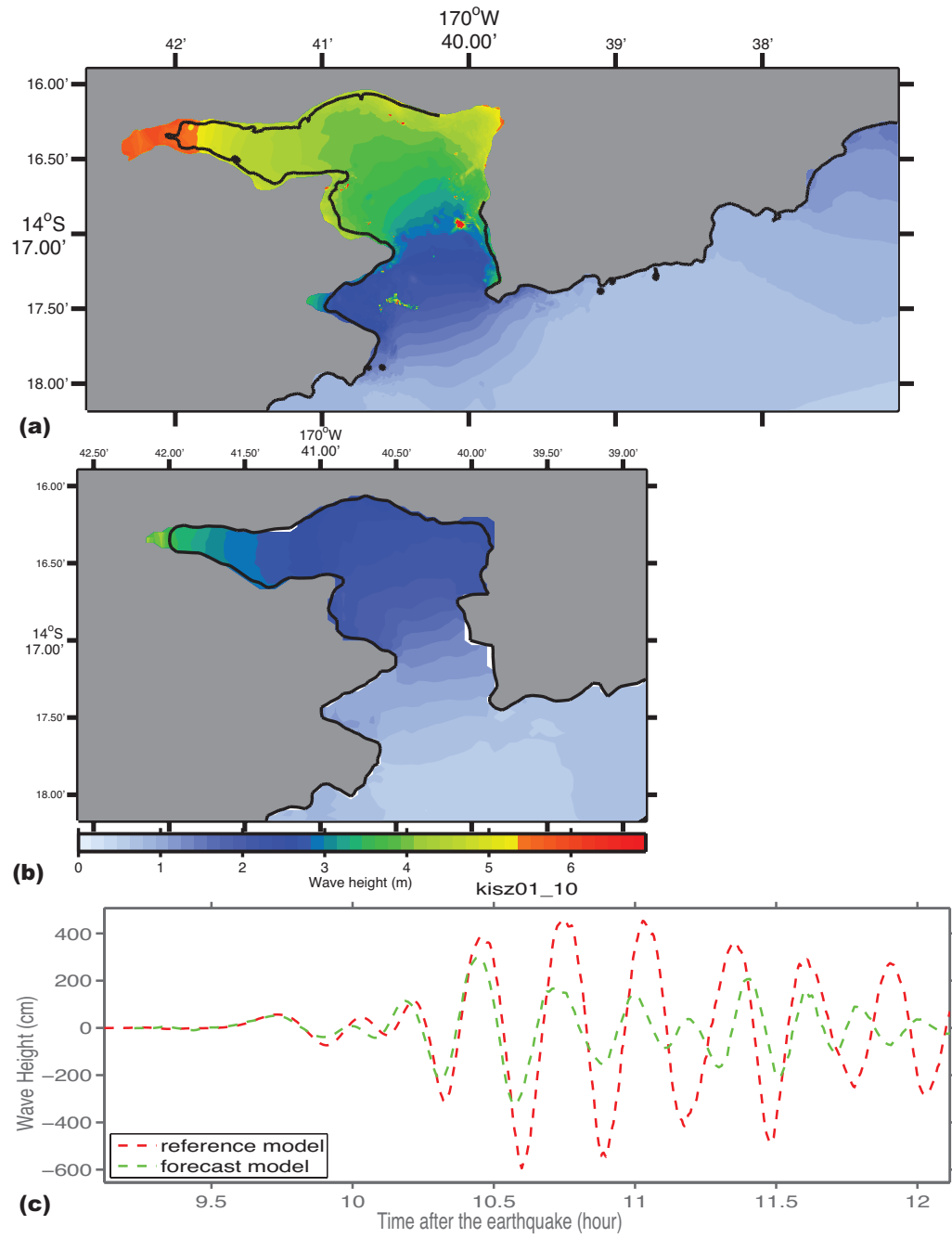
Figure 27: Magnitude 9.4 KISZ source segment 1-10 synthetic scenario model results. (a) Maximum computed wave heights computed with reference model grids. (b) Maximum computed wave heights computed with forecast model grids. (c) Comparison of time series computed with reference model and forecast model grids at the Pago Pago tide gauge
