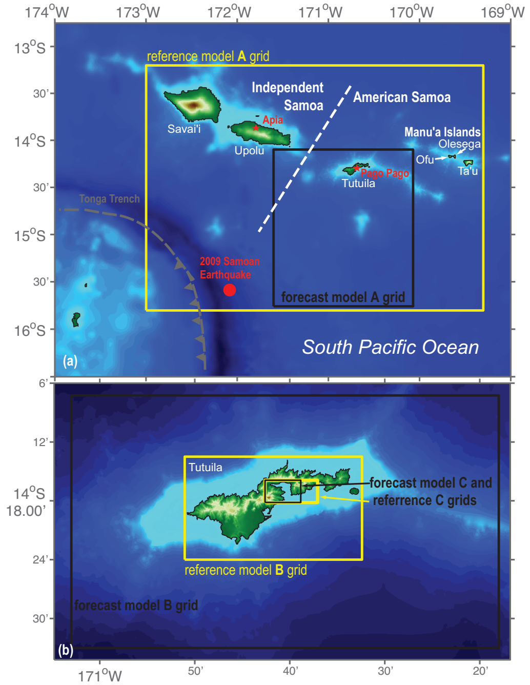
Figure 2: The three nested grids developed for the Pago Pago tsunami forecast model are illustrated. In 2a) the grid extent of the outermost A-grid in South Pacific and the location of Samoan islands and Tonga Trench are shown. The island of Tutuila and the extent of the innermost C-grid and the extent of the intermediate B-grid are shown in 2b).
