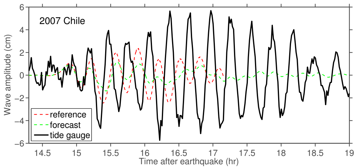
Figure 10: Pago Pago harbor tide gauge observations during the 2007 Chile tsunami compared to reference and forecast model predictions.
