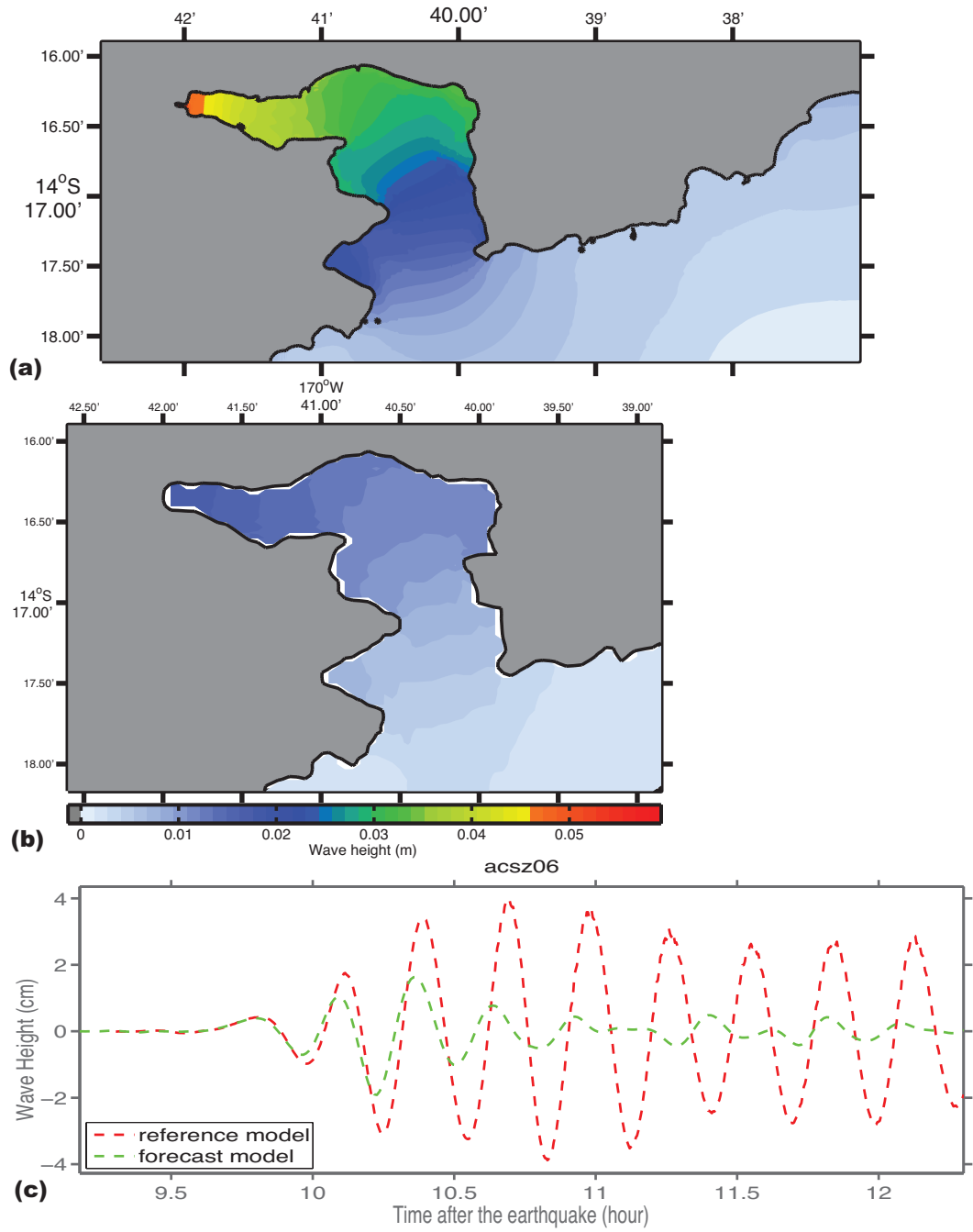
Figure 38: Magnitude 7.5 ACSZ source segment B6 synthetic scenario model results. (a) Maximum computed wave heights computed with reference model grids. (b) Maximum computed wave heights computed with forecast model grids. (c) Comparison of time series computed with reference model and forecast model grids at the Pago Pago tide gauge.
