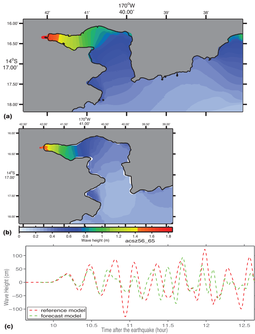
Figure 21: Magnitude 9.4 AASZ source segment 56-65 synthetic scenario model results. (a) Maximum computed wave heights computed with reference model grids. (b) Maximum computed wave heights computed with forecast model grids. (c) Comparison of time series computed with reference model and forecast model grids at the Pago Pago tide gauge.
