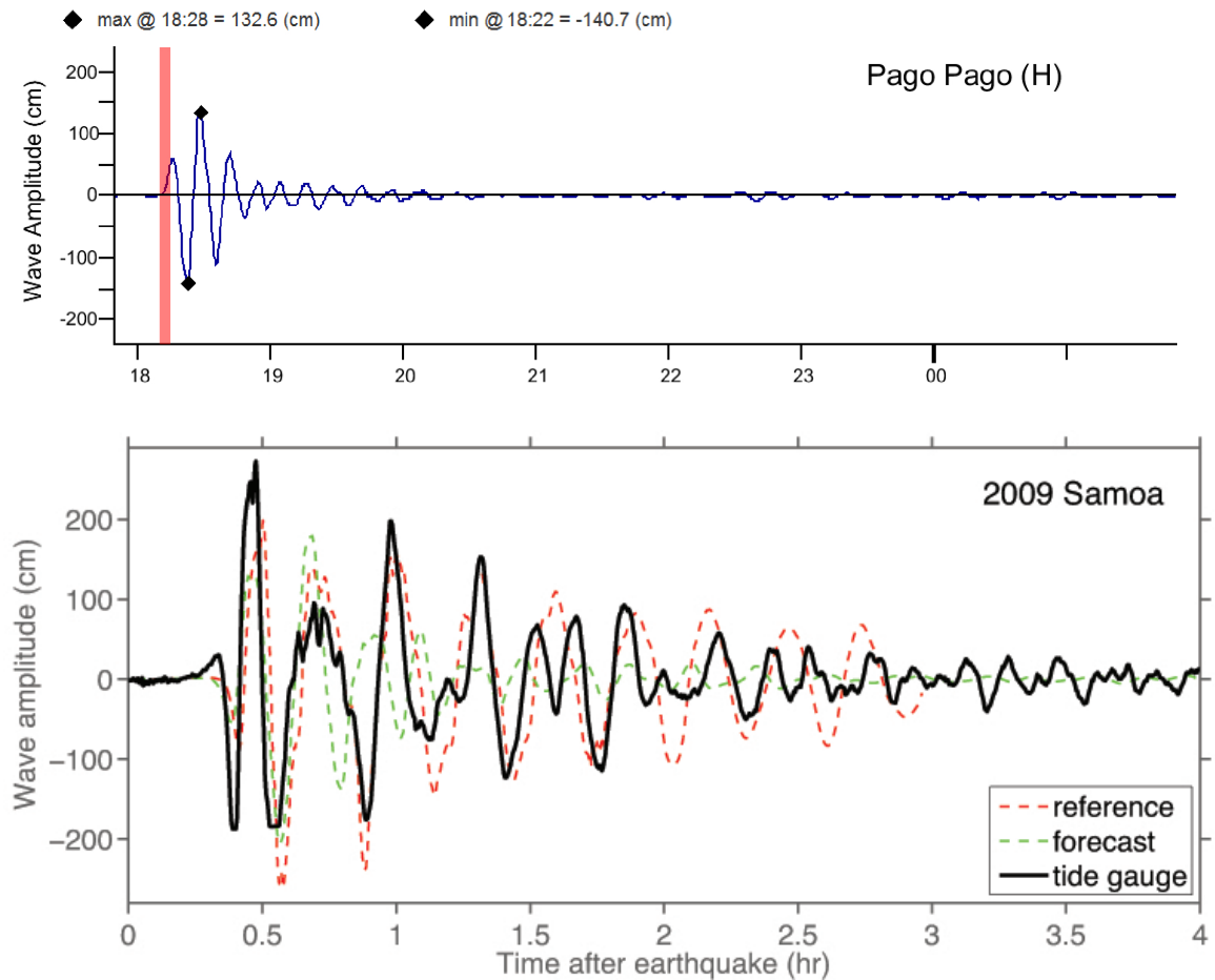
Figure C.5: Response of the Pago Pago forecast model to the 2009 Samoa tsunami. Maximum sea surface elevation for (a) A-grid, b) B-grid, c) C-grid. Sea surface elevation time series at the C-grid warning point (d). The lower time series plot is the result obtained during model development and is shown for comparison with test results.
