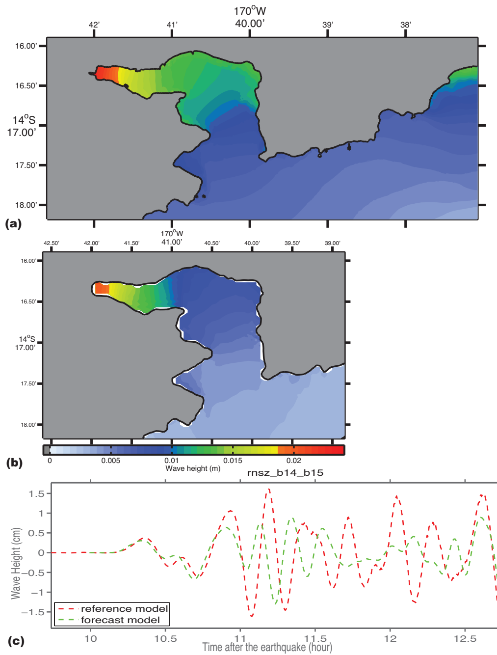
Figure 37: Magnitude 8.0 RNSZ source segment B14-B15 synthetic scenario model results. (a) Maximum computed wave heights computed with reference model grids. (b) Maximum computed wave heights computed with forecast model grids. (c) Comparison of time series computed with reference model and forecast model grids at the Pago Pago tide gauge.
