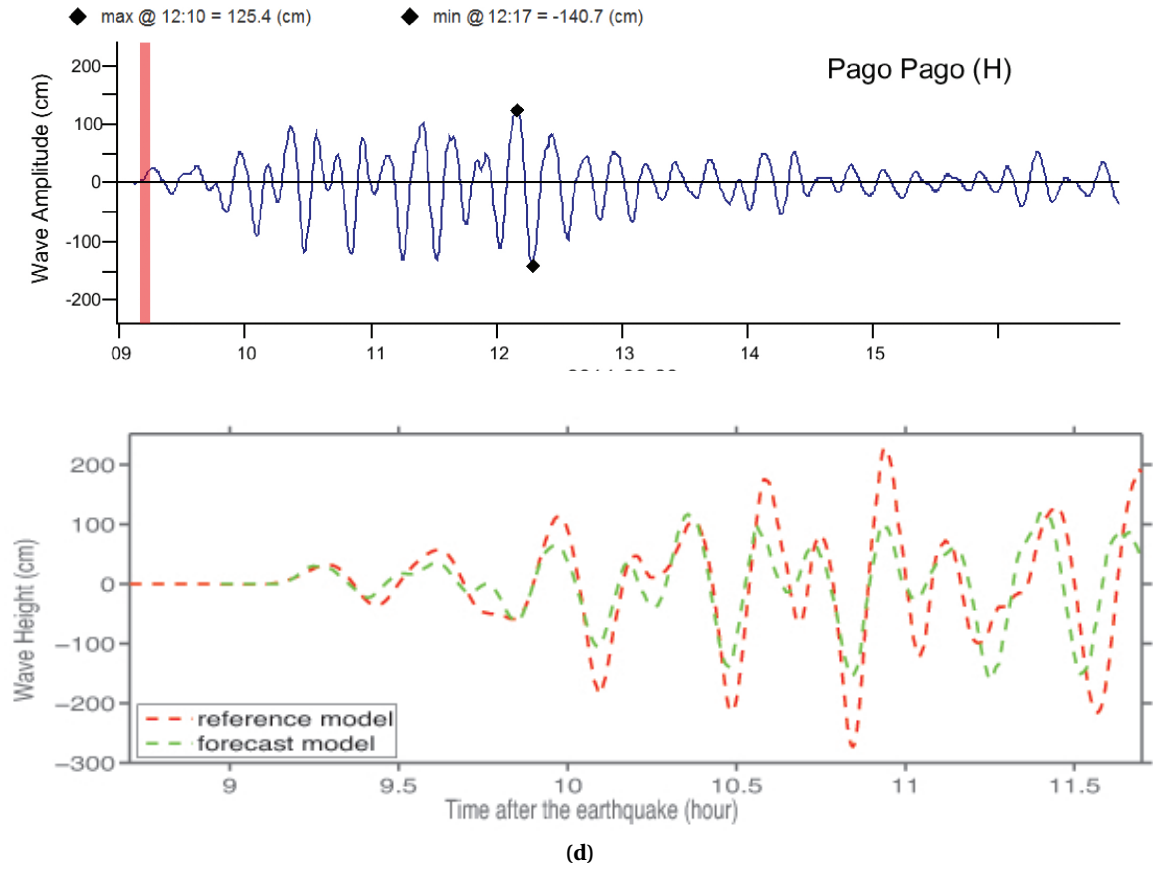
Figure C.1: Response of the Pago Pago forecast model to synthetic scenario KISZ 22-31 ( \alpha=25 ). Maximum sea surface elevation for (a) A-grid, b) B-grid, c) C-grid. Sea surface elevation time series at the C-grid warning point (d). The lower time series plot is the result obtained during model development and is shown for comparison with test results.
