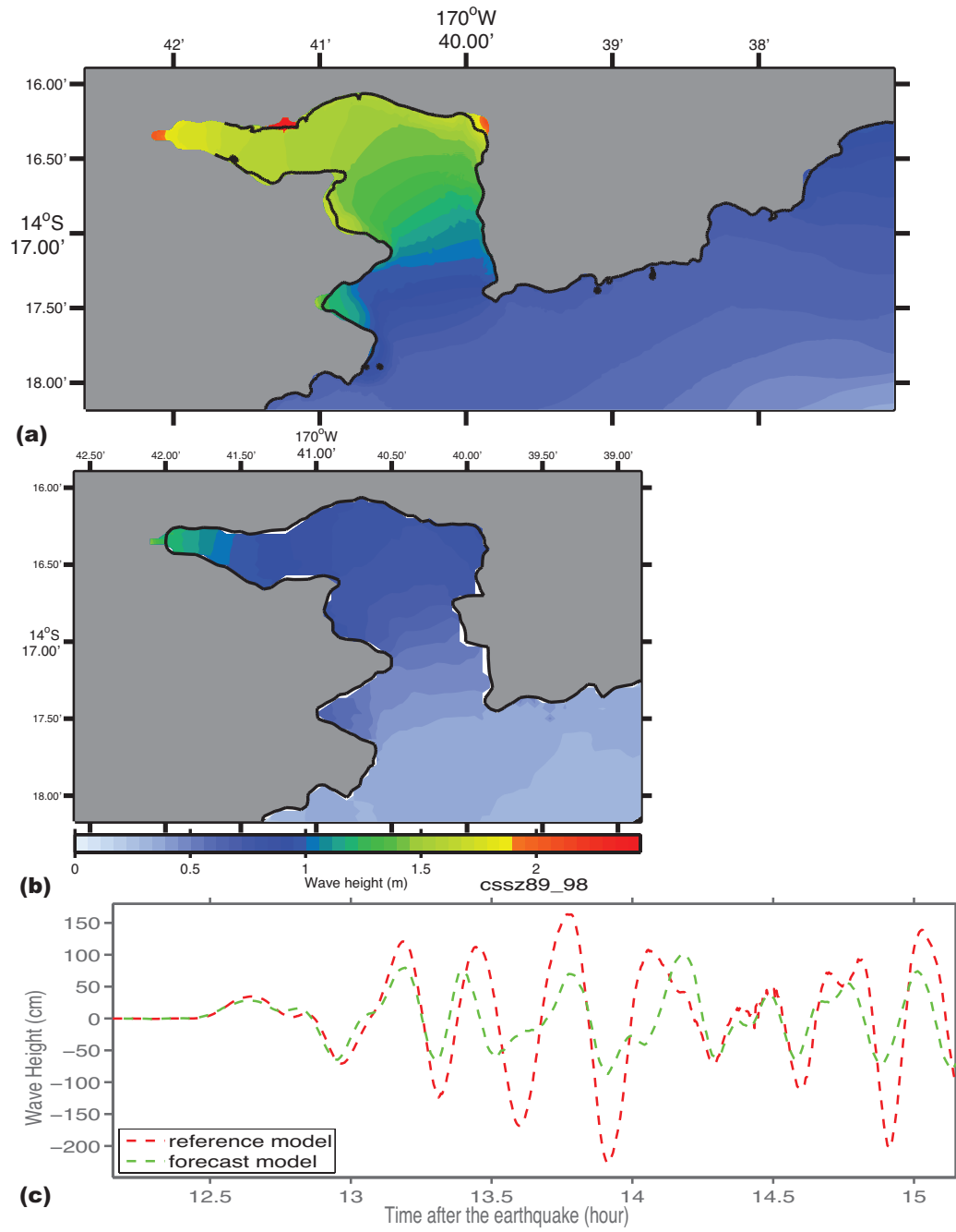
Figure 24: Magnitude 9.4 CSSZ source segment 89-98 synthetic scenario model results. (a) Maximum computed wave heights computed with reference model grids. (b) Maximum computed wave heights computed with forecast model grids. (c) Comparison of time series computed with reference model and forecast model grids at the Pago Pago tide gauge.
