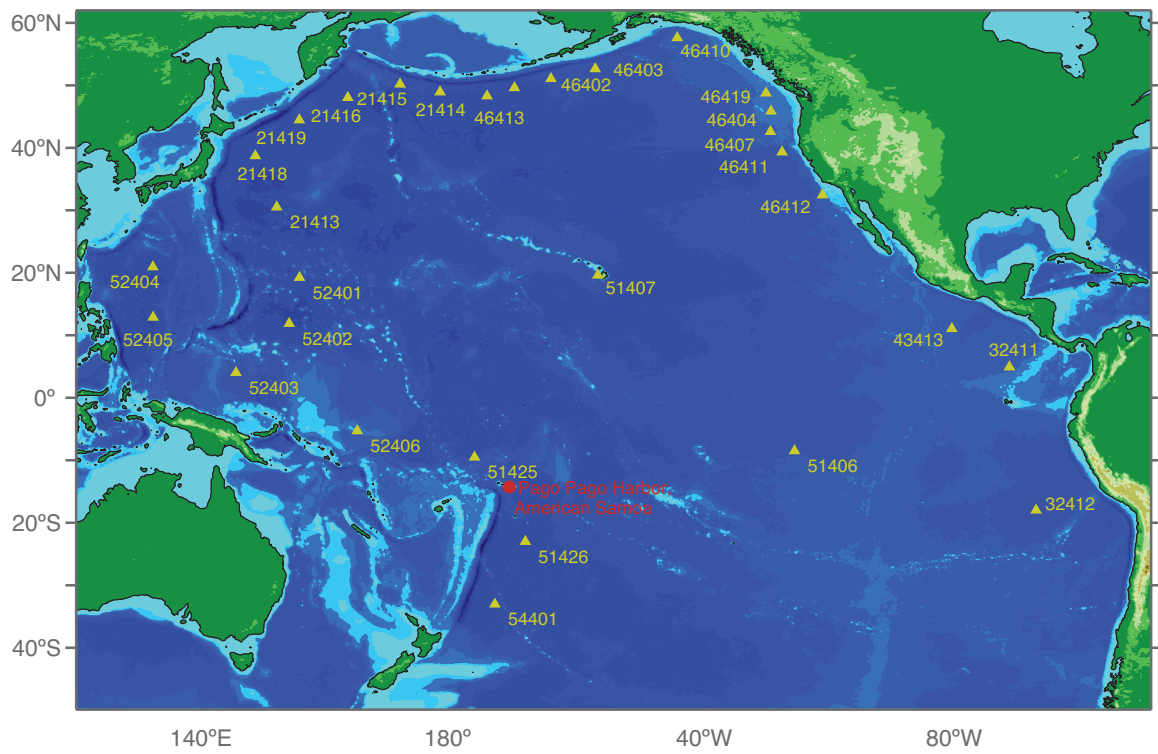
Figure 1: Pacific Ocean network of tsunameters.
