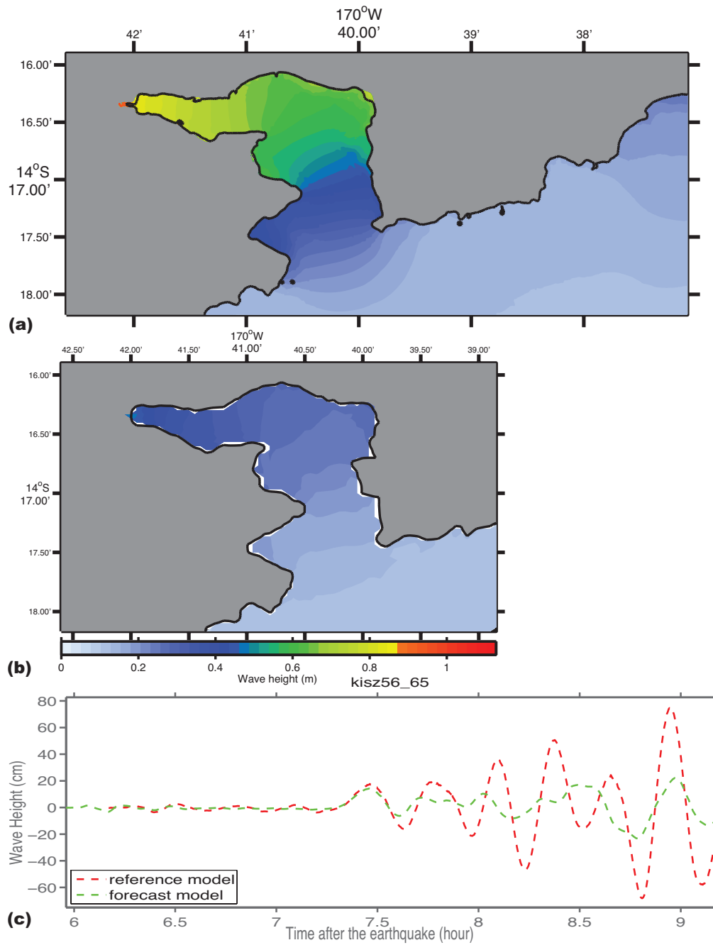
Figure 30: Magnitude 9.4 KISZ source segment 56-65 synthetic scenario model results. (a) Maximum computed wave heights computed with reference model grids. (b) Maximum computed wave heights computed with forecast model grids. (c) Comparison of time series computed with reference model and forecast model grids at the Pago Pago tide gauge.
