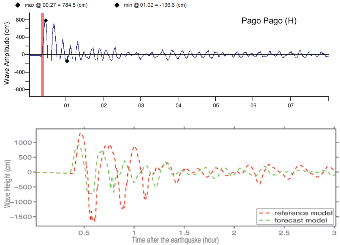
Figure C.4: Response of the Pago Pago forecast model to synthetic scenario NTSZ 30-39 ( \alpha=25 ). Maximum sea surface elevation for (a) A-grid, b) B-grid, c) C-grid. Sea surface elevation time series at the C-grid warning point (d). The lower time series plot is the result obtained during model development and is shown for comparison with test results.
