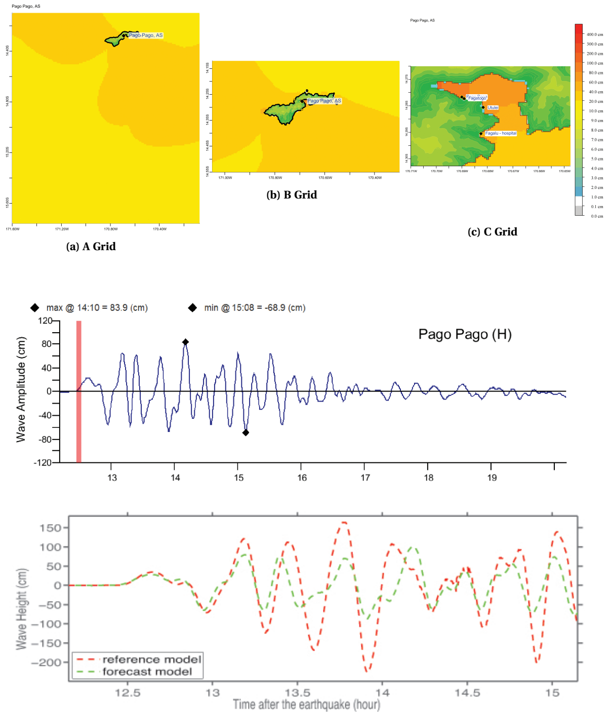
Figure C.3: Response of the Pago Pago forecast model to synthetic scenario CSSZ 89-98 ( \alpha=25 ). Maximum sea surface elevation for (a) A-grid, b) B-grid, c) C-grid. Sea surface elevation time series at the C-grid warning point (d). The lower time series plot is the result obtained during model development and is shown for comparison with test results.
