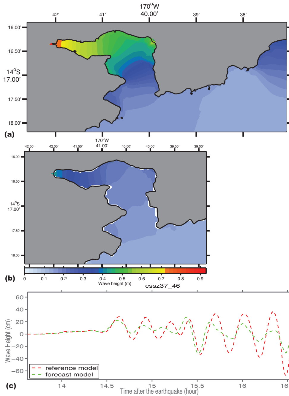
Figure 23: Magnitude 9.4 CSSZ source segment 37-46 synthetic scenario model results. (a) Maximum computed wave heights computed with reference model grids. (b) Maximum computed wave heights computed with forecast model grids. (c) Comparison of time series computed with reference model and forecast model grids at the Pago Pago tide gauge.
