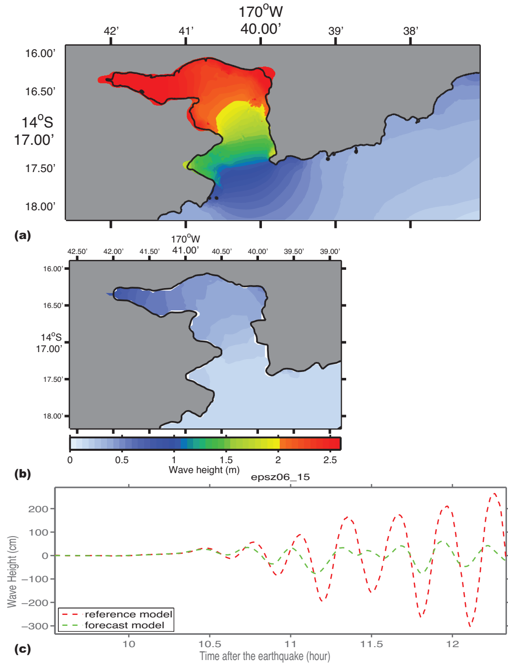
Figure 26: Magnitude 9.4 EPSZ source segment 6-15 synthetic scenario model results. (a) Maximum computed wave heights computed with reference model grids. (b) Maximum computed wave heights computed with forecast model grids. (c) Comparison of time series computed with reference model and forecast model grids at the Pago Pago tide gauge.
