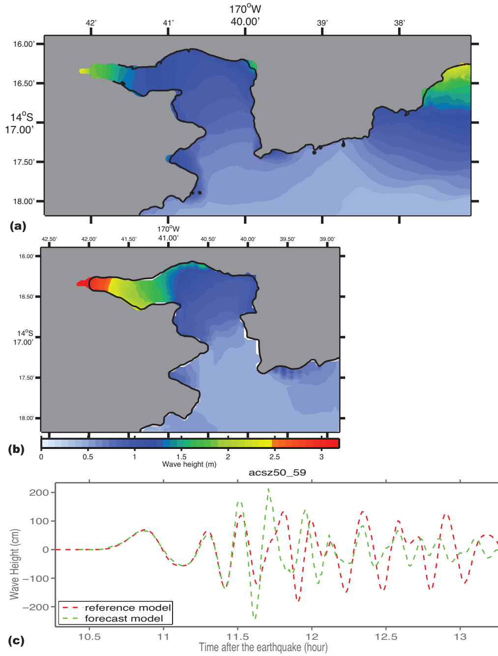
Figure 20: Magnitude 9.4 AASZ source segment 50-59 synthetic scenario model results. (a) Maximum computed wave heights computed with reference model grids. (b) Maximum computed wave heights computed with forecast model grids. (c) Comparison of time series computed with reference model and forecast model grids at the Pago Pago tide gauge.
