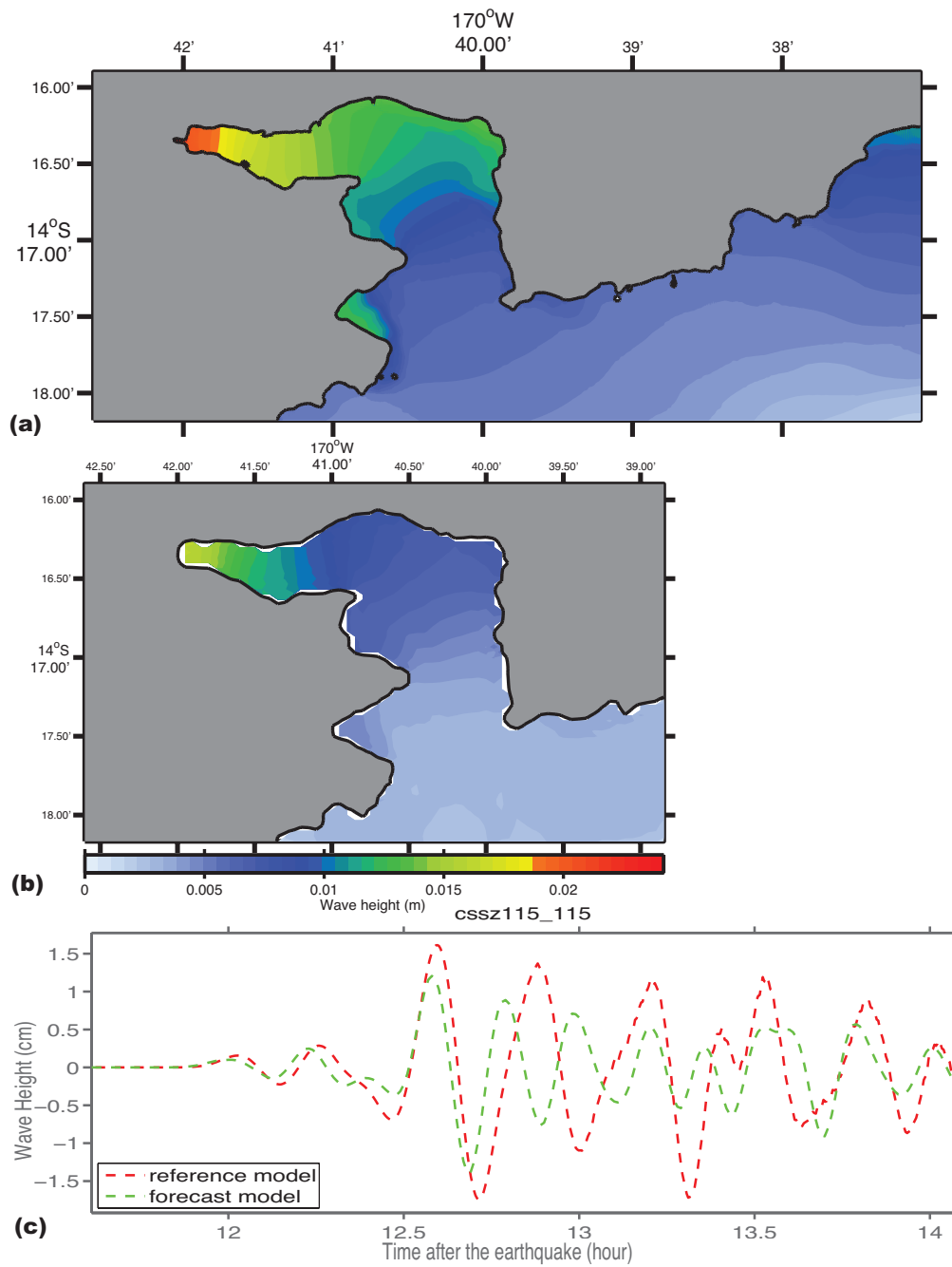
Figure 39: Magnitude 7.5 CSSZ source segment B115 synthetic scenario model results. (a) Maximum computed wave heights computed with reference model grids. (b) Maximum computed wave heights computed with forecast model grids. (c) Comparison of time series computed with reference model and forecast model grids at the Pago Pago tide gauge.
