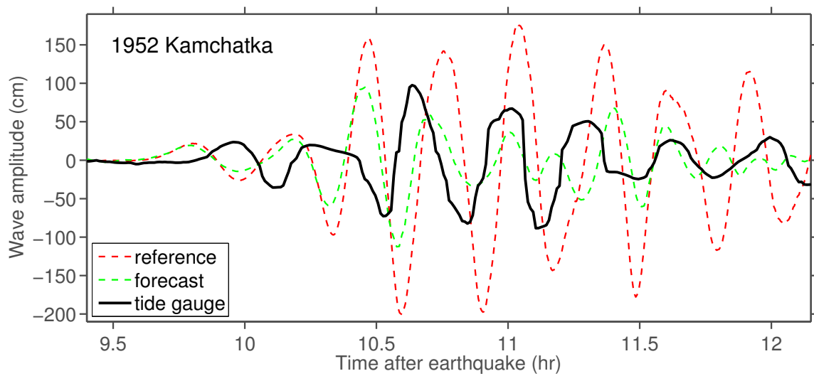
Figure 7: Pago Pago harbor tide gauge observations during the 1952 Kamchatka tsunami compared to reference and forecast model predictions.
