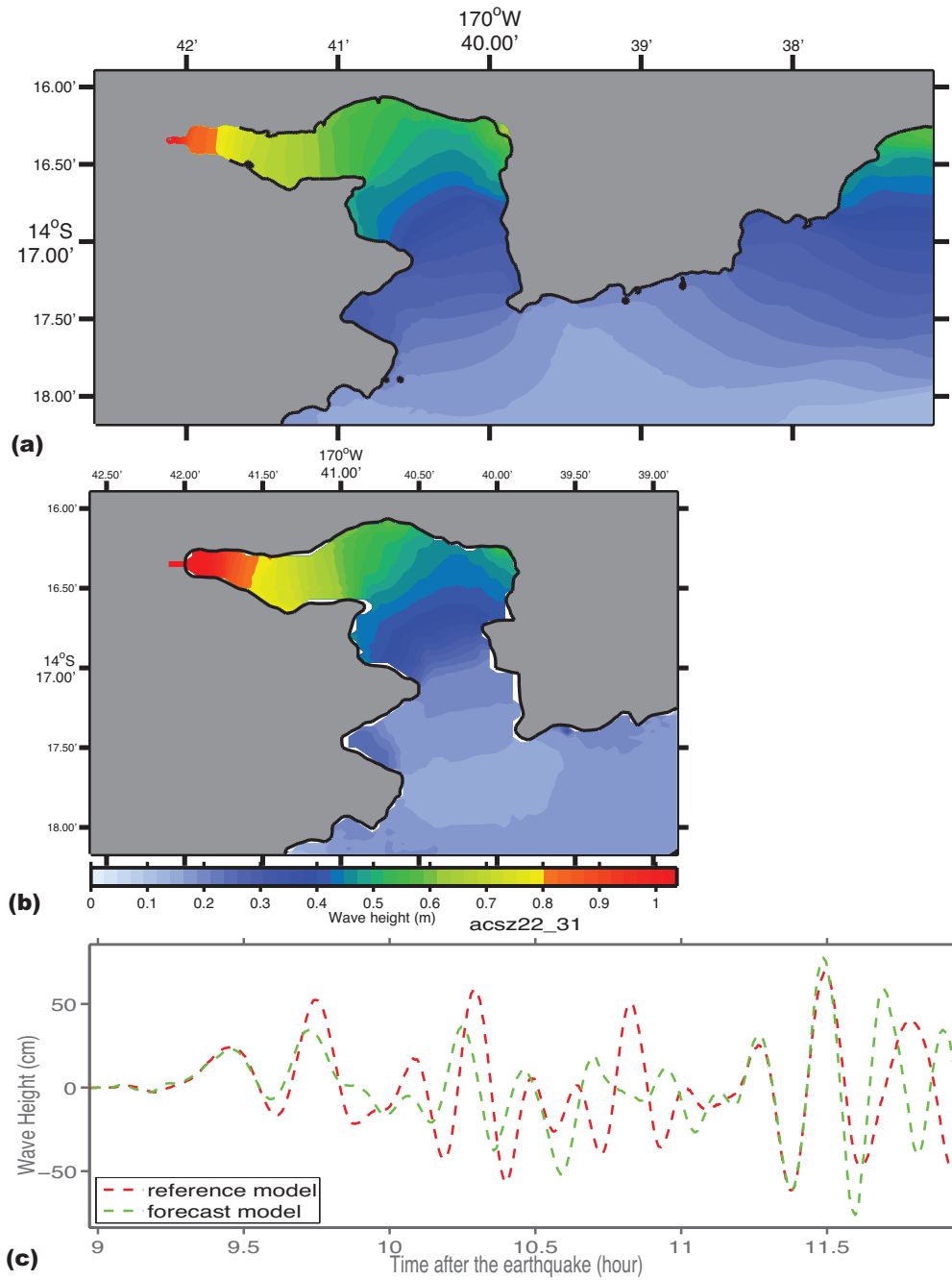
Figure 19: Magnitude 9.4 AASZ source segment 22-31 synthetic scenario model results. (a) Maximum computed wave heights computed with reference model grids. (b) Maximum computed wave heights computed with forecast model grids. (c) Comparison of time series computed with reference model and forecast model grids at the Pago Pago tide gauge.
