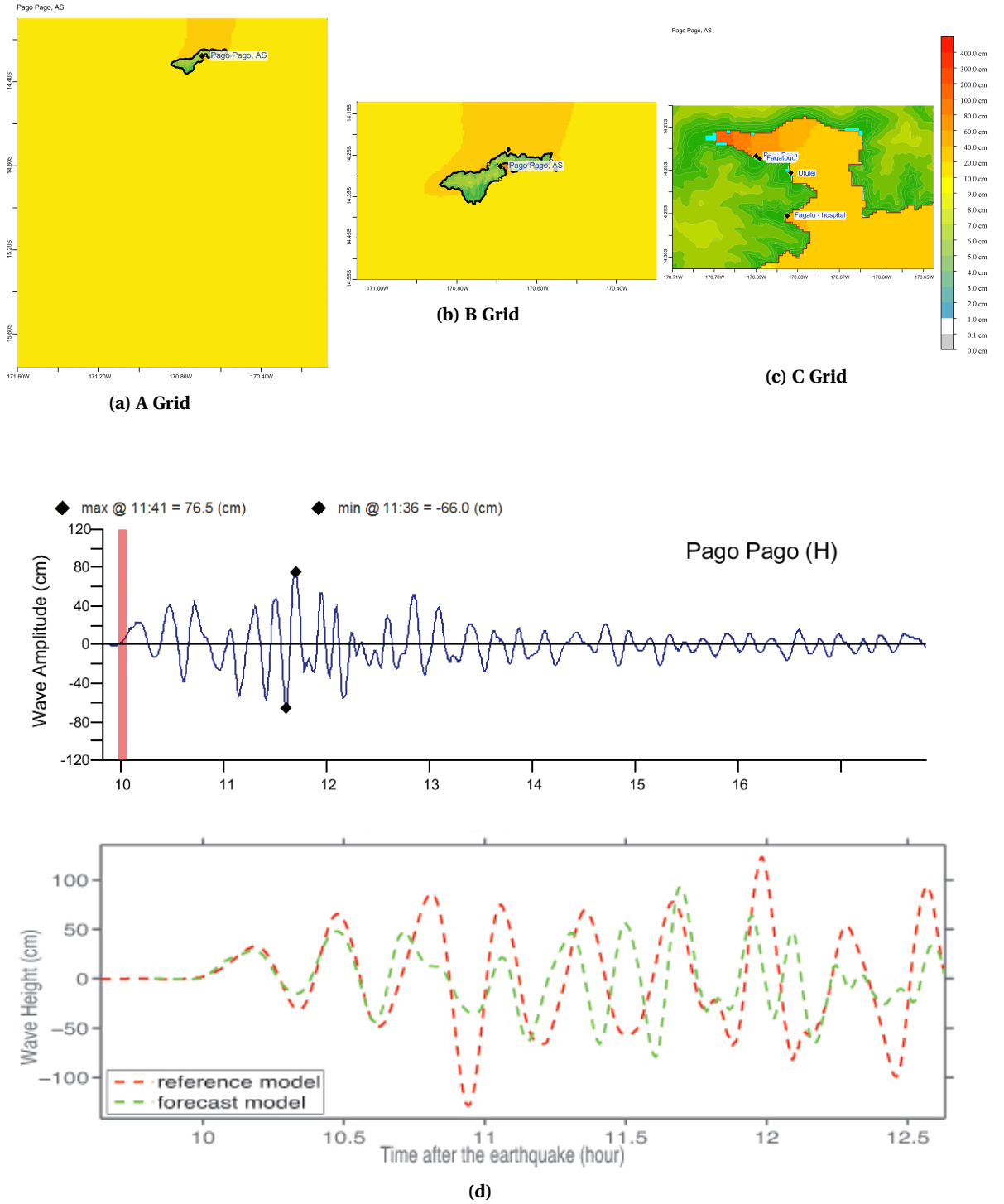
Figure C.2: Response of the Pago Pago forecast model to synthetic scenario ACSZ 56-65 ( \alpha=25 ). Maximum sea surface elevation for (a) A-grid, b) B-grid, c) C-grid. Sea surface elevation time series at the C-grid warning point (d). The lower time series plot is the result obtained during model development and is shown for comparison with test
