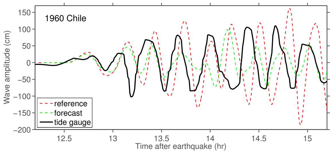
Figure 8: Pago Pago harbor tide gauge observations during the 1960 Chile tsunami compared to reference and forecast model predictions.
