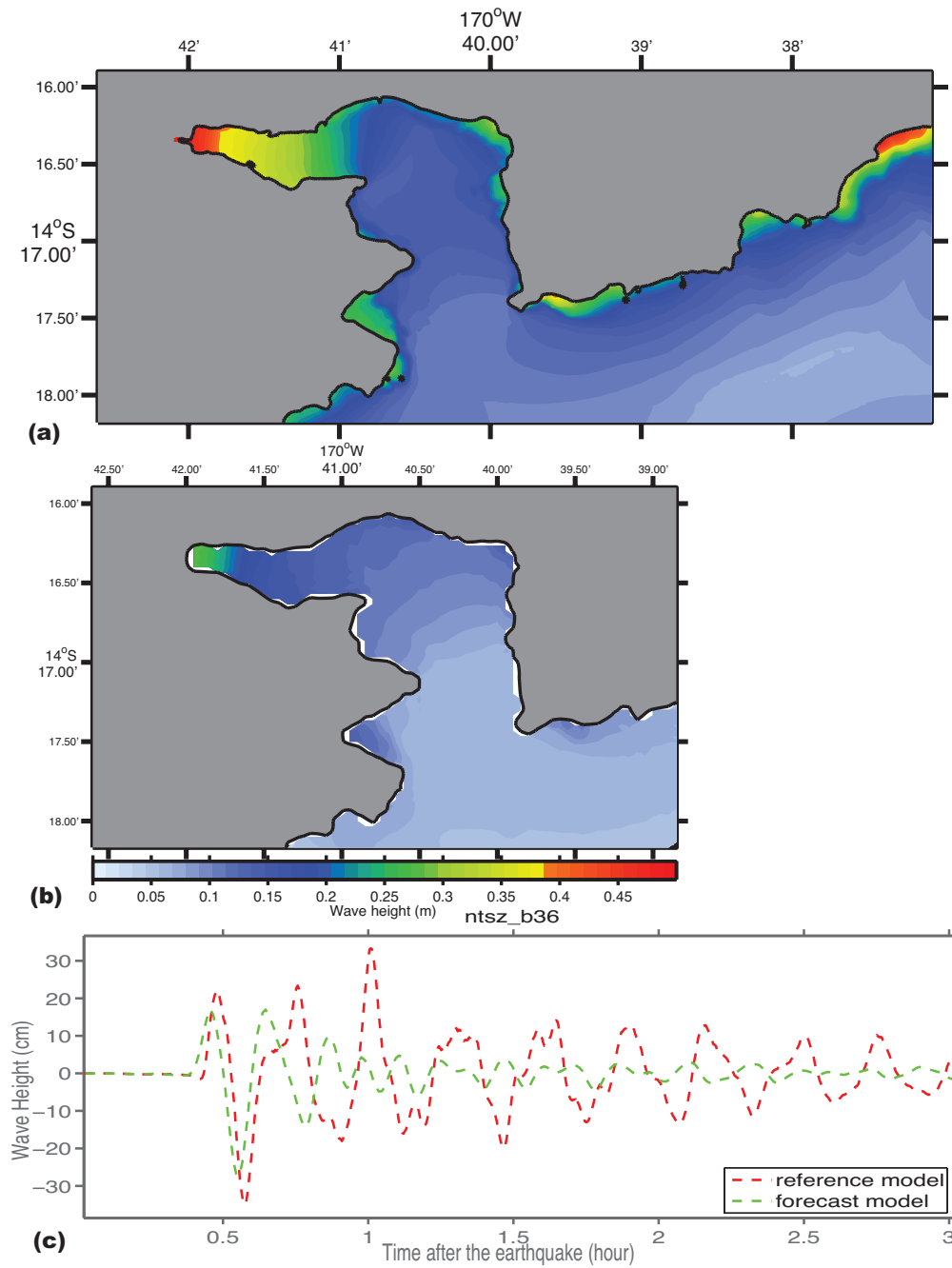
Figure 36: Magnitude 7.5 NTSZ source segment B36 synthetic scenario model results. (a) Maximum computed wave heights computed with reference model grids. (b) Maximum computed wave heights computed with forecast model grids. (c) Comparison of time series computed with reference model and forecast model grids at the Pago Pago tide gauge.
