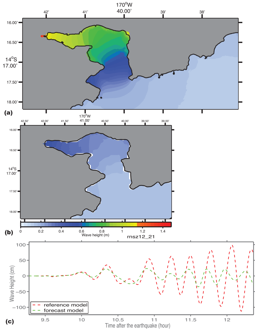
Figure 35: Magnitude 9.4 RNSZ source segment 12-21 synthetic scenario model results. (a) Maximum computed wave heights computed with reference model grids. (b) Maximum computed wave heights computed with forecast model grids. (c) Comparison of time series computed with reference model and forecast model grids at the Pago Pago tide gauge.
