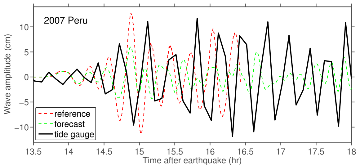
Figure 12: Pago Pago harbor tide gauge observations during the 2007 Peru tsunami compared to reference and forecast model predictions.
