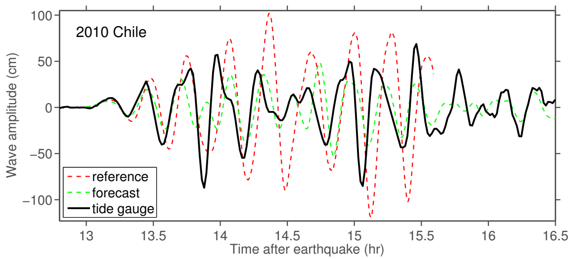
Figure 14: Pago Pago harbor tide gauge observations during the 2010 Chile tsunami compared to reference and forecast model predictions.
