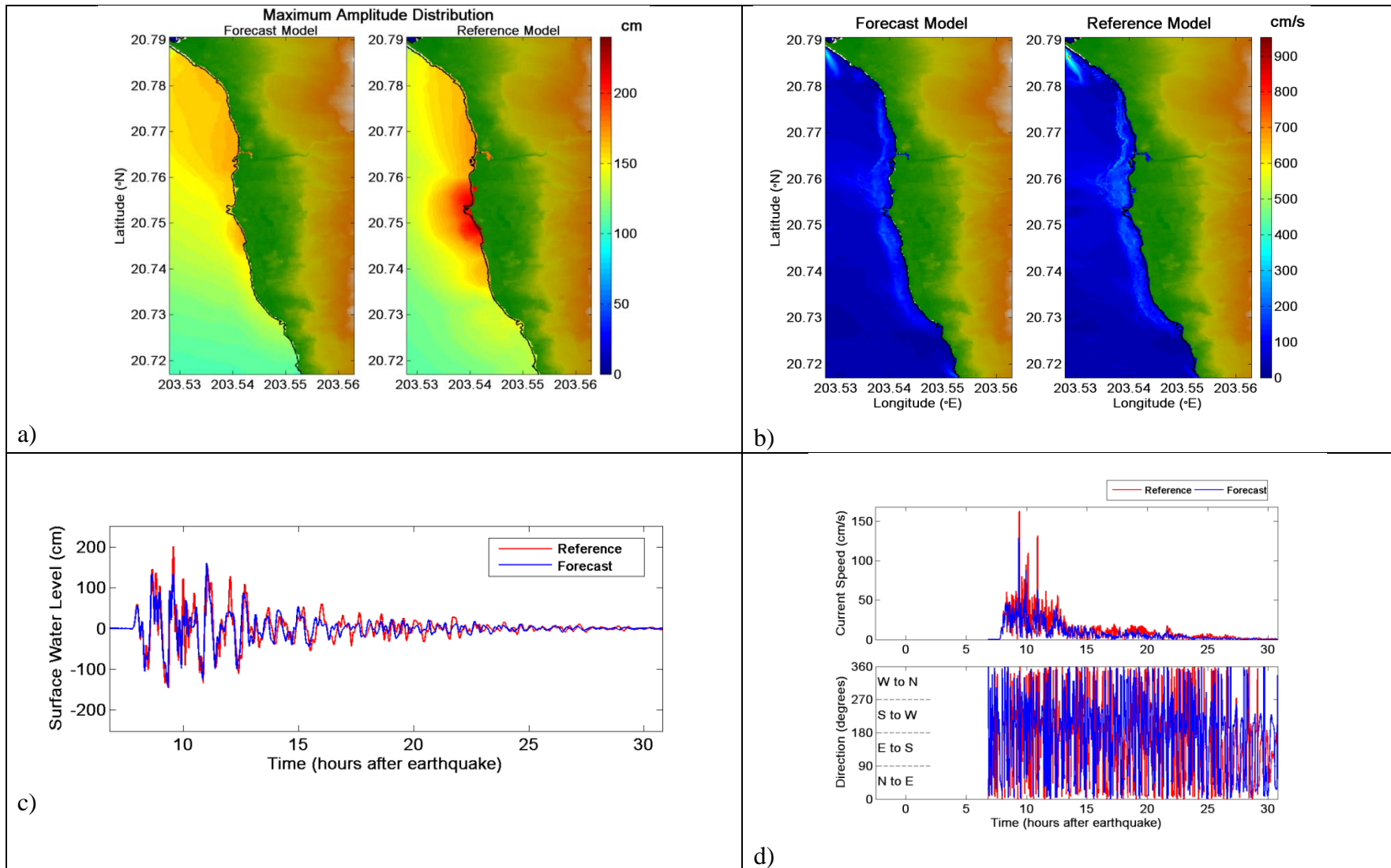
Figure 18. Comparative plot of 2011 Tohoku tsunami between forecast and reference models, a) maximum tsunami wave amplitude distribution, b) maximum current speed distribution, c) tsunami time series at the warning point, and d) current speed, and directionality at the warning point.
