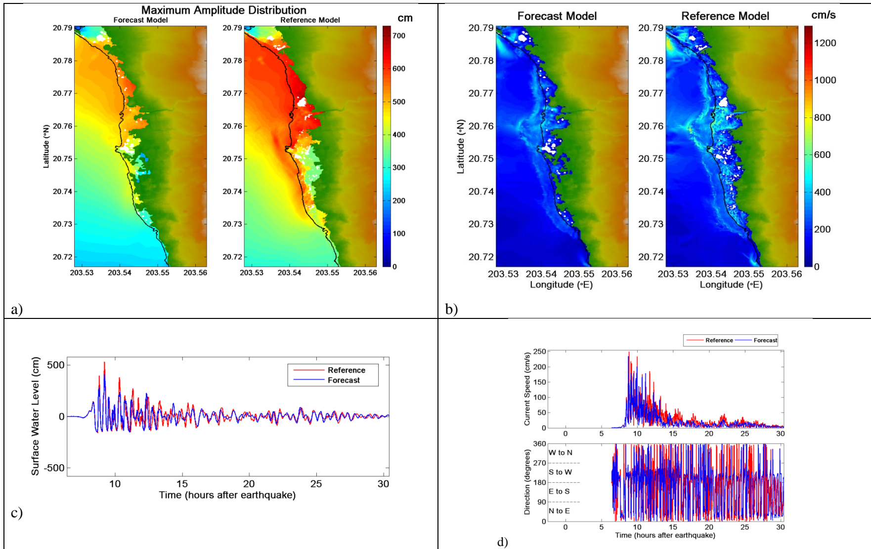
Figure 57. Comparative plot of synthetic case NVSZ 28-37 between forecast and reference models, a) maximum tsunami wave amplitude distribution, b) maximum current speed distribution, c) tsunami time series at the warning point, and d) current speed, and directionality at the warning point. White areas on land for the top figure indicate non-inundated sections.
