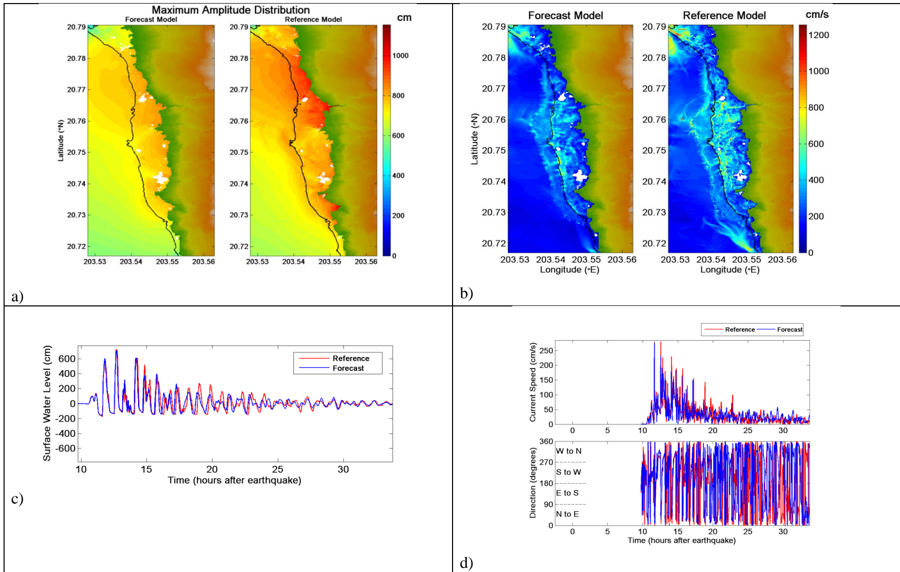
Figure 39. Comparative plot of synthetic case EPSZ 9-18 between forecast and reference models, a) maximum tsunami wave amplitude distribution, b) maximum current speed distribution, c) tsunami time series at the warning point, and d) current speed, and directionality at the warning point. White areas on land for the top figure indicate non-inundated sections.
