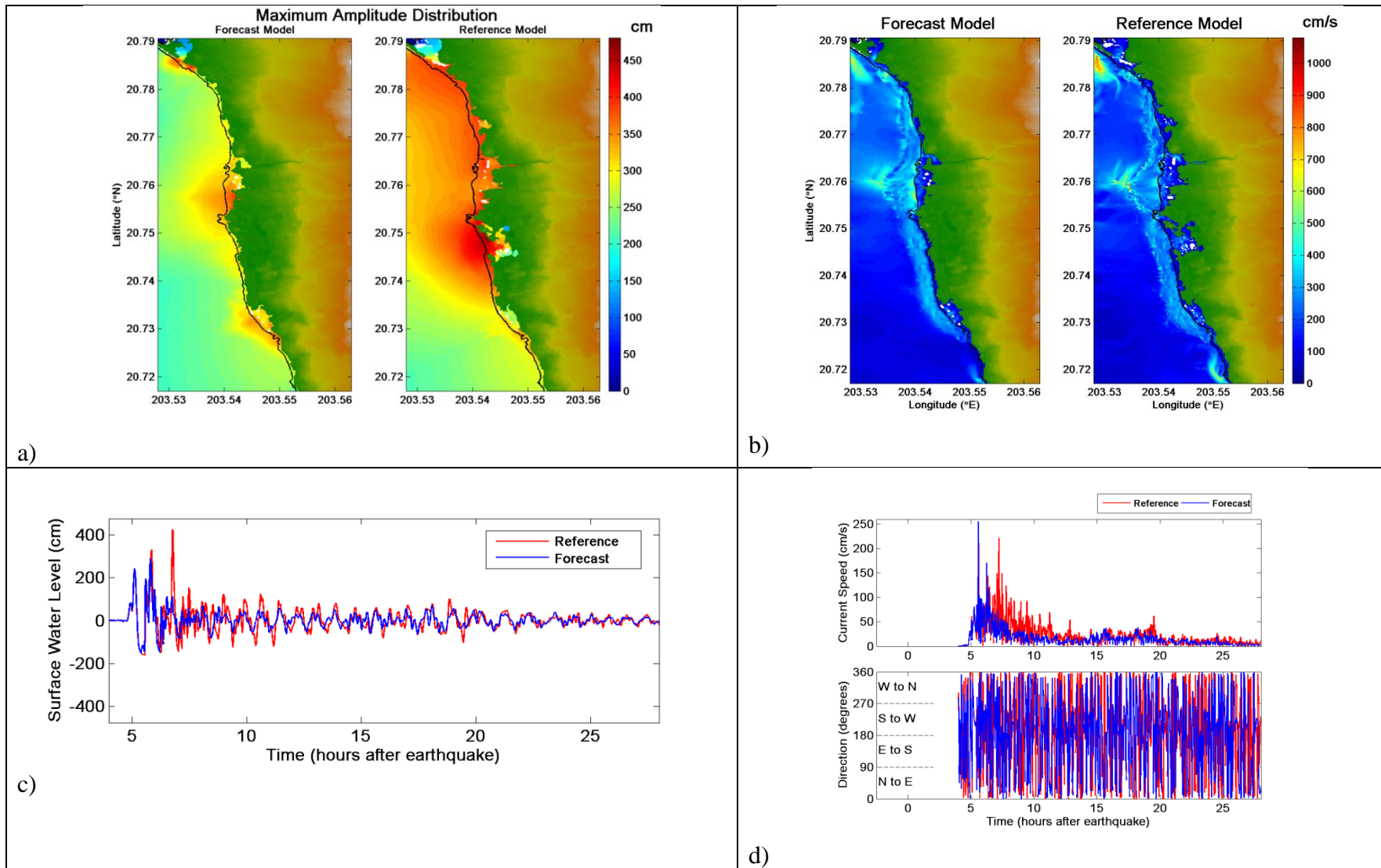
Figure 21. Comparative plot of synthetic case ACSZ 21-30 between forecast and reference models, a) maximum tsunami wave amplitude distribution, b) maximum current speed distribution, c) tsunami time series at the warning point, and d) current speed, and directionality at the warning point. White areas on land for the top figure indicate non-inundated sections.
