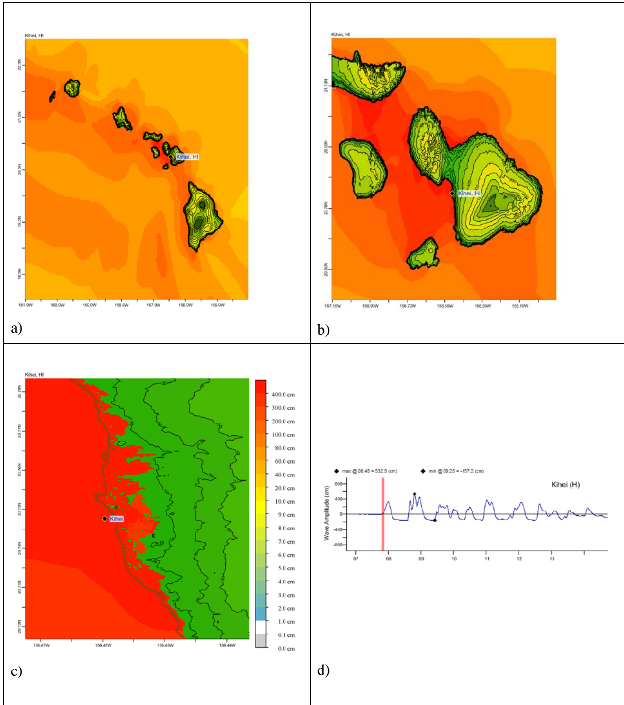
Figure C.1. Response of the Kihei forecast model to synthetic scenario KISZ 22-31 ( \alpha=30 ). Maximum sea surface elevation for (a) A-grid, b) B-grid, c) C-grid. Sea surface elevation time series at the C-grid warning point (d). This scenario was not part of the development tests.
