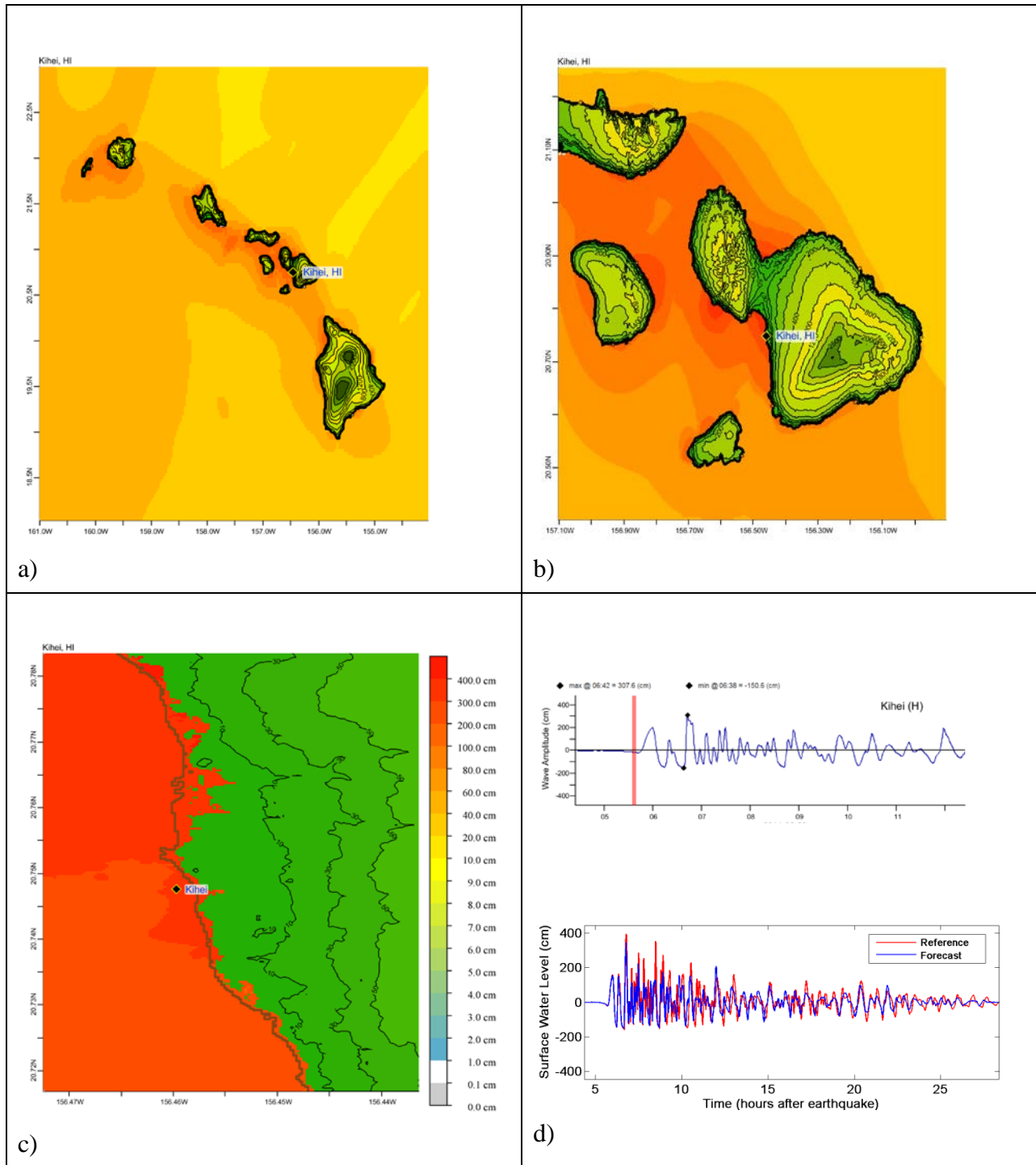
Figure C.4. Response of the Kihei forecast model to synthetic scenario NTSZ 30-39 ( \alpha=30 ). Maximum sea surface elevation for (a) A-grid, b) B-grid, c) C-grid. Sea surface elevation time series at the C-grid warning point (d). The lower time series plot is the result obtained during model development and is shown for comparison with test results.
