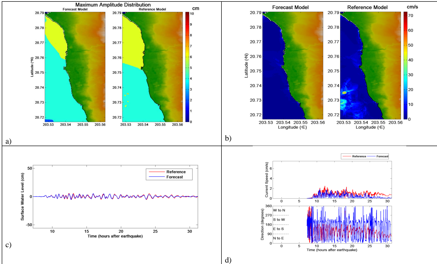
Figure 14. Comparative plot of 2007 Solomon tsunami between forecast and reference models, a) maximum tsunami wave amplitude distribution, b) maximum current speed distribution, c) tsunami time series at the warning point, and d) current speed, and directionality at the warning point.
