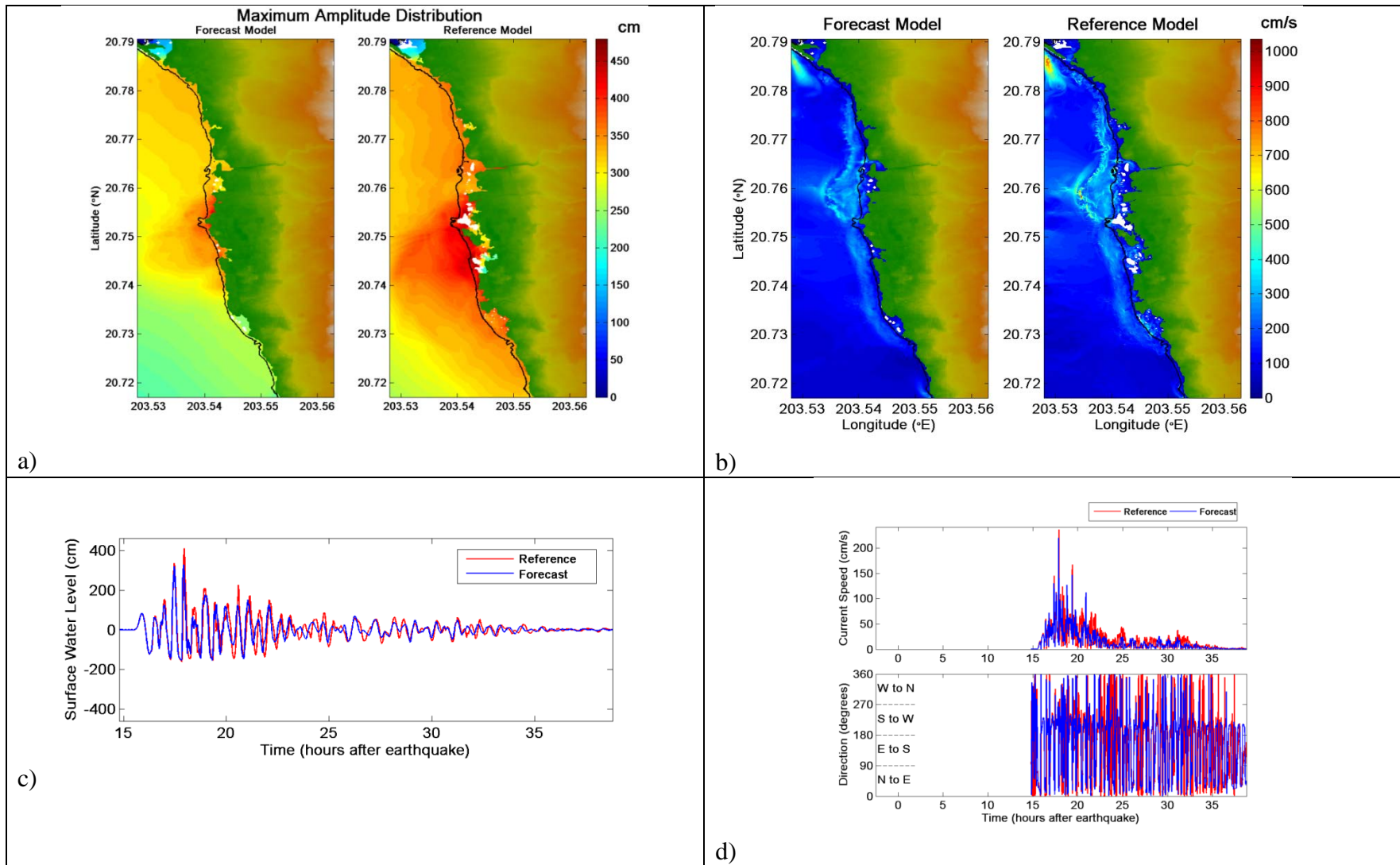
Figure 37. Comparative plot of synthetic case CSSZ 106-115 between forecast and reference models, a) maximum tsunami wave amplitude distribution, b) maximum current speed distribution, c) tsunami time series at the warning point, and d) current speed, and directionality at the warning point. White areas on land for the top figure indicate non-inundated sections.
