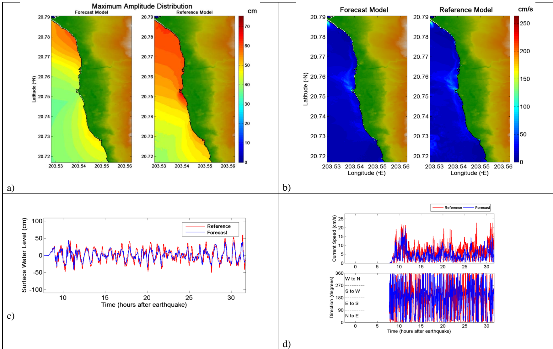
Figure 27. Comparative plot of synthetic case CSSZ 11-20 between forecast and reference models, a) maximum tsunami wave amplitude distribution, b) maximum current speed distribution, c) tsunami time series at the warning point, and d) current speed, and directionality at the warning point.
