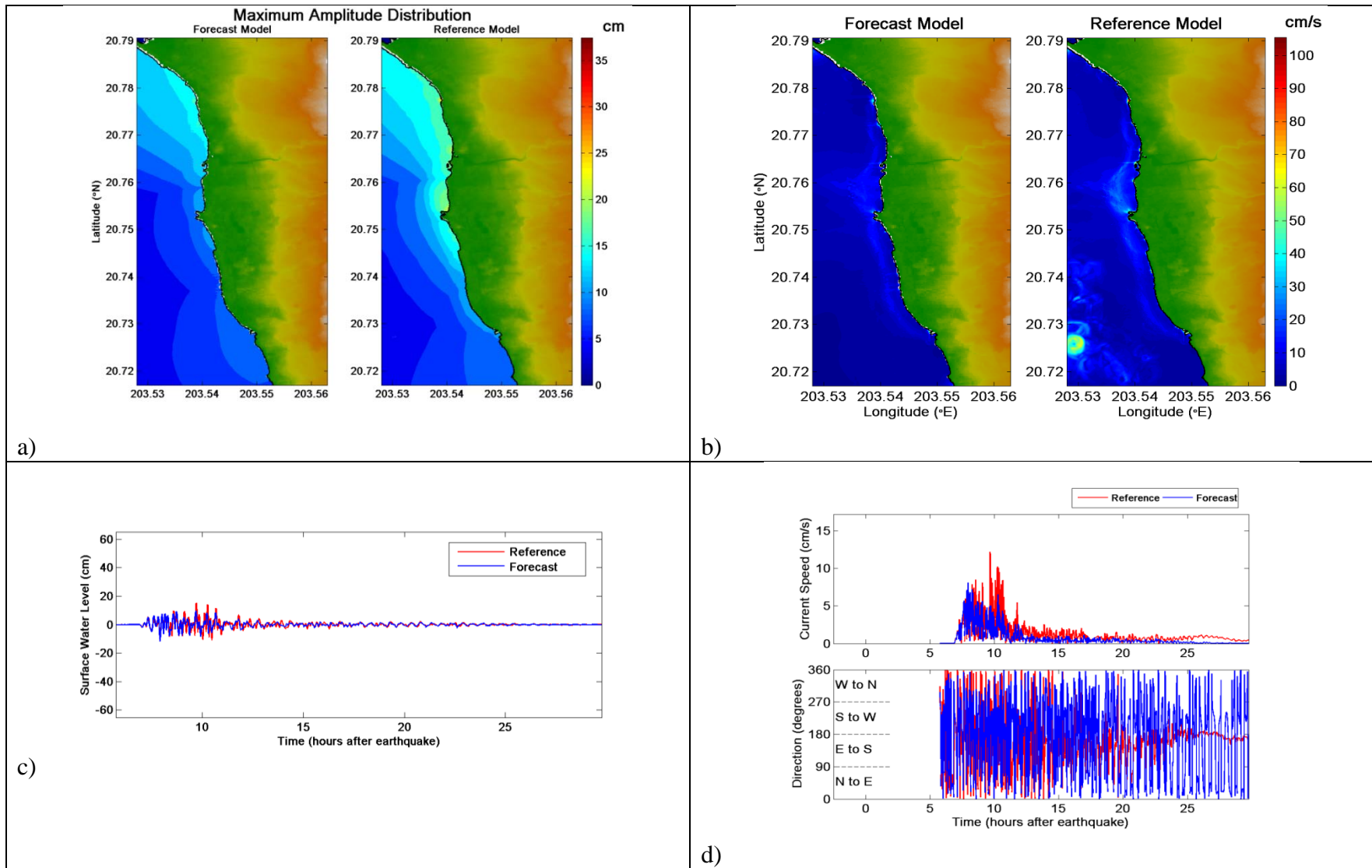
Figure 13. Comparative plot of 2007 Kuril tsunami between forecast and reference models, a) maximum tsunami wave amplitude distribution, b) maximum current speed distribution, c) tsunami time series at the warning point, and d) current speed, and directionality at the warning point.
