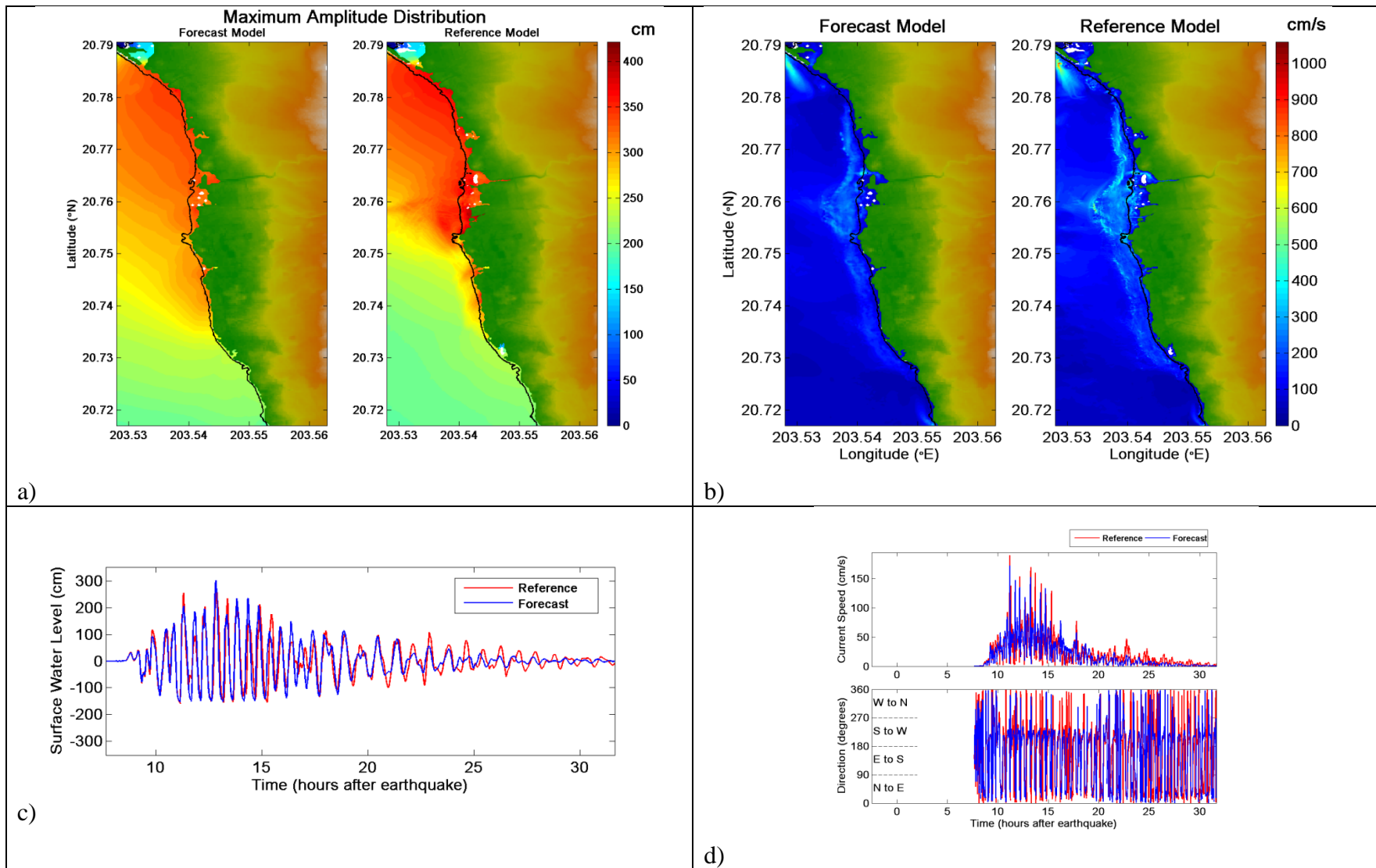
Figure 59. Comparative plot of synthetic case RNSZ 13-22 between forecast and reference models, a) maximum tsunami wave amplitude distribution, b) maximum current speed distribution, c) tsunami time series at the warning point, and d) current speed, and directionality at the warning point. White areas on land for the top figure indicate non-inundated sections.
