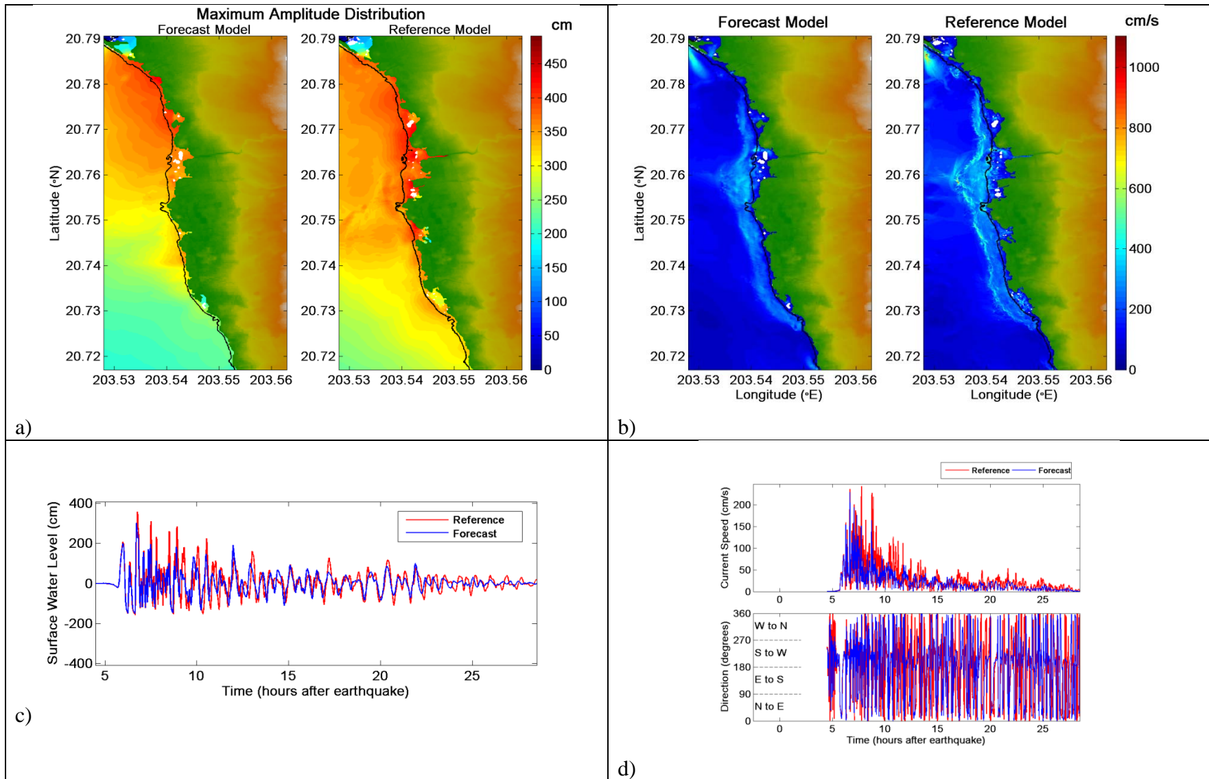
Figure 51. Comparative plot of synthetic case NTSZ 1-10 between forecast and reference models, a) maximum tsunami wave amplitude distribution, b) maximum current speed distribution, c) tsunami time series at the warning point, and d) current speed, and directionality at the warning point. White areas on land for the top figure indicate non-inundated sections.
