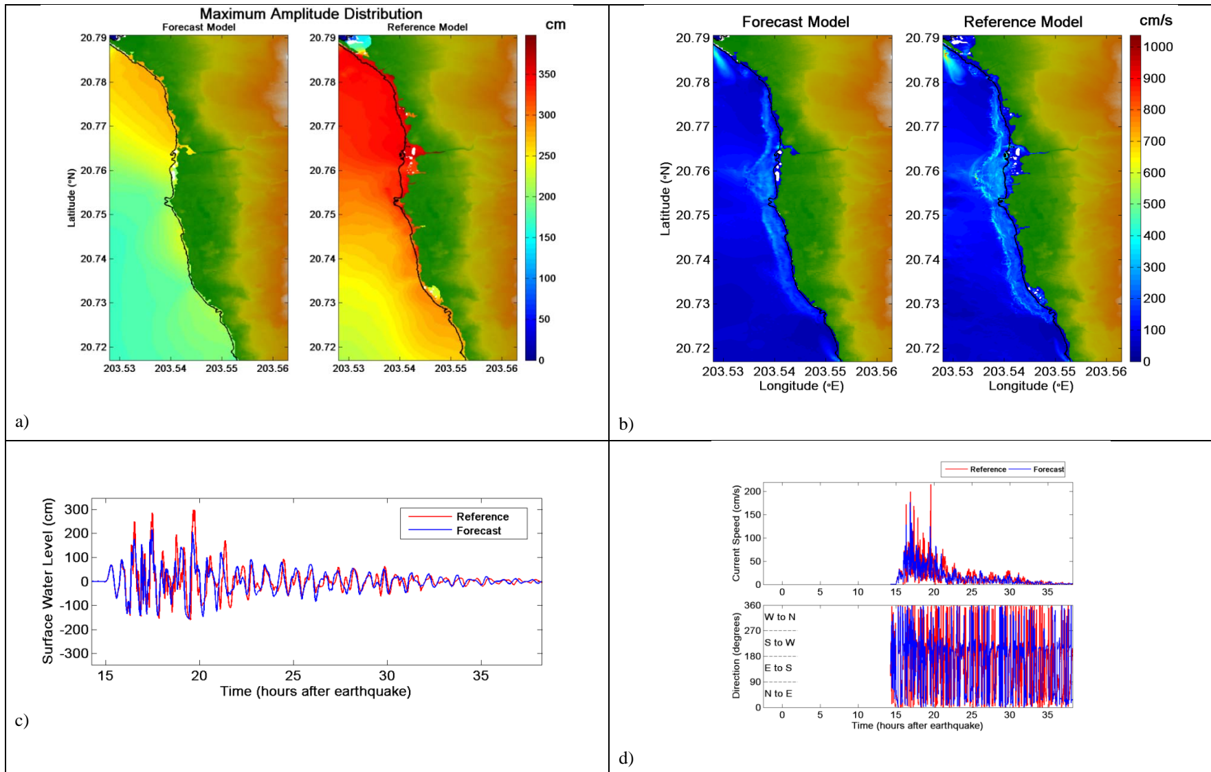
Figure 35. Comparative plot of synthetic case CSSZ 91-100 between forecast and reference models, a) maximum tsunami wave amplitude distribution, b) maximum current speed distribution, c) tsunami time series at the warning point, and d) current speed, and directionality at the warning point. White areas on land for the top figure indicate non-inundated sections.
