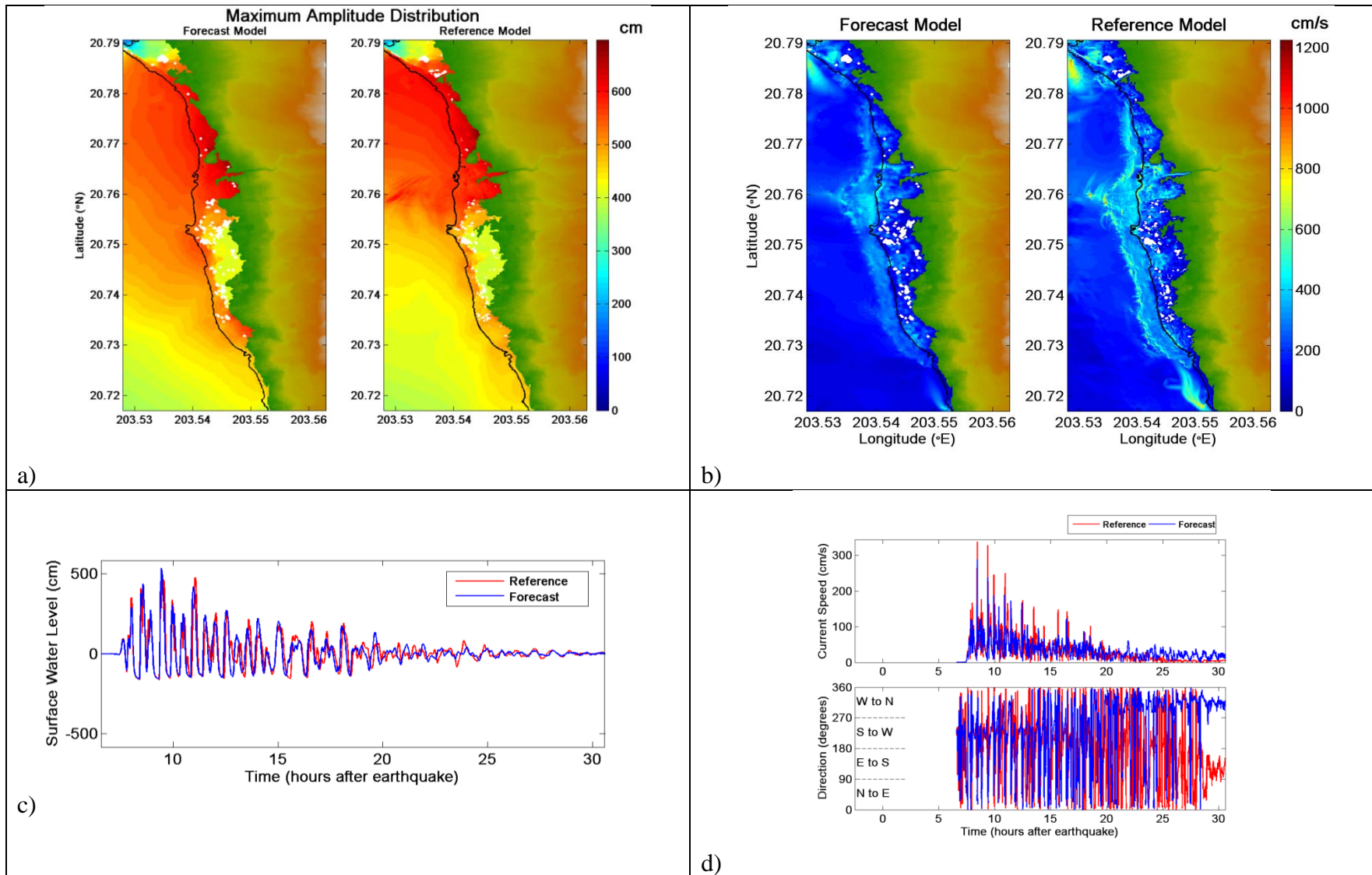
Figure 43. Comparative plot of synthetic case KISZ 42-51 between forecast and reference models, a) maximum tsunami wave amplitude distribution, b) maximum current speed distribution, c) tsunami time series at the warning point, and d) current speed, and directionality at the warning point. White areas on land for the top figure indicate non-inundated sections.
