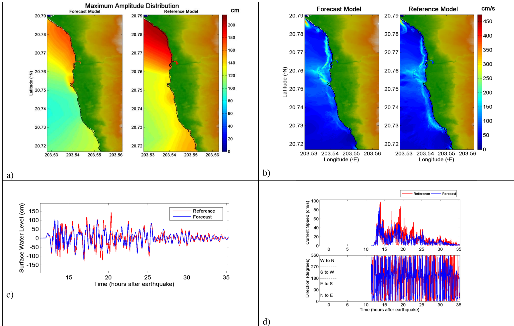
Figure 31. Comparative plot of synthetic case CSSZ 51-60 between forecast and reference models, a) maximum tsunami wave amplitude distribution, b) maximum current speed distribution, c) tsunami time series at the warning point, and d) current speed, and directionality at the warning point.
