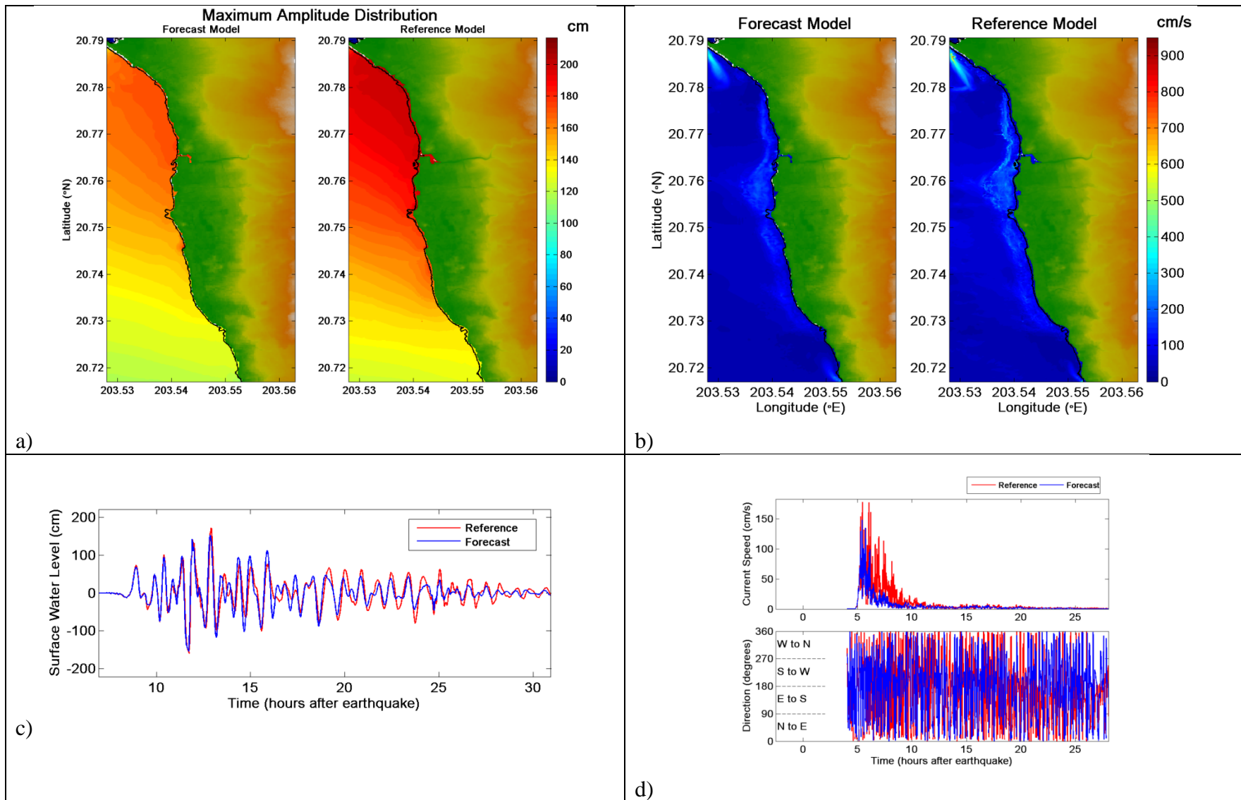
Figure 55. Comparative plot of synthetic case NVSZ 1-10 between forecast and reference models, a) maximum tsunami wave amplitude distribution, b) maximum current speed distribution, c) tsunami time series at the warning point, and d) current speed, and directionality at the warning point.
