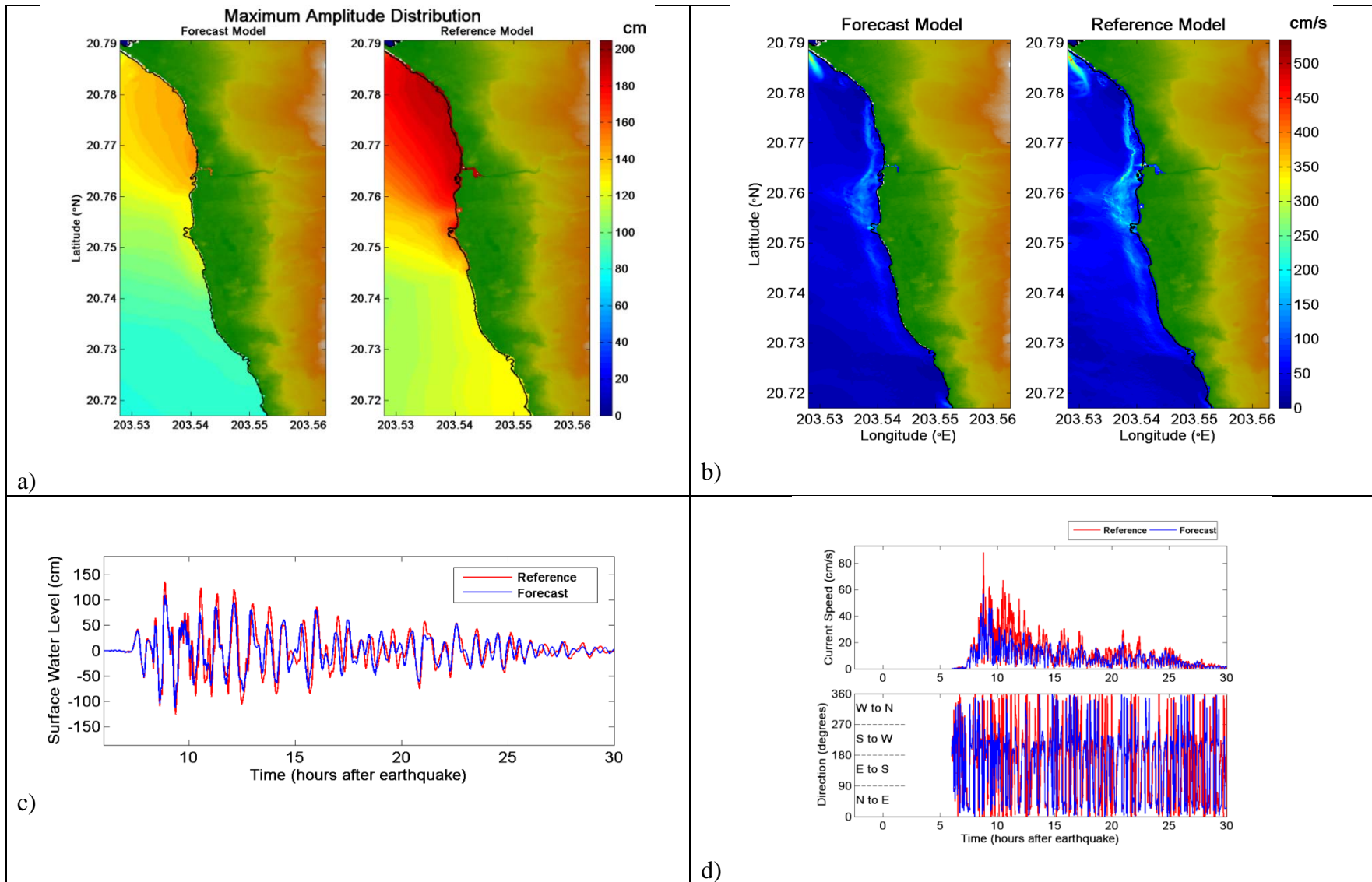
Figure 56. Comparative plot of synthetic case NVSZ 11-20 between forecast and reference models, a) maximum tsunami wave amplitude distribution, b) maximum current speed distribution, c) tsunami time series at the warning point, and d) current speed, and directionality at the warning point.
