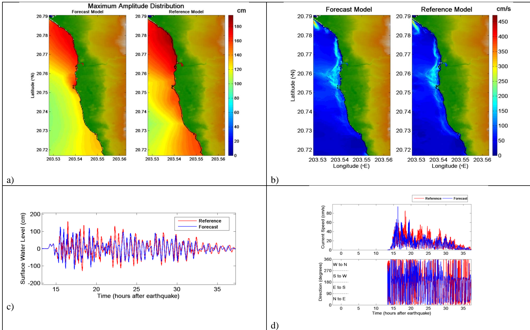
Figure 33. Comparative plot of synthetic case CSSZ 71-80 between forecast and reference models, a) maximum tsunami wave amplitude distribution, b) maximum current speed distribution, c) tsunami time series at the warning point, and d) current speed, and directionality at the warning point.
