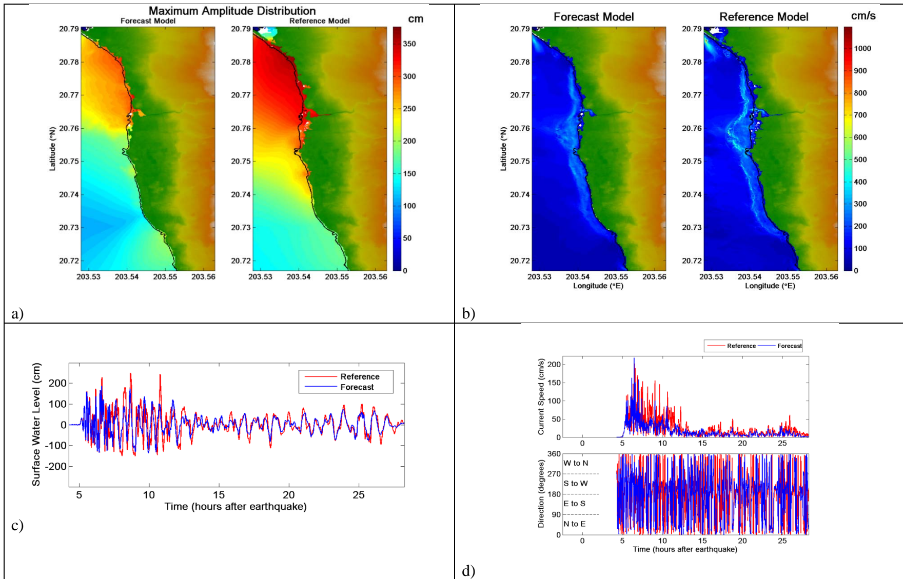
Figure 25. Comparative plot of synthetic case ACSZ 56-65 between forecast and reference models, a) maximum tsunami wave amplitude distribution, b) maximum current speed distribution, c) tsunami time series at the warning point, and d) current speed, and directionality at the warning point. White areas on land for the top figure indicate non-inundated sections.
