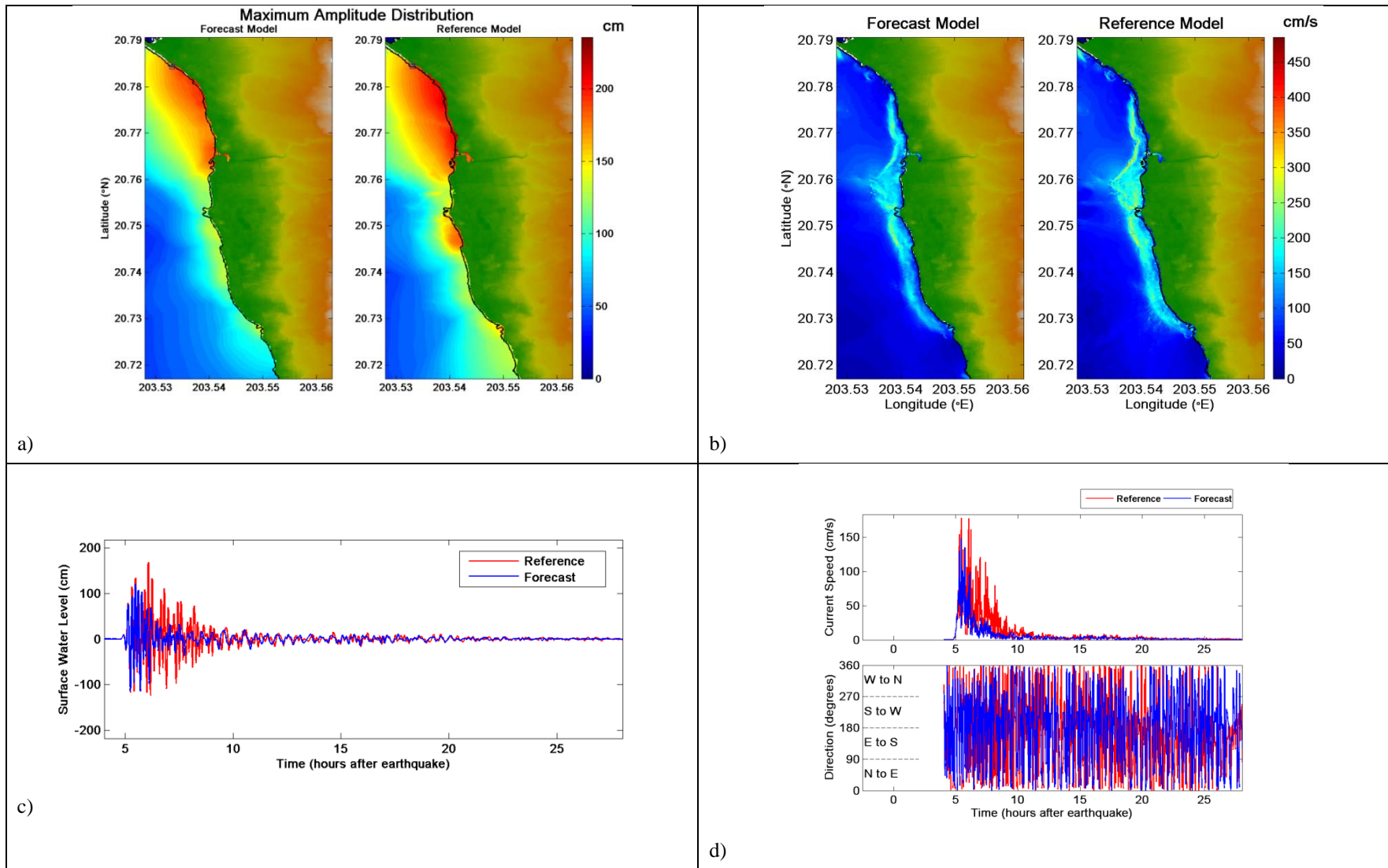
Figure 6. Comparative plot of 1946 Unimak tsunami between forecast and reference models, a) maximum tsunami wave amplitude distribution, b) maximum current speed distribution, c) tsunami time series at the warning point, and d) current speed, and directionality at the warning point.
