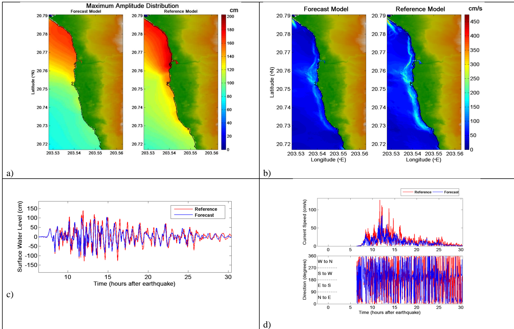
Figure 52. Comparative plot of synthetic case NTSZ 11-20 between forecast and reference models, a) maximum tsunami wave amplitude distribution, b) maximum current speed distribution, c) tsunami time series at the warning point, and d) current speed, and directionality at the warning point.
