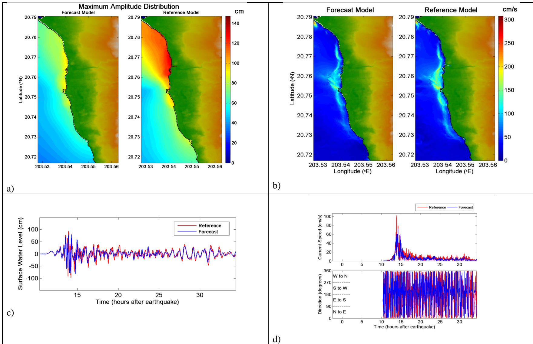
Figure 29. Comparative plot of synthetic case CSSZ 31-40 between forecast and reference models, a) maximum tsunami wave amplitude distribution, b) maximum current speed distribution, c) tsunami time series at the warning point, and d) current speed, and directionality at the warning point.
