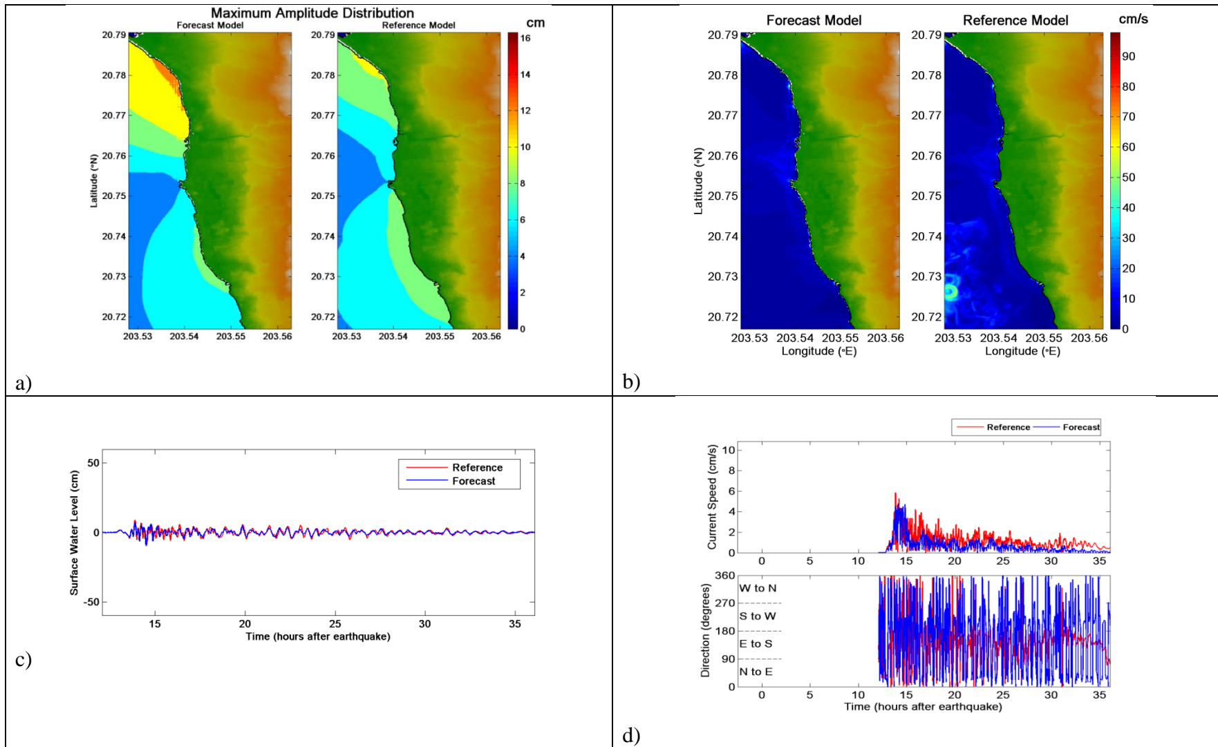
Figure 15. Comparative plot of 2007 Peru tsunami between forecast and reference models, a) maximum tsunami wave amplitude distribution, b) maximum current speed distribution, c) tsunami time series at the warning point, and d) current speed, and directionality at the warning point.
