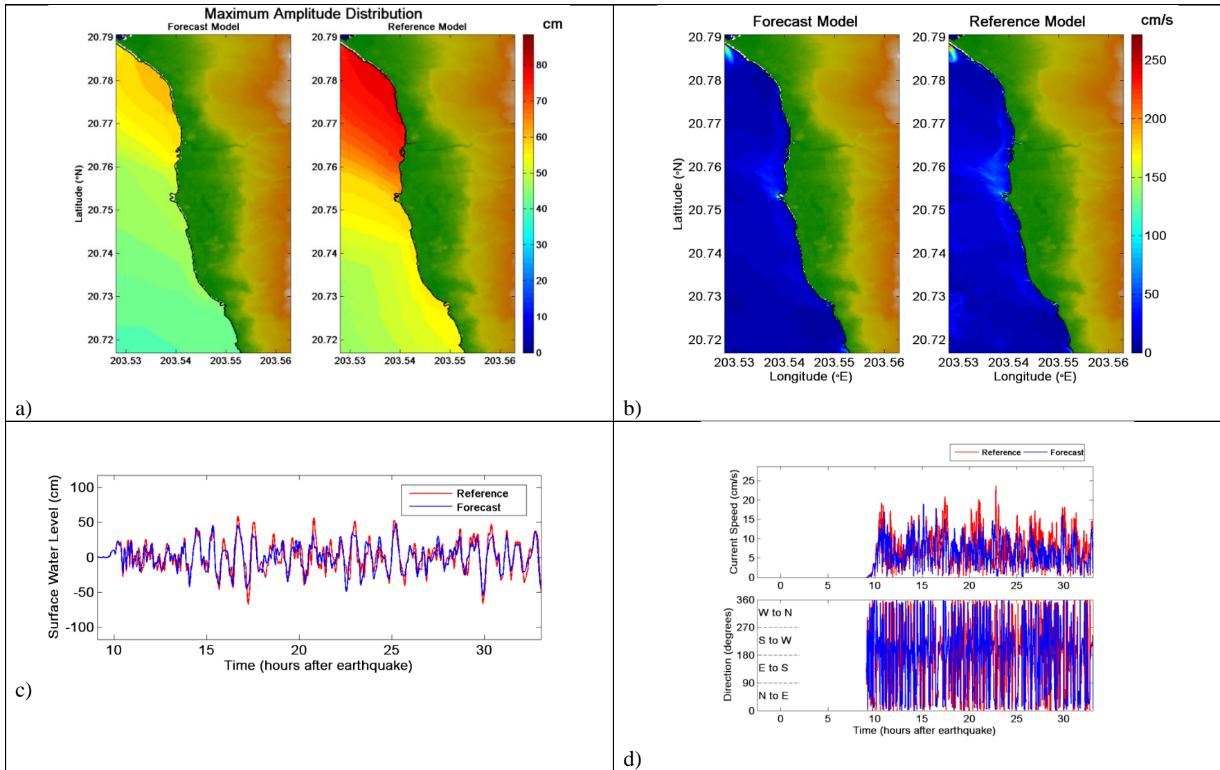
Figure 28. Comparative plot of synthetic case CSSZ 21-30 between forecast and reference models, a) maximum tsunami wave amplitude distribution, b) maximum current speed distribution, c) tsunami time series at the warning point, and d) current speed, and directionality at the warning point.
