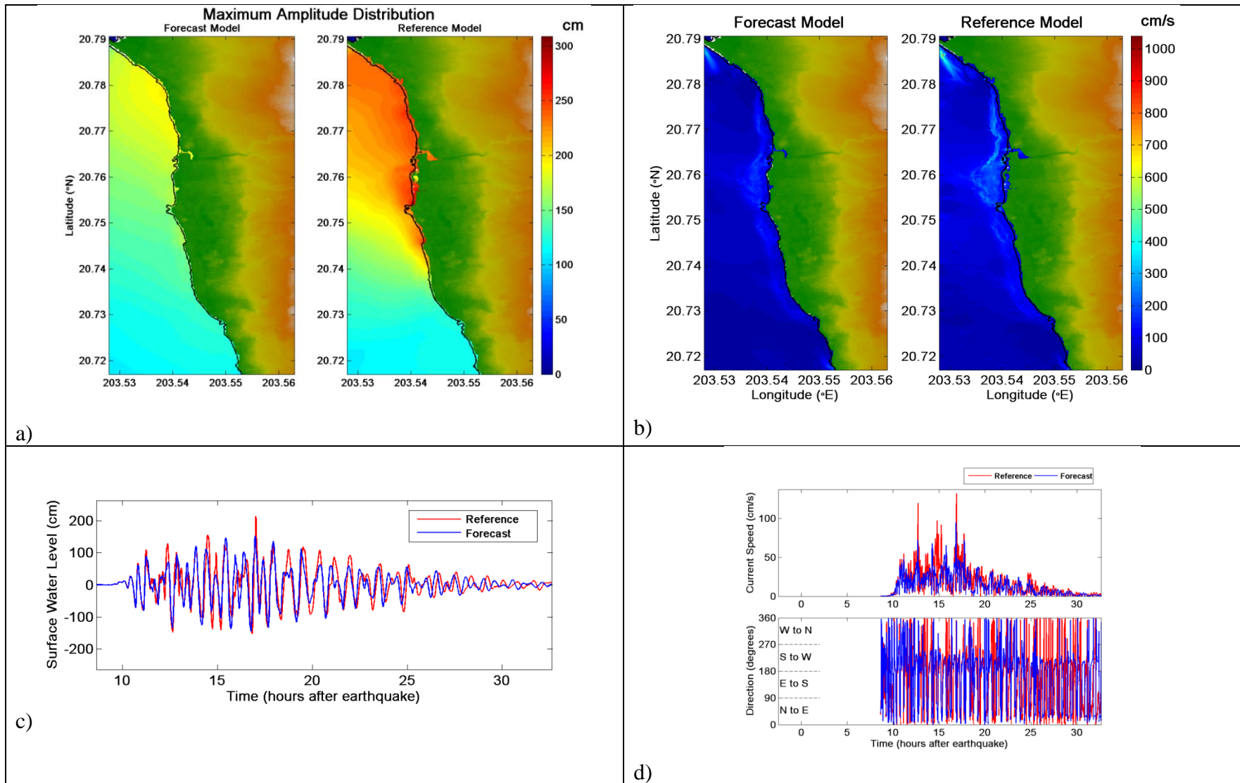
Figure 58. Comparative plot of synthetic case RNSZ 1-10 between forecast and reference models, a) maximum tsunami wave amplitude distribution, b) maximum current speed distribution, c) tsunami time series at the warning point, and d) current speed, and directionality at the warning point.
