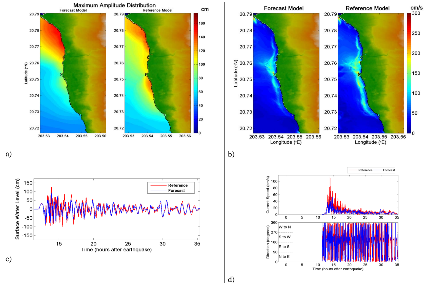
Figure 30. Comparative plot of synthetic case CSSZ 41-50 between forecast and reference models, a) maximum tsunami wave amplitude distribution, b) maximum current speed distribution, c) tsunami time series at the warning point, and d) current speed, and directionality at the warning point.
