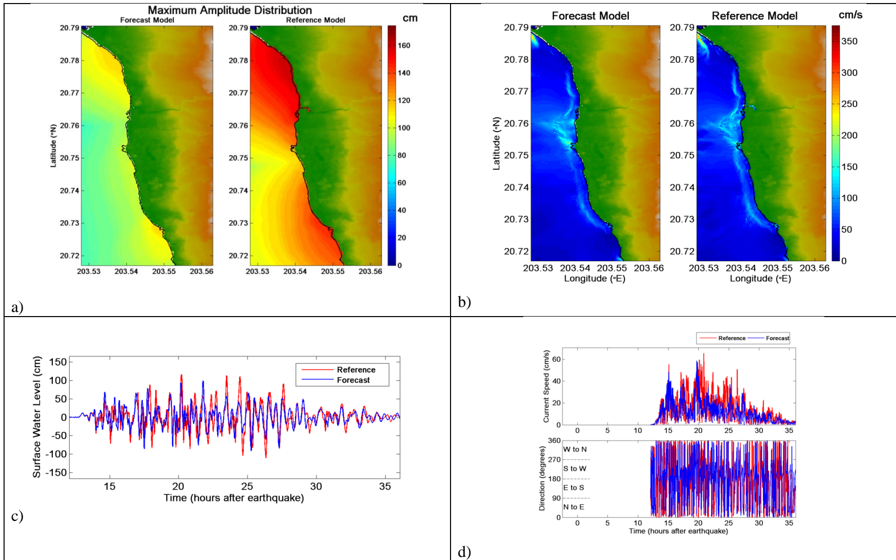
Figure 32. Comparative plot of synthetic case CSSZ 61-70 between forecast and reference models, a) maximum tsunami wave amplitude distribution, b) maximum current speed distribution, c) tsunami time series at the warning point, and d) current speed, and directionality at the warning point.
