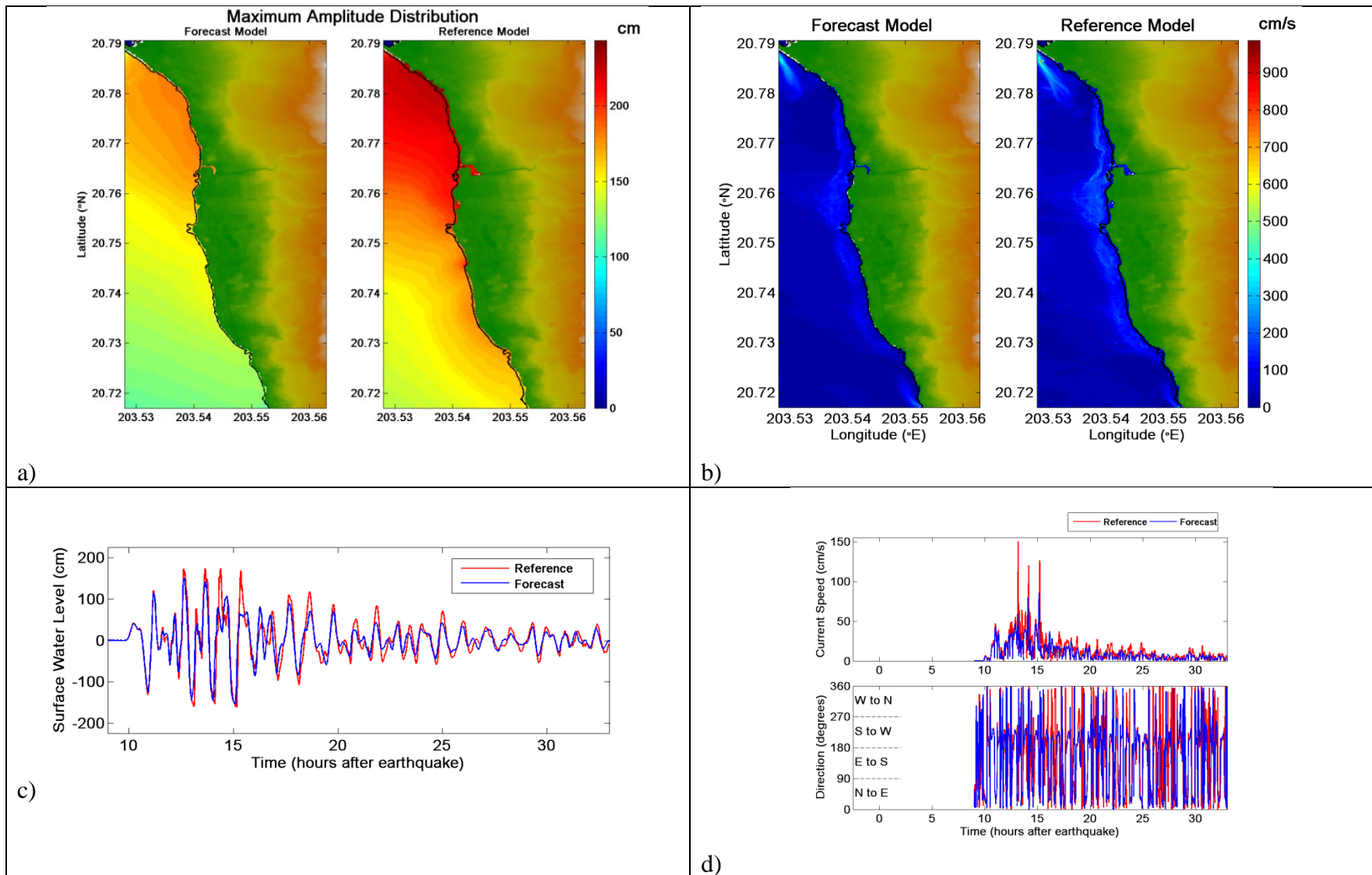
Figure 50. Comparative plot of synthetic case NGSZ 6-15 between forecast and reference models, a) maximum tsunami wave amplitude distribution, b) maximum current speed distribution, c) tsunami time series at the warning point, and d) current speed, and directionality at the warning point.
