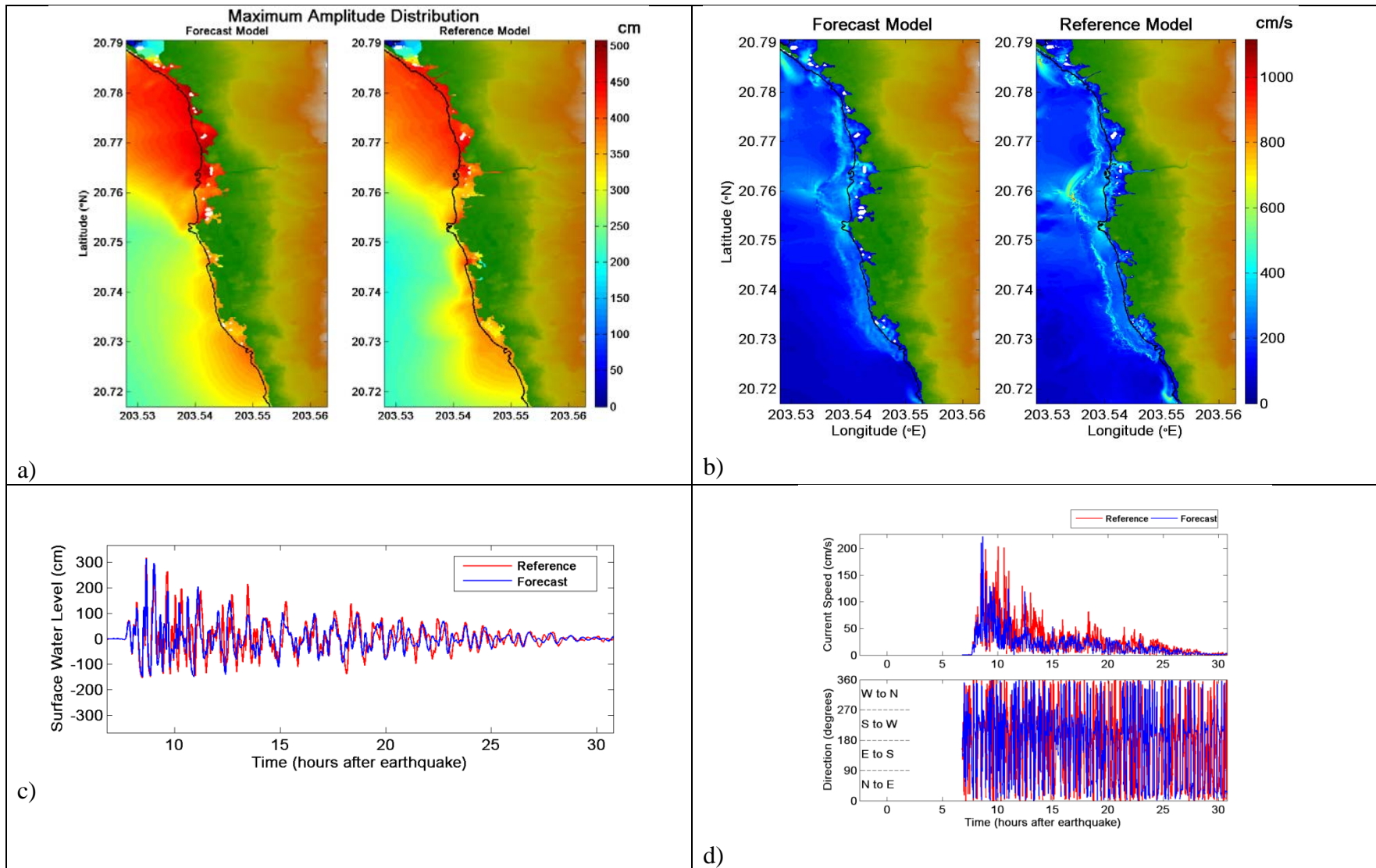
Figure 42. Comparative plot of for synthetic case KISZ 32-41 between forecast and reference models, a) maximum tsunami wave amplitude distribution, b) maximum current speed distribution, c) tsunami time series at the warning point, and d) current speed, and directionality at the warning point. White areas on land for the top figure indicate non-inundated sections.
