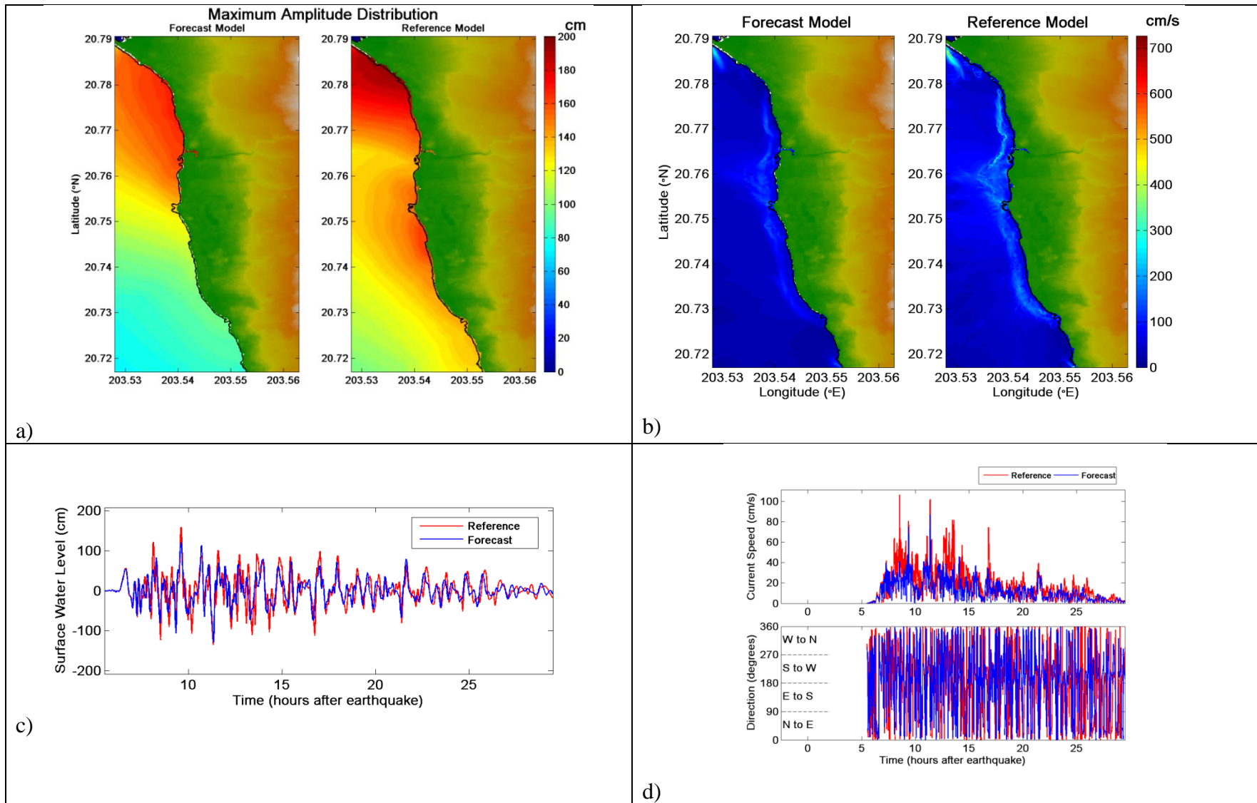
Figure 53. Comparative plot of synthetic case NTSZ 21-30 between forecast and reference models, a) maximum tsunami wave amplitude distribution, b) maximum current speed distribution, c) tsunami time series at the warning point, and d) current speed, and directionality at the warning point.
