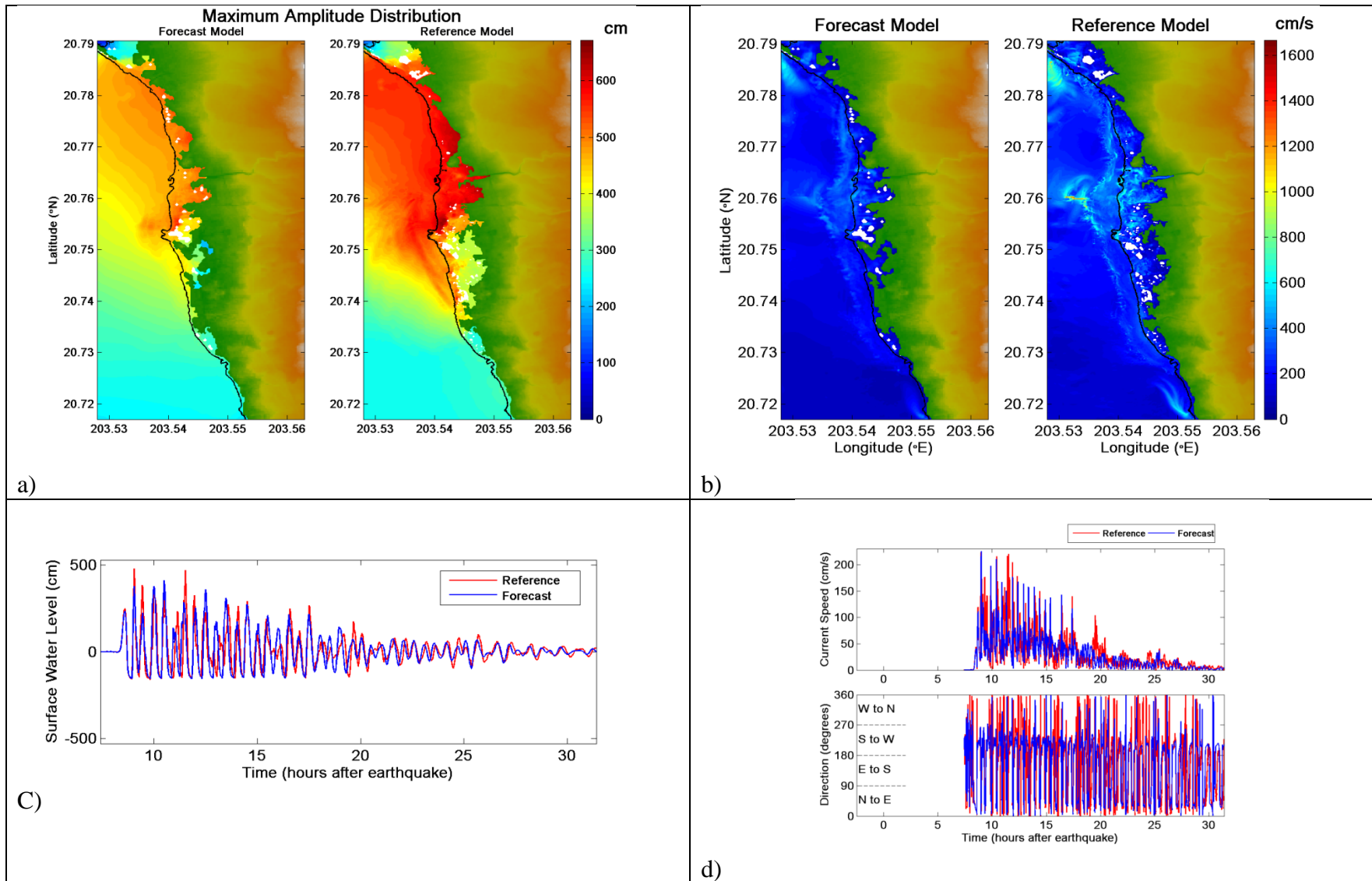
Figure 47. Comparative plot of synthetic case MOSZ 1-10 between forecast and reference models, a) maximum tsunami wave amplitude distribution, b) maximum current speed distribution, c) tsunami time series at the warning point, and d) current speed, and directionality at the warning point. White areas on land for the top figure indicate non-inundated sections.
