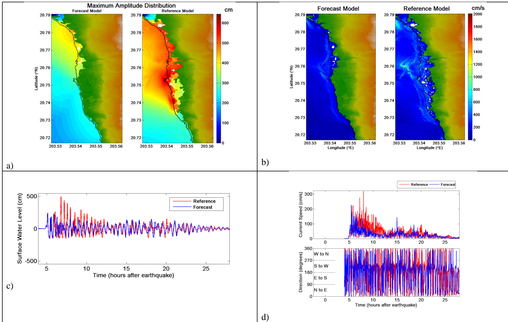
Figure 20. Comparative plot of synthetic case ACSZ 11-20 between forecast and reference models, a) maximum tsunami wave amplitude distribution, b) maximum current speed distribution, c) tsunami time series at the warning point, and d) current speed, and directionality at the warning point. White areas on land for the top figures indicate non-inundated sections.
