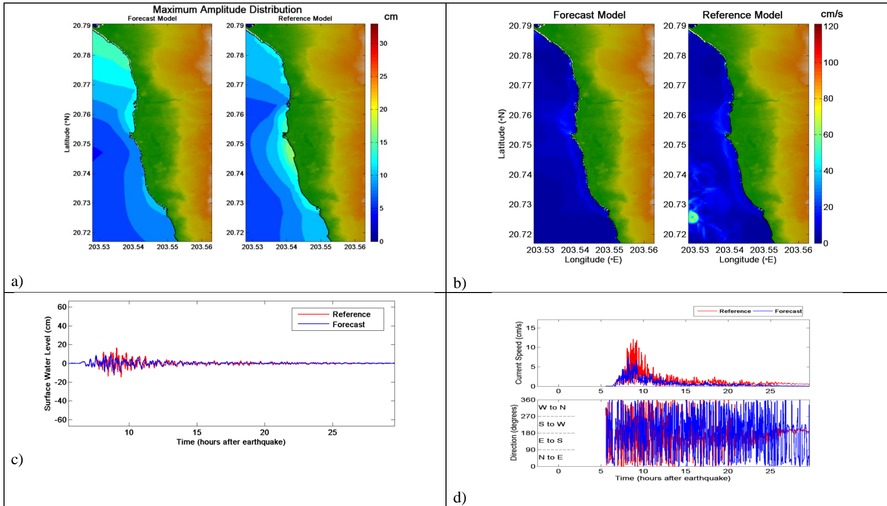
Figure 11. Comparative plot of 2006 Tonga tsunami between forecast and reference models, a) maximum tsunami wave amplitude distribution, b) maximum current speed distribution, c) tsunami time series at the warning point, and d) current speed, and directionality at the warning point.
