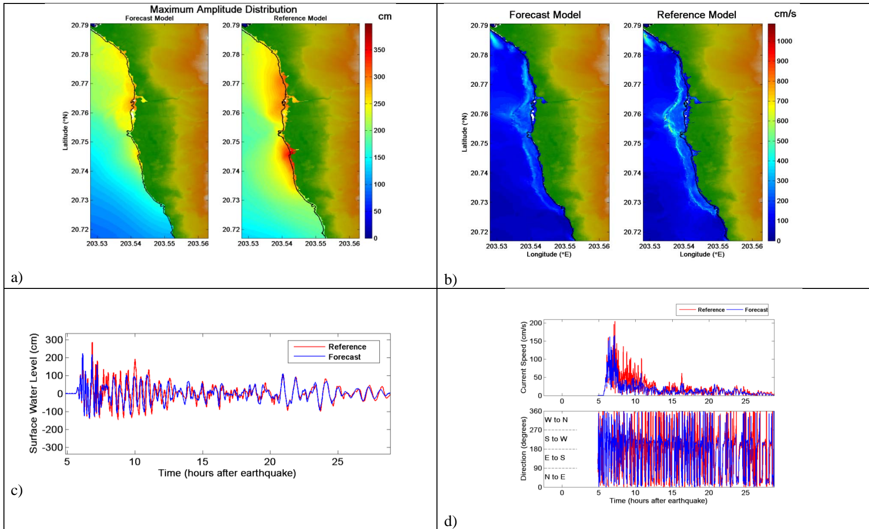
Figure 23. Comparative plot of synthetic case ACSZ 41-50 between forecast and reference models, a) maximum tsunami wave amplitude distribution, b) maximum current speed distribution, c) tsunami time series at the warning point, and d) current speed, and directionality at the warning point. White areas on land for the top figure indicate non-inundated sections.
