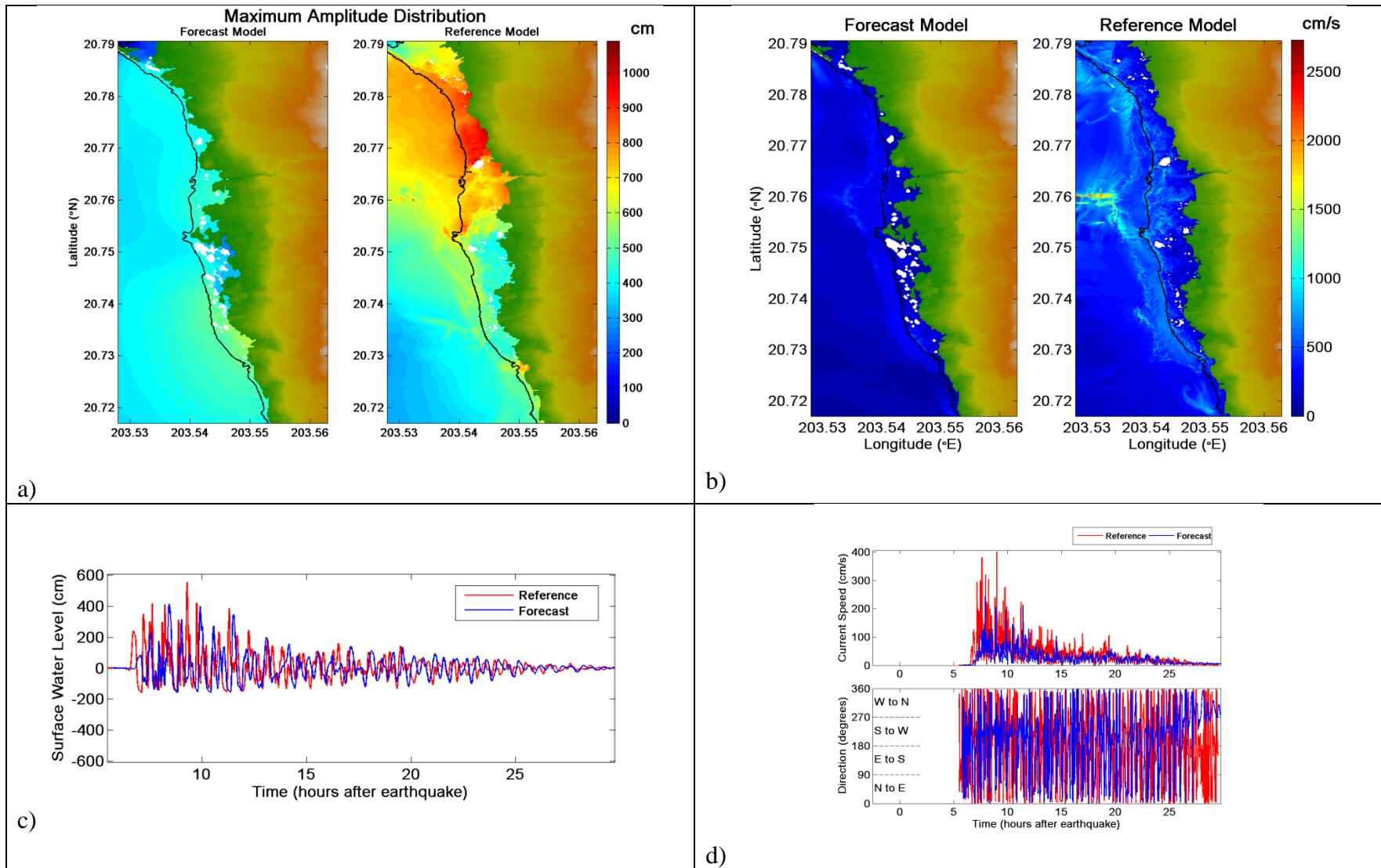
Figure 41. Comparative plot of synthetic case KISZ 11-20 between forecast and reference models, a) maximum tsunami wave amplitude distribution, b) maximum current speed distribution, c) tsunami time series at the warning point, and d) current speed, and directionality at the warning point. White areas on land for the top figure indicate non-inundated sections.
