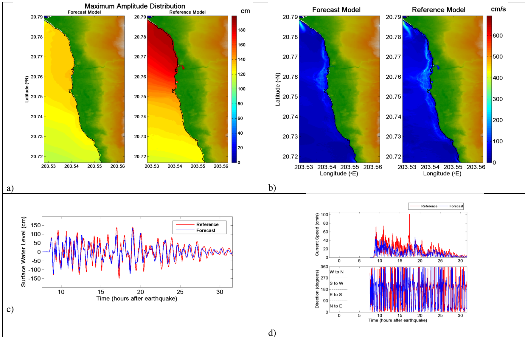
Figure 48. Comparative plot of synthetic case MOSZ 8-17 between forecast and reference models, a) maximum tsunami wave amplitude distribution, b) maximum current speed distribution, c) tsunami time series at the warning point, and d) current speed, and directionality at the warning point.
