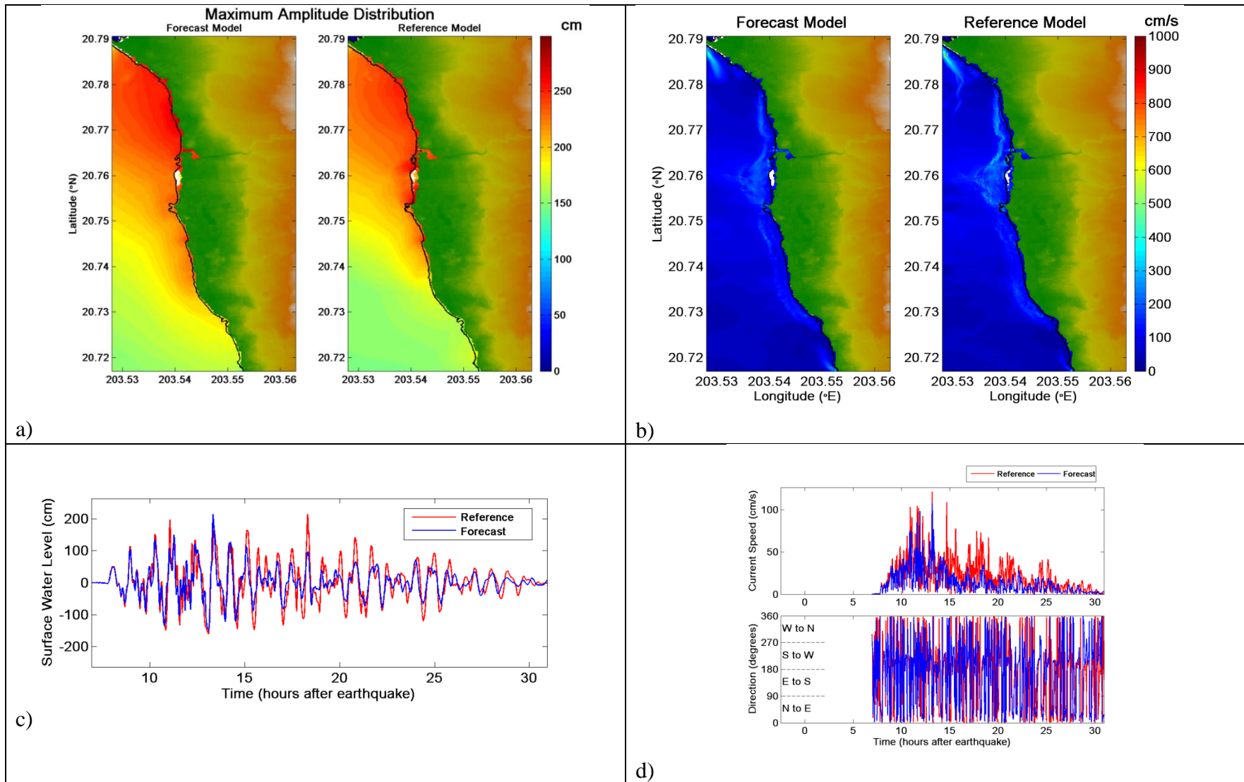
Figure 45. Comparative plot of synthetic case KISZ 56-65 between forecast and reference models, a) maximum tsunami wave amplitude distribution, b) maximum current speed distribution, c) tsunami time series at the warning point, and d) current speed, and directionality at the warning point. White areas on land for the top figure indicate non-inundated sections.
