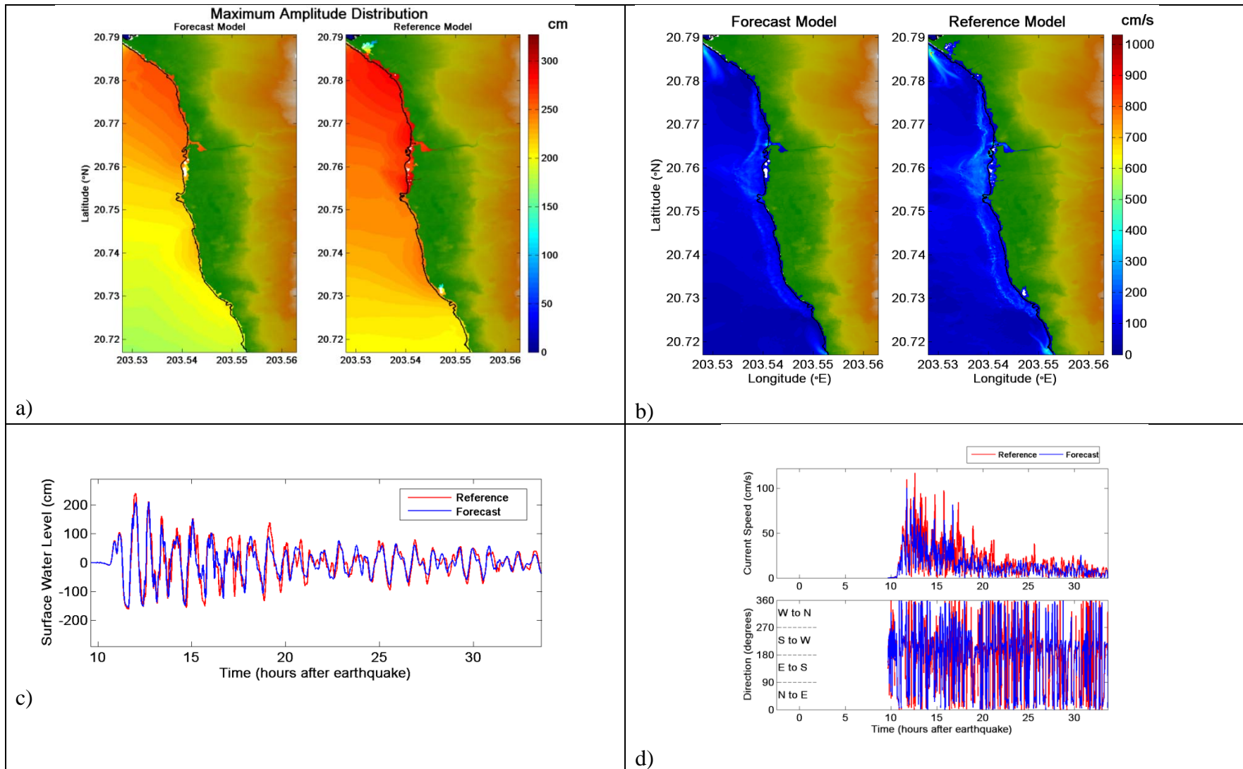
Figure 38. Comparative plot of synthetic case EPSZ 01-10 between forecast and reference models, a) maximum tsunami wave amplitude distribution, b) maximum current speed distribution, c) tsunami time series at the warning point, and d) current speed, and directionality at the warning point. White areas on land for the top figure indicate non-inundated sections.
