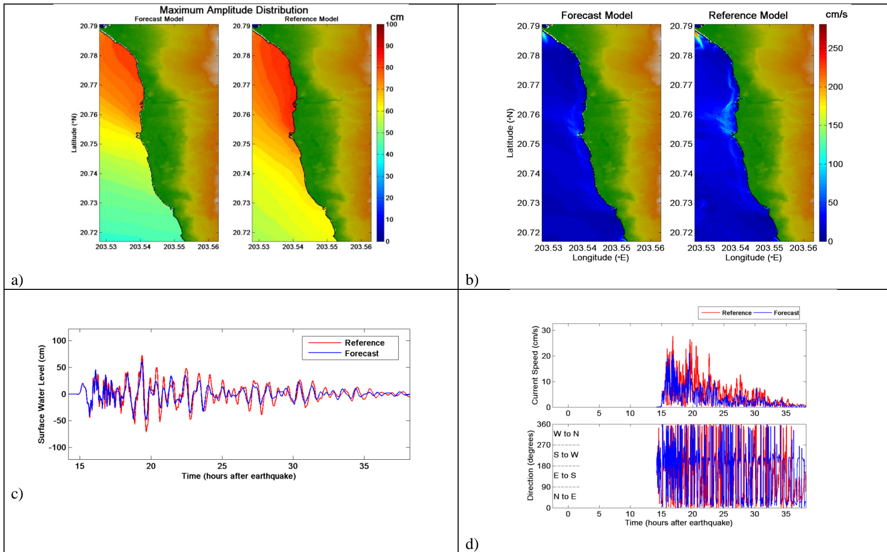
Figure 17. Comparative plot of 2010 Chile tsunami between forecast and reference models, a) maximum tsunami wave amplitude distribution, b) maximum current speed distribution, c) tsunami time series at the warning point, and d) current speed, and directionality at the warning point.
