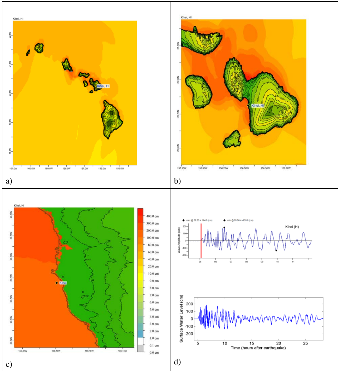
Figure C.2. Response of the Kihei forecast model to synthetic scenario ACSZ 56-65 ( \alpha=30 ). Maximum sea surface elevation for (a) A-grid, b) B-grid, c) C-grid. Sea surface elevation time series at the C-grid warning point (d). The lower time series plot is the result obtained during model development and is shown for comparison with test results.
