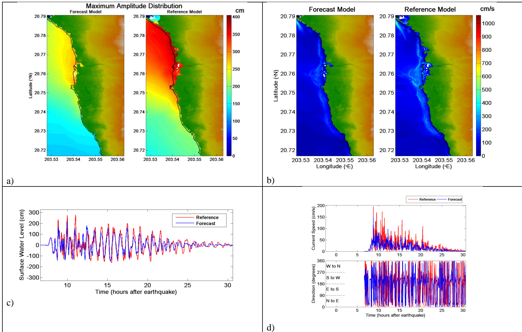
Figure 44. Comparative plot of synthetic case KISZ 52-61 between forecast and reference models, a) maximum tsunami wave amplitude distribution, b) maximum current speed distribution, c) tsunami time series at the warning point, and d) current speed, and directionality at the warning point. White areas on land for the top figure indicate non-inundated sections.
