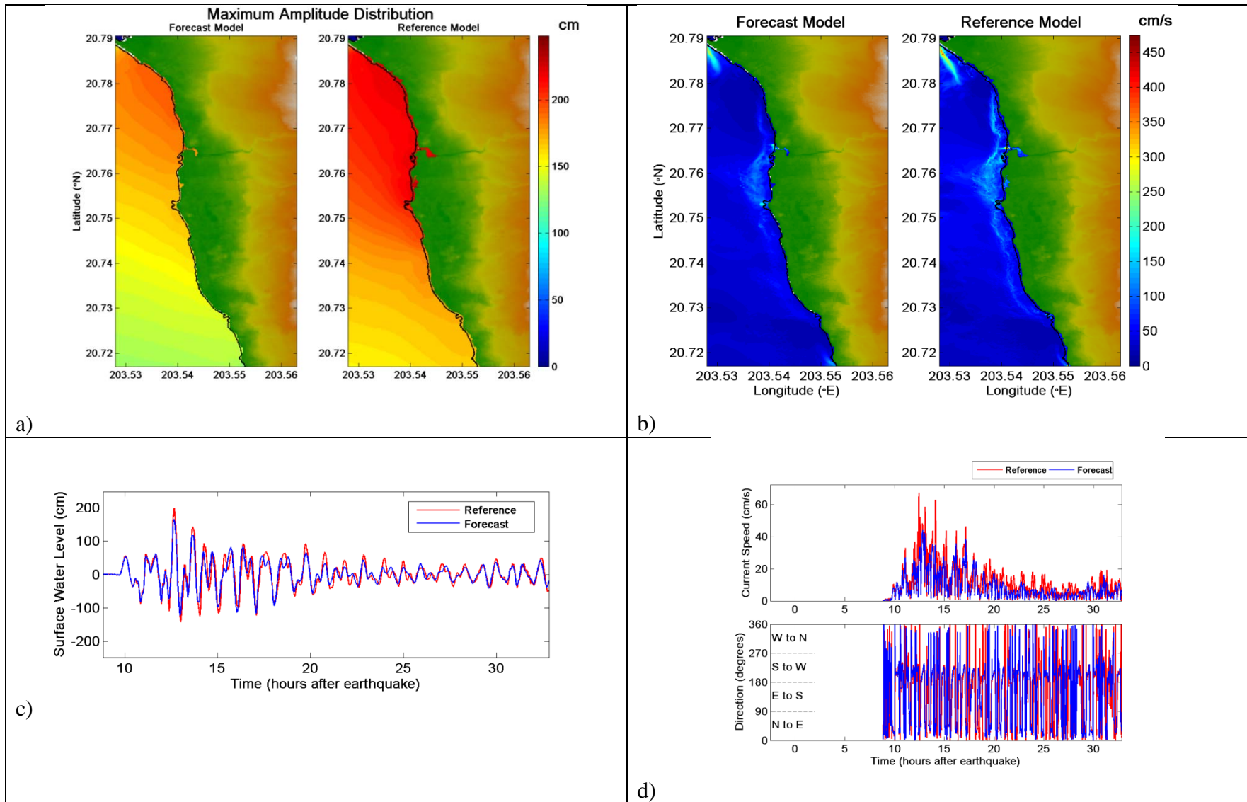
Figure 49. Comparative plot of synthetic case NGSZ 1-10 between forecast and reference models, a) maximum tsunami wave amplitude distribution, b) maximum current speed distribution, c) tsunami time series at the warning point, and d) current speed, and directionality at the warning point.
