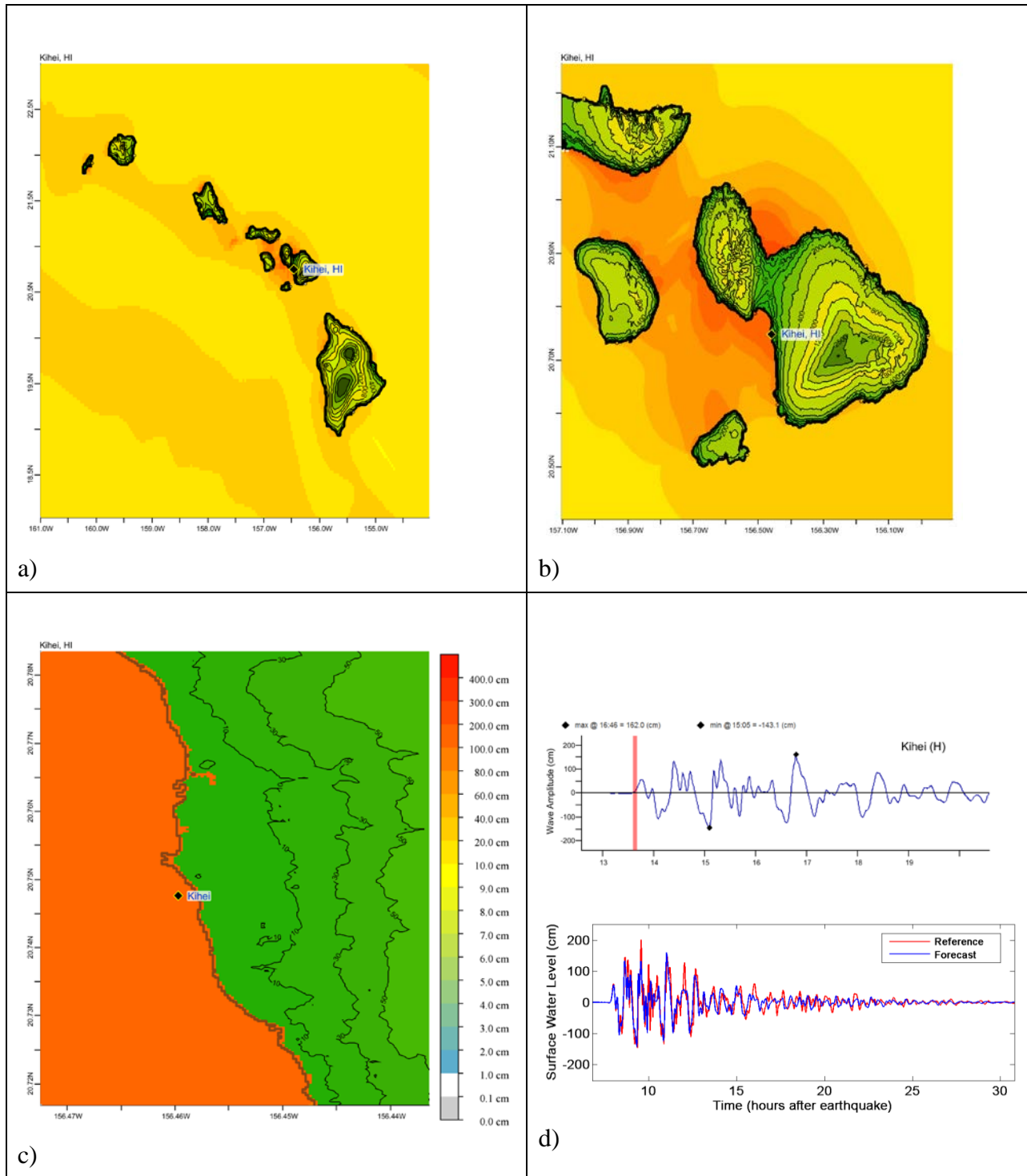
Figure C.5. Response of the Kihei forecast model to the 2011 Tohoku tsunami. Maximum sea surface elevation for (a) A-grid, b) B-grid, c) C-grid. Sea surface elevation time series at the C-grid warning point (d). The lower time series plot is the result obtained during model development and is shown for comparison with test results.
