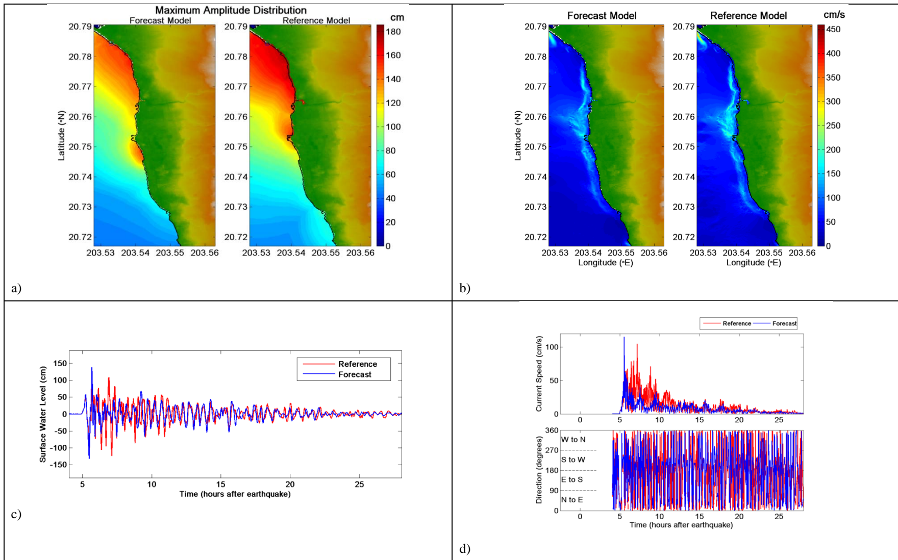
Figure 7. Comparative plot of 1957 Andreev tsunami between forecast and reference models, a) maximum tsunami wave amplitude distribution, b) maximum current speed distribution, c) tsunami time series at the warning point, and d) current speed, and directionality at the warning point.
