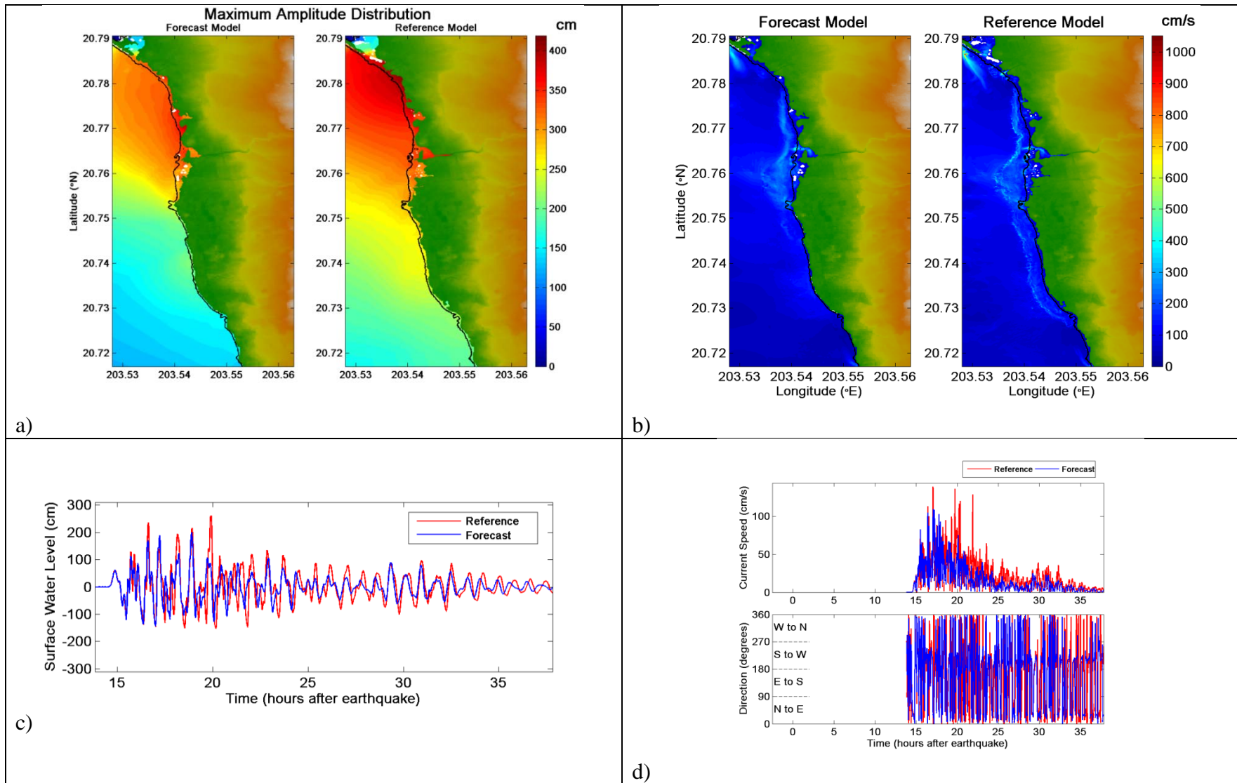
Figure 34. Comparative plot of synthetic case CSSZ 81-90 between forecast and reference models. White areas on land for the top figure indicate non-inundated sections, a) maximum tsunami wave amplitude distribution, b) maximum current speed distribution, c) tsunami time series at the warning point, and d) current speed, and directionality at the warning point.
