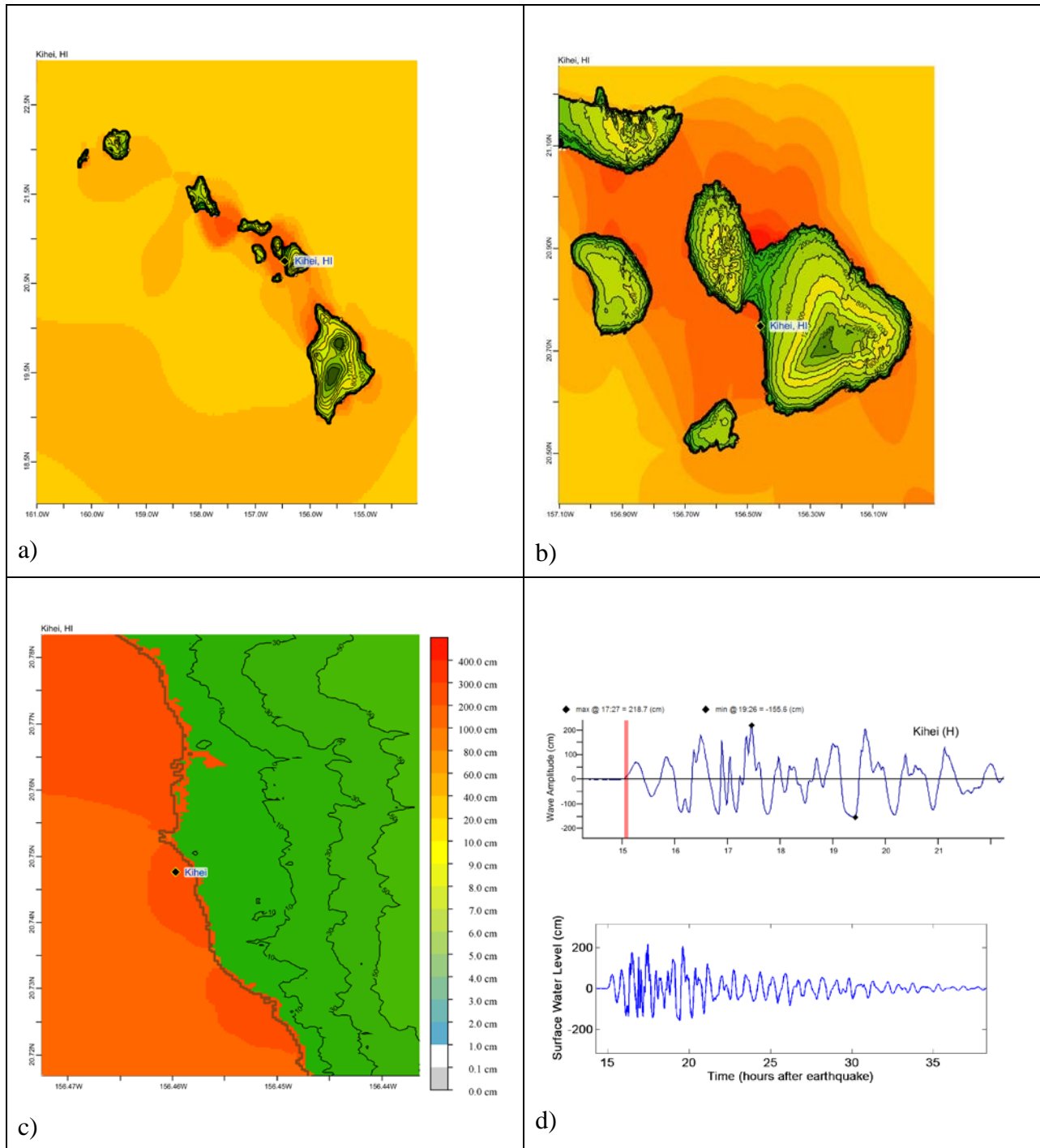
Figure C.3. Response of the Kihei forecast model to synthetic scenario CSSZ 91-100 ( \alpha=30 ). Maximum sea surface elevation for (a) A-grid, b) B-grid, c) C-grid. Sea surface elevation time series at the C-grid warning point (d). The lower time series plot is the result obtained during model development and is shown for comparison with test results.
