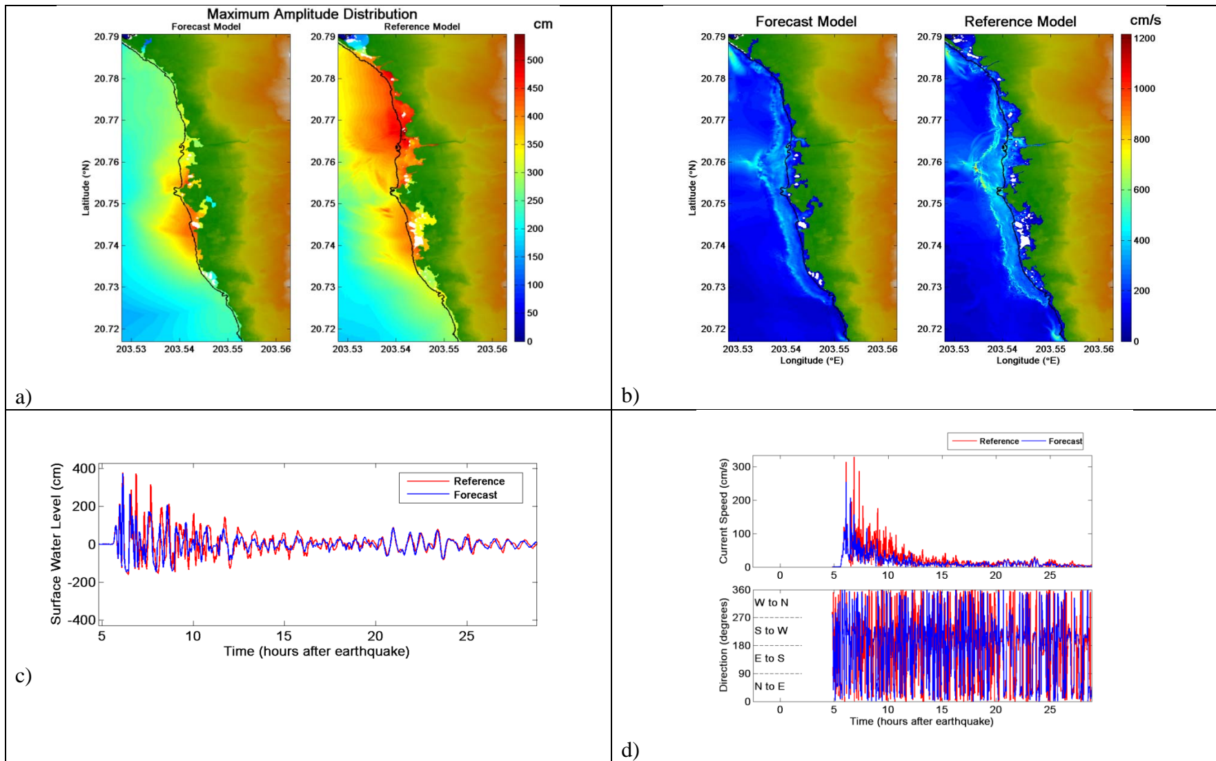
Figure 24. Comparative plot of synthetic case ACSZ 46-55 between forecast and reference models, a) maximum tsunami wave amplitude distribution, b) maximum current speed distribution, c) tsunami time series at the warning point, and d) current speed, and directionality at the warning point. White areas on land for the top figure indicate non-inundated sections.
