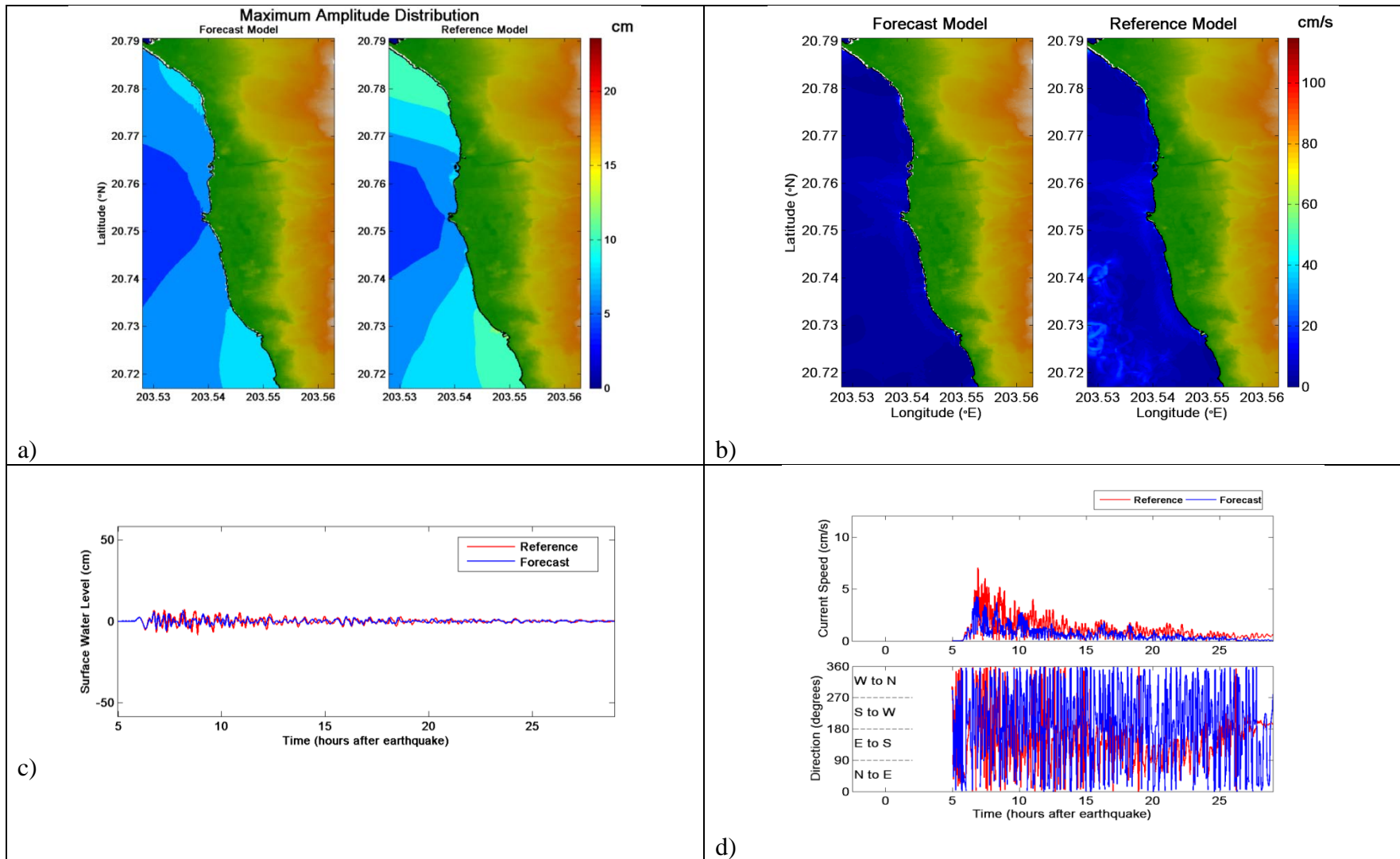
Figure 16. Comparative plot of 2009 Samoa tsunami between forecast and reference models, a) maximum tsunami wave amplitude distribution, b) maximum current speed distribution, c) tsunami time series at the warning point, and d) current speed, and directionality at the warning point.
