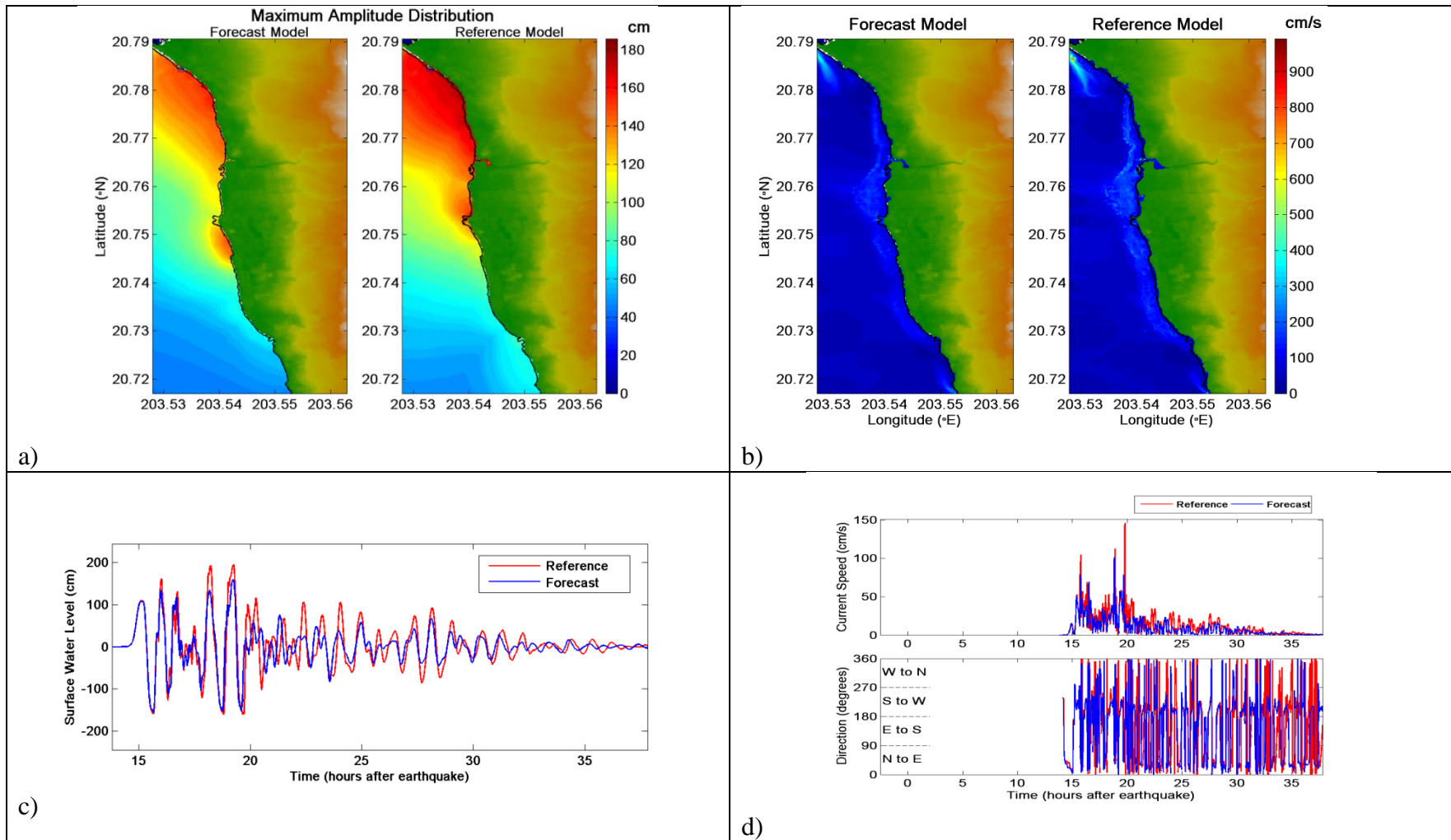
Figure 8. Comparative plot of 1960 Chile tsunami between forecast and reference models, a) maximum tsunami wave amplitude distribution, b) maximum current speed distribution, c) tsunami time series at the warning point, and d) current speed, and directionality at the warning point.
