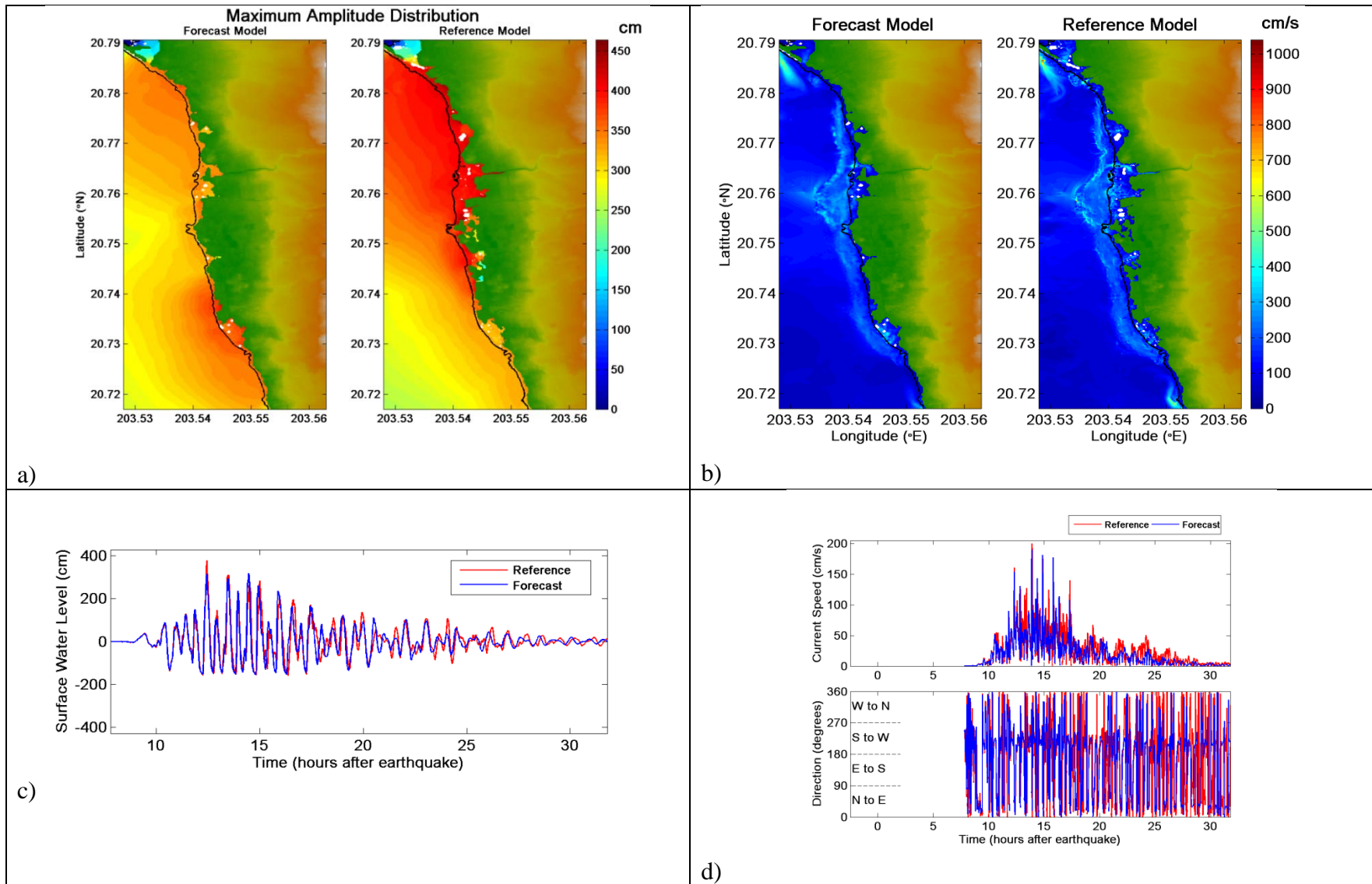
Figure 46. Comparative plot of synthetic case KISZ 66-75 between forecast and reference models, a) maximum tsunami wave amplitude distribution, b) maximum current speed distribution, c) tsunami time series at the warning point, and d) current speed, and directionality at the warning point. White areas on land for the top figure indicate non-inundated sections.
