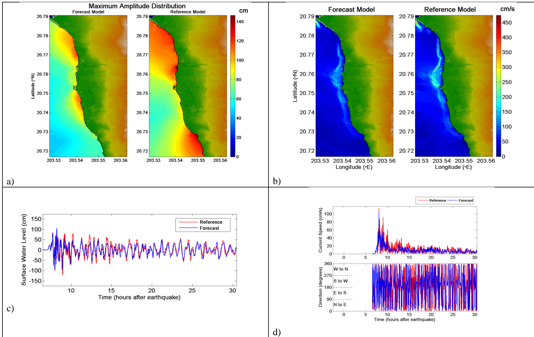
Figure 26. Comparative plot of synthetic case CSSZ 1-10 between forecast and reference models, a) maximum tsunami wave amplitude distribution, b) maximum current speed distribution, c) tsunami time series at the warning point, and d) current speed, and directionality at the warning point.
