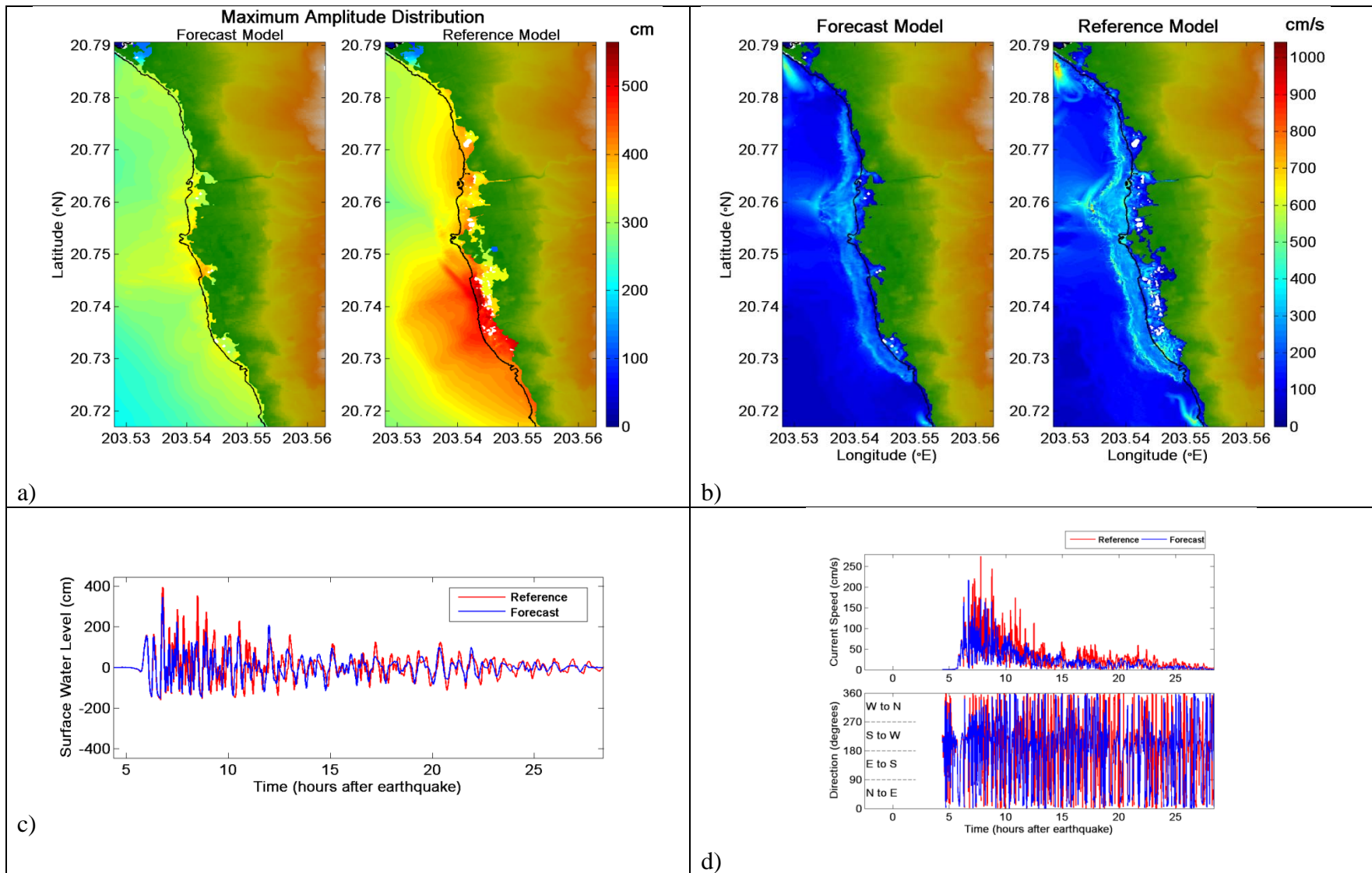
Figure 54. Comparative plot of synthetic case NTSZ 30-39 between forecast and reference models, a) maximum tsunami wave amplitude distribution, b) maximum current speed distribution, c) tsunami time series at the warning point, and d) current speed, and directionality at the warning point. White areas on land for the top figure indicate non-inundated sections.
