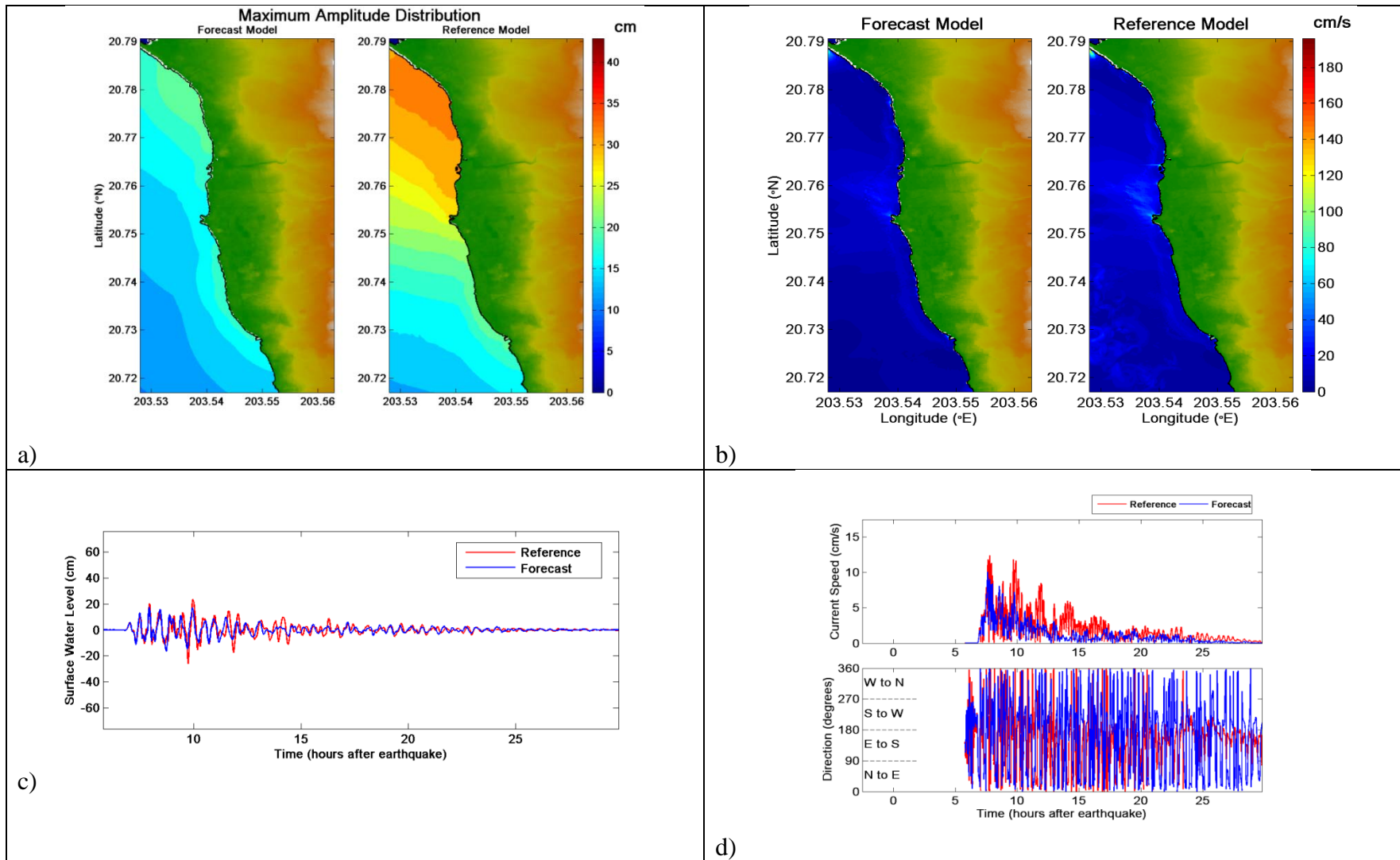
Figure 12. Comparative plot of 2006 Kuril tsunami between forecast and reference models, a) maximum tsunami wave amplitude distribution, b) maximum current speed distribution, c) tsunami time series at the warning point, and d) current speed, and directionality at the warning point.
