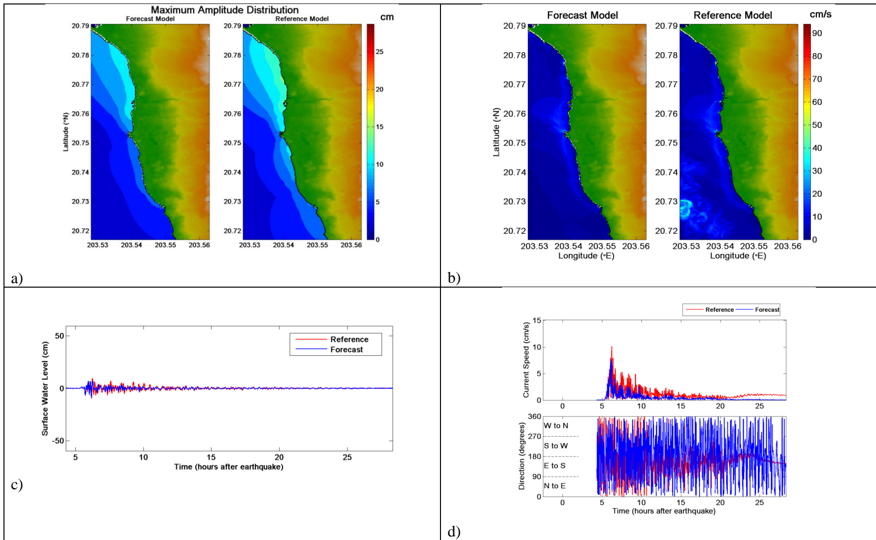
Figure 10. Comparative plot of 2003 Rat Island tsunami between forecast and reference models, a) maximum tsunami wave amplitude distribution, b) maximum current speed distribution, c) tsunami time series at the warning point, and d) current speed, and directionality at the warning point.
