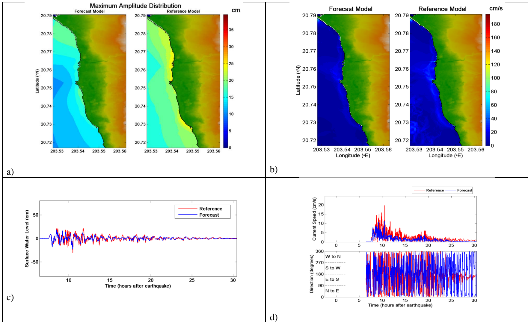
Figure 9. Comparative plot of 1994 East Kuril tsunami between forecast and reference models, a) maximum tsunami wave amplitude distribution, b) maximum current speed distribution, c) tsunami time series at the warning point, and d) current speed, and directionality at the warning point.
