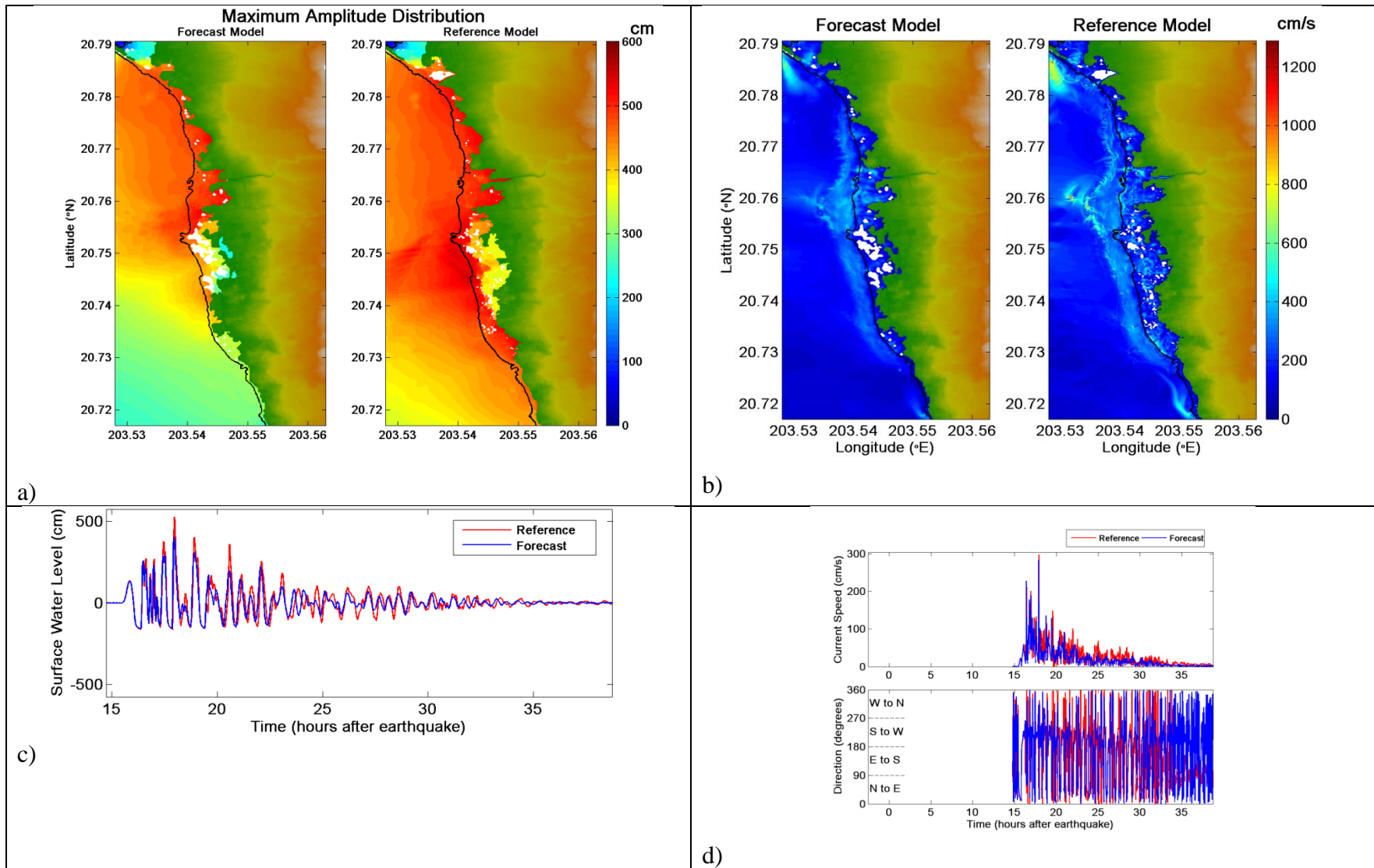
Figure 36. Comparative plot of synthetic case CSSZ 101-110 between forecast and reference models, a) maximum tsunami wave amplitude distribution, b) maximum current speed distribution, c) tsunami time series at the warning point, and d) current speed, and directionality at the warning point. White areas on land for the top figure indicate non-inundated sections.
