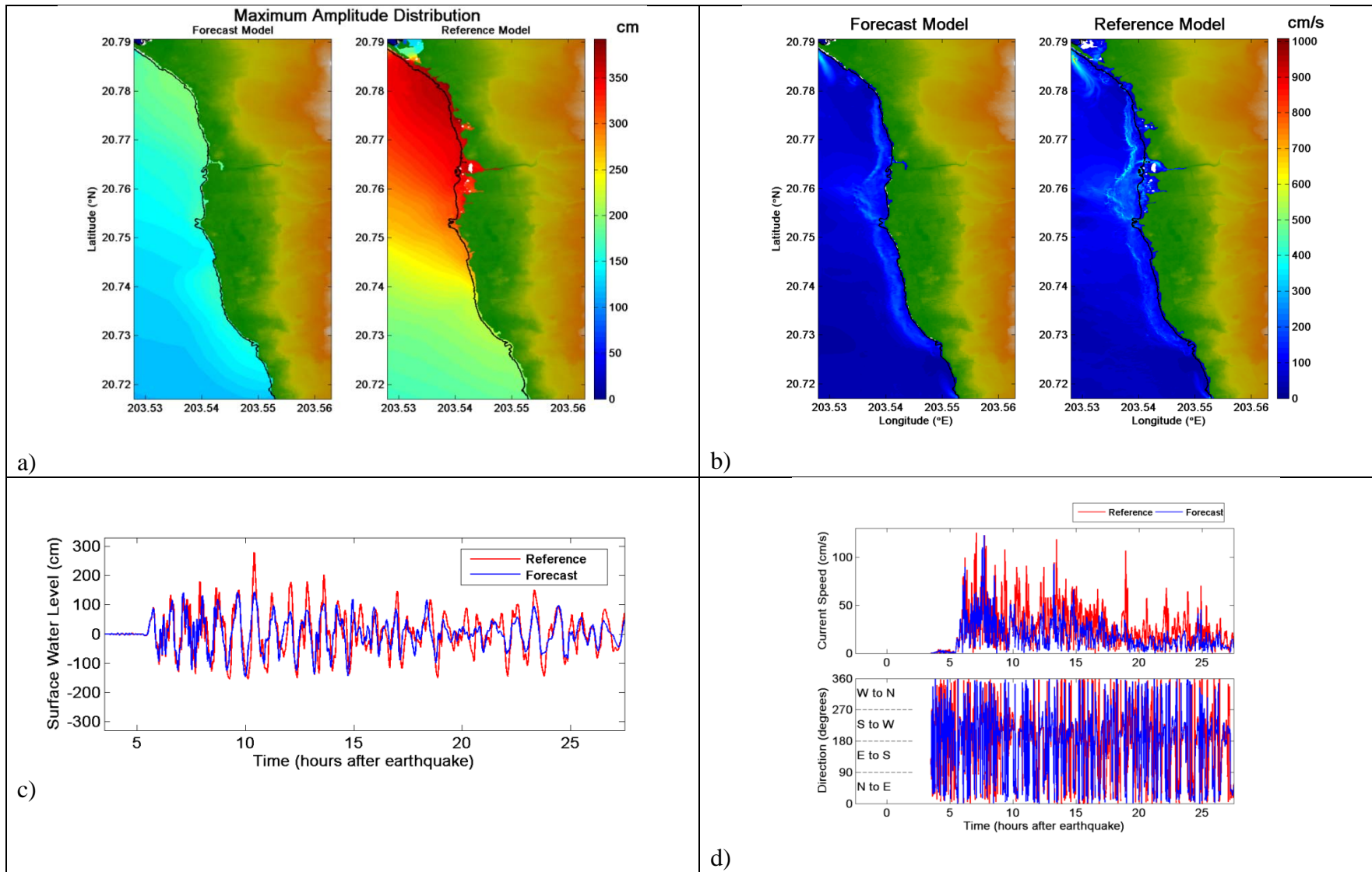
Figure 19. Comparative plot of synthetic case ACSZ 1-10 between forecast and reference models, a) maximum tsunami wave amplitude distribution, b) maximum current speed distribution, c) tsunami time series at the warning point, and d) current speed, and directionality at the warning point. White areas on land for the top figure indicate non-inundated sections.
