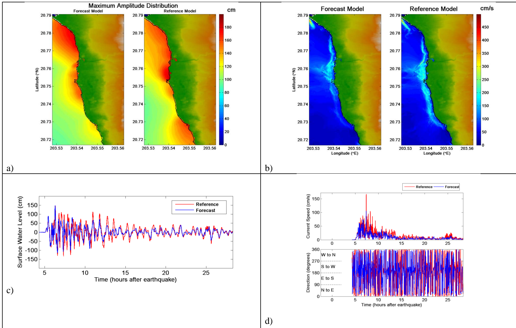
Figure 22. Comparative plot of synthetic case ACSZ 31-40 between forecast and reference models, a) maximum tsunami wave amplitude distribution, b) maximum current speed distribution, c) tsunami time series at the warning point, and d) current speed, and directionality at the warning point.
