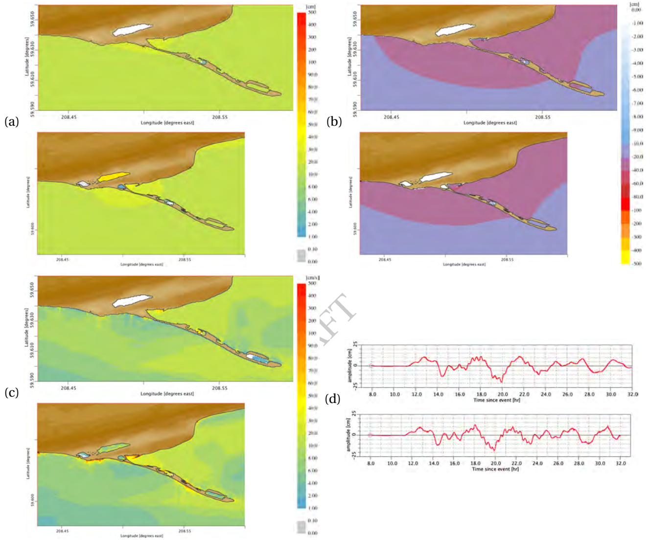
Figure 21: Comparisons for the FM (top insets) and the RM (bottom insets) C-grid results for the magnitude 9.3 synthetic scenario event with the source segment 56–65 on Kamchatka–Yap–Mariana–Izu–Bonin Subduction Zone (KISZ) (Figure B.5, Table B.5). (a) Maximum and (b) minimum sea surface elevations, (c) maximum wave speeds at each C-grid point and (d) time histories of water surface elevations at the Homer forecast point.
