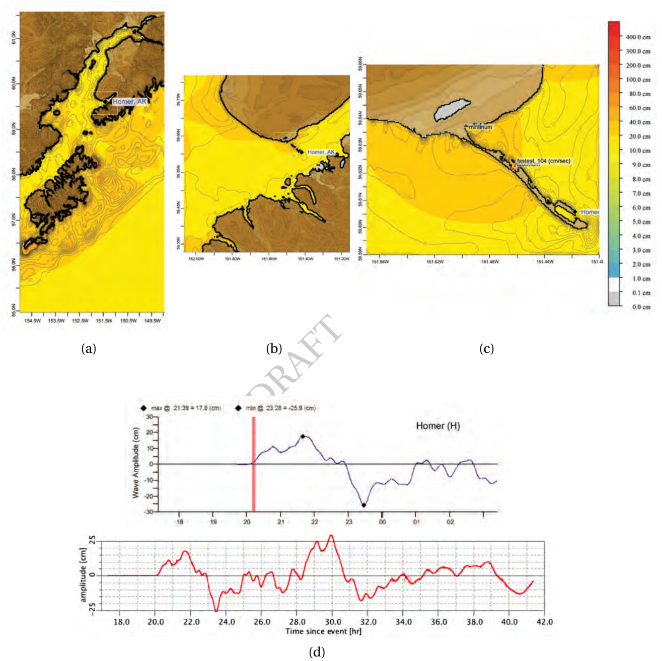
Figure C.2: Response of the Homer forecast model to synthetic scenario CSSZ 89–98 ( \alpha = 25 ). Maximum sea surface elevation for (a) A-grid, b) B-grid, c) C-grid and d) sea surface elevation time series at the C-grid warning point. Sea surface elevation time series obtained during SIFT testing (upper inset) is compared the one obtained during model development (lower inset).
