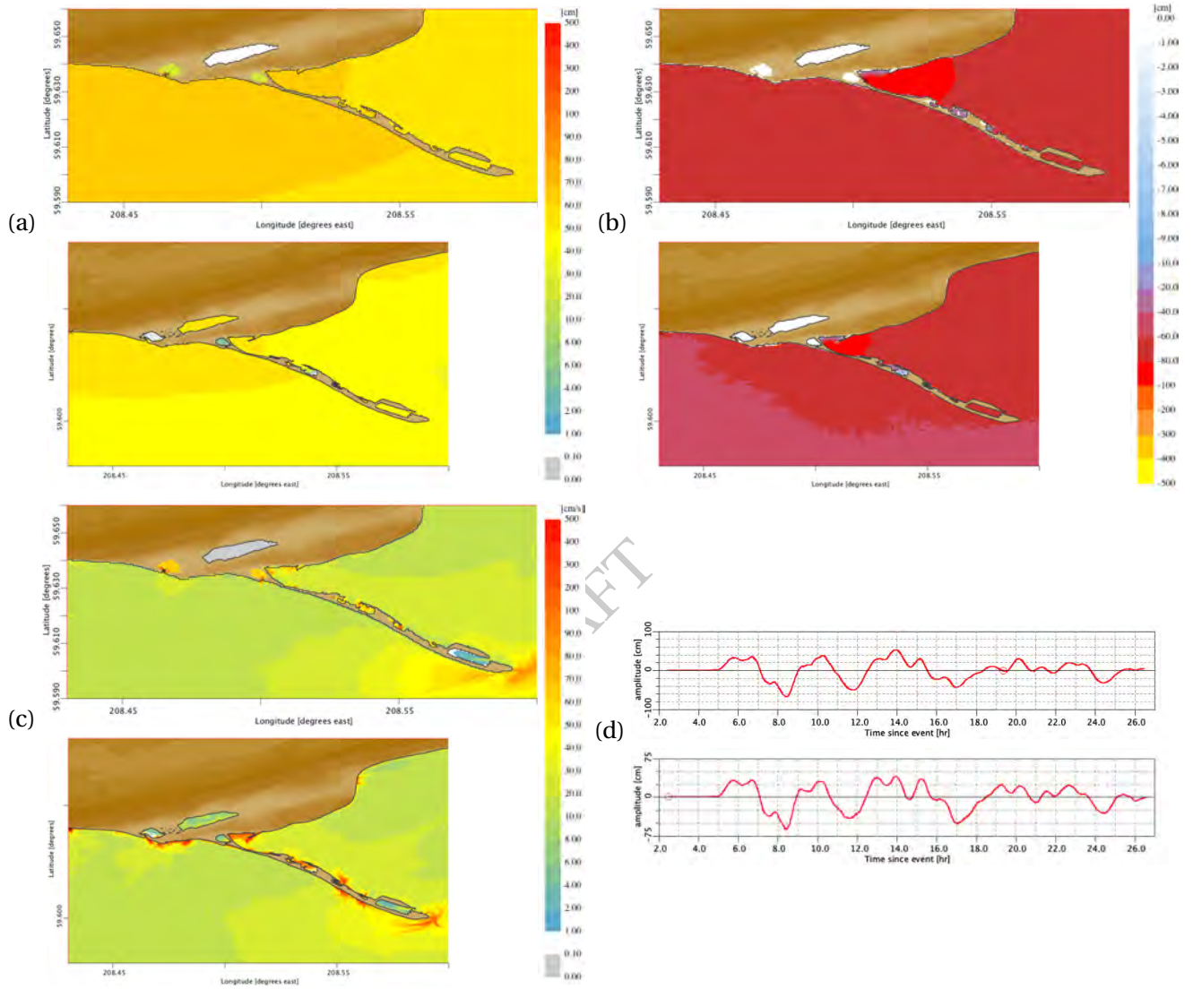
Figure 12: Comparisons for the FM (top insets) and the RM (bottom insets) C-grid results for the magnitude 9.3 synthetic scenario event with the source segment 56–65 on Aleutian–Alaska–Cascadia Subduction Zone (ACSZ) (Figure B.1, Table B.1). (a) Maximum and (b) minimum sea surface elevations, (c) maximum wave speeds at each C-grid point and (d) time histories of water surface elevations at the Homer forecast point.
