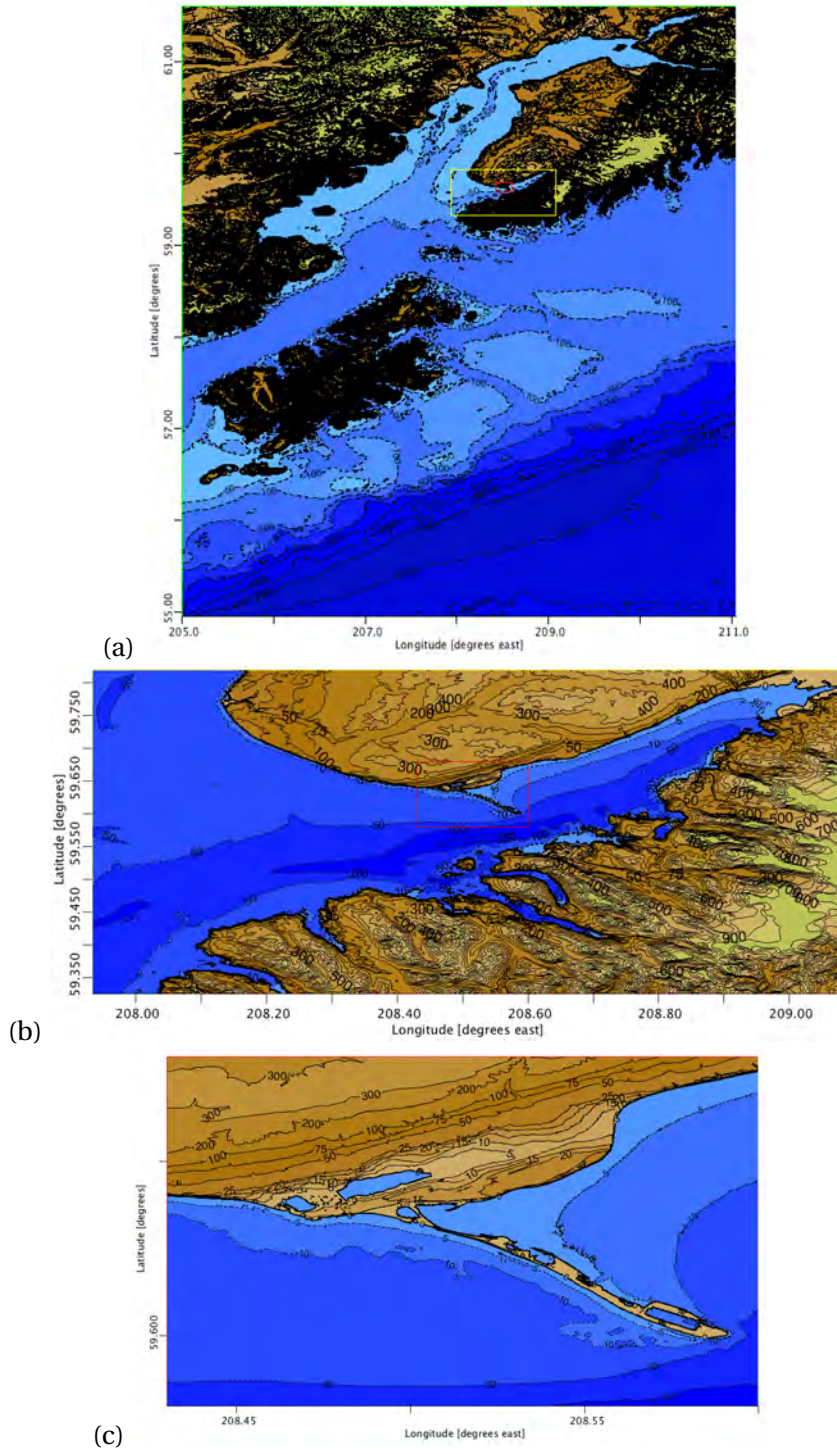
Figure 4: Extent of Homer, Alaska RM grids: (a) A-grid, (b) B-grid, (c) C-grid. Yellow and red rectangles in insets show B-grid and C-grid extensions respectively. Grid extents, resolutions and sources are summarized in Table 1.
