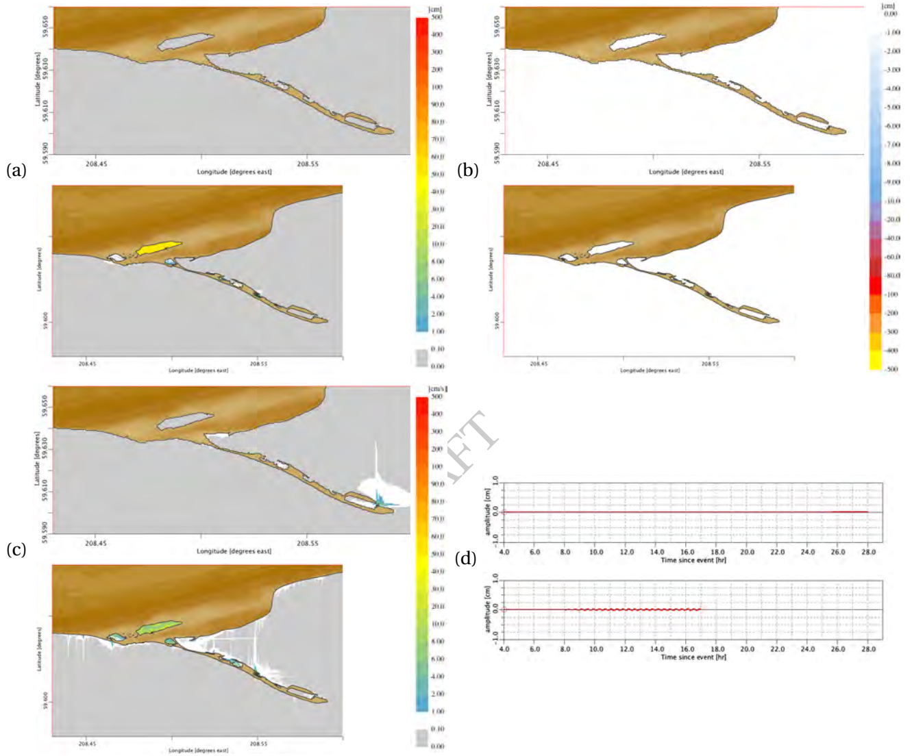
Figure 28: Comparisons for the FM (top insets) and the RM (bottom insets) C-grid results for the micro-tsunami synthetic scenario event with the source 6b on Aleutian-Alaska-Cascadia Subduction Zone (ACSZ) (Figure B.1, Table B.1). (a) Maximum and (b) minimum sea surface elevations, (c) maximum wave speeds at each C-grid point and (d) time histories of water surface elevations at the Homer forecast point.
