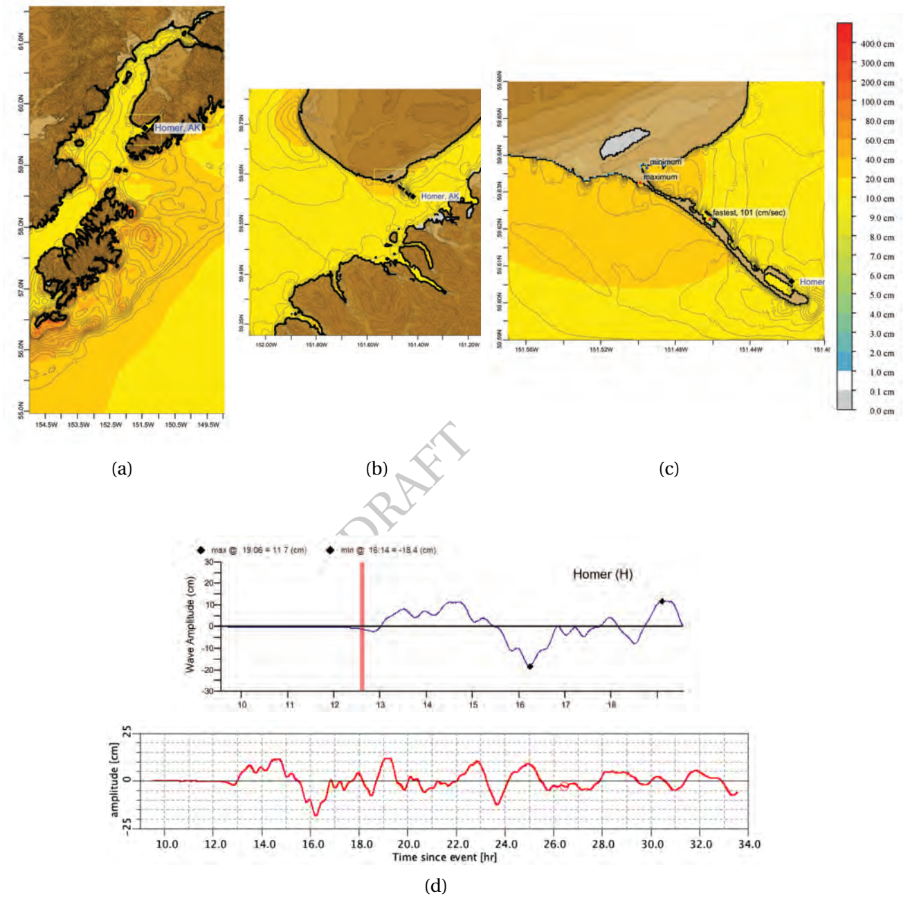
Figure C.4: Response of the Homer forecast model to synthetic scenario NTSZ 30–39 ( \alpha = 25 ). Maximum sea surface elevation for (a) A-grid, b) B-grid, c) C-grid and d) sea surface elevation time series at the C-grid warning point. Sea surface elevation time series obtained during SIFT testing (upper inset) is compared the one obtained during model development (lower inset).
