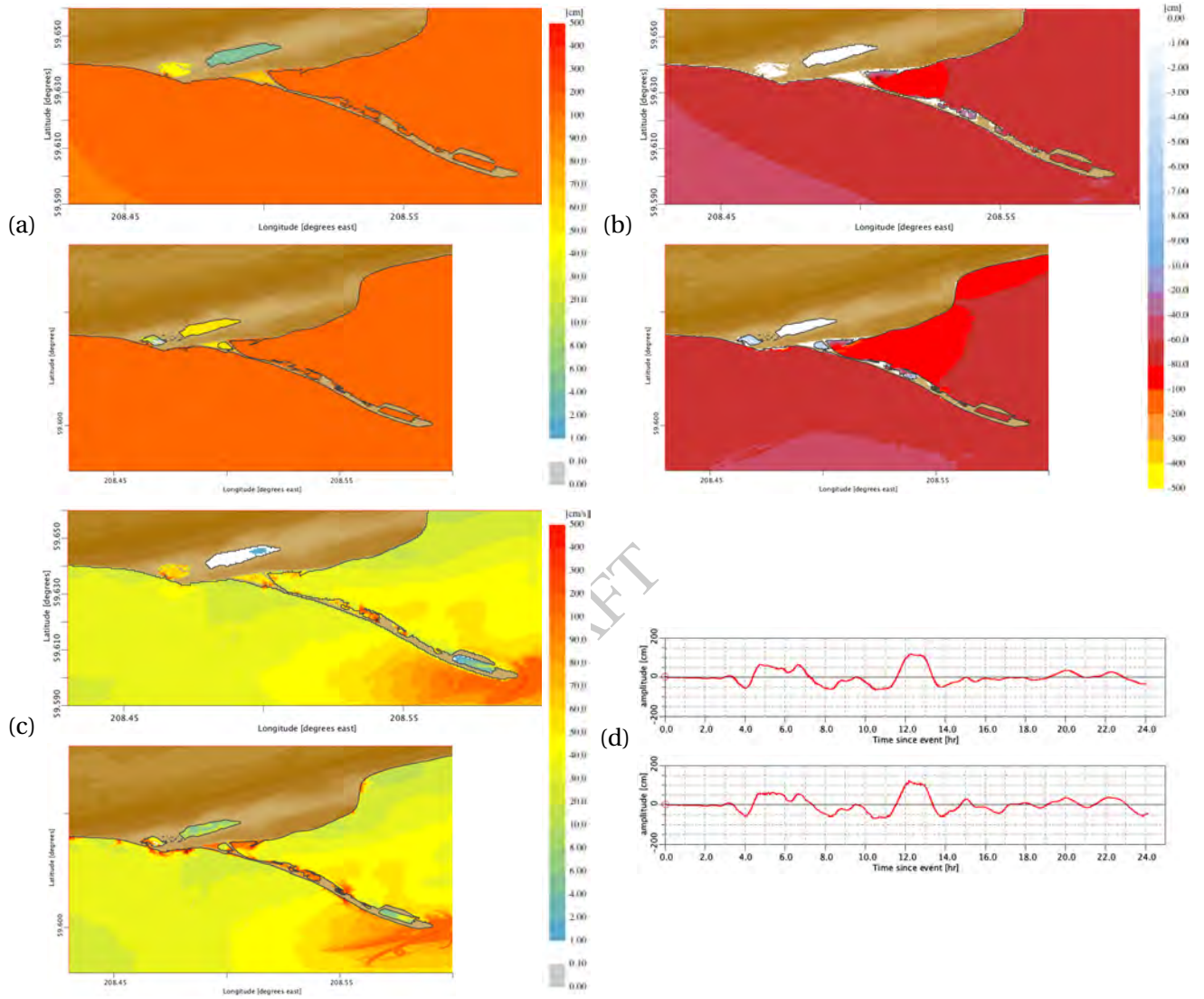
Figure 10: Comparisons for the FM (top insets) and the RM (bottom insets) C-grid results for the magnitude 9.3 synthetic scenario event with the source segment 22–31 on Aleutian–Alaska–Cascadia Subduction Zone (ACSZ) (Figure B.1, Table B.1). (a) Maximum and (b) minimum sea surface elevations, (c) maximum wave speeds at each C-grid point and (d) time histories of water surface elevations at the Homer forecast point.
