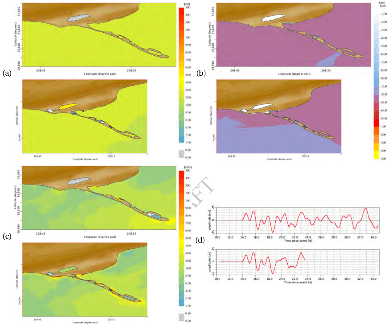
Figure 23: Comparisons for the FM (top insets) and the RM (bottom insets) C-grid results for the magnitude 9.3 synthetic scenario event with the source segment 3–12 on New Guinea Subduction Zone (NGSZ) (Figure B.7, Table B.7). (a) Maximum and (b) minimum sea surface elevations, (c) maximum wave speeds at each C-grid point and (d) time histories of water surface elevations at the Homer forecast point.
