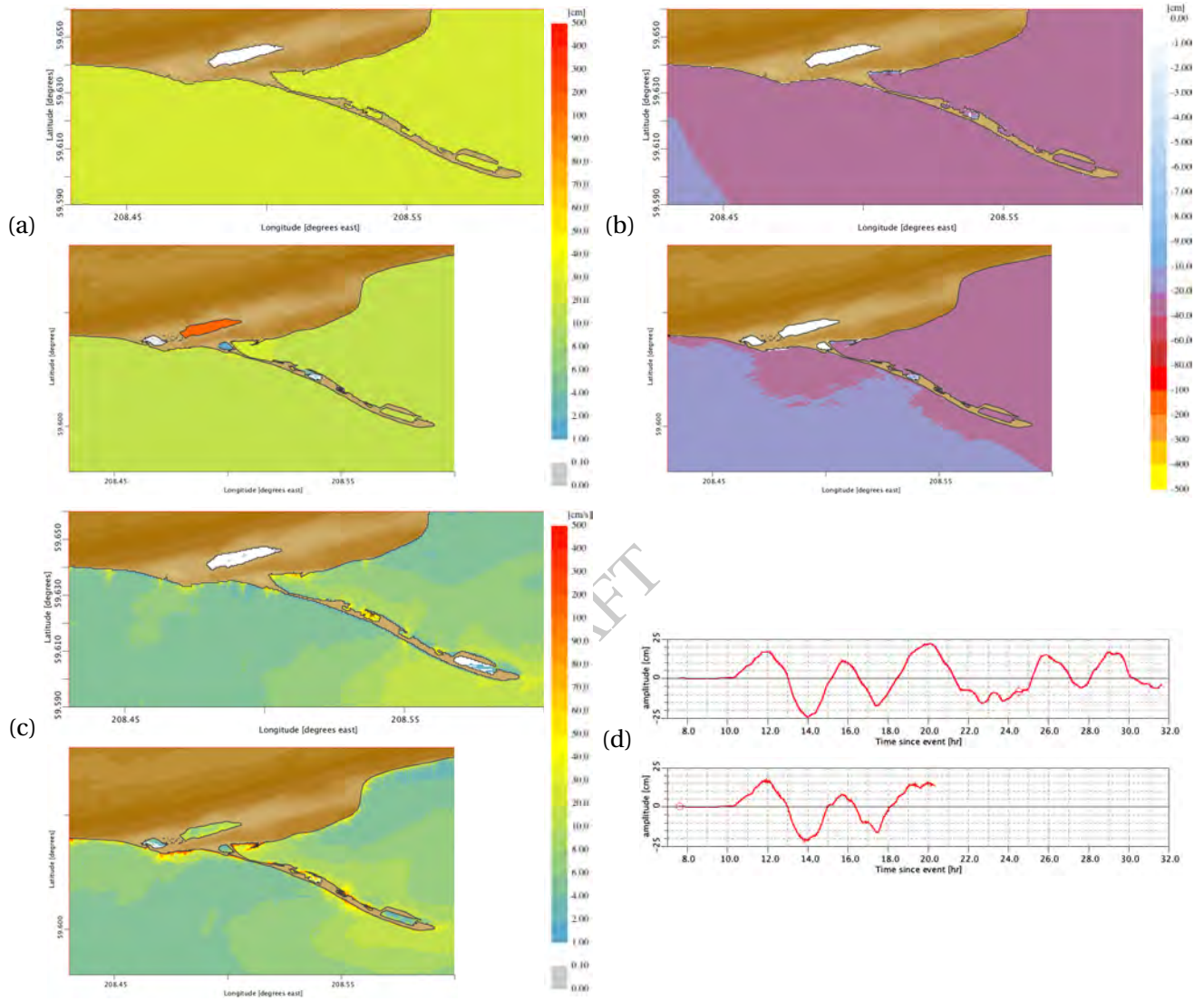
Figure 13: Comparisons for the FM (top insets) and the RM (bottom insets) C-grid results for the magnitude 9.3 synthetic scenario event with the source segment 1–10 on Central and South America Subduction Zone (CSSZ) (Figure B.2, Table B.2). (a) Maximum and (b) minimum sea surface elevations, (c) maximum wave speeds at each C-grid point and (d) time histories of water surface elevations at the Homer forecast point.
