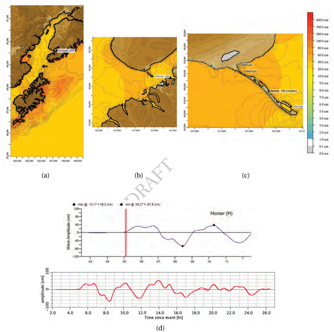
Figure C.1: Response of the Homer forecast model to synthetic scenario ACSZ 56–65 ( \alpha = 25 ). Maximum sea surface elevation for (a) A-grid, b) B-grid, c) C-grid and d) sea surface elevation time series at the C-grid warning point. Sea surface elevation time series obtained during SIFT testing (upper inset) is compared the one obtained during model development (lower inset).
