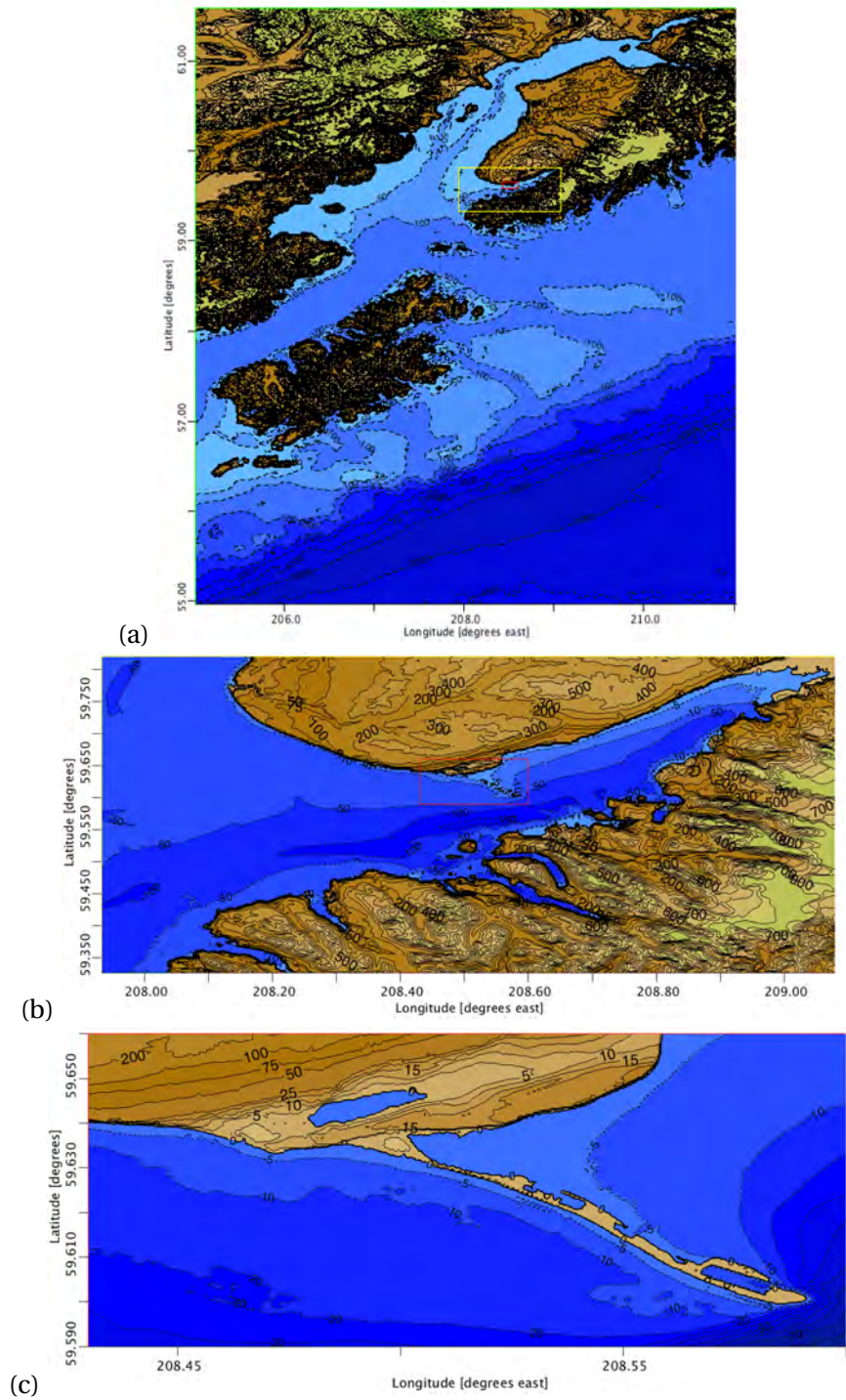
Figure 5: Extent of Homer, Alaska FM grids: (a) A-grid, (b) B-grid, and (c) C-grid. Yellow and red rectangles in insets show B-grid and C-grid extensions respectively. Grid extents, resolutions and sources are summarized in Table 1.
