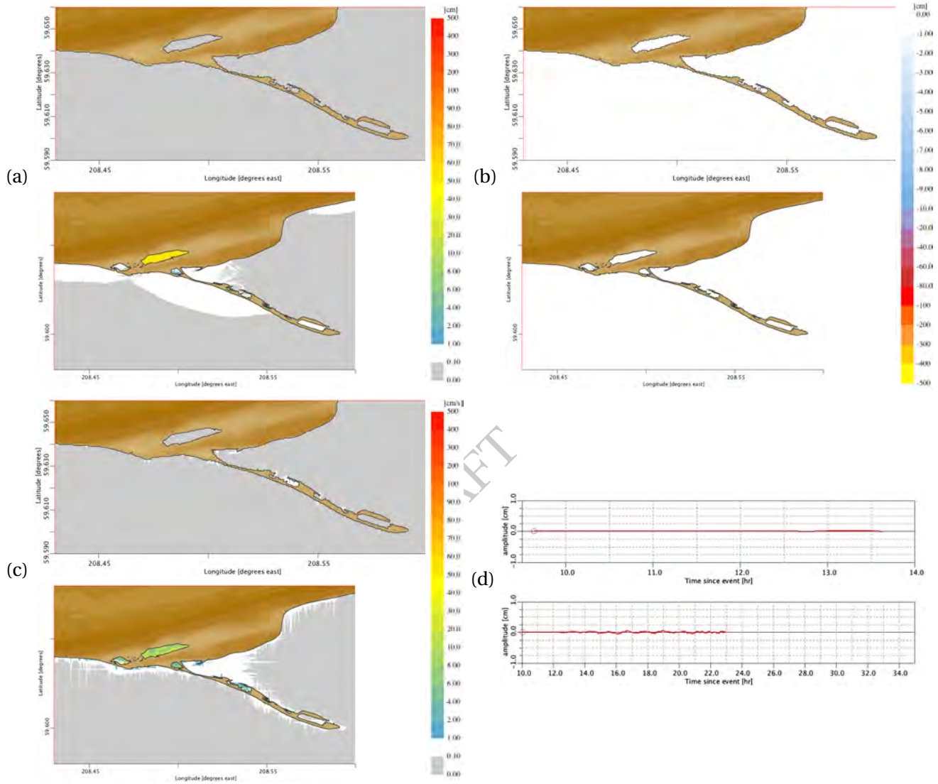
Figure 27: Comparisons for the FM (top insets) and the RM (bottom insets) C-grid results for the magnitude 7.5 synthetic scenario event with the source 36b on New Zealand–Kermadec–Tonga Subduction Zone (NTSZ) (Figure B.8, Table B.8). (a) Maximum and (b) minimum sea surface elevations, (c) maximum wave speeds at each C-grid point and (d) time histories of water surface elevations at the Homer forecast point.
