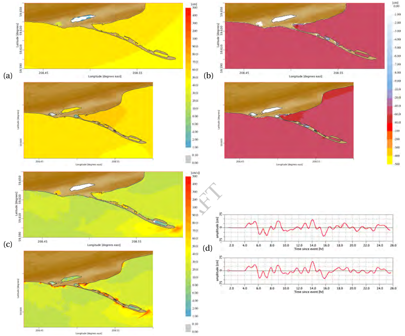
Figure 11: Comparisons for the FM (top insets) and the RM (bottom insets) C-grid results for the magnitude 9.3 synthetic scenario event with the source segment 50–59 on Aleutian–Alaska–Cascadia Subduction Zone (ACSZ) (Figure B.1, Table B.1). (a) Maximum and (b) minimum sea surface elevations, (c) maximum wave speeds at each C-grid point and (d) time histories of water surface elevations at the Homer forecast point.
