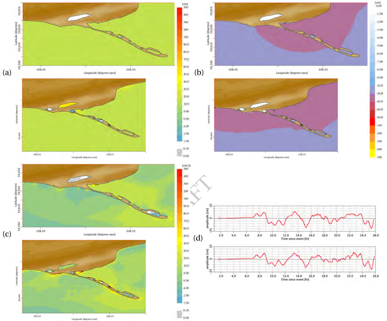
Figure 18: Comparisons for the FM (top insets) and the RM (bottom insets) C-grid results for the magnitude 9.3 synthetic scenario event with the source segment 1–10 on Kamchatka–Yap–Mariana–Izu–Bonin Subduction Zone (KISZ) (Figure B.5, Table B.5). (a) Maximum and (b) minimum sea surface elevations, (c) maximum wave speeds at each C-grid point and (d) time histories of water surface elevations at the Homer forecast point.
