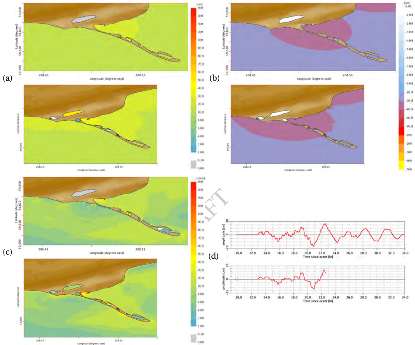
Figure 22: Comparisons for the FM (top insets) and the RM (bottom insets) C-grid results for the magnitude 9.3 synthetic scenario event with the source segment 1–10 on Manus–Oceanic Convergent Boundary Subduction Zone (MOSZ) (Figure B.6, Table B.6). (a) Maximum and (b) minimum sea surface elevations, (c) maximum wave speeds at each C-grid point and (d) time histories of water surface elevations at the Homer forecast point.
