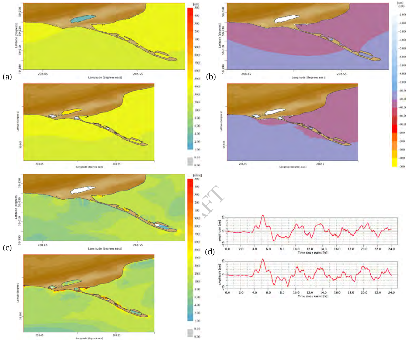
Figure 9: Comparisons for the FM (top insets) and the RM (bottom insets) C-grid results for the magnitude 9.3 synthetic scenario event with the source segment 16–25 on Aleutian–Alaska–Cascadia Subduction Zone (ACSZ) (Figure B.1, Table B.1). (a) Maximum and (b) minimum sea surface elevations, (c) maximum wave speeds at each C-grid point and (d) time histories of water surface elevations at the Homer forecast point.
