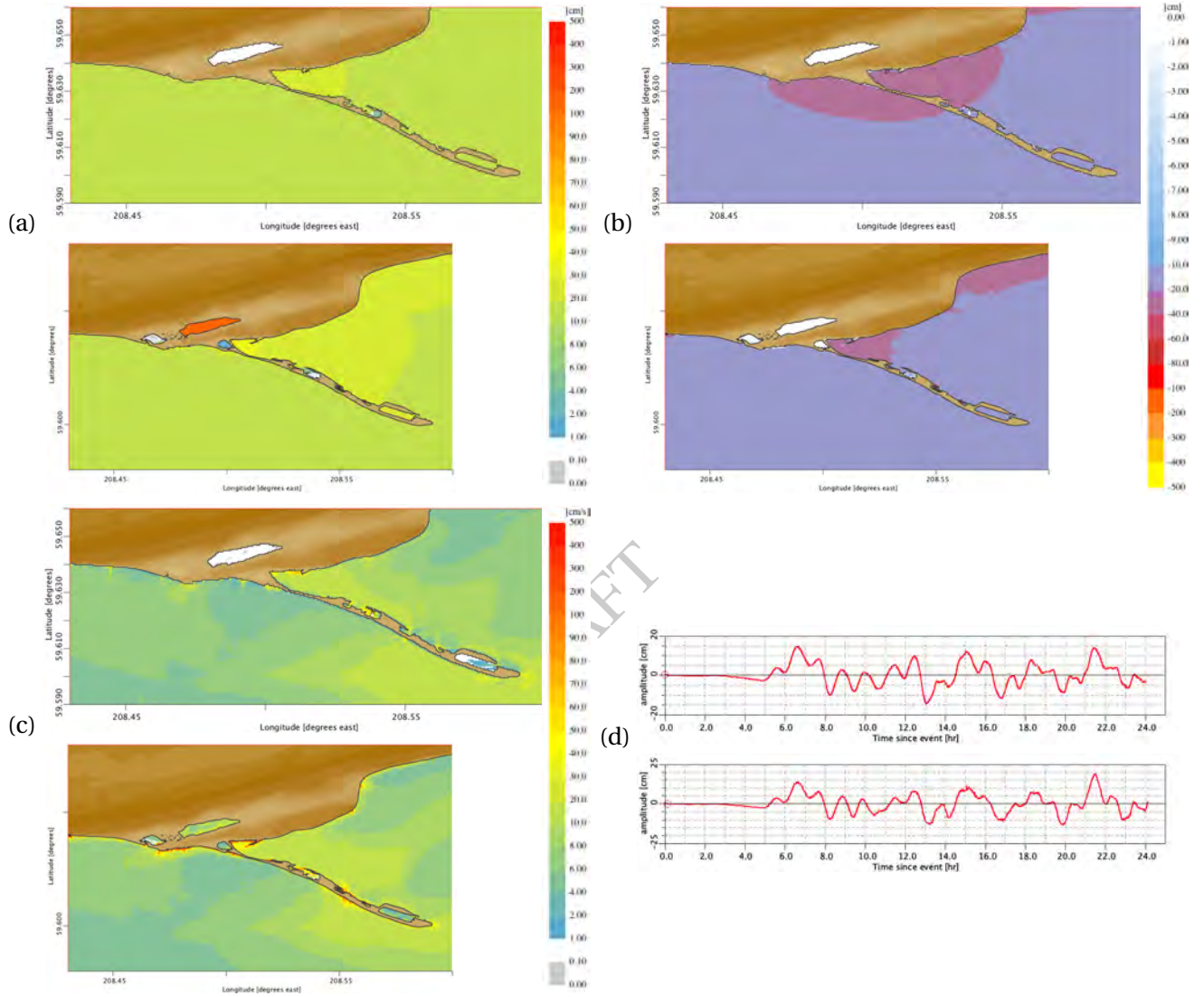
Figure 8: Comparisons for the FM (top insets) and the RM (bottom insets) C-grid results for the magnitude 9.3 synthetic scenario event with the source segment 6–15 on Aleutian–Alaska–Cascadia Subduction Zone (ACSZ) (Figure B.1, Table B.1). (a) Maximum and (b) minimum sea surface elevations, (c) maximum wave speeds at each C-grid point and (d) time histories of water surface elevations at the Homer forecast point.
