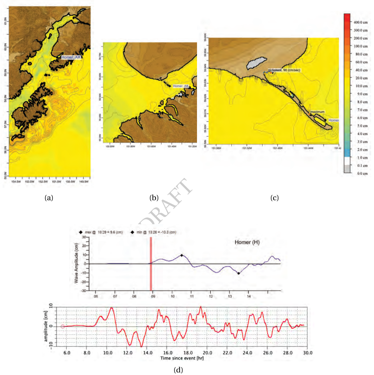
Figure C.3: Response of the Homer forecast model to synthetic scenario KISZ 22–31 ( \alpha = 25 ). Maximum sea surface elevation for (a) A-grid, b) B-grid, c) C-grid and d) sea surface elevation time series at the C-grid warning point. Sea surface elevation time series obtained during SIFT testing (upper inset) is compared the one obtained during model development (lower inset).
