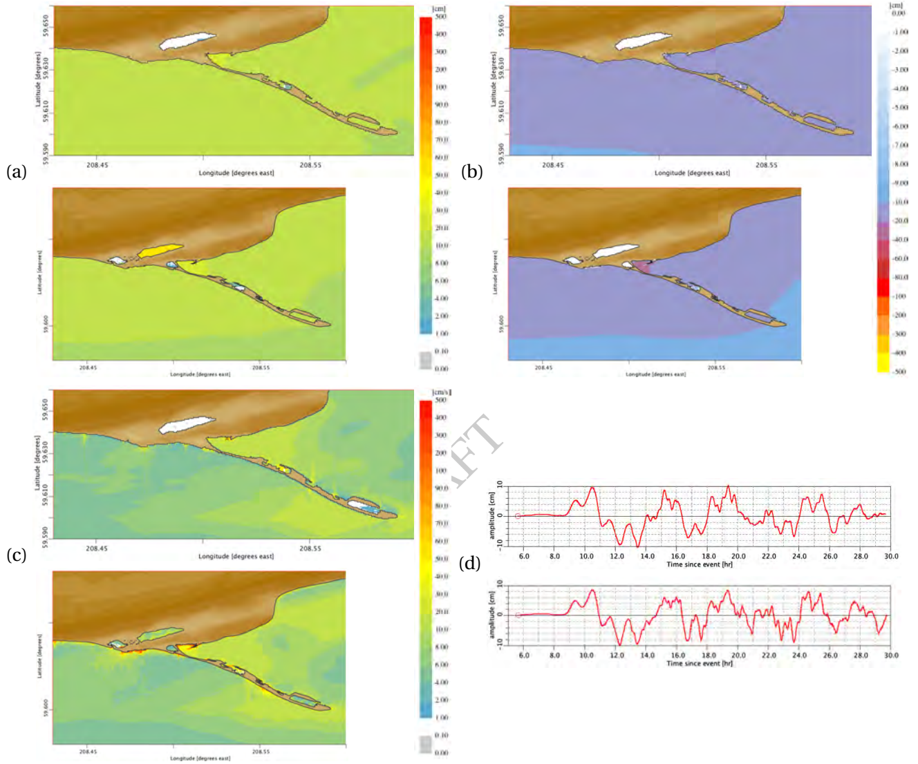
Figure 19: Comparisons for the FM (top insets) and the RM (bottom insets) C-grid results for the magnitude 9.3 synthetic scenario event with the source segment 22–31 on Kamchatka–Yap–Mariana–Izu–Bonin Subduction Zone (KISZ) (Figure B.5, Table B.5). (a) Maximum and (b) minimum sea surface elevations, (c) maximum wave speeds at each C-grid point and (d) time histories of water surface elevations at the Homer forecast point.
