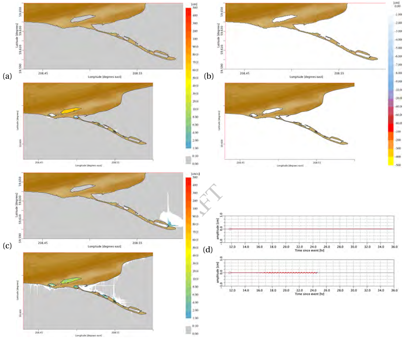
Figure 29: Comparisons for the FM (top insets) and the RM (bottom insets) C-grid results for the micro-tsunami synthetic scenario event with the source 19b on Eastern Philippines Subduction Zone (EPSZ) (Figure B.3, Table B.3). (a) Maximum and (b) minimum sea surface elevations, (c) maximum wave speeds at each C-grid point and (d) time histories of water surface elevations at the Homer forecast point.
