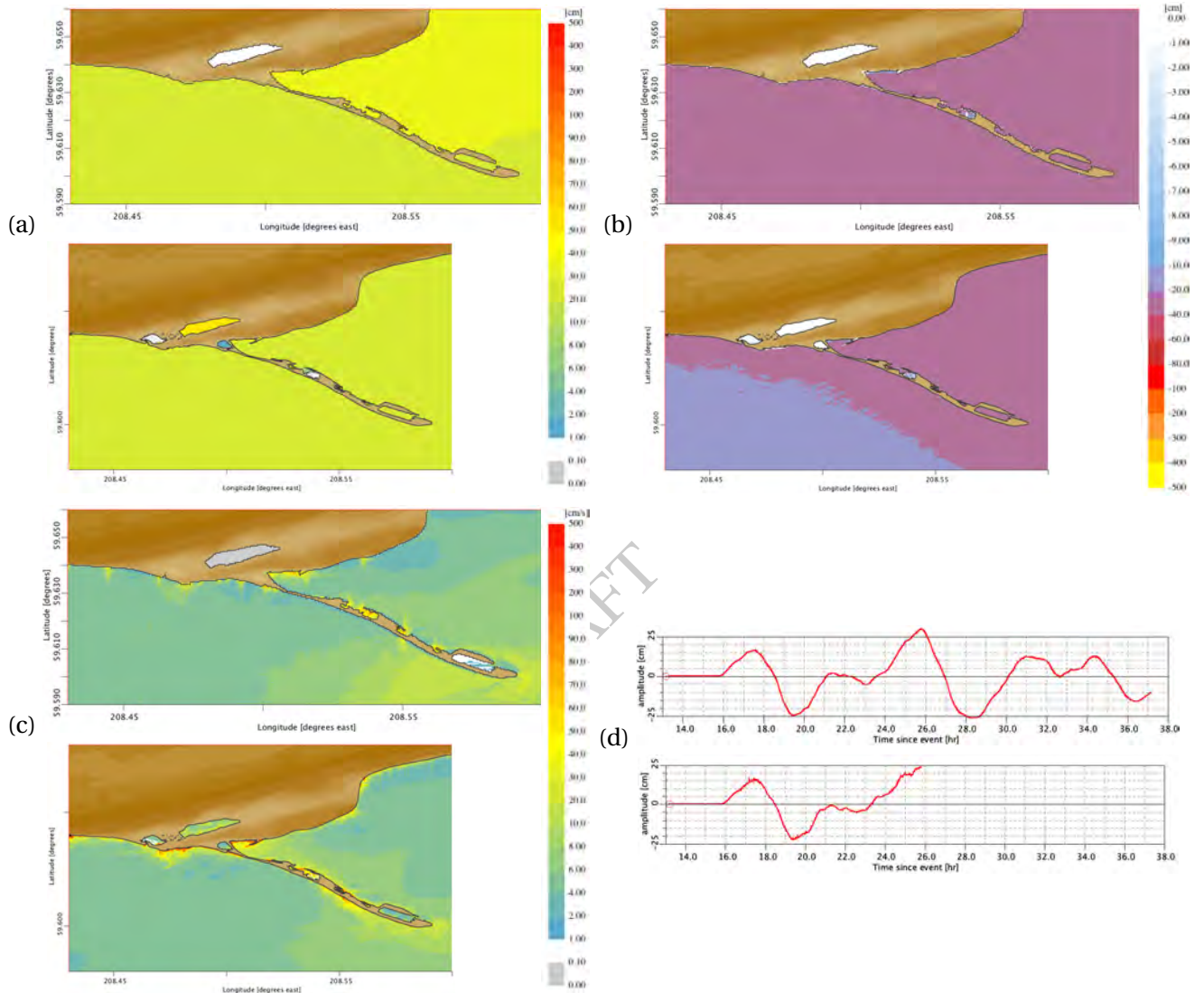
Figure 14: Comparisons for the FM (top insets) and the RM (bottom insets) C-grid results for the magnitude 9.3 synthetic scenario event with the source segment 37–46 on Central and South America Subduction Zone (CSSZ) (Figure B.2, Table B.2). (a) Maximum and (b) minimum sea surface elevations, (c) maximum wave speeds at each C-grid point and (d) time histories of water surface elevations at the Homer forecast point.
