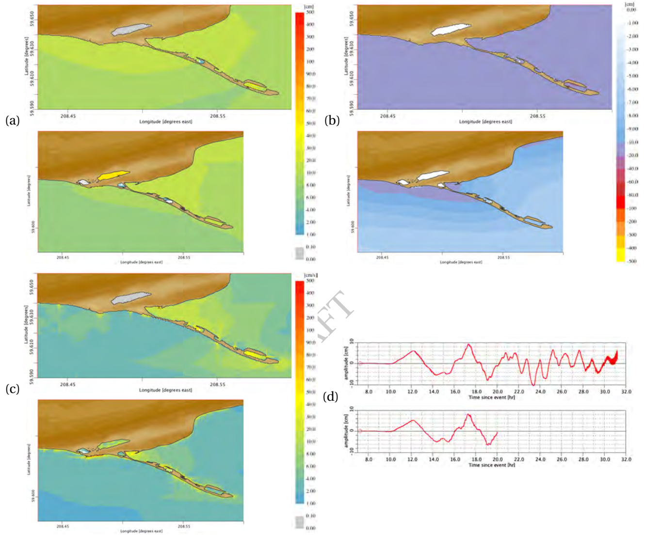
Figure 26: Comparisons for the FM (top insets) and the RM (bottom insets) C-grid results for the magnitude 9.3 synthetic scenario event with the source segment 12–21 on Ryukyu–Kyushu–Nankai Subduction Zone (RNSZ) (Figure B.11, Table B.11). (a) Maximum and (b) minimum sea surface elevations, (c) maximum wave speeds at each C-grid point and (d) time histories of water surface elevations at the Homer forecast point.
