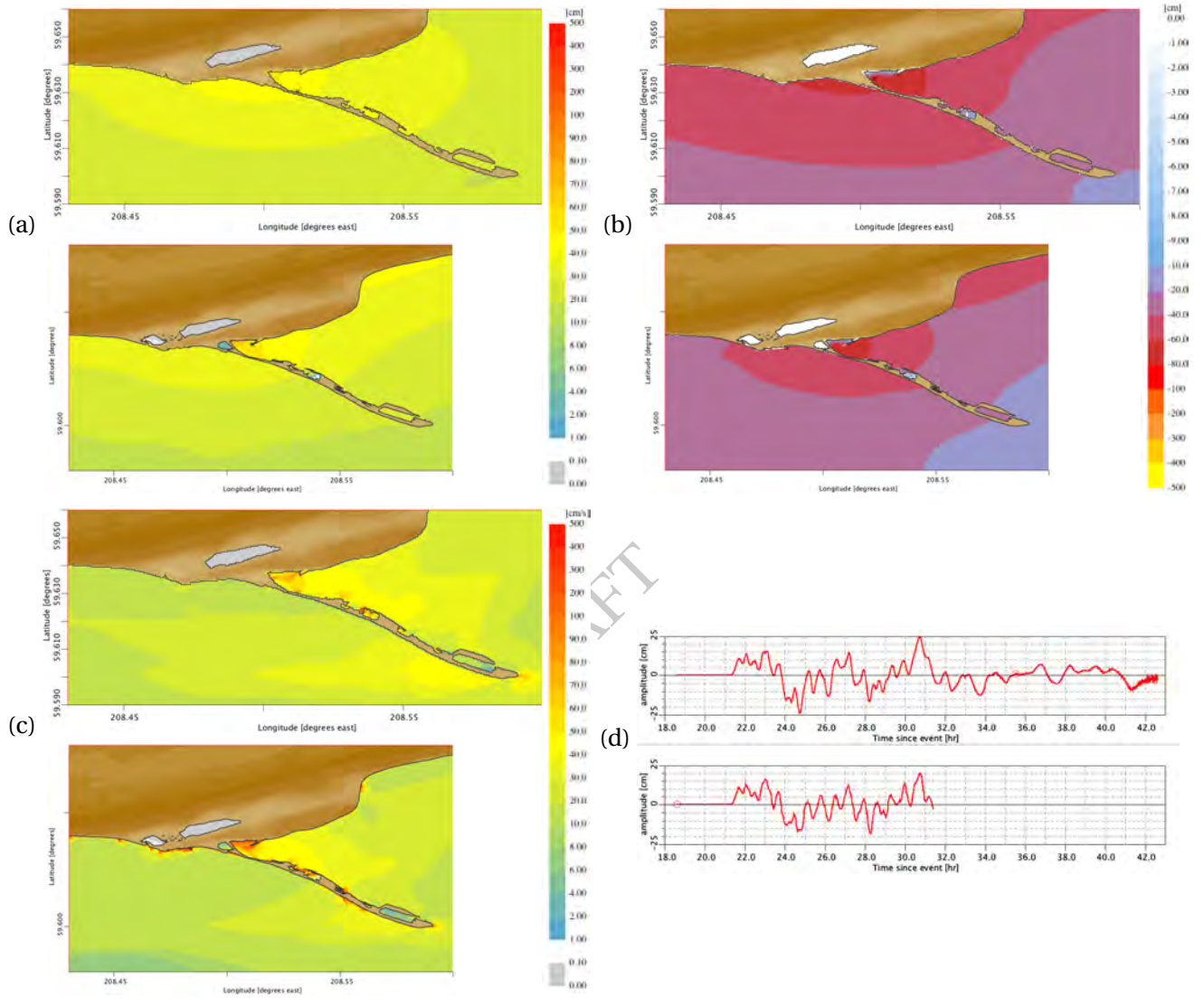
Figure 16: Comparisons for the FM (top insets) and the RM (bottom insets) C-grid results for the magnitude 9.3 synthetic scenario event with the source segment 102–111 on Central and South America Subduction Zone (CSSZ) (Figure B.2, Table B.2). (a) Maximum and (b) minimum sea surface elevations, (c) maximum wave speeds at each C-grid point and (d) time histories of water surface elevations at the Homer forecast point.
