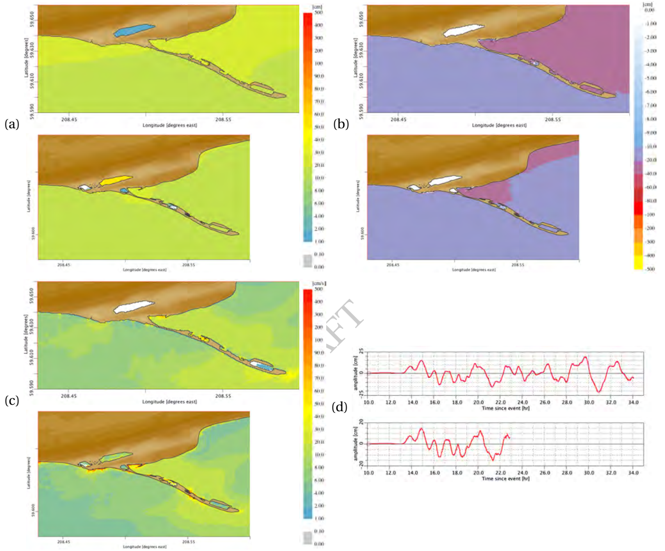
Figure 17: Comparisons for the FM (top insets) and the RM (bottom insets) C-grid results for the magnitude 9.3 synthetic scenario event with the source segment 6–15 on Eastern Philippines Subduction Zone (EPSZ) (Figure B.3, Table B.3). (a) Maximum and (b) minimum sea surface elevations, (c) maximum wave speeds at each C-grid point and (d) time histories of water surface elevations at the Homer forecast point.
