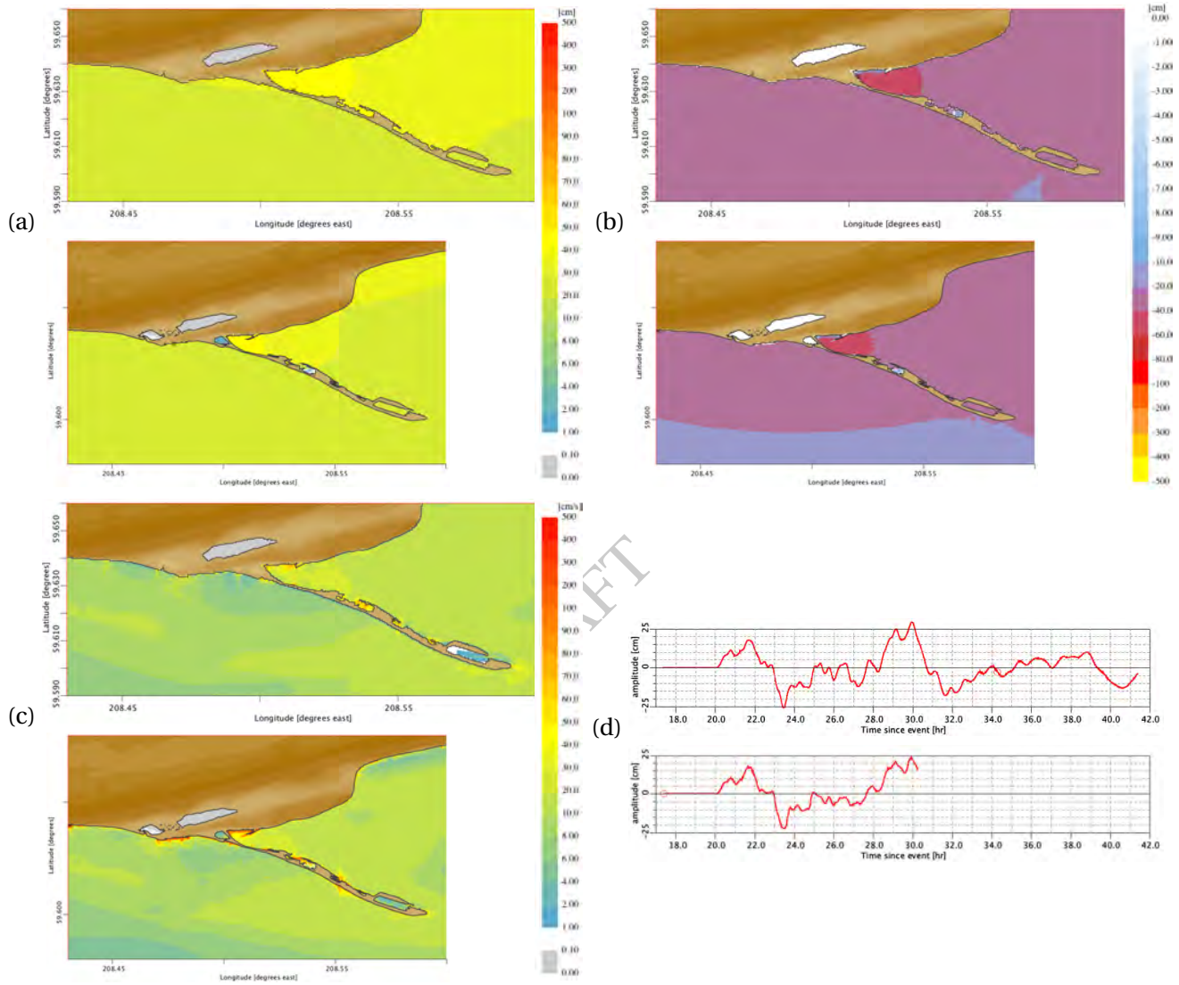
Figure 15: Comparisons for the FM (top insets) and the RM (bottom insets) C-grid results for the magnitude 9.3 synthetic scenario event with the source segment 89–98 on Central and South America Subduction Zone (CSSZ) (Figure B.2, Table B.2). (a) Maximum and (b) minimum sea surface elevations, (c) maximum wave speeds at each C-grid point and (d) time histories of water surface elevations at the Homer forecast point.
