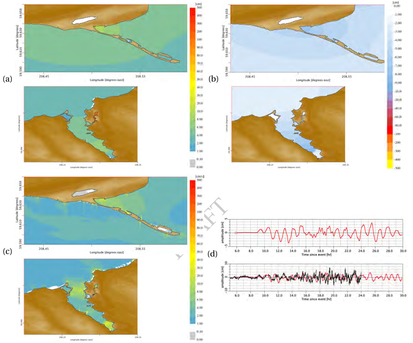
Figure 32: The FM (top insets) results for Homer, Alaska for the 11 March 2011 Japan tsunami. Results of the Seldovia, Alaska model is also given (lower insets) for the 11 March 2011 Japan tsunami. (a) Maximum and (b) minimum sea surface elevations, (c) maximum wave speeds at each C-grid point and (d) time histories of water surface elevations at the Homer forecast point (upper inset) and Seldovia tide gage (lower inset). Time histories of water surface elevations at the Seldovia tide gage is compared with the 11 March 2011 Japan tsunami measurement (black line).
