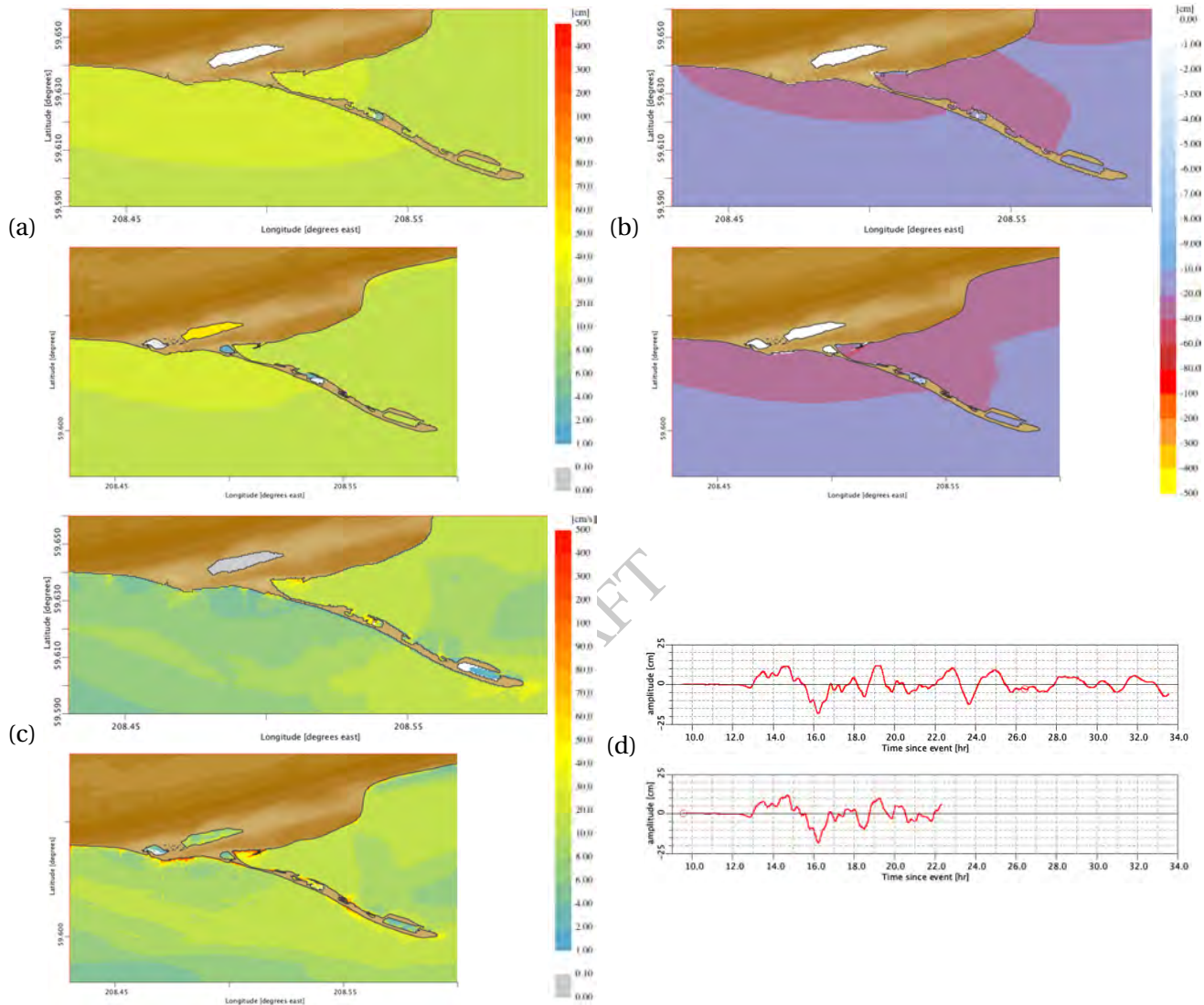
Figure 24: Comparisons for the FM (top insets) and the RM (bottom insets) C-grid results for the magnitude 9.3 synthetic scenario event with the source segment 30–39 on New Zealand–Kermadec–Tonga Subduction Zone (NTSZ) (Figure B.8, Table B.8). (a) Maximum and (b) minimum sea surface elevations, (c) maximum wave speeds at each C-grid point and (d) time histories of water surface elevations at the Homer forecast point.
