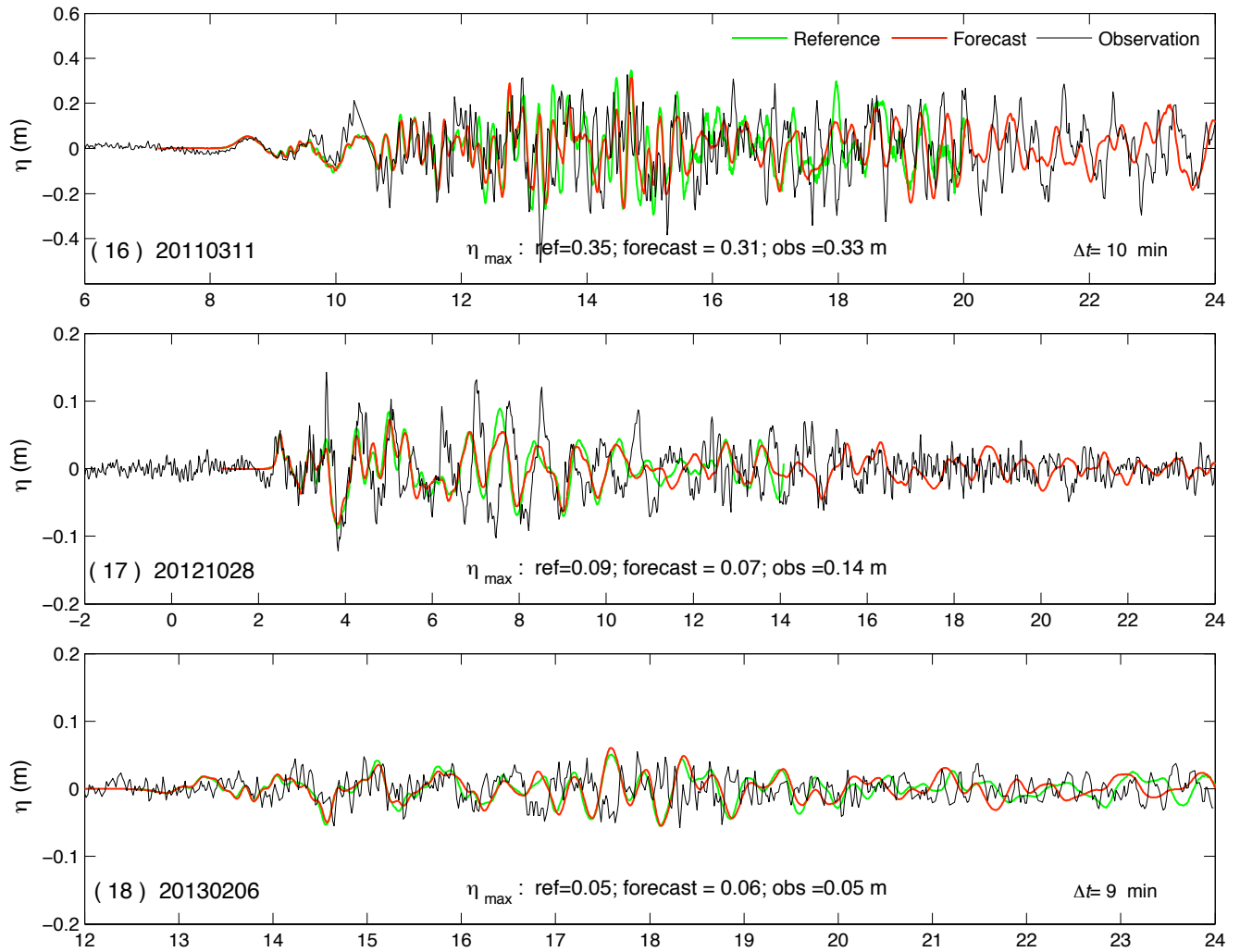
Figure 11 Observed and modeled tsunami amplitude time series for historical tsunamis. Black, observations; red forecast model; green, reference model.
