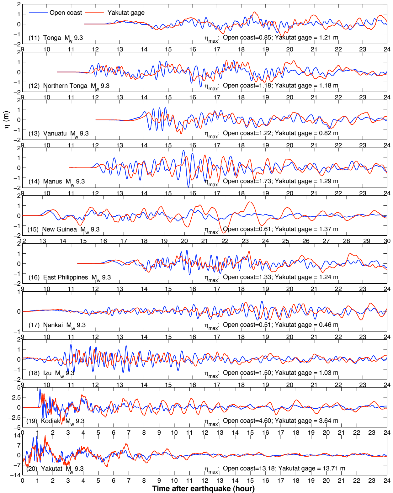
Figure 17 Time series of sea surface elevation \eta at the open coast and Yakutat tide gage for the 20 simulated magnitude-9.3 tsunamis. Results are from the forecast model.
