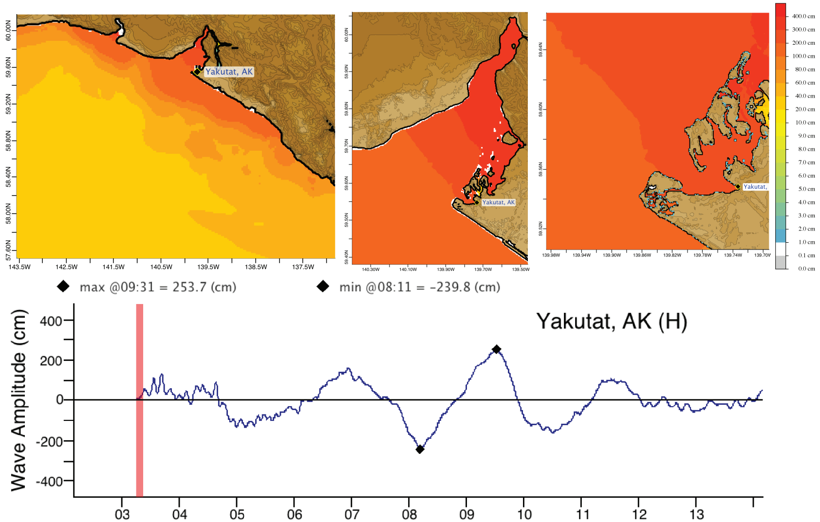
Figure C2: Response of the Yakutat forecast model to synthetic scenario ACSZ 56-65 ( \alpha=29 ). Maximum sea surface elevation for (a) A-grid, b) B-grid, c) C-grid. Sea surface elevation time series at the C-grid warning point (d).
