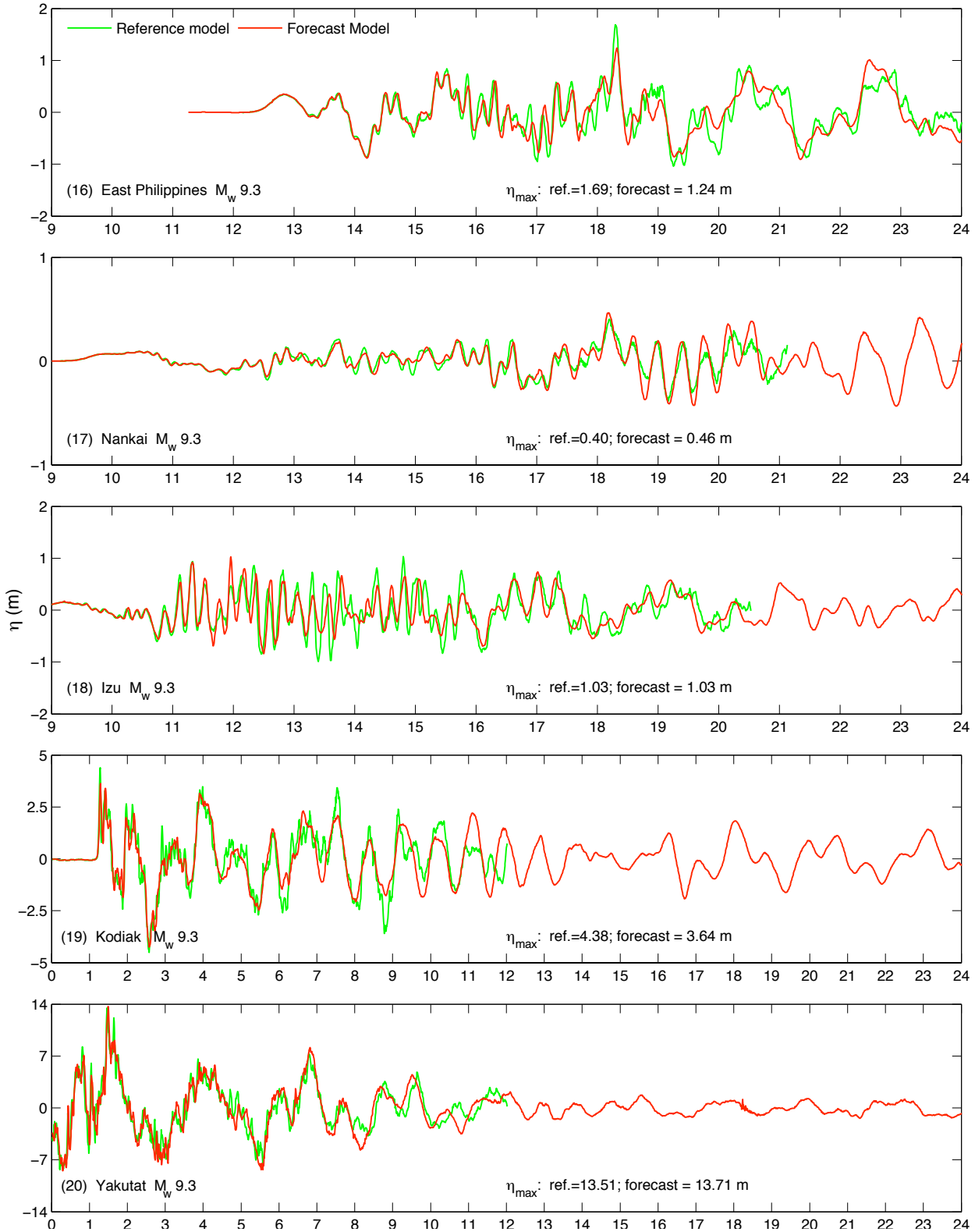
Figure 12 Modeled \eta time series by the Yakutat reference and forecast models for simulated magnitude-9.3 tsunamis.
