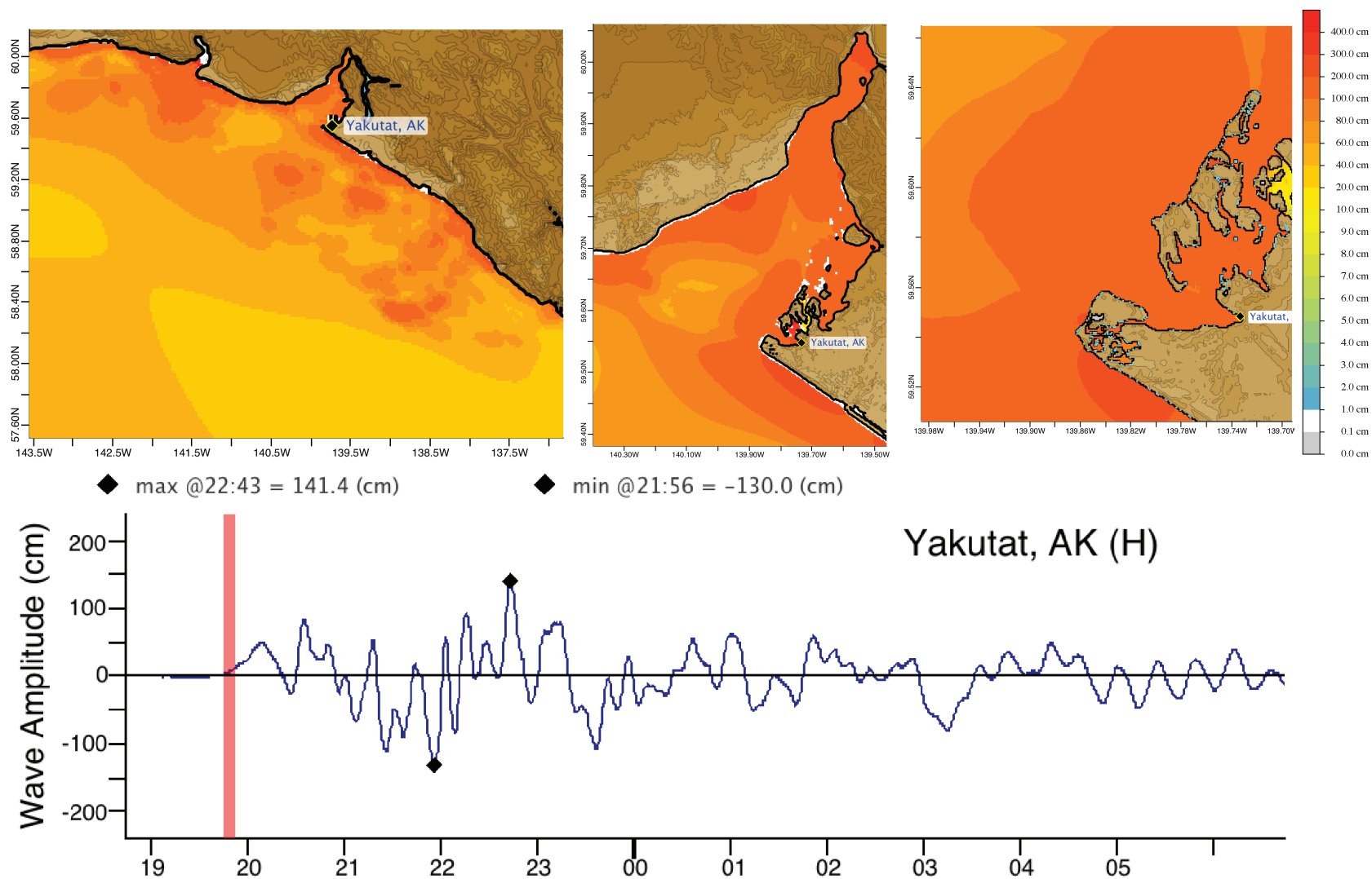
Figure C3: Response of the Yakutat forecast model to synthetic scenario CSSZ 89-98( \alpha=29 ). Maximum sea surface elevation for (a) A-grid, b) B-grid, c) C-grid. Sea surface elevation time series at the C-grid warning point (d).
