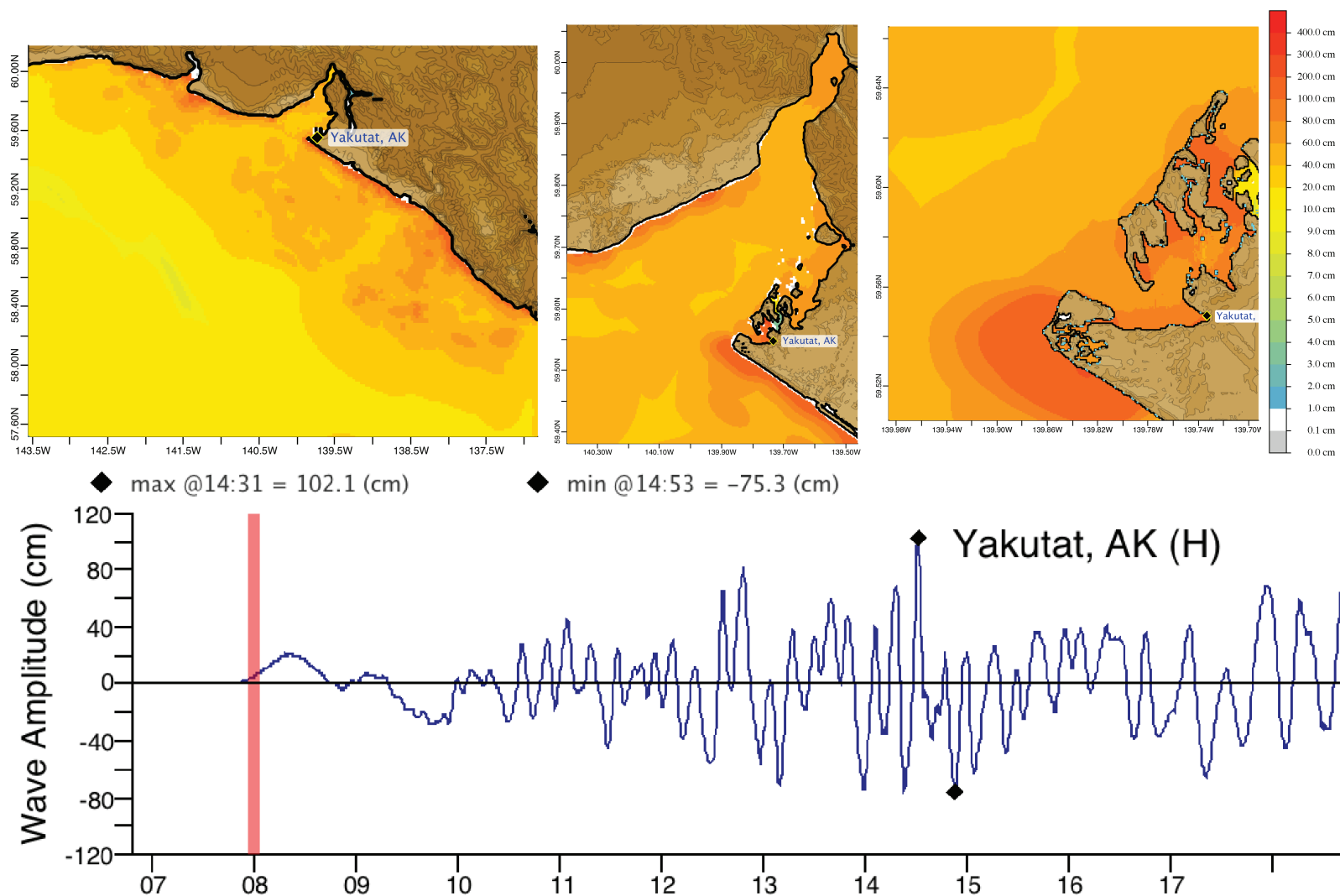
Figure C1: Response of the Yakutat forecast model to synthetic scenario KISZ 22-31 ( \alpha=29 ). Maximum sea surface elevation for (a) A-grid, b) B-grid, c) C-grid. Sea surface elevation time series at the C-grid warning point (d).
