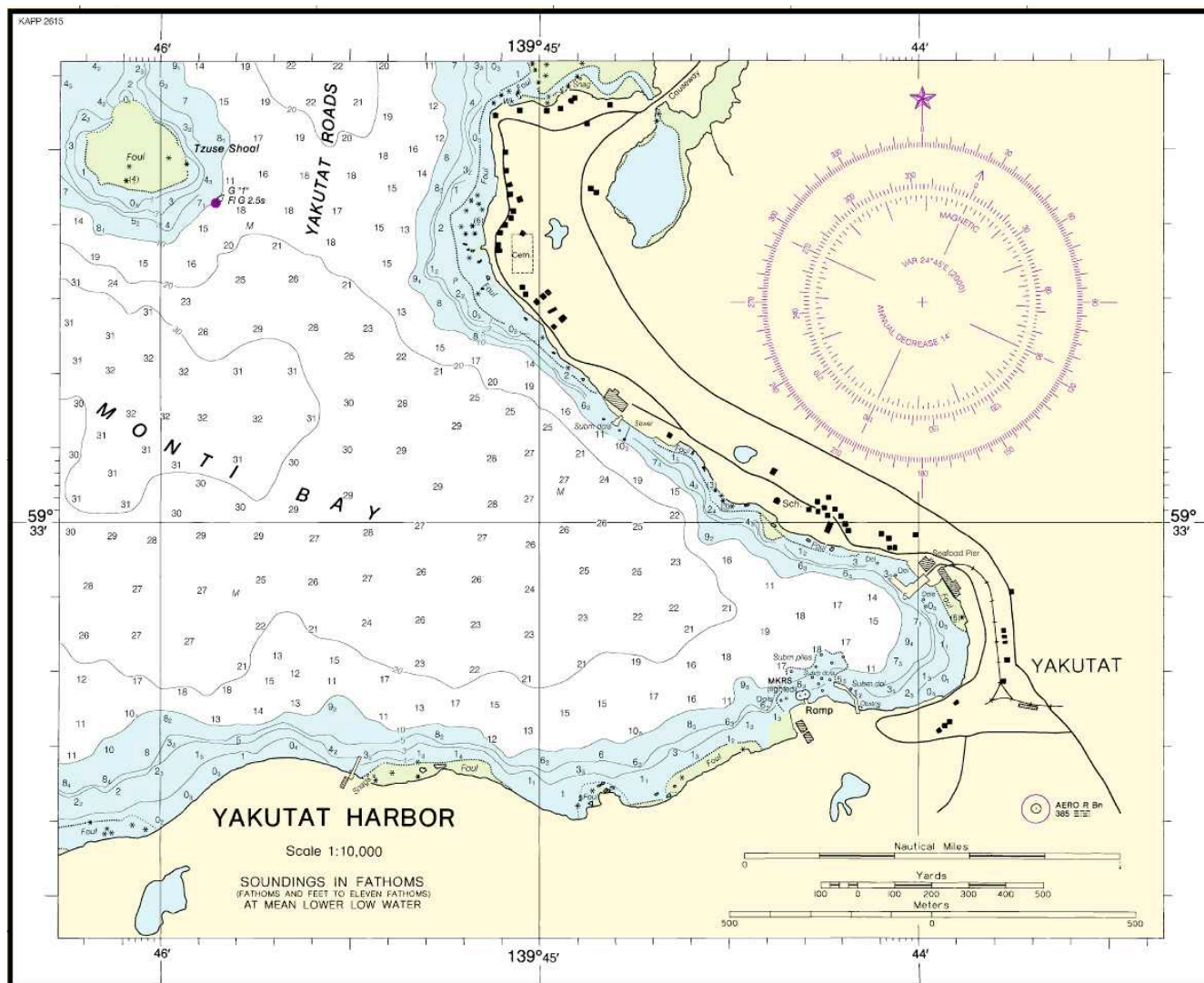
Figure 5 NOAA charts show (a) Yakutat and (b) Yakutat Harbor (NOAA Chart 16716). Soundings in fathoms at Mean Lower Low Water. Contour and summit elevation values are in feet above Mean Sea Level.
