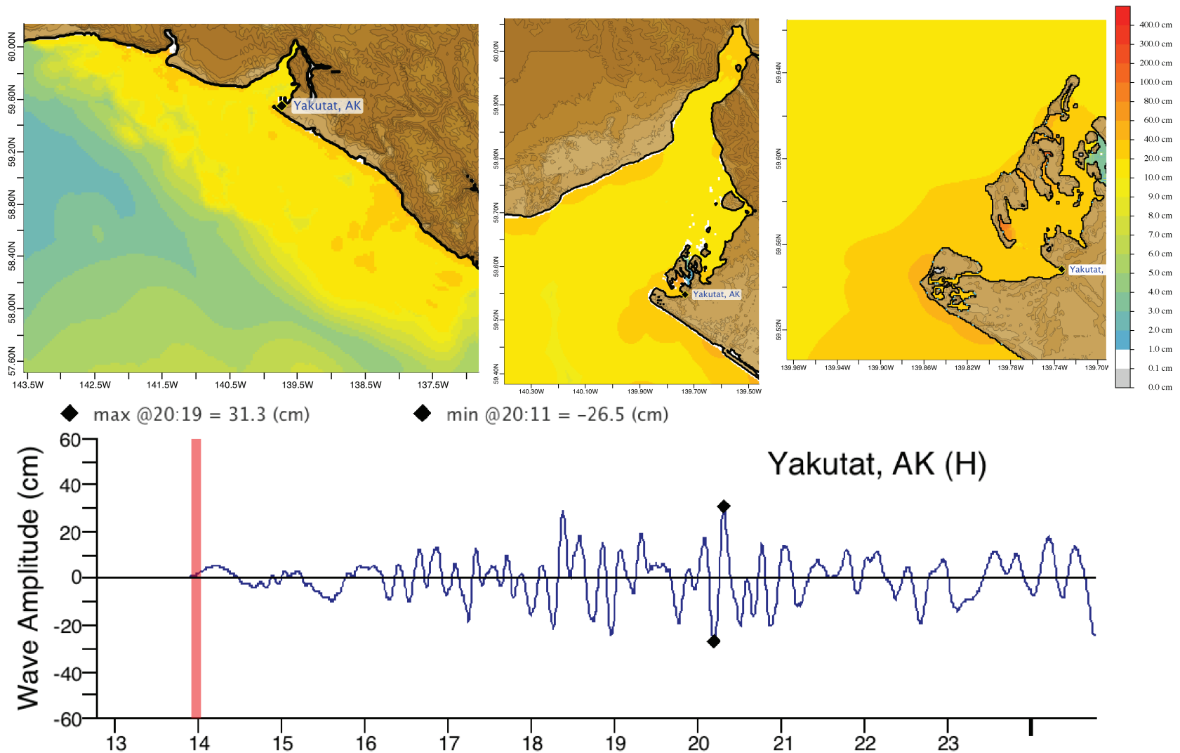
Figure C5: Response of the Yakutat forecast model to the 2011 Tohoku tsunami. Maximum sea surface elevation for (a) A-grid, b) B-grid, c) C-grid. Sea surface elevation time series at the C-grid warning point (d).
