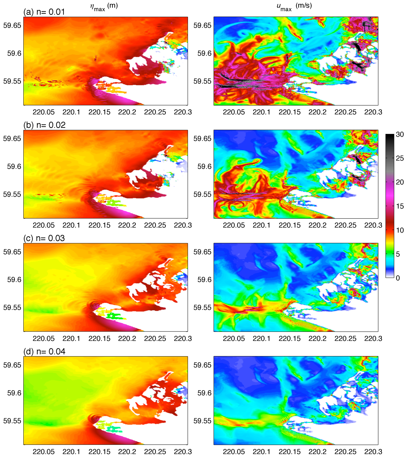
Figure 10 Sensitivity of maximum amplitude and current to friction coefficients for the Yakutat forecast model for a local magnitude-9.3 tsunami (#20).
