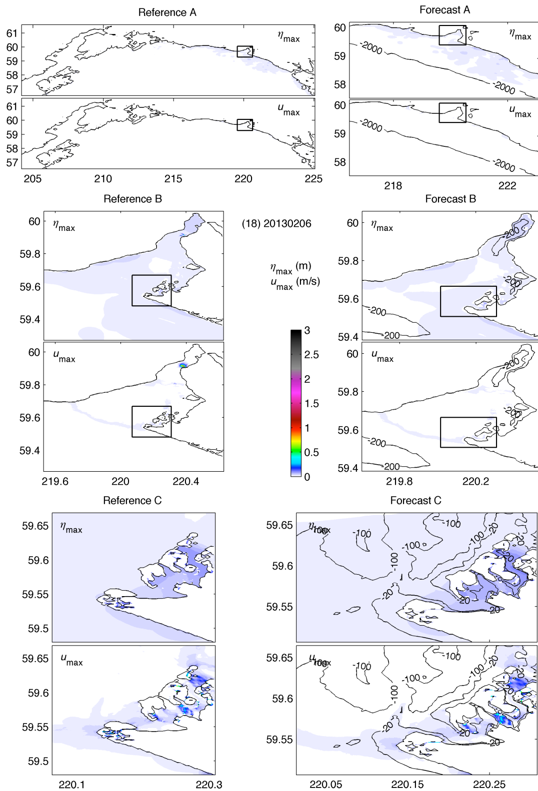
Figure 19 Maximum water elevation and current computed by the Yakutat reference and forecast models for 18 historical tsunamis.
