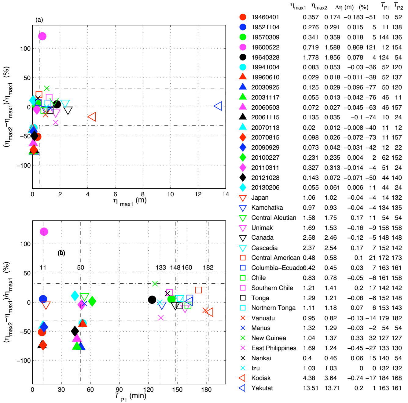
Figure 15 (a) Forecast error/uncertainty in the \eta_{\max} at the Yakutat tide gage for the 38 tsunamis. (b) Uncertainty vs. peak period. Filled markers, 18 historic tsunamis; open markers, 20 simulated magnitude- 9.3 tsunamis. \eta_{\max 1} and T_{p1} , maximum water elevation and peak period at the gage from either observations or the reference model( when the observations are not available). \eta_{\max 2} and T_{p2} , maximum water surface elevation and peak period at the gage computed by the forecast model.
