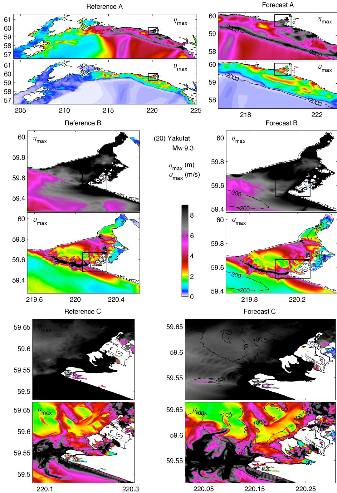
Figure 20 Maximum water elevation and current computed by the Yakutat reference and forecast models for 20 simulated magnitude-9.3 tsunamis.
