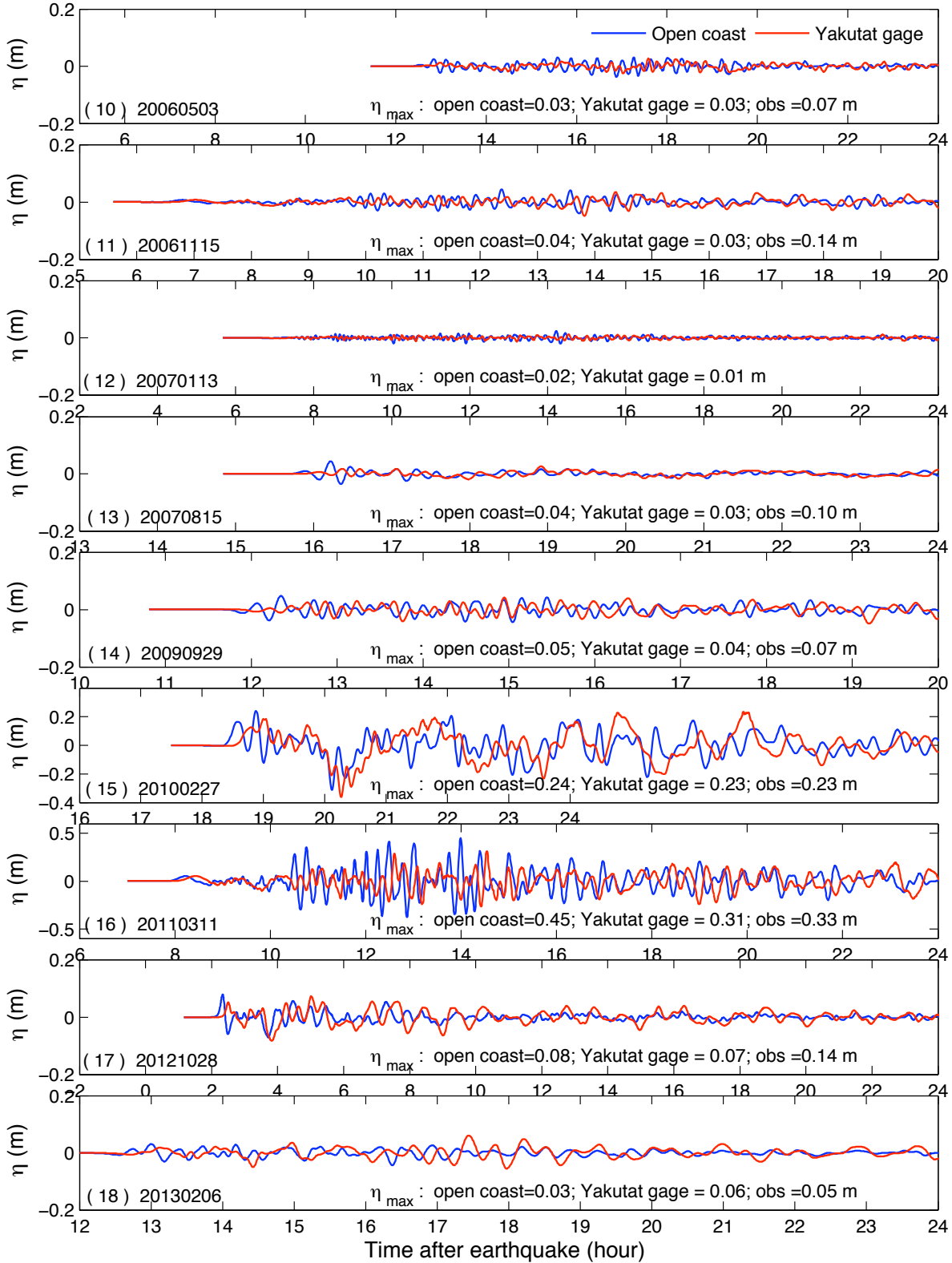
Figure 16 Time series of sea surface elevation \eta at the open coast and Yakutat gage for the historical tsunamis. Results are from the forecast model.
