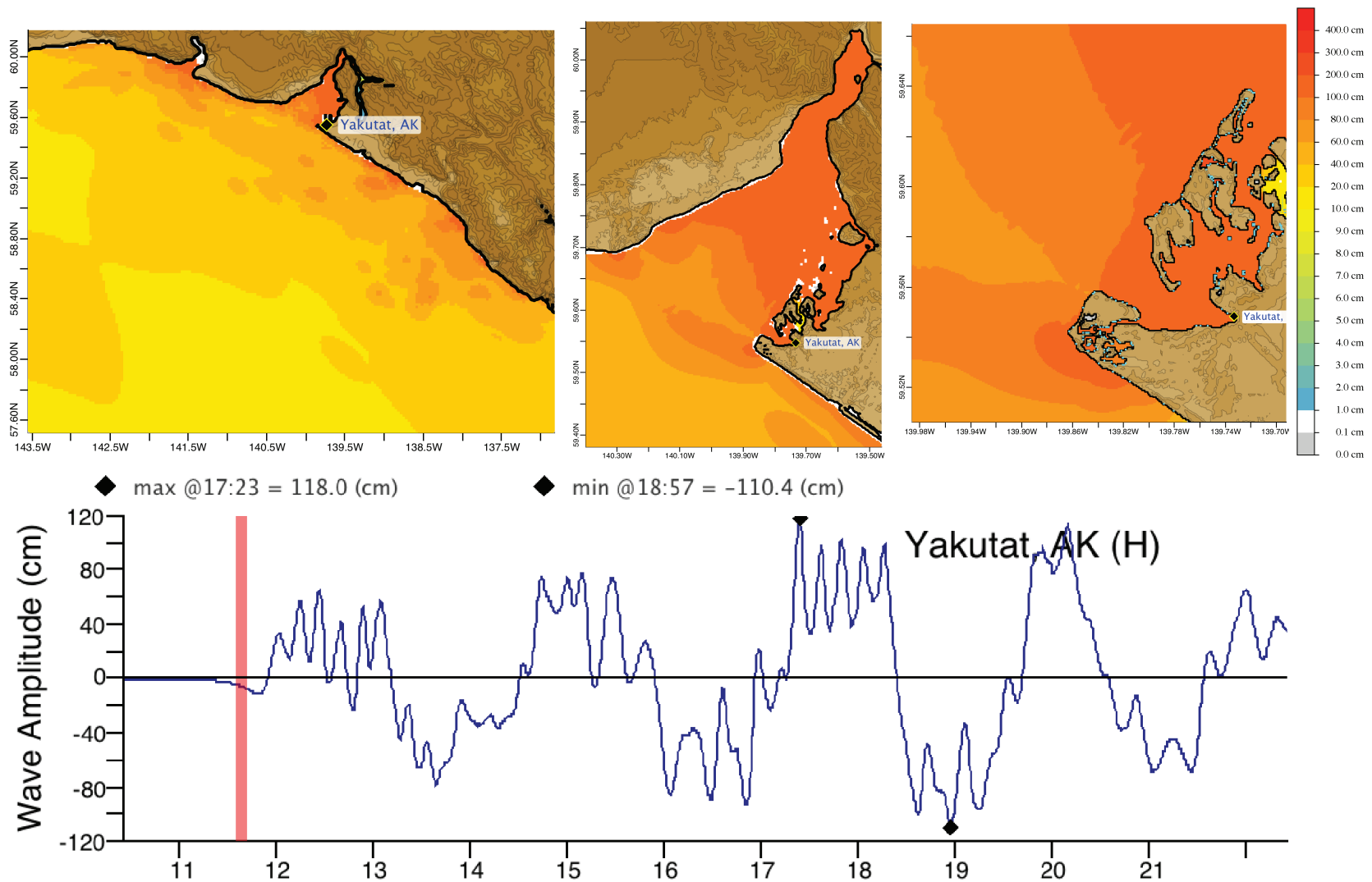
Figure C4: Response of the Yakutat forecast model to synthetic scenario NTSZ 30-39 ( \alpha=29 ). Maximum sea surface elevation for (a) A-grid, b) B-grid, c) C-grid. Sea surface elevation time series at the C-grid warning point (d).
