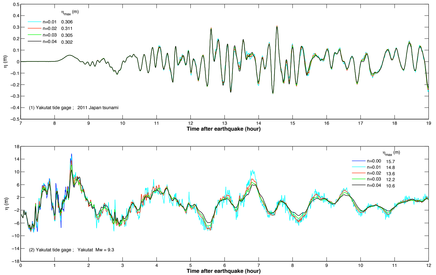
Figure 9 Sensitivity of \eta to friction coefficients for the Yakutat forecast model. (1) The 2011 Japan tsunami; (2) A local magnitude-9.3 tsunami (#20).
