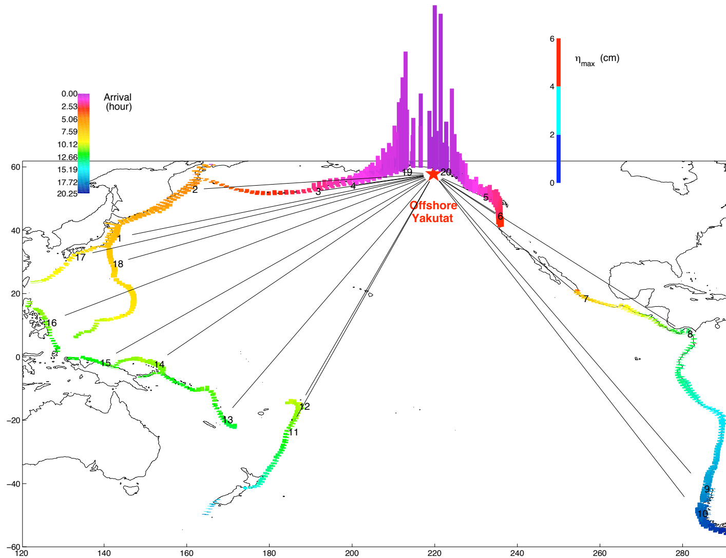
Figure 2 Maximum sea surface elevation ( \eta_{\max} ) at Yakutat offshore from 1129 tsunamis from NCTR's pre-computed propagation database in Pacific. Each tsunami was originated from a 100x50 km magnitude-7.5 earthquake. Heights and colors of the bars represent \eta_{\max} and the first arrival at the offshore point (219.75°E, 57.7936°N; water depth = 3278 m) respectively. Points labeled 1-20 are the locations of simulated magnitude-9.3 tsunamis.
